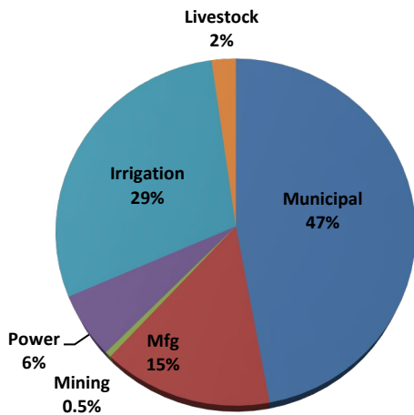
2019 Surface Water Estimates by Category
