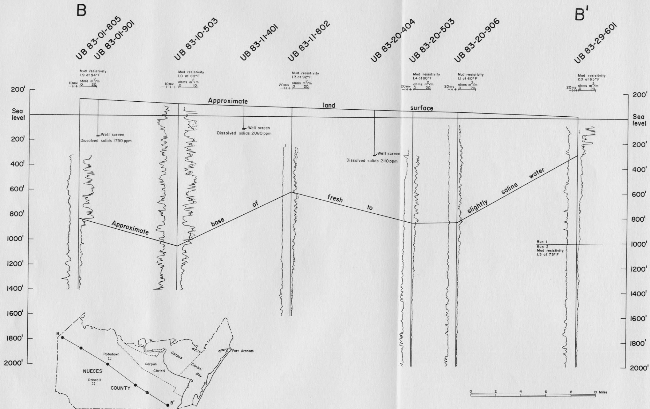
Figure 17 Geologic Section B-B', Nueces County
