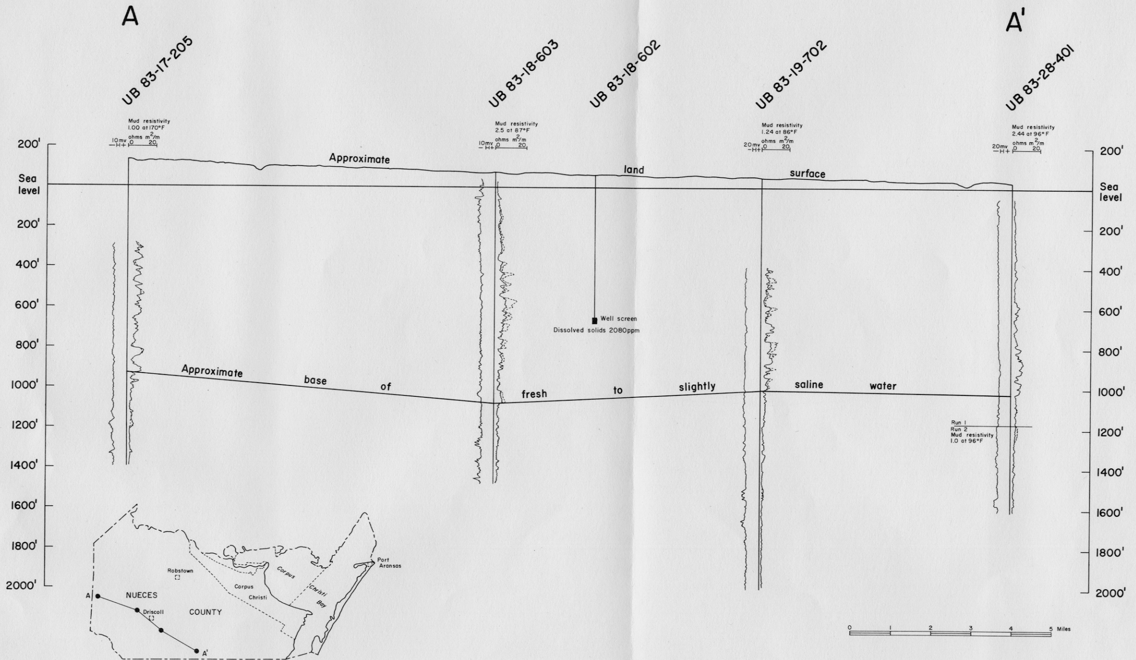
Figure 16 Geologic Section A-A', Nueces County
