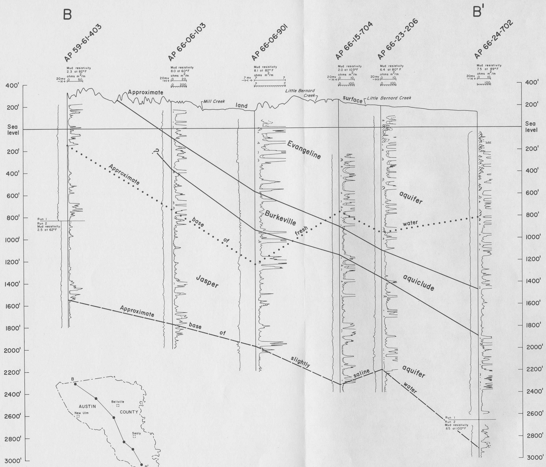
Figure 24 Section B-B', Showing Hydrologic Units and the Approximate Base of Fresh and Slightly Saline Water
