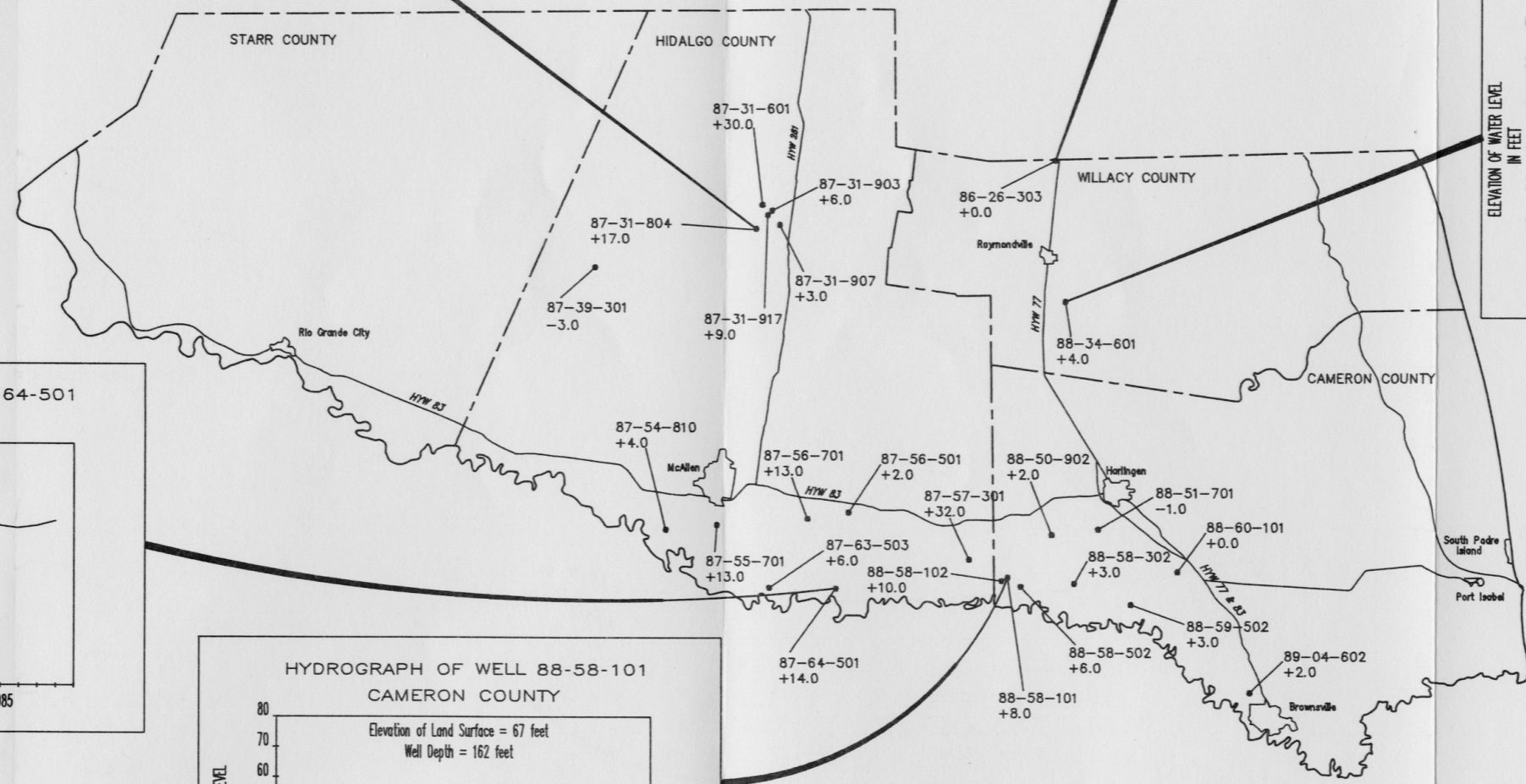
Figure 9 WATER-LEVEL RISE AND DECLINE IN SELECTED WELLS IN THE LOWER RIO GRANDE VALLEY, 1970 THROUGH 1988
