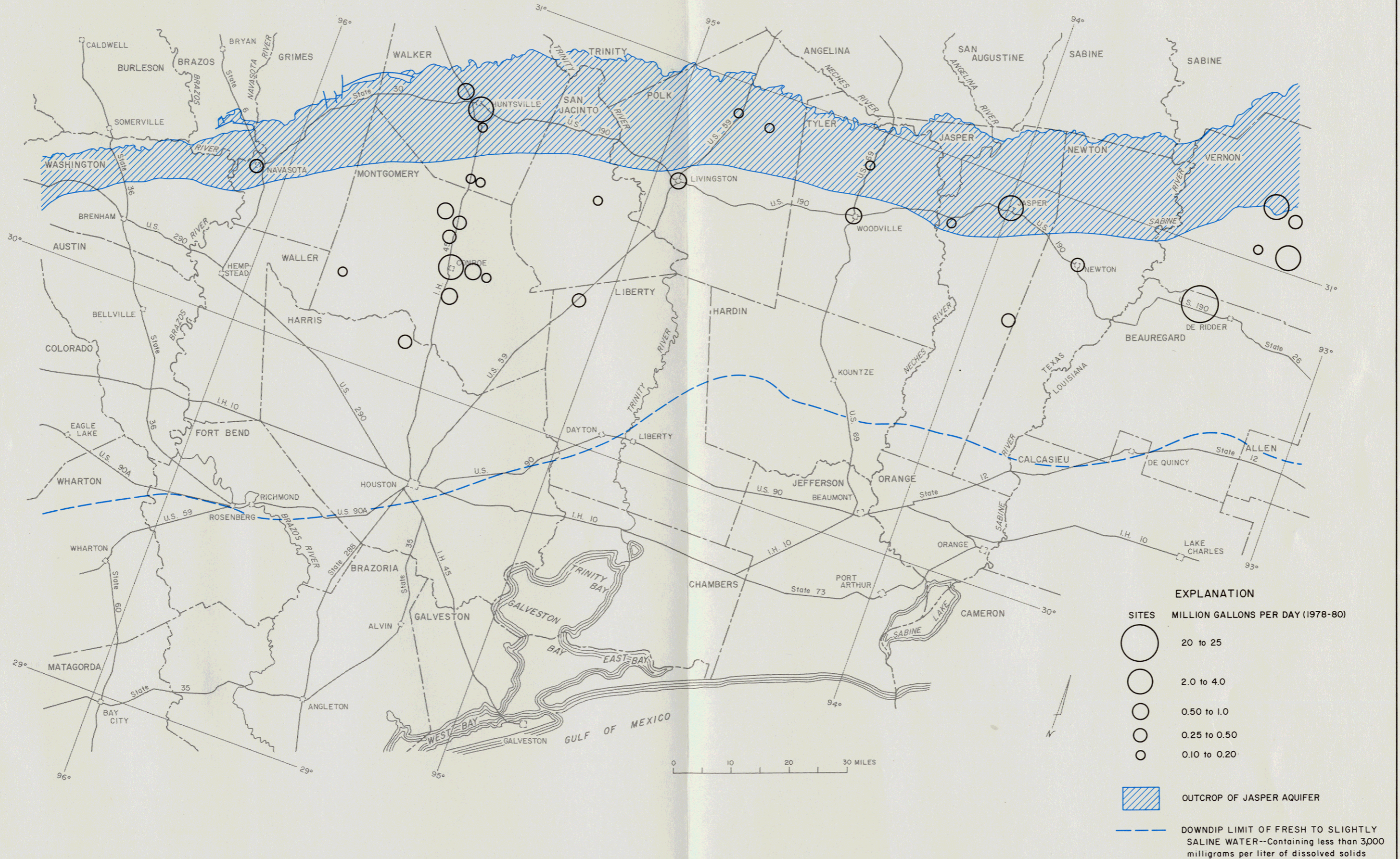
Figure 9 Sites Where Moderate to Large Volumes of Water Are Pumped From the Jasper Aquifer
