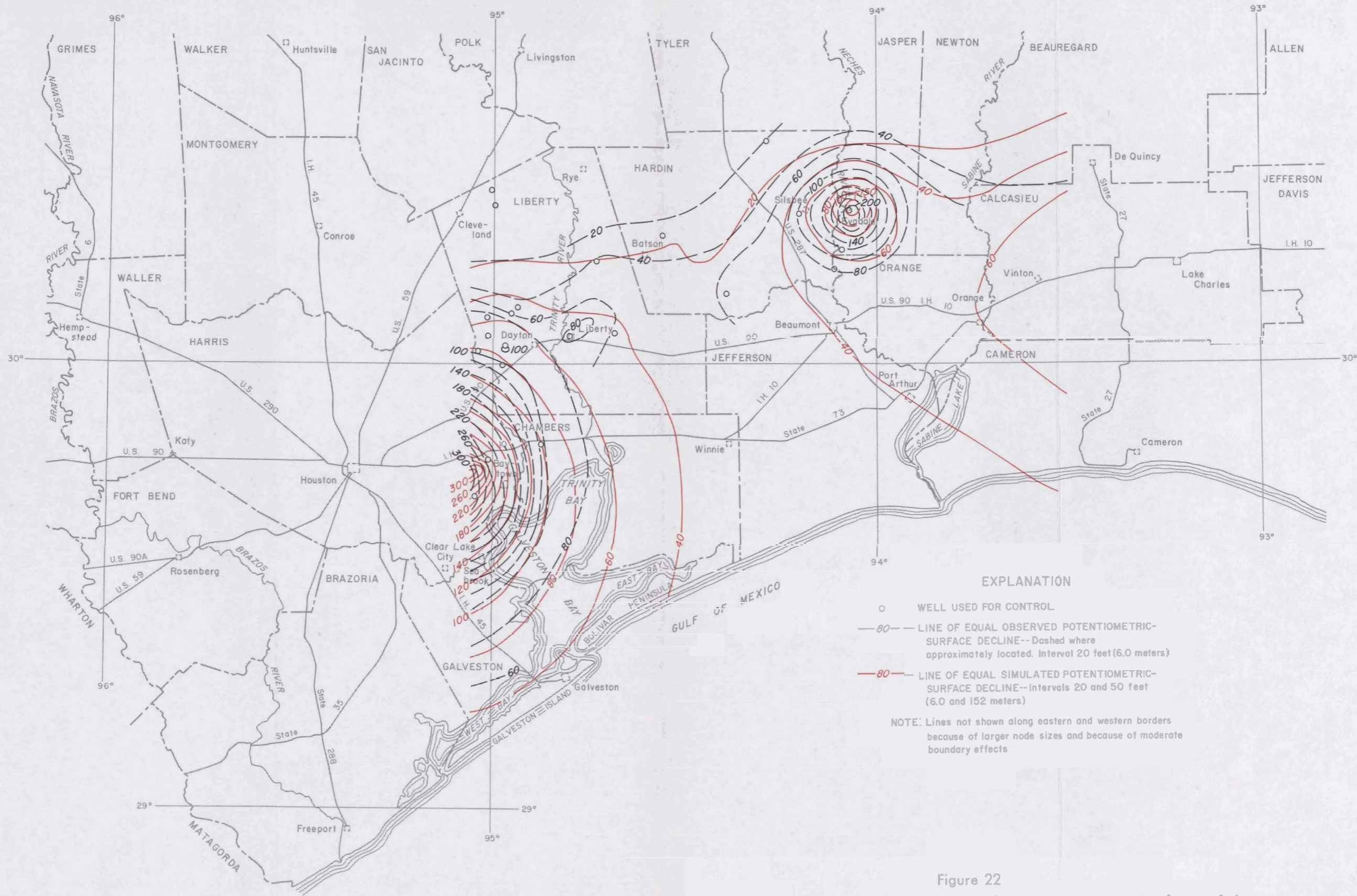
Observed and Simulated Declines in the Potentiometric Surface of the Evangeline Aquifer, Eastern-Subregion Model, 1900-1970
