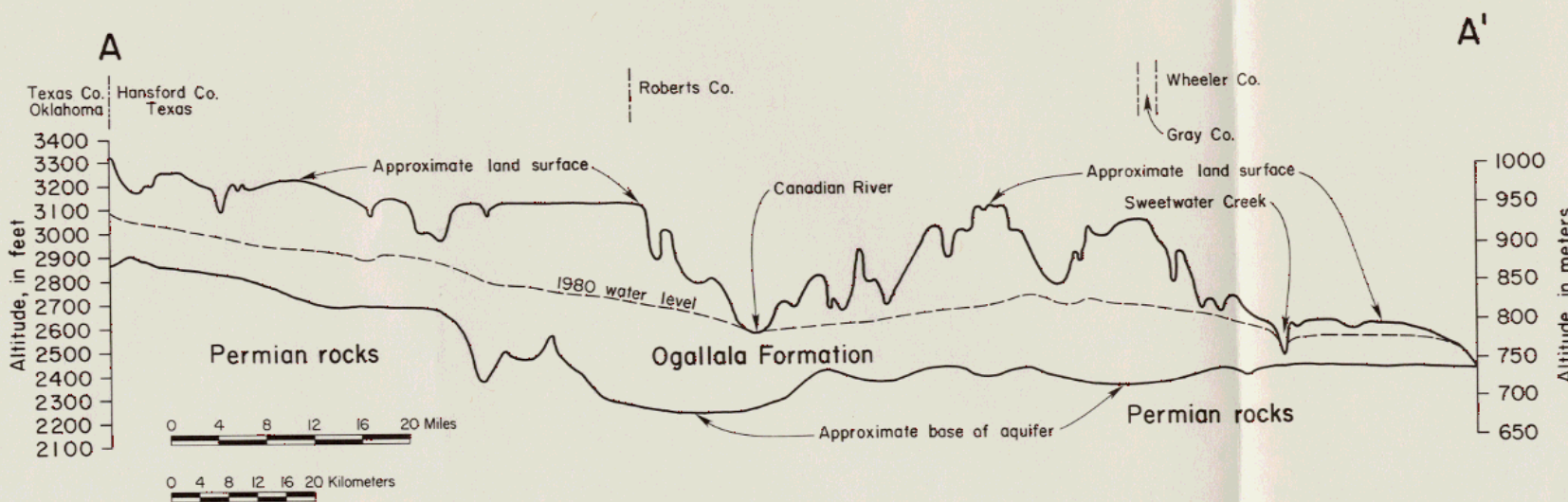
Figure 22 Generalized Geologic Section A-A'
