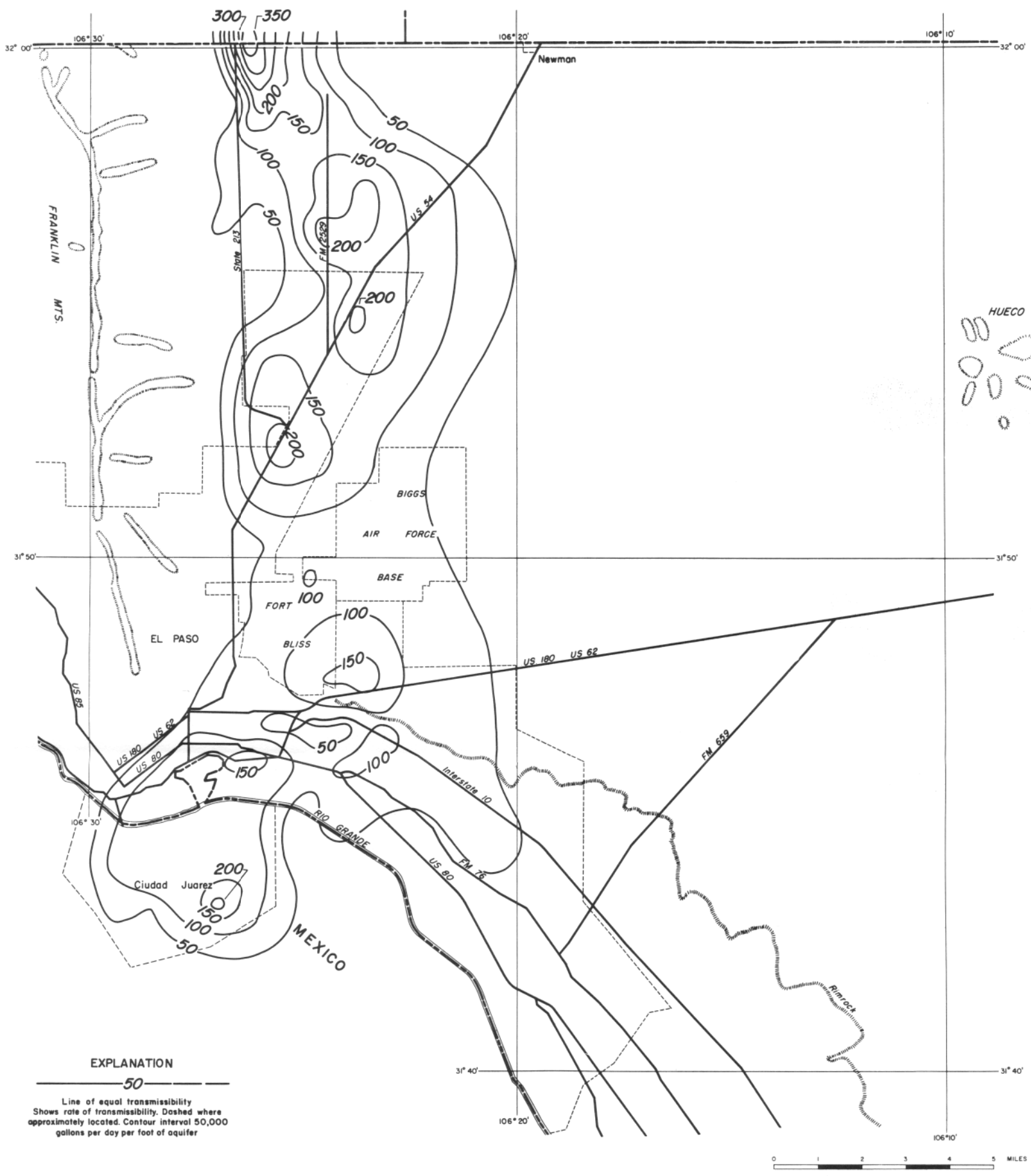
Figure 8 Approximate Transmissibility of Fresh Water-Bearing Deposits in the Hueco Bolson
