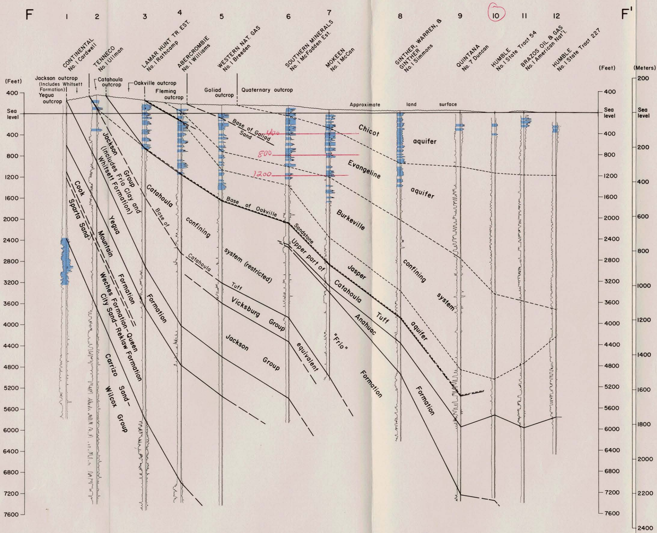
Figure 7 Stratigraphic and Hydrogeologic Section F-F'
