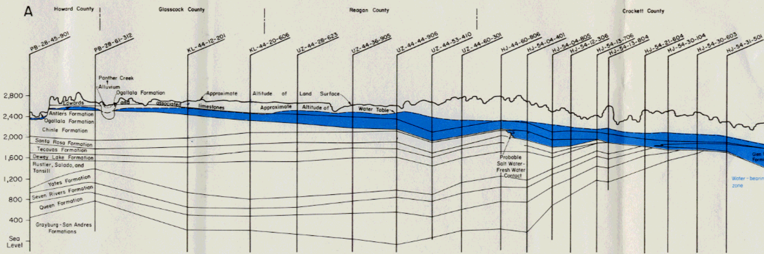
Figure 10 Geologic Section A-A' Howard County to Crockett County
