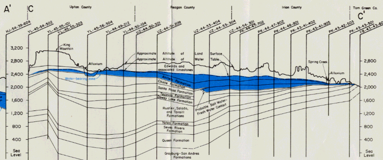
Figure 12 Geologic Section C-C' Upton County to Tom Green County
