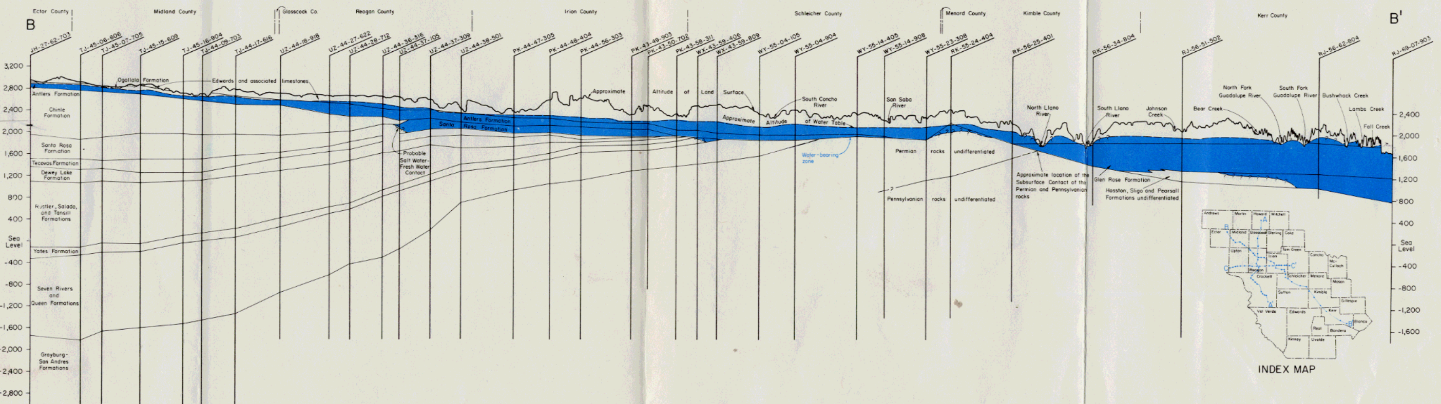
Figure 11 Geologic Section B-B' Ector County to Kerr County
