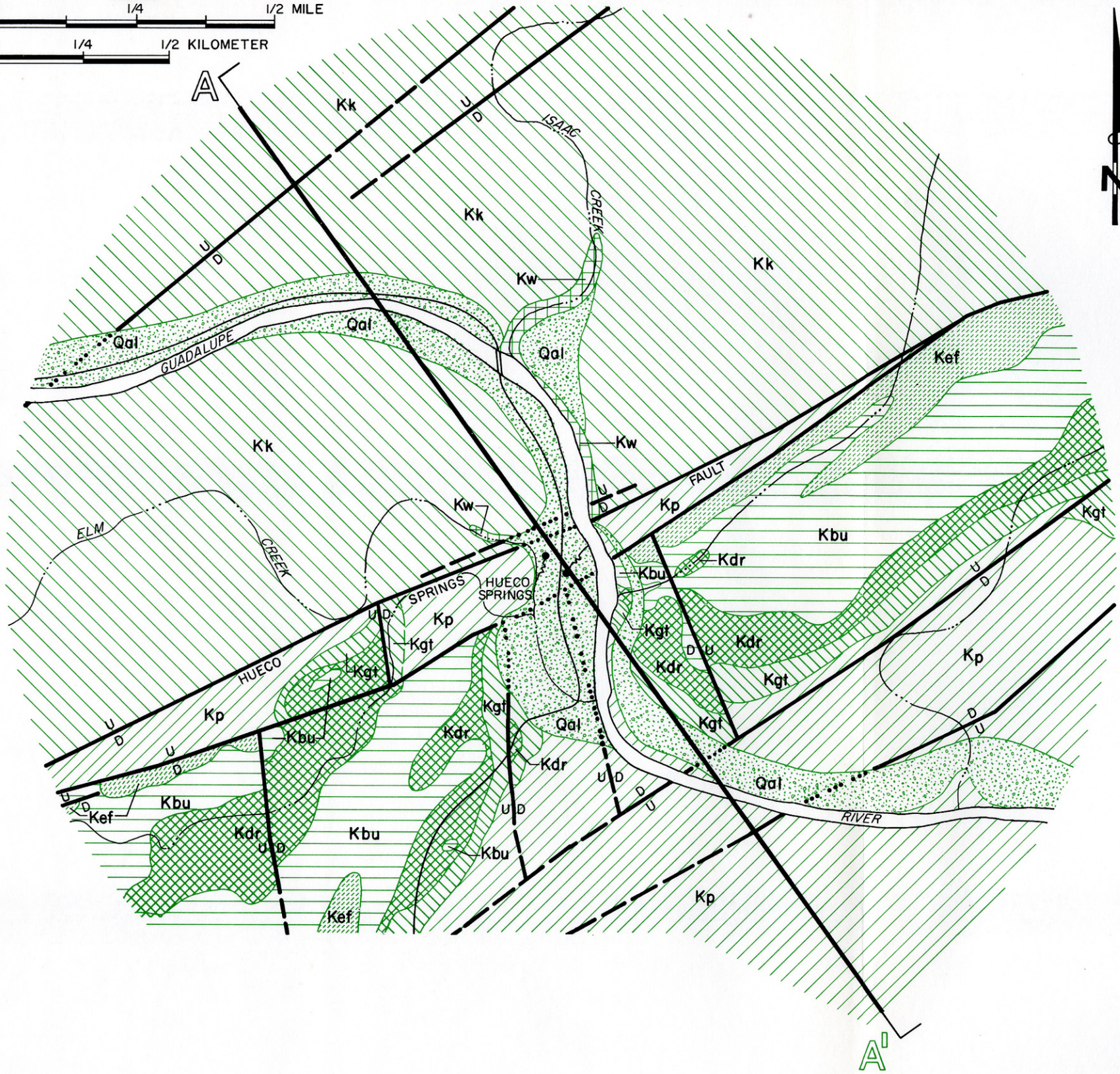
Figure 9 Surface Geology of Hueco Springs Locality
