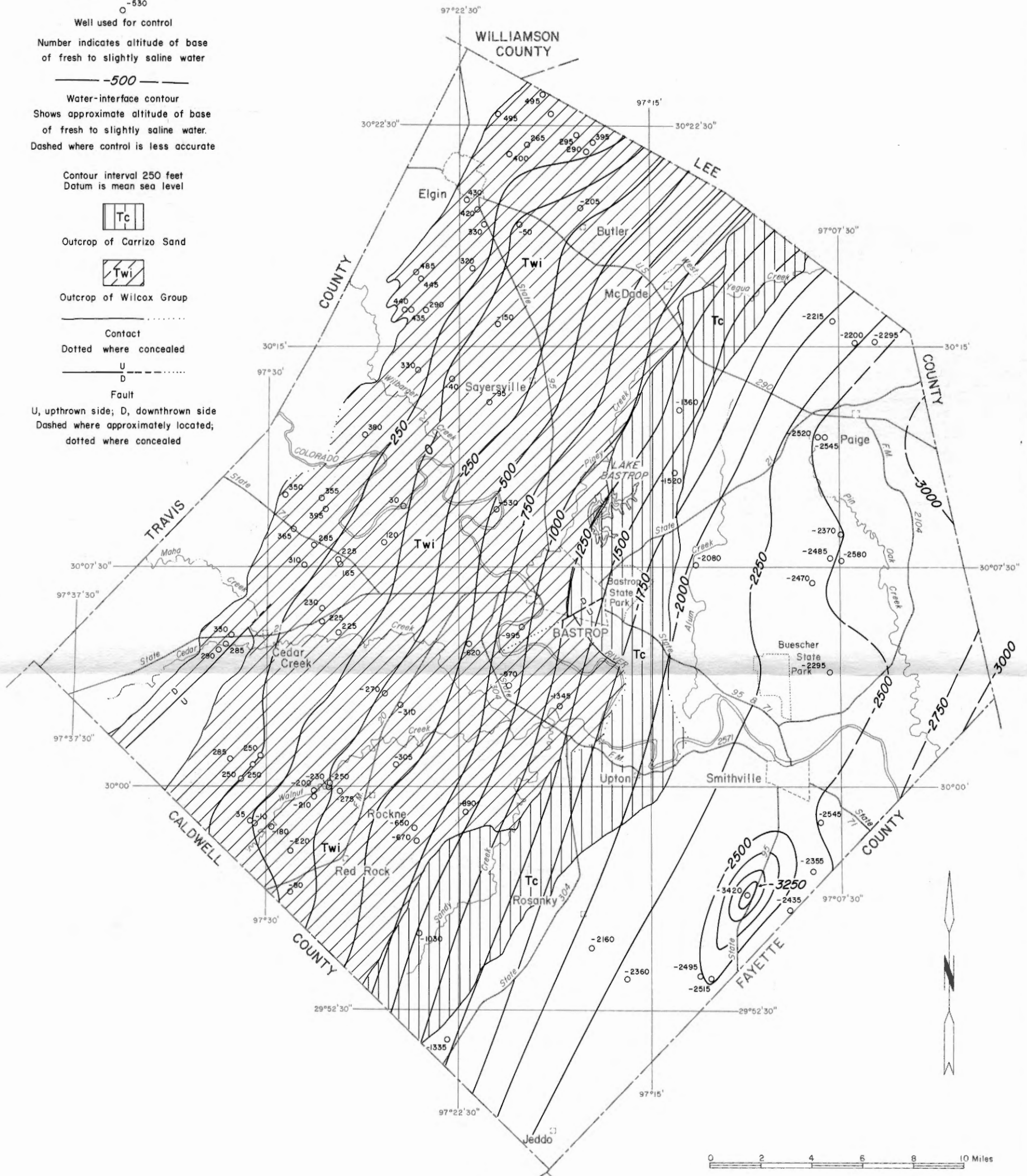
Figure 19 APPROXIMATE ALTITUDE OF THE BASE OF FRESH TO SLIGHTLY SALINE WATER IN THE CARRIZO SAND AND WILCOX GROUP
