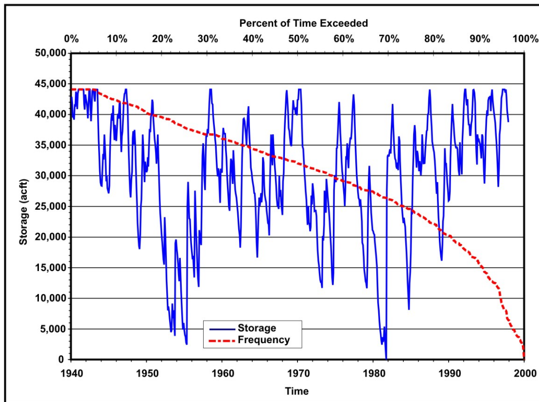
Figure 3.4.16-6. Simulated System Storage for Lake Palo Pinto and Wilson Hollow Reservoirs (System Diversion = 14,216 acft/yr)
