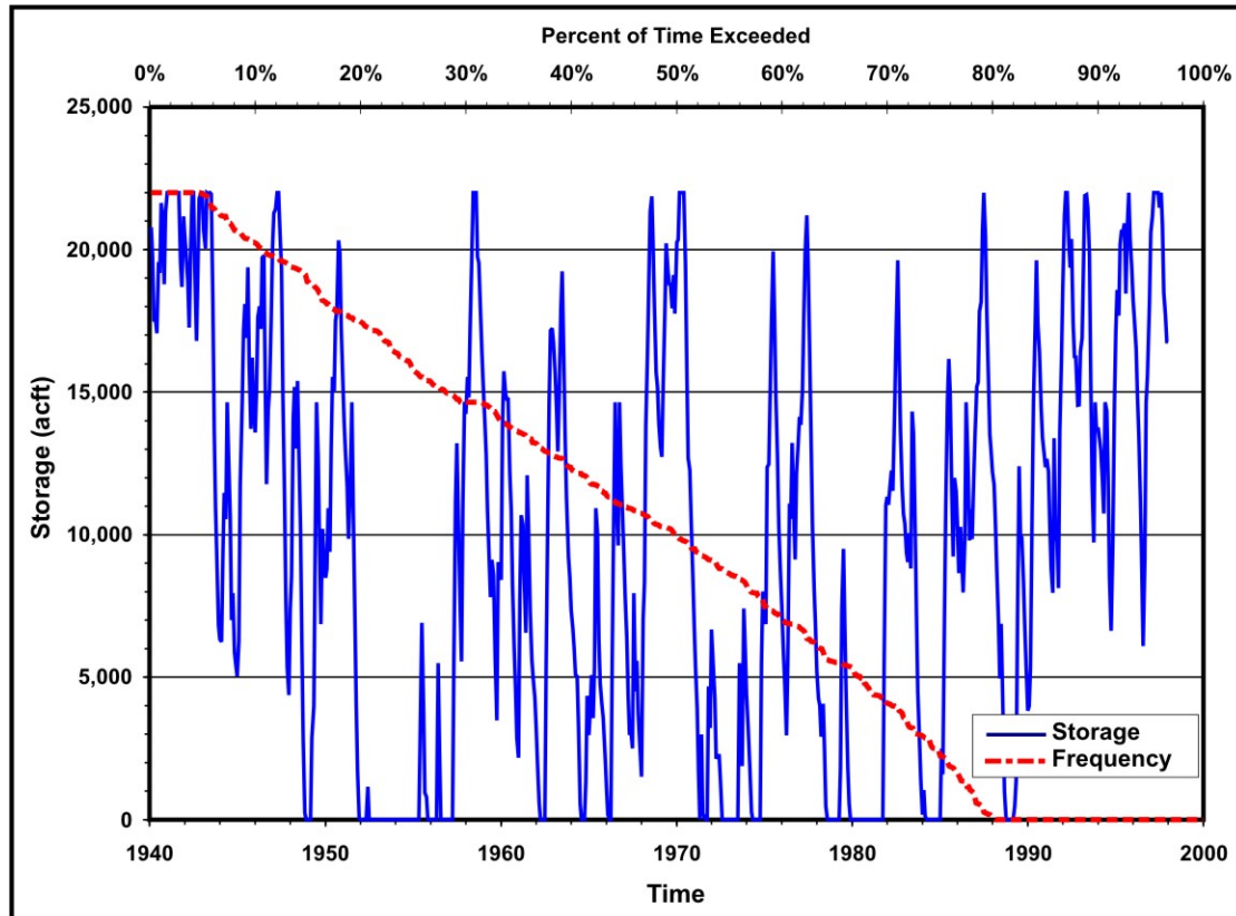
Figure 3.4.16-5. Simulated Storage in Wilson Hollow Reservoir (Conservation Elevation = 1077 ft-msl, Incremental Diversion = 7,556 acft/yr)
