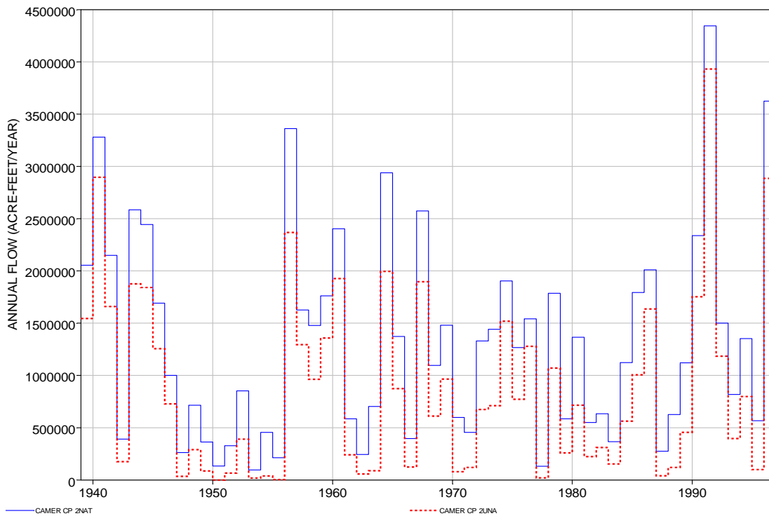
Figure 3.4 Naturalized and Unappropriated Annual Flows at CAMER Control Point Plotted with HEC-DSSVue from DSS File Created with TABLES
