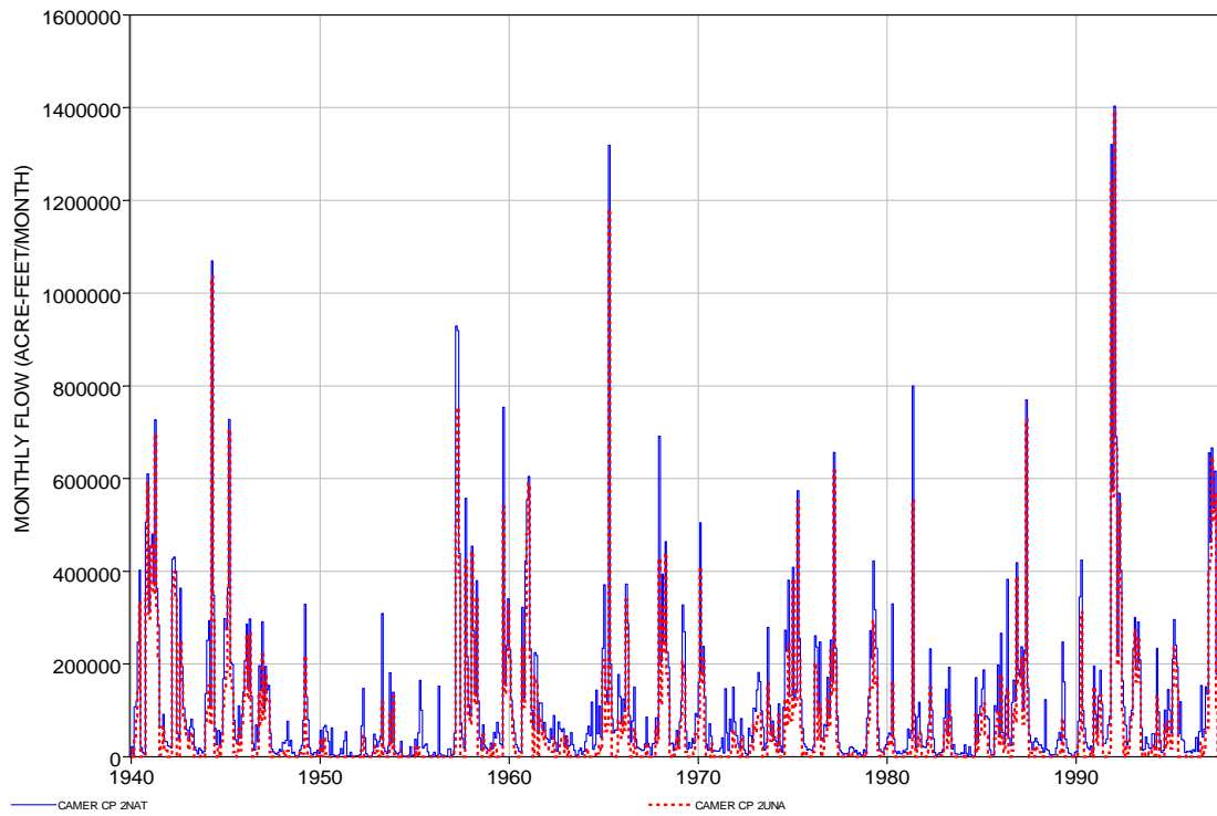
Figure 3.3 Naturalized and Unappropriated Monthly Flows at CAMER Control Point
