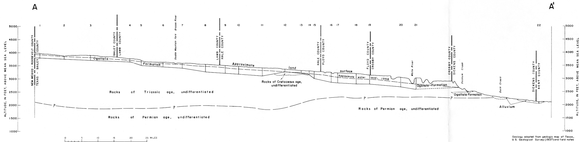
Figure 6 Section A-A', Region I, Brazos River Basin U.S. Geological Survey in cooperation with the Texas Water Commission
