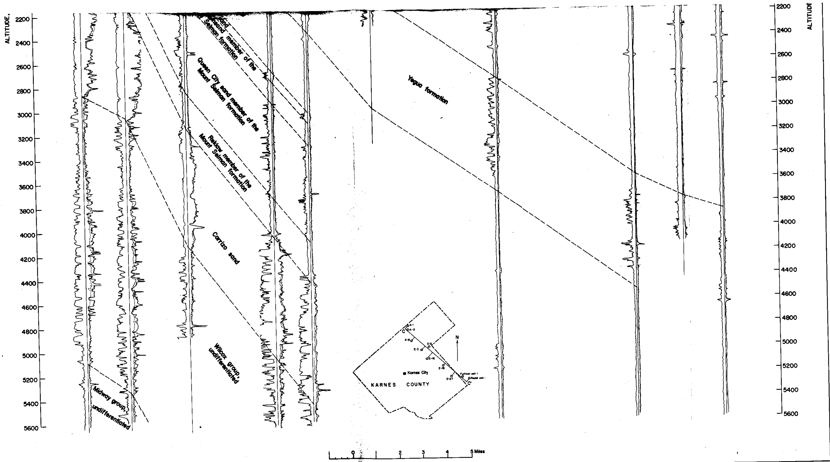
GEOLOGIC SECTION C-C'
