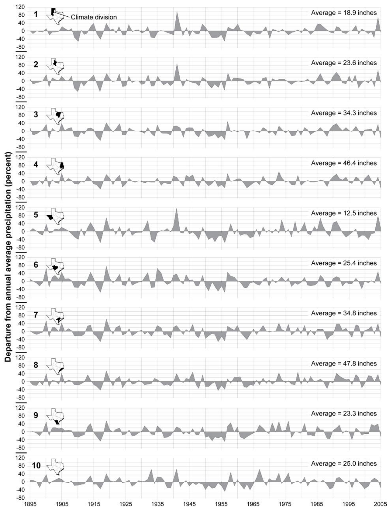
Figure 5.6. Historical plots of percent departure from average annual precipitation for each climate division of Texas for 1895 to 2005 (data from NCDC, 2006).
