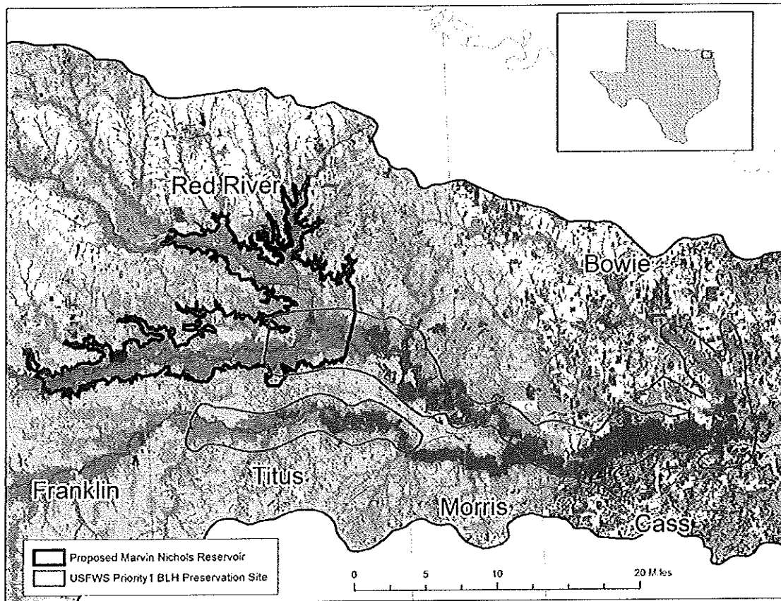
Figure 1 Location of proposed Marvin Nichols Reservoir in relation to USFWS designated Priority Bottomland Hardwood Preservations Site.
