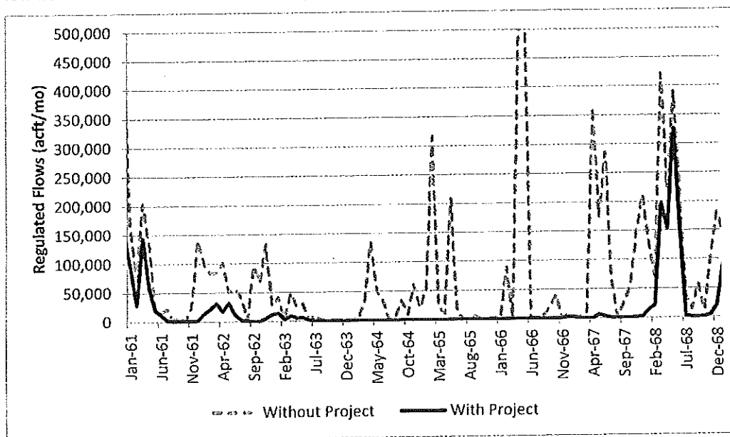
Figure 4 Regulated flows with and without the Marvin Nichols I Reservoir Project (1961-1968)
