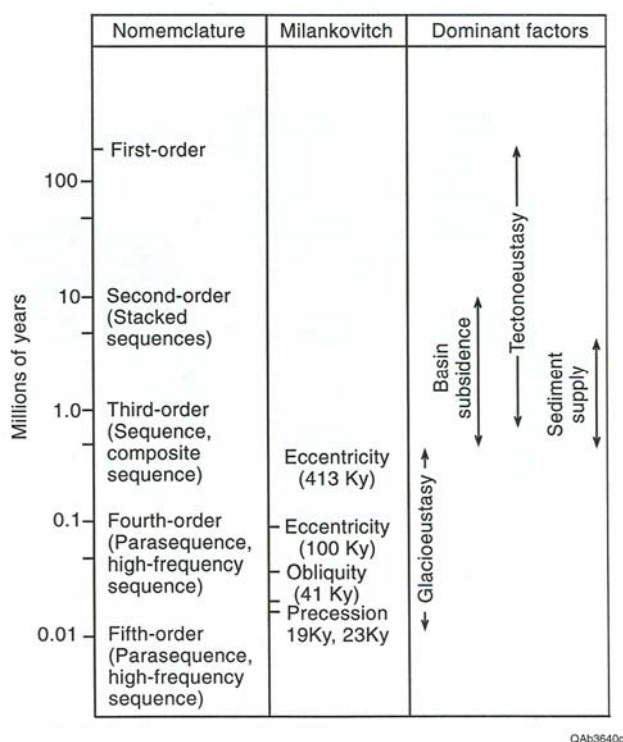
Figure 4-8. Hierarchical cycle nomenclature and dominant factors at each scale. Modified from Fisher (1964), Hays and others (1976), Meckel and Galloway (1996), and Mitchum and Van Wagoner (1991). (Ky = 1,000 years)
