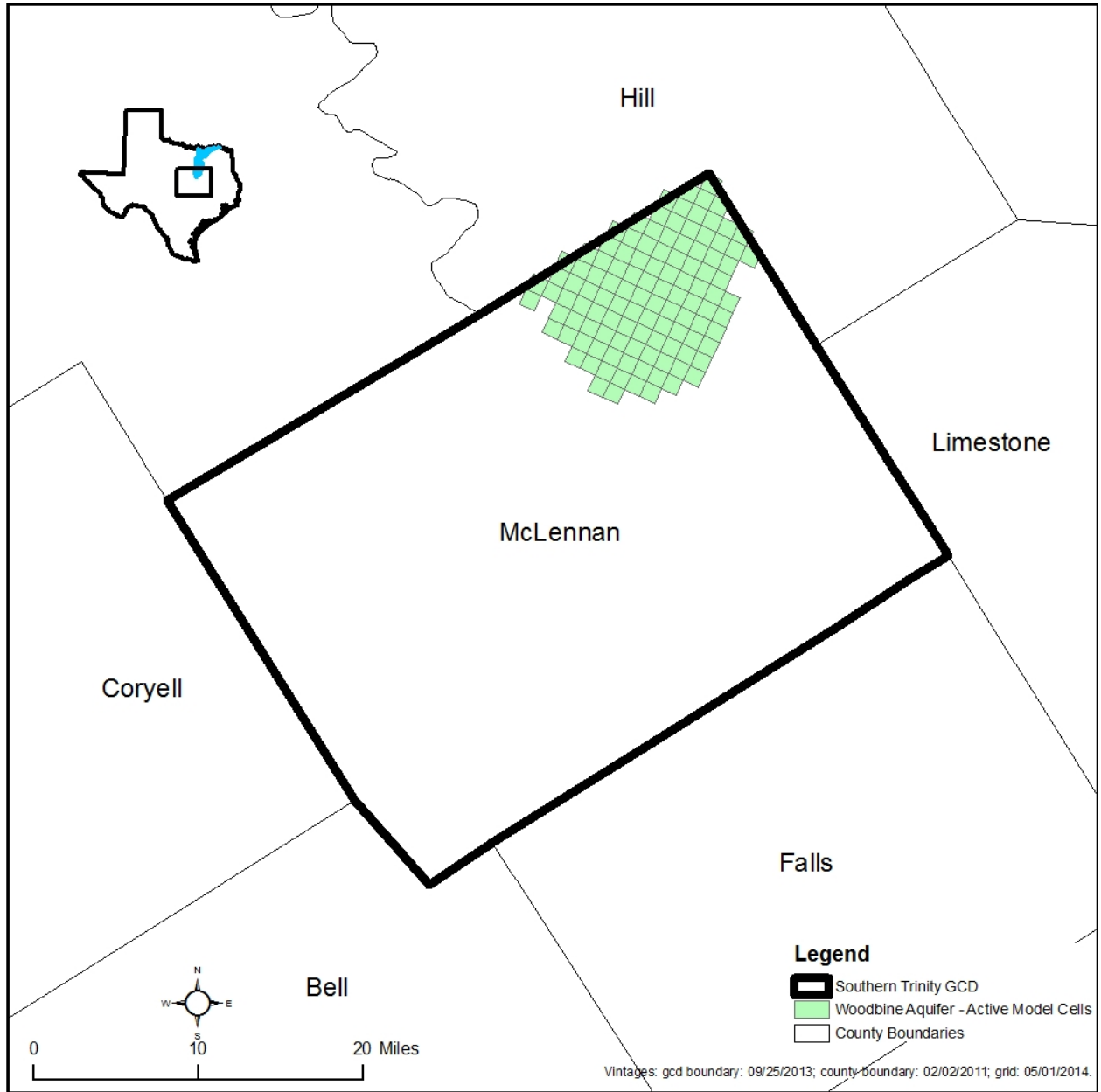
FIGURE 1: AREA OF THE GROUNDWATER AVAILABILITY MODEL FOR THE WOODBINE AQUIFER FROM WHICH THE INFORMATION IN TABLE 1 WAS EXTRACTED (THE WOODBINE AQUIFER FOOTPRINT EXTENT WITHIN THE DISTRICT BOUNDARY).
