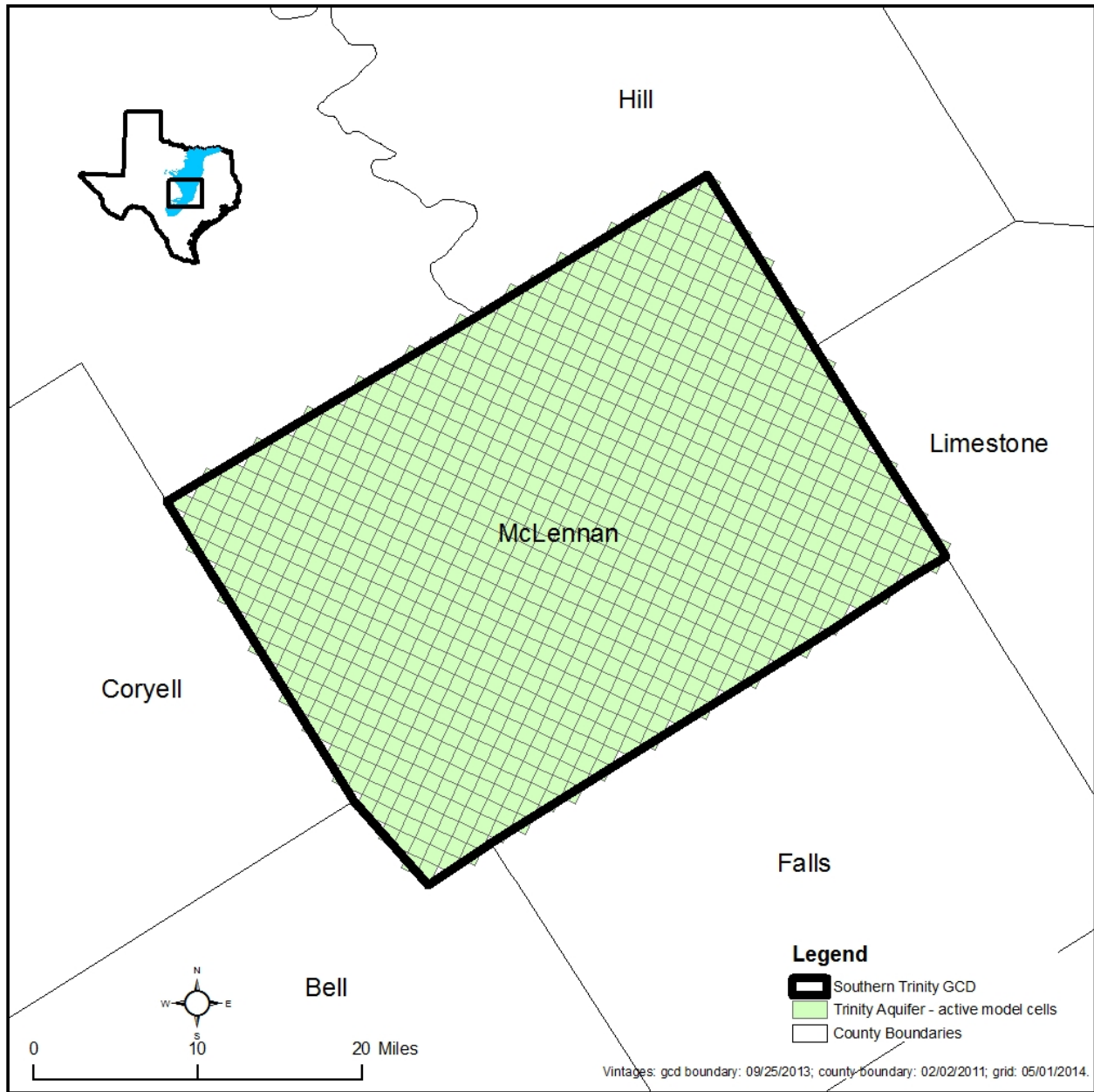
FIGURE 2: AREA OF THE GROUNDWATER AVAILABILITY MODEL FOR THE TRINITY AQUIFER FROM WHICH THE INFORMATION IN TABLE 2 WAS EXTRACTED (THE TRINITY AQUIFER FOOTPRINT EXTENT WITHIN THE DISTRICT BOUNDARY).
