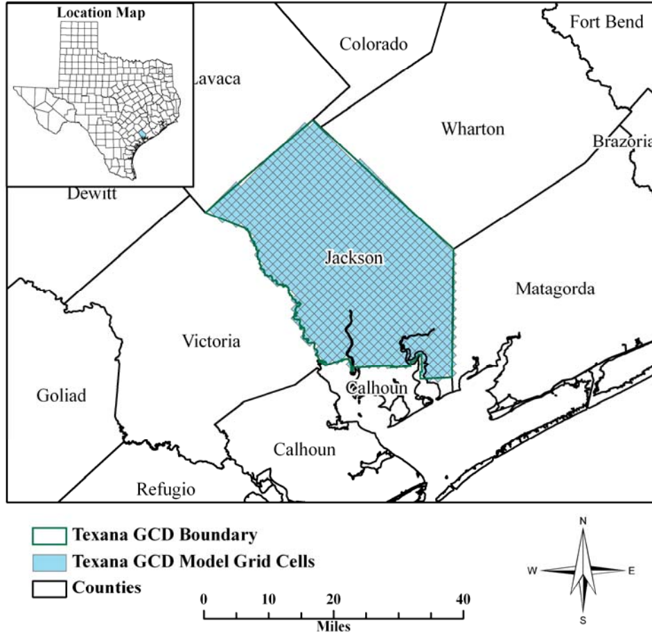
Figure 1: Area of the groundwater availability model for the central portion of the Gulf Coast Aquifer from which the information in Table 1 was extracted. Note that model grid cells that straddle a political boundary were assigned to one side of the boundary based on the centroid of the model cell as described above.
