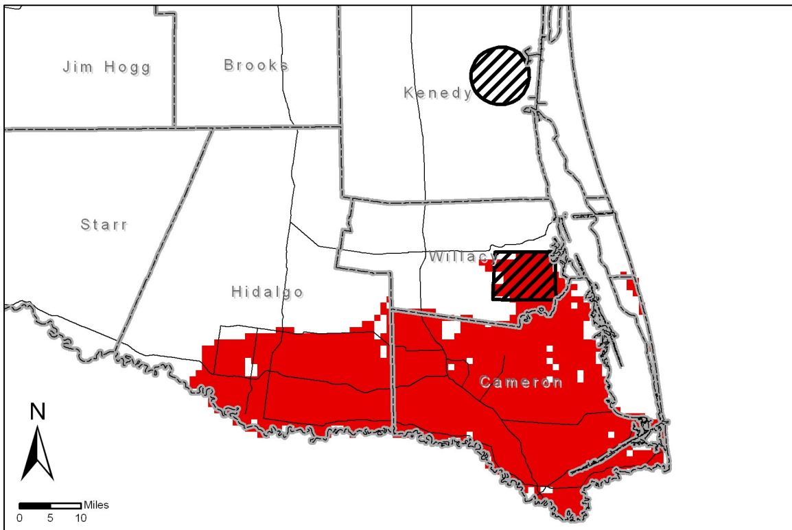
Figure 1. Specific areas in the Chicot Aquifer where additional pumpage was added in Kenedy and Willacy counties. Pumpage present in the baseline pumpage data set is shown in red. Additional pumpage in other counties was added uniformly to all active cells in each county.
