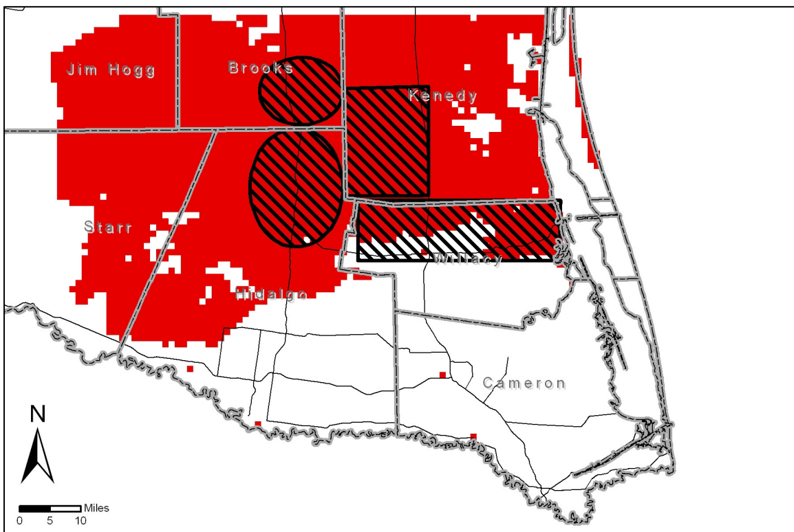
Figure 2. Specific areas in the Evangeline Aquifer where additional pumpage was added in Brooks, Hidalgo, Kenedy, and Willacy counties. Pumpage present in the baseline pumpage data set is shown in red. Additional pumpage in other counties was added uniformly to all active cells in each county.
