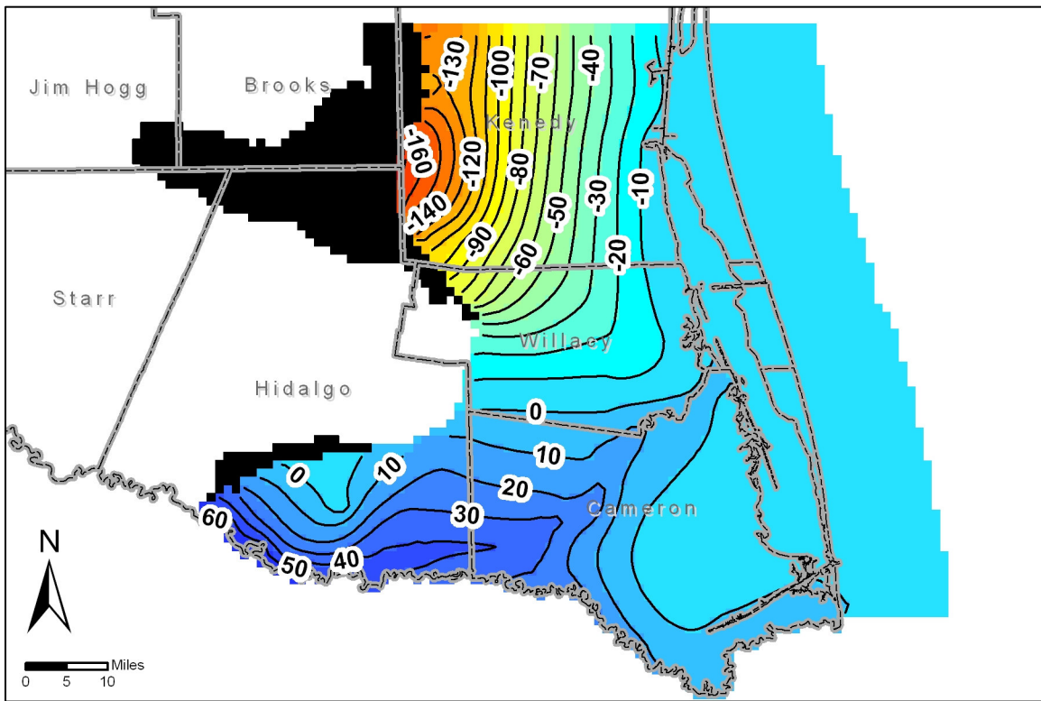
Figure 5. Water level elevations after 60 years using the requested pumpage in the Chicot Aquifer. Water level elevations are in feet above mean sea level. Contour interval is 10 feet. Dry cells are shown in black.
