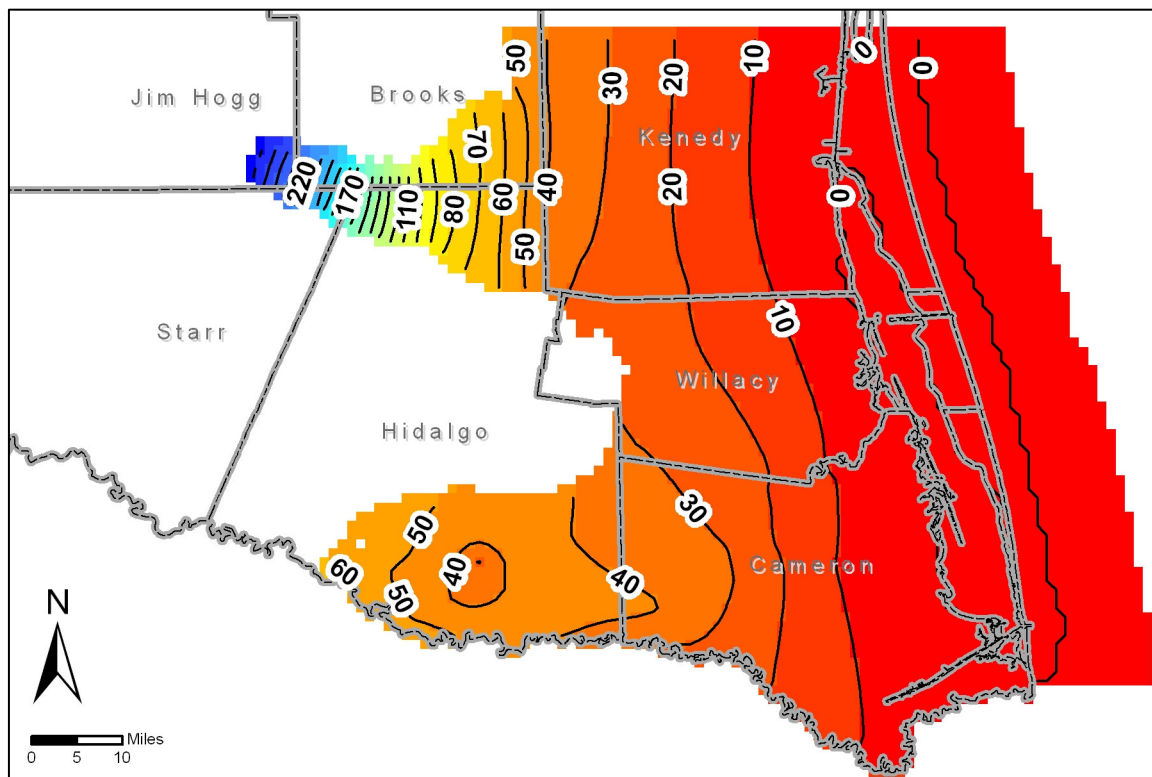
Figure 3. Initial water level elevations for the predictive model run in the Chicot Aquifer from the southern part of the Gulf Coast groundwater availability model. Water level elevations are in feet above mean sea level. Contour interval is 10 feet.
