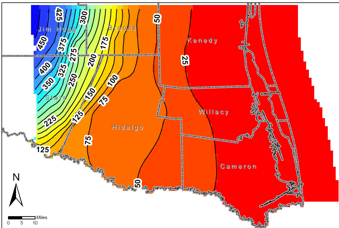
Figure 4. Initial water level elevations for the predictive model run in the Evangeline Aquifer from the southern part of the Gulf Coast groundwater availability model. Water level elevations are in feet above mean sea level. Contour interval is 25 feet.
