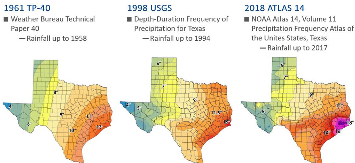
Figure 12: Evolution of Texas rainfall (24-hour, 100-year precipitation)
