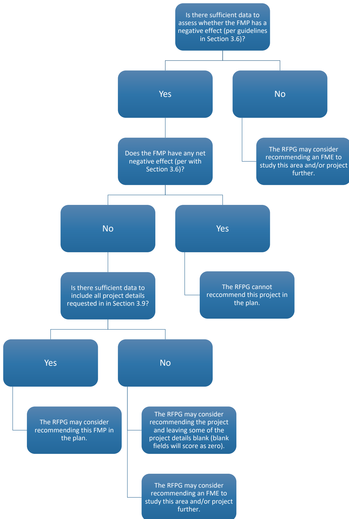
Figure 4. FMP flowchart
