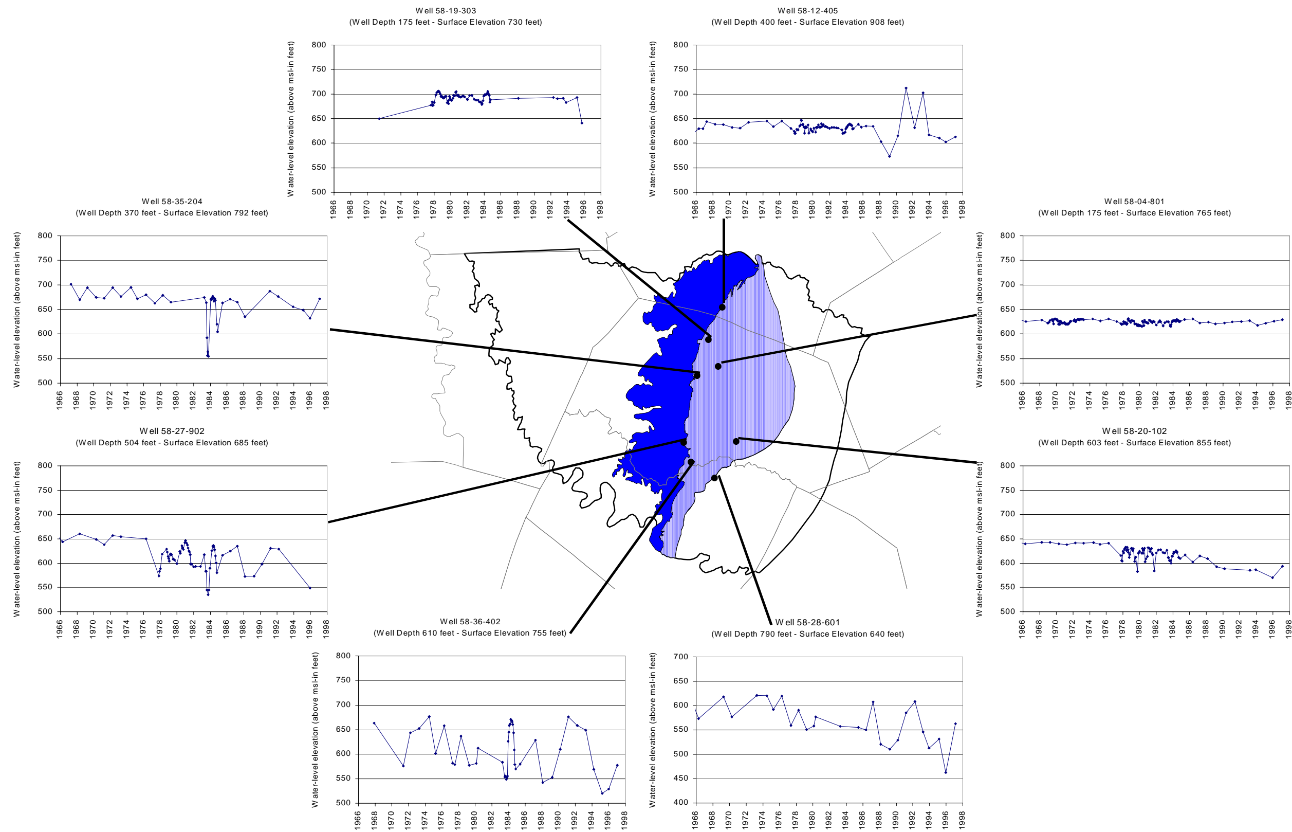
Figure 3. Water-level hydrographs for selected wells completed in the Edwards aquifer. Note: The eastern boundary of the Edwards aquifer is portrayed using TDS levels >3,000 mg/l.
