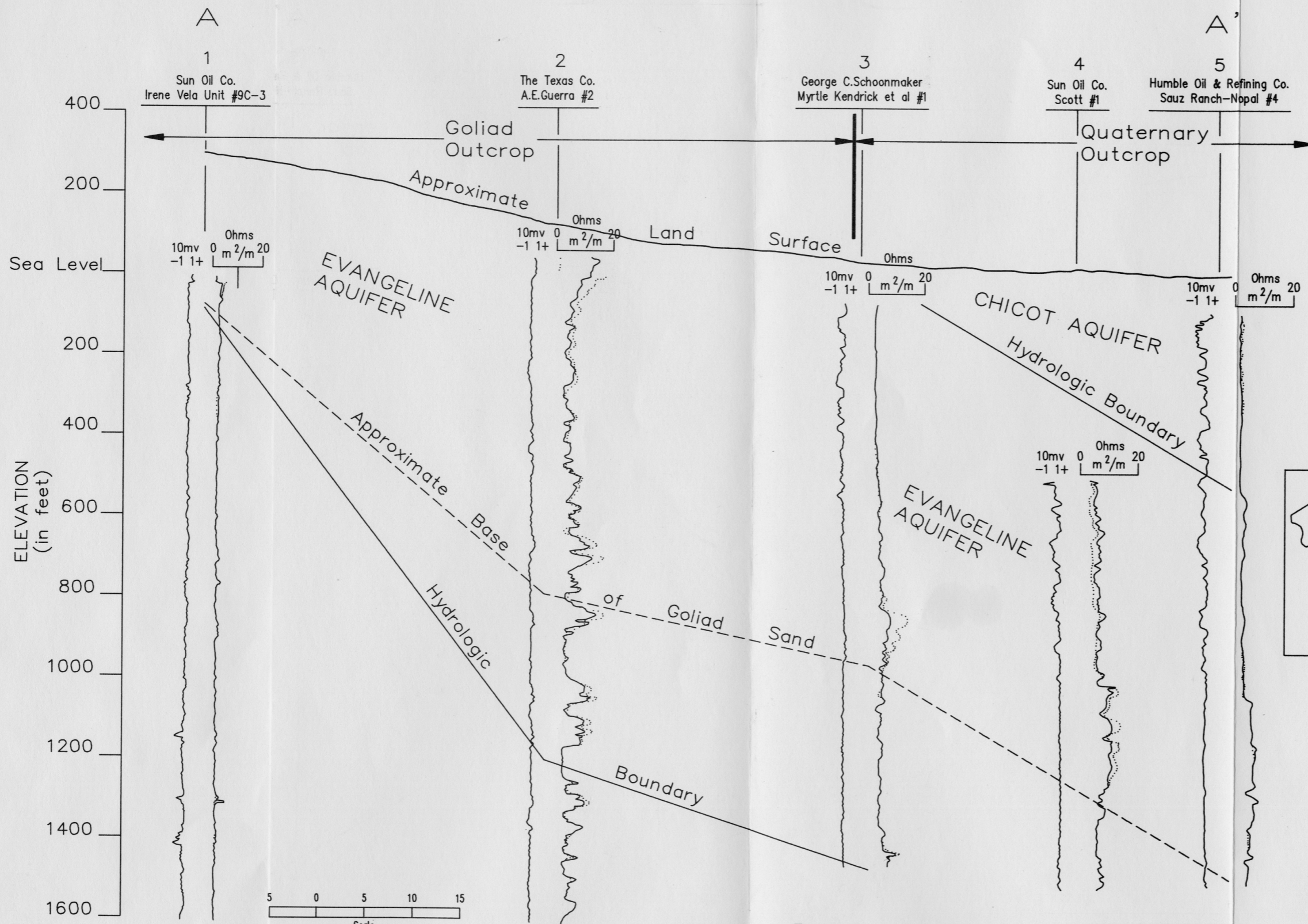
Figure 6 STRATIGRAPHIC CROSS-SECTION A-A' LOWER RIO GRANDE VALLEY
