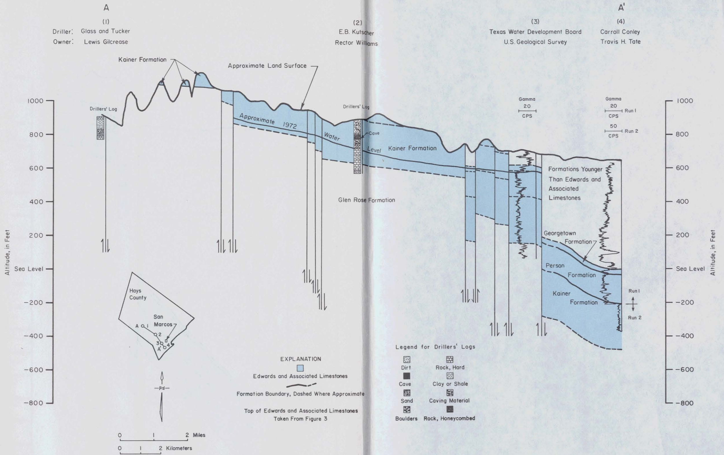
Figure 5 Geohydrologic Section A-A'
