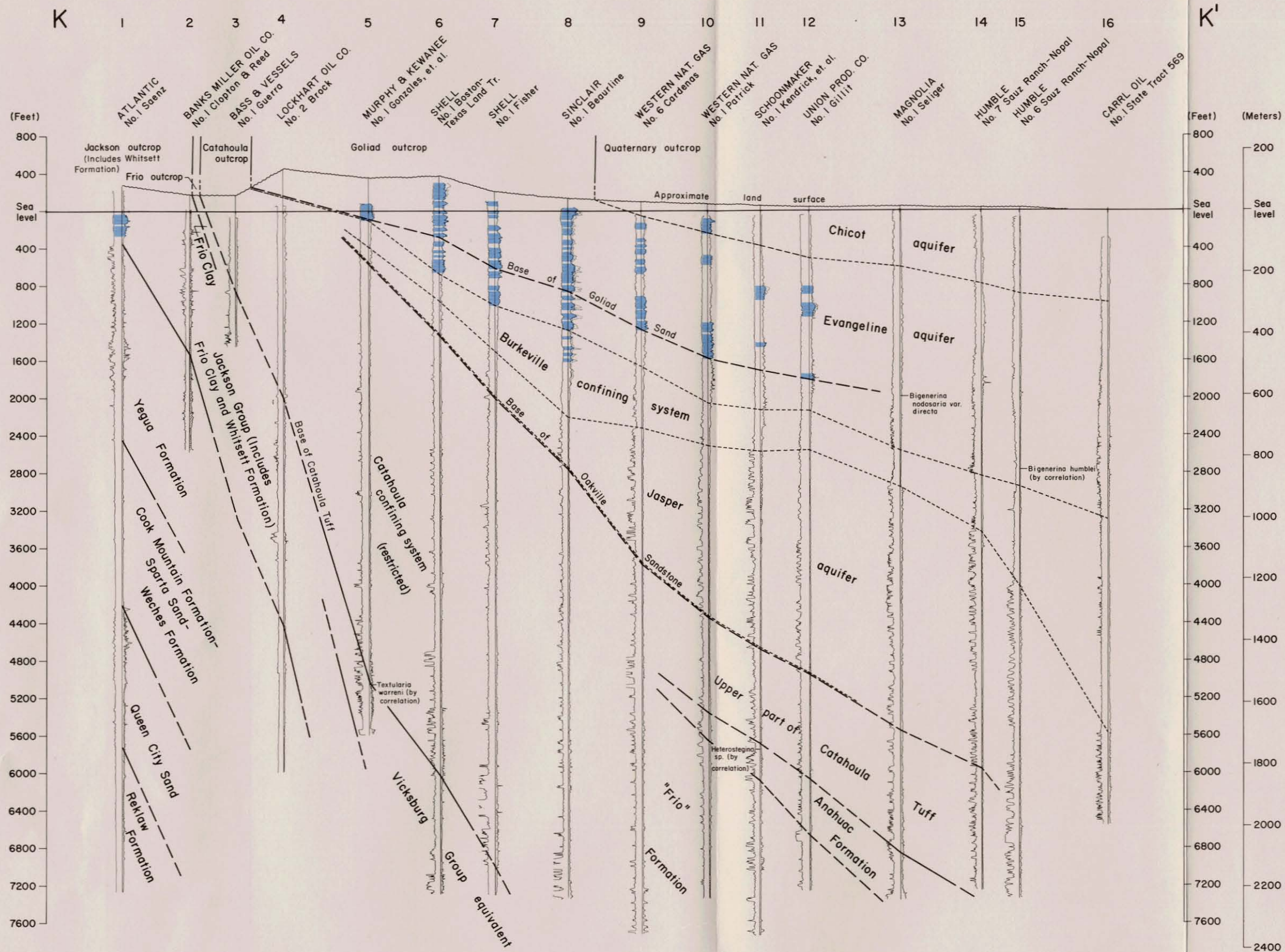
Figure 12 Stratigraphic and Hydrogeologic Section K-K'
