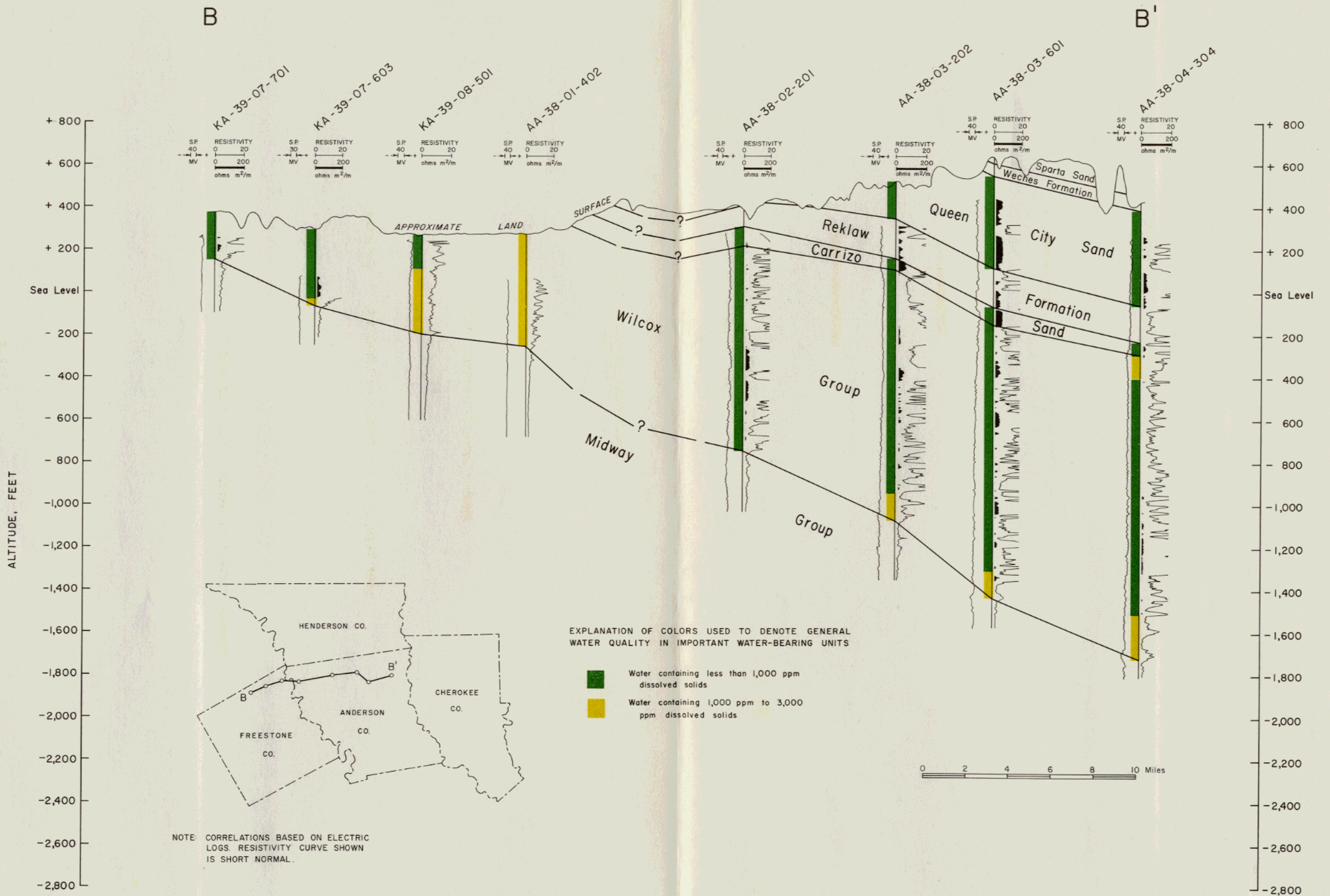
Figure 31 Geologic Section B-B'
