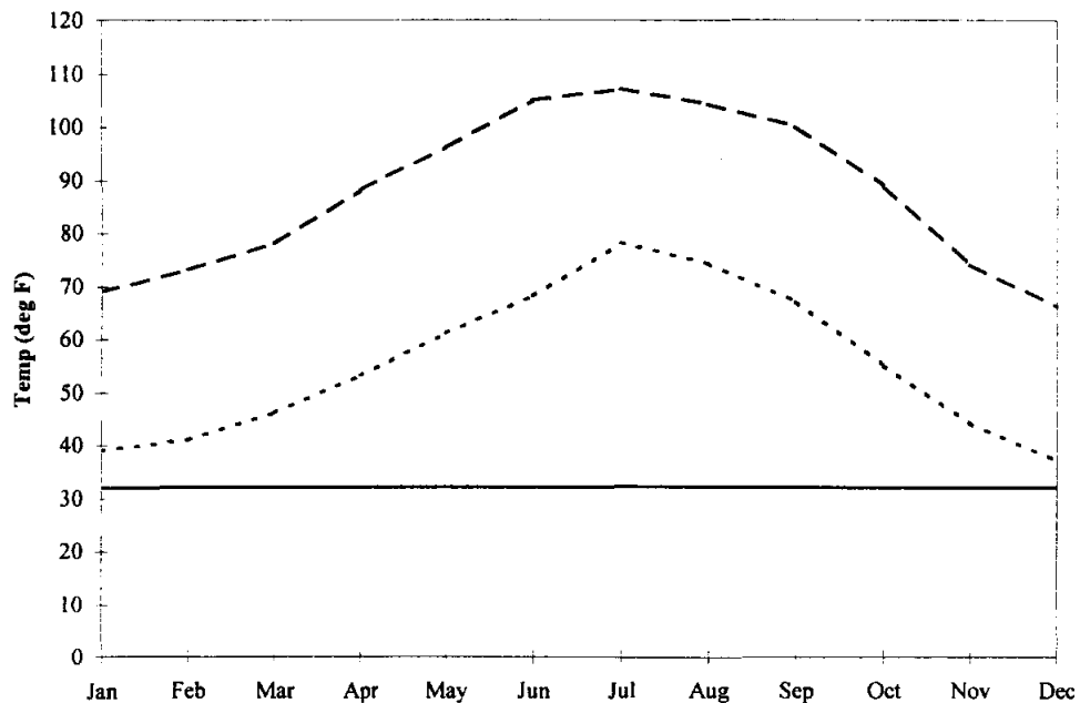
Figure 51.-Mean Monthly Minimum and Maximum Air Temperatures for Blythe, CA.
