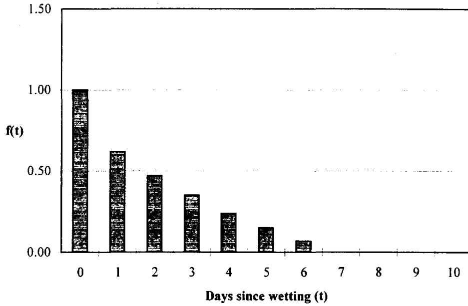
Figure 8.-Wet Soil Surface Evaporation Decay Function f(t) for Clay Loam Soil (adapted from SCS, 1993).
