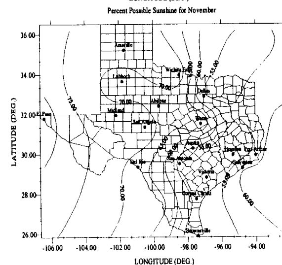
Figure B6.--Percent Possible Sunshine.
