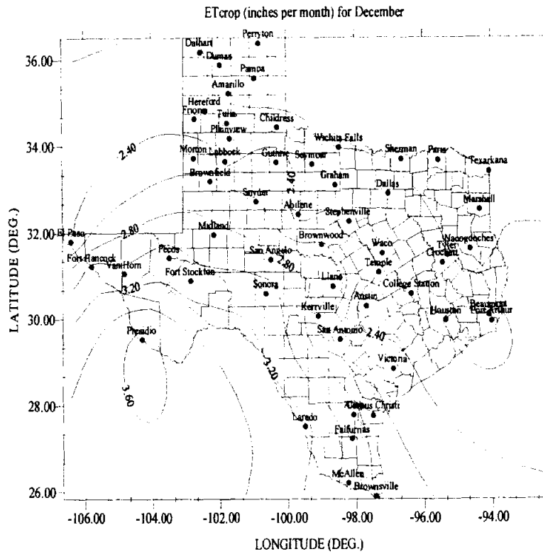
Figure 30.-ET crop for Alfalfa (inches per month).
