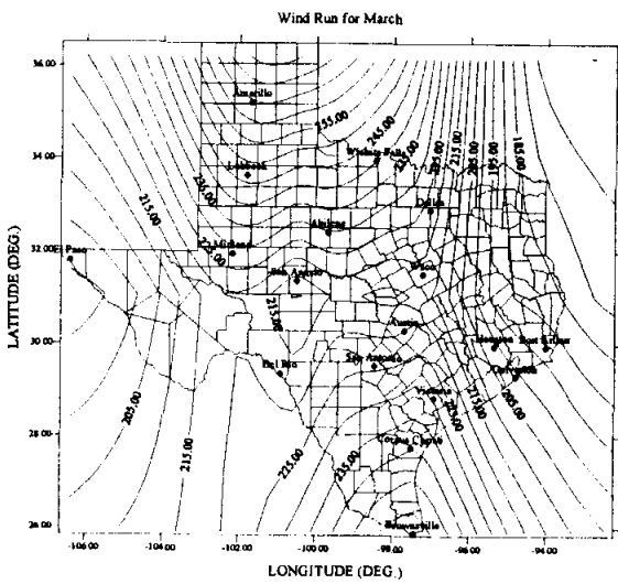
Figure B2.-Wind Run (miles per day) Adjusted to 2 m Height.
