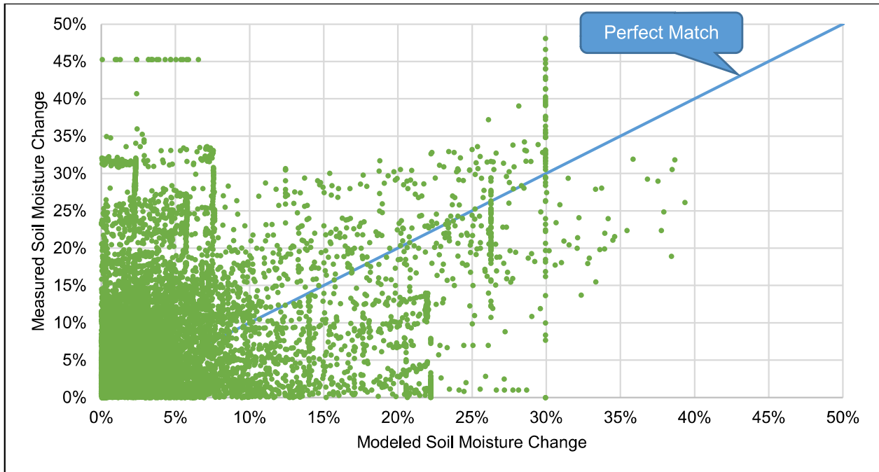
Figure 4-4: Measured versus modeled absolute value of the soil moisture change relative to the first measurement from the Soil Water Balance model.
