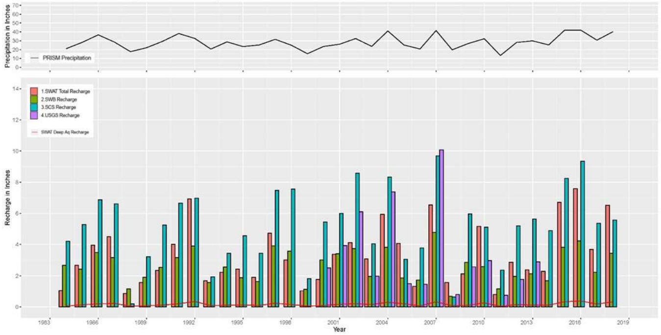
Concho Watershed – Precipitation and Recharge in Inches
