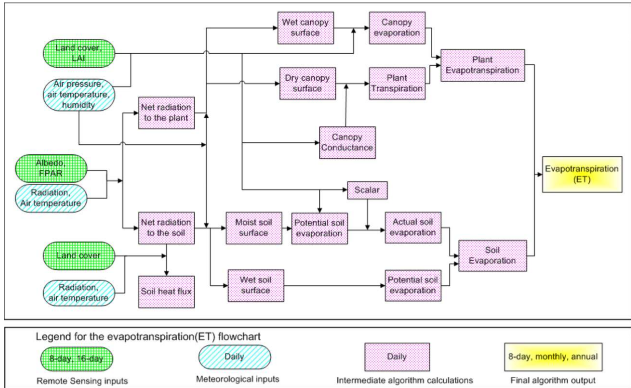
Figure 2-8: Data Sources and Steps in Moderate Resolution Imaging Spectroradiometer Evapotranspiration Calculation Algorithm (Running and others, 2019)
