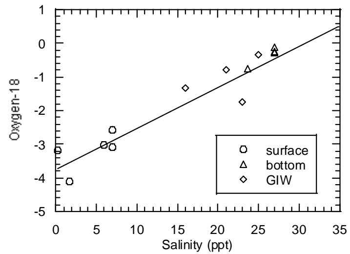
Figure 2. . 18O versus salinity plot for the samples collected on Oct. 10, 2001. The regression line was drawn for all the samples plotted.
