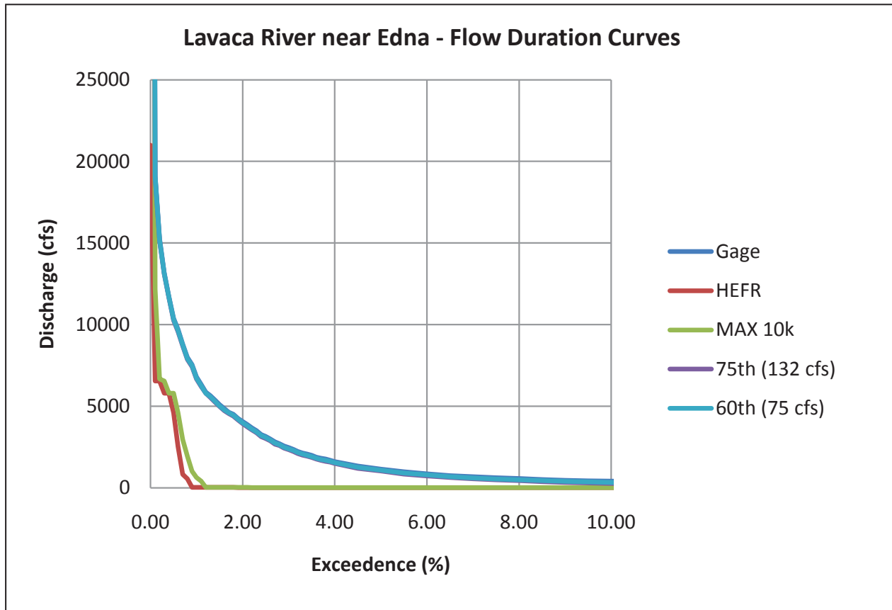
Figure 3.10.13 Flow Duration Curves for the Lavaca River near Edna
