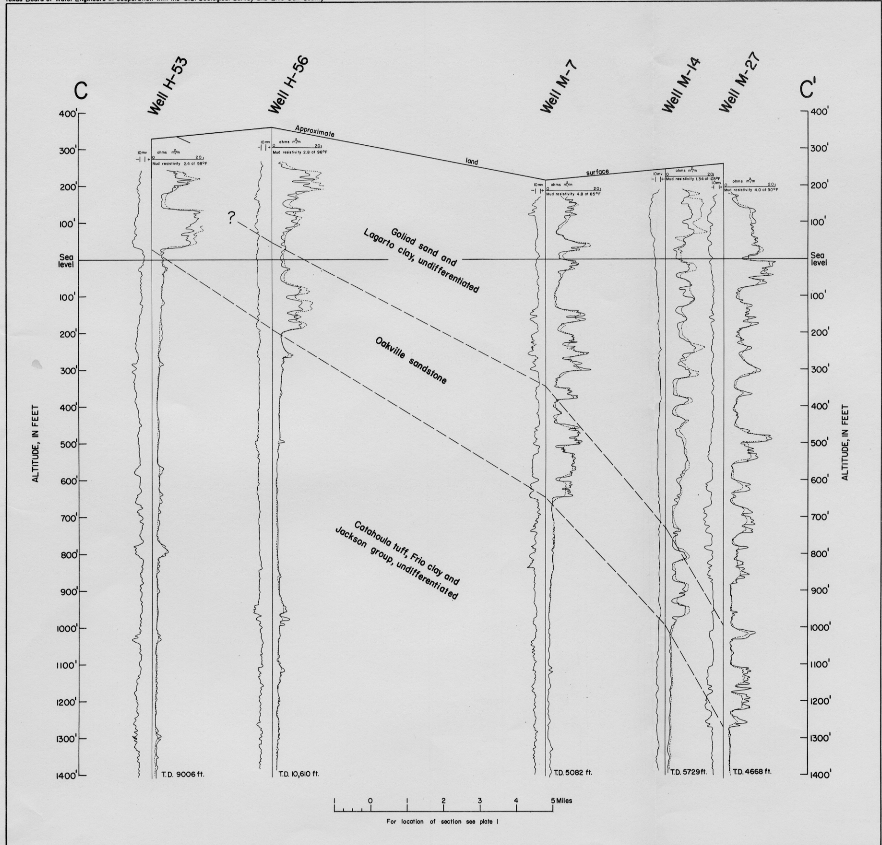
GEOLOGIC SECTION C-C', LIVE OAK COUNTY
