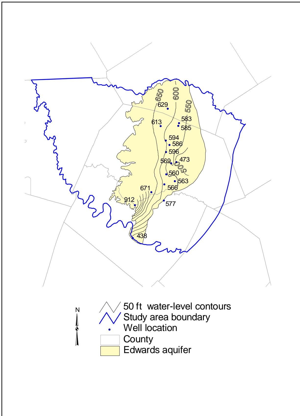
Figure 4. Potentiometric surface map for the Edwards aquifer from data collected 1997-1998.
