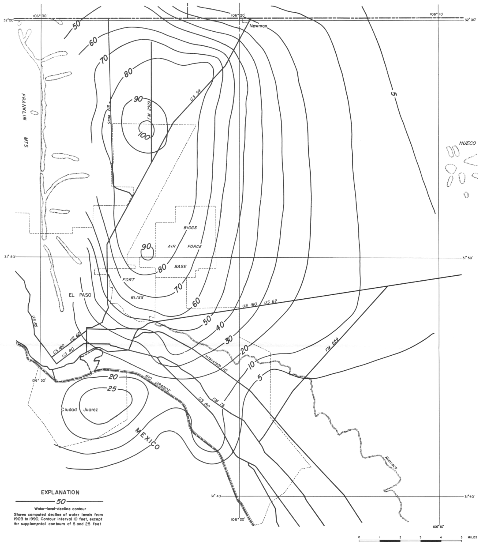
Figure 13 Predicted Decline in Water Levels Resulting from Redistribution of Pumping, 1903-90, as Computed by Electrical-Analog Model
