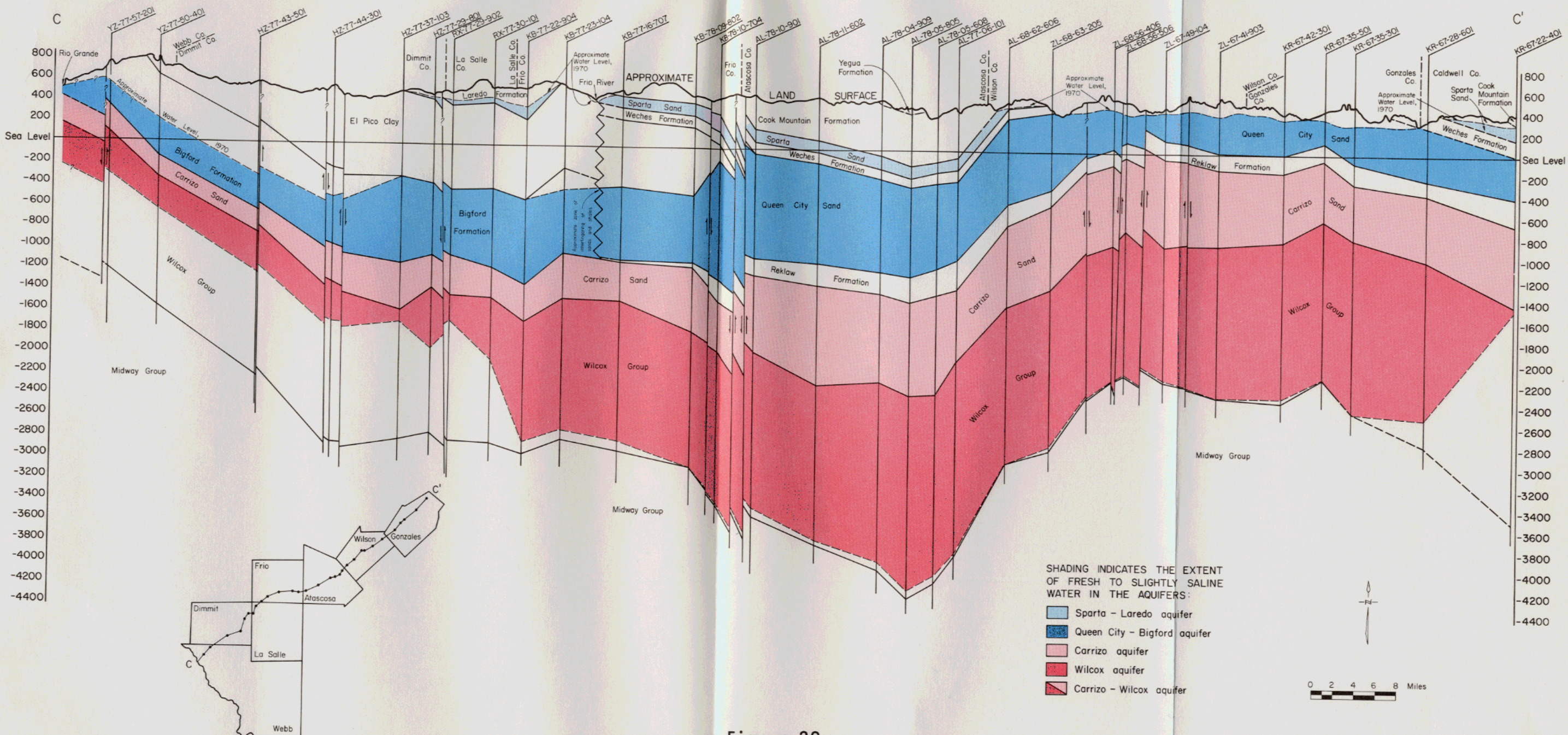
Figure 29 Geohydrologic Section C-C', Webb, Dimmit, La Salle, Frio, Atascosa, Wilson, and Gonzales Counties
