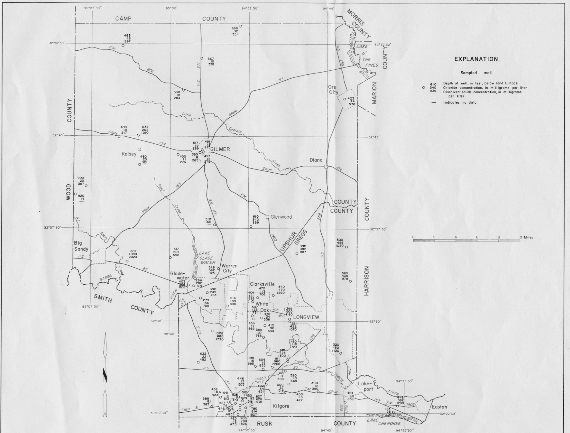
Figure 10 Chloride and Dissolved-Solids Content of Water From Selected Wells Tapping the Carrizo-Wilcox Aquifer
