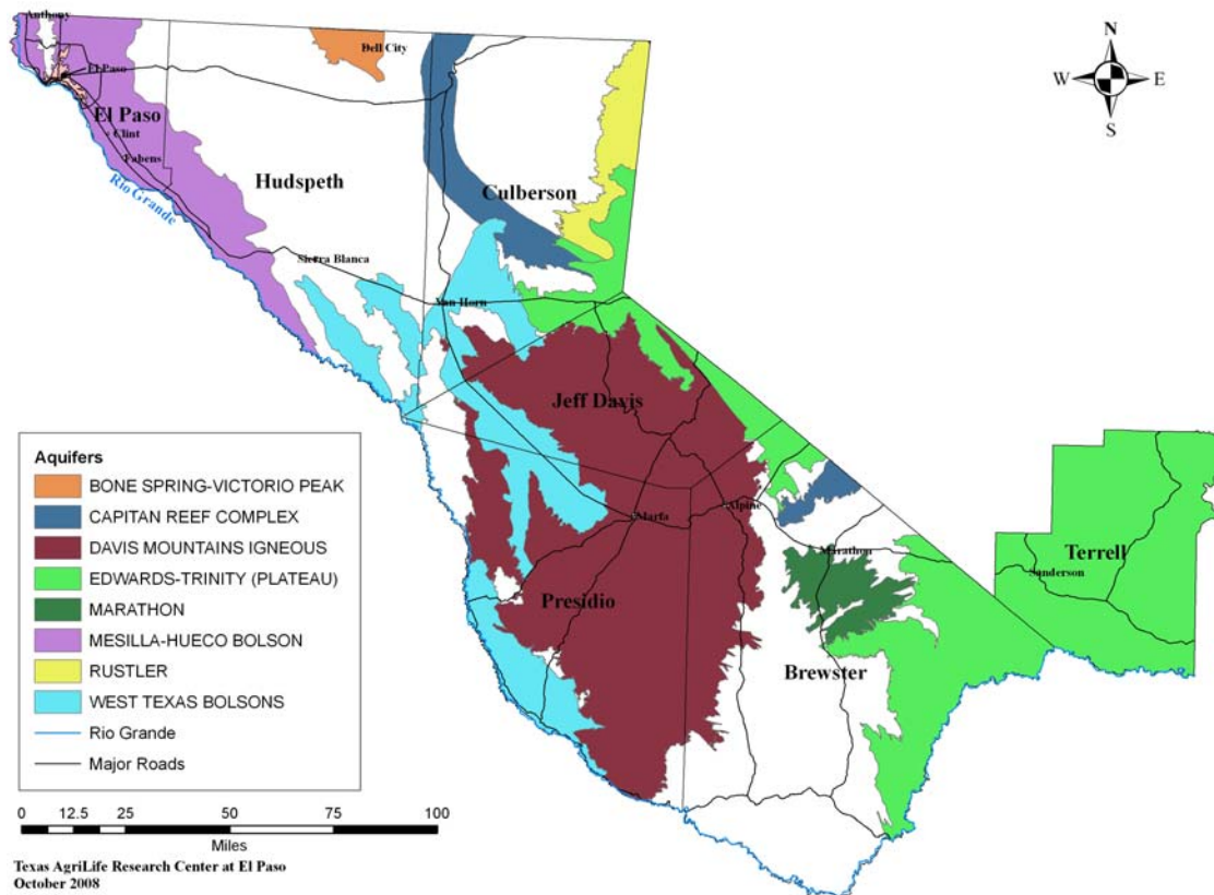
Figure 3 Major aquifers in Far West Texas Water Planning Region. Source: Figure 3-1, Far West Texas Water Plan, 2006, pp. 3-24.
