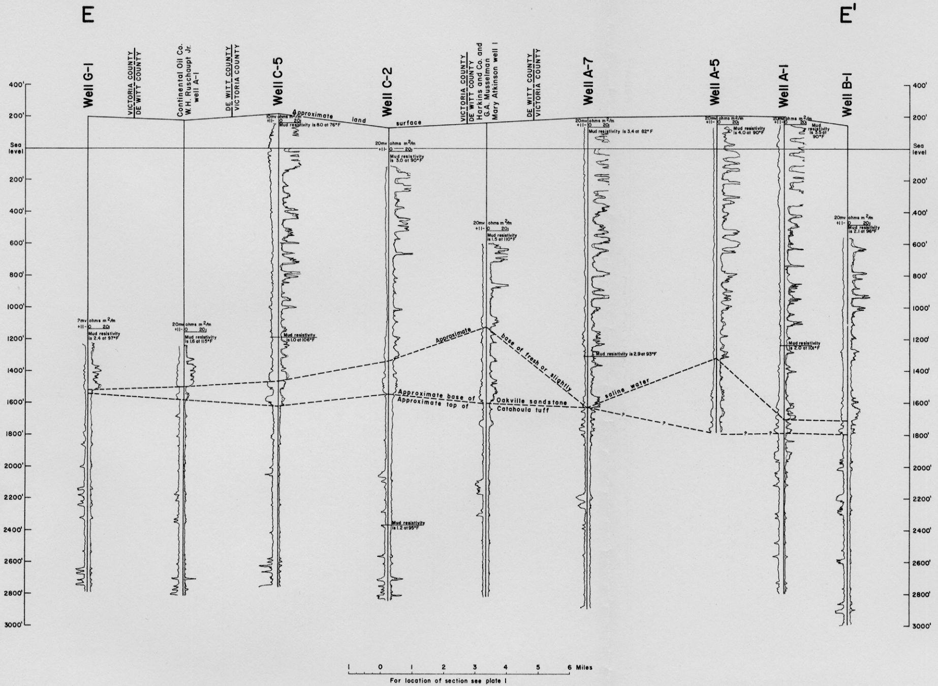
CROSS SECTION E-E', VICTORIA COUNTY, TEXAS
