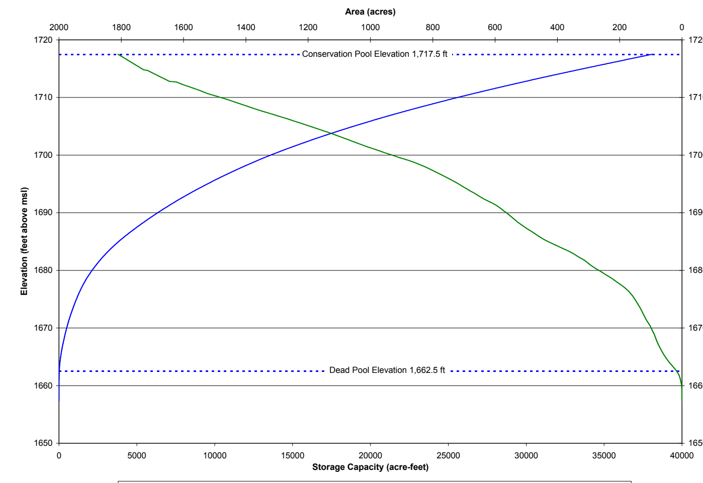
Lake Coleman July-August 2006 Survey Prepared by: TWDB Area-Capacity Curves
