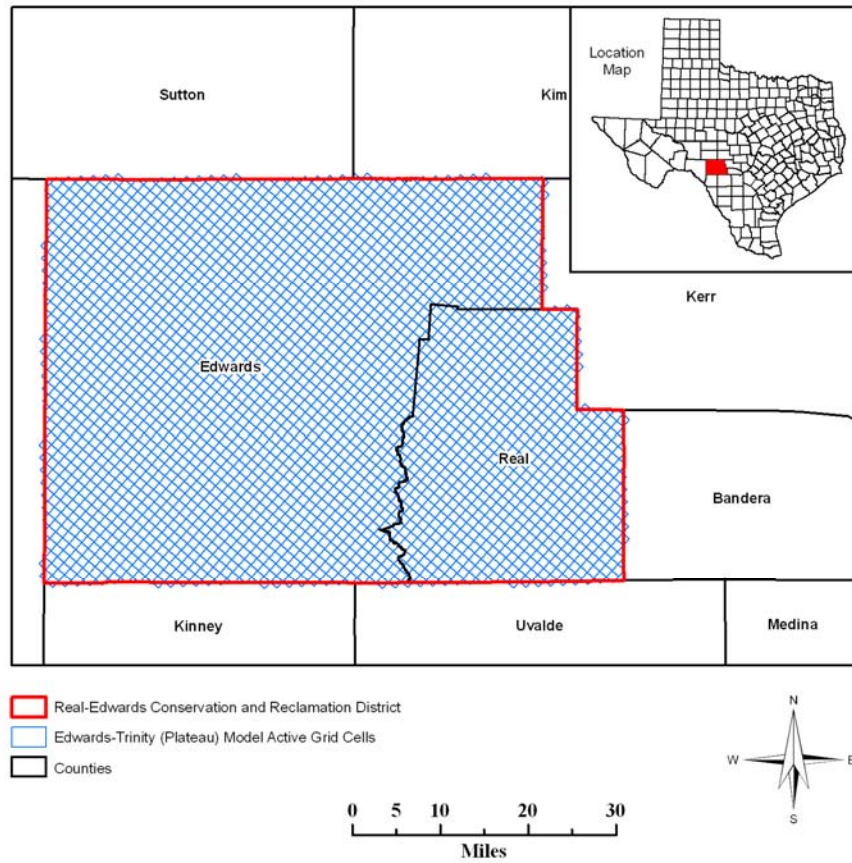
Figure 1: Area of the groundwater availability model for the Edwards-Trinity (Plateau) Aquifer from which the information in Table 1 was extracted (the aquifer extent within the Real-Edwards Conservation and Reclamation District boundary).
