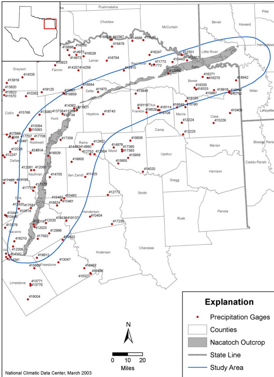
Figure 2.2.5 Location of precipitation gages
