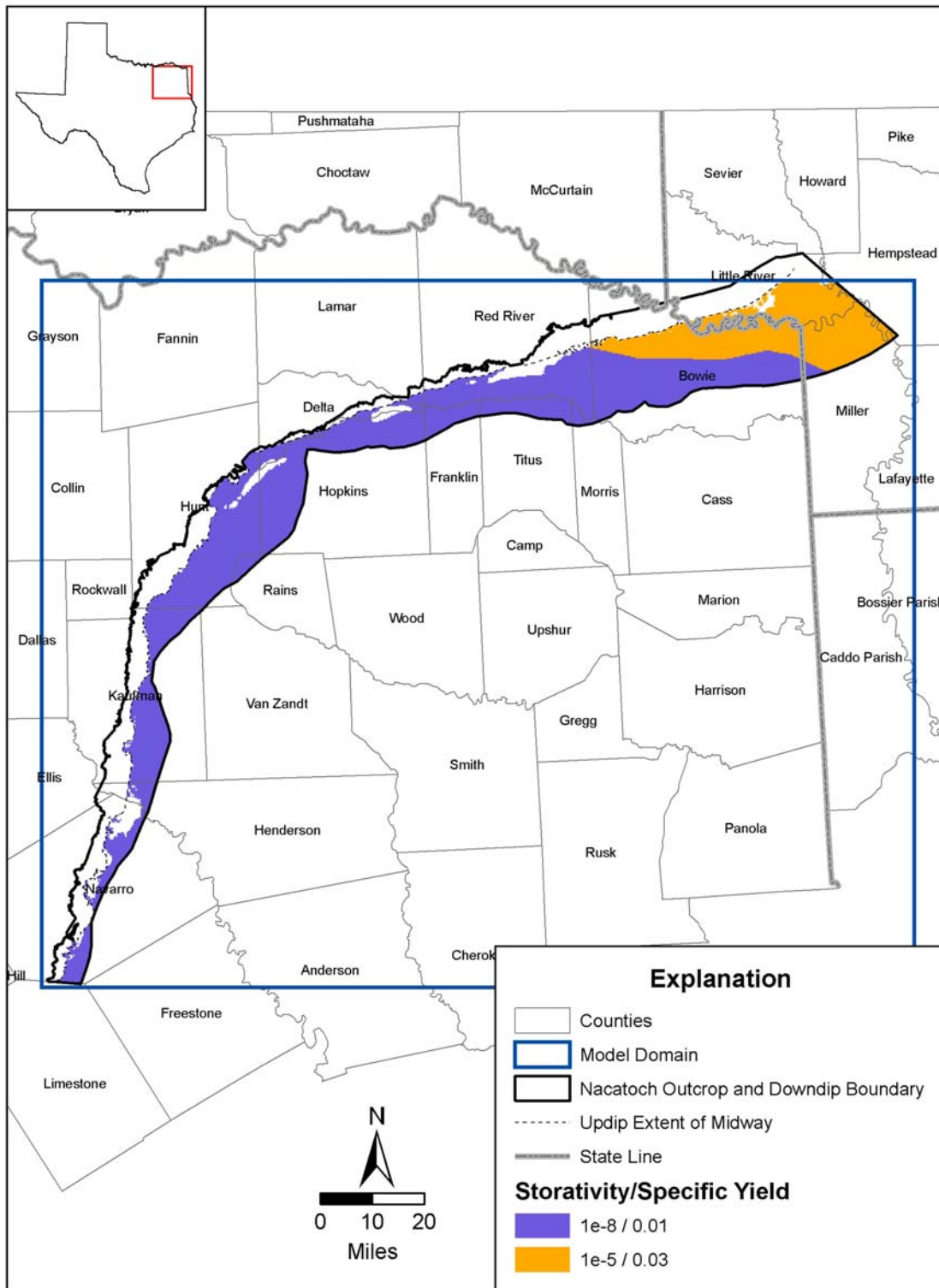
Figure 9.1.2 Final distribution of storage properties in layer 1
