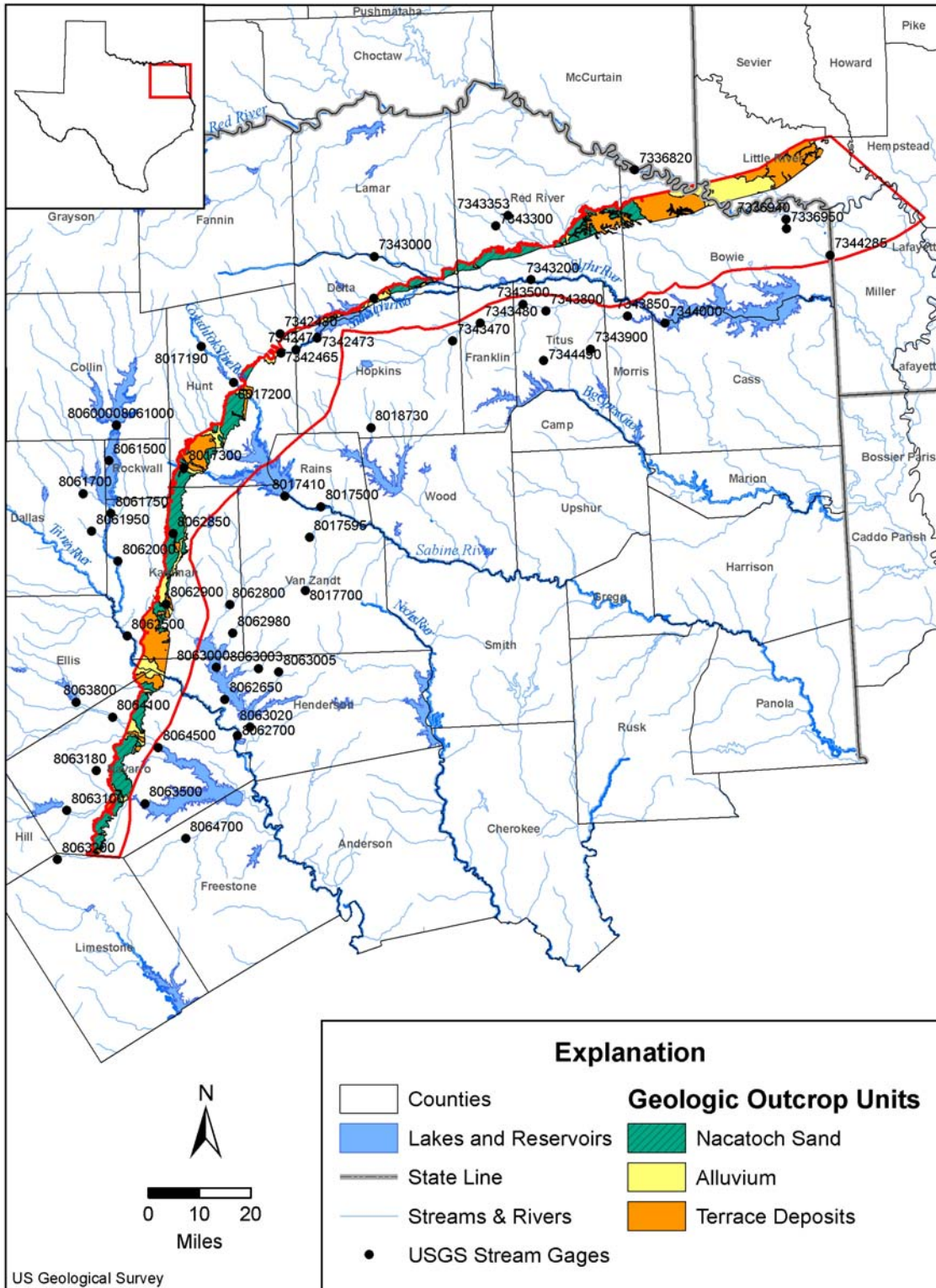
Figure 4.7.1 Stream gages in the model area
