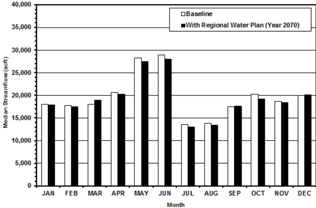
Figure 6-15 San Antonio River at Goliad
