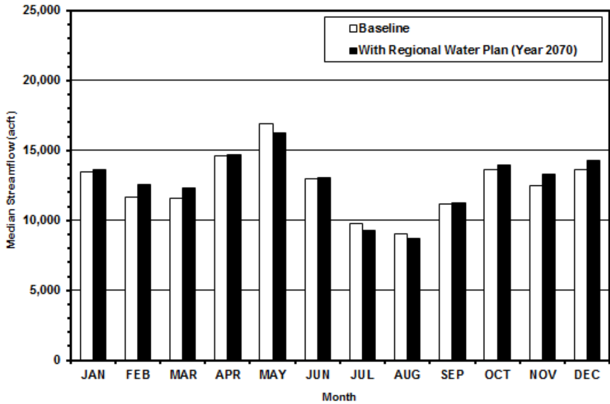
Figure 6-14 San Antonio River near Falls City
