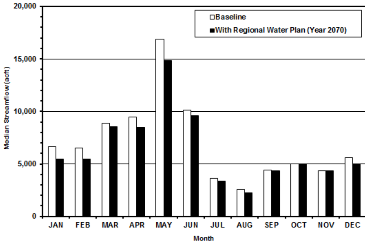
Figure 6-11 Guadalupe River above Comal River at New Braunfels
