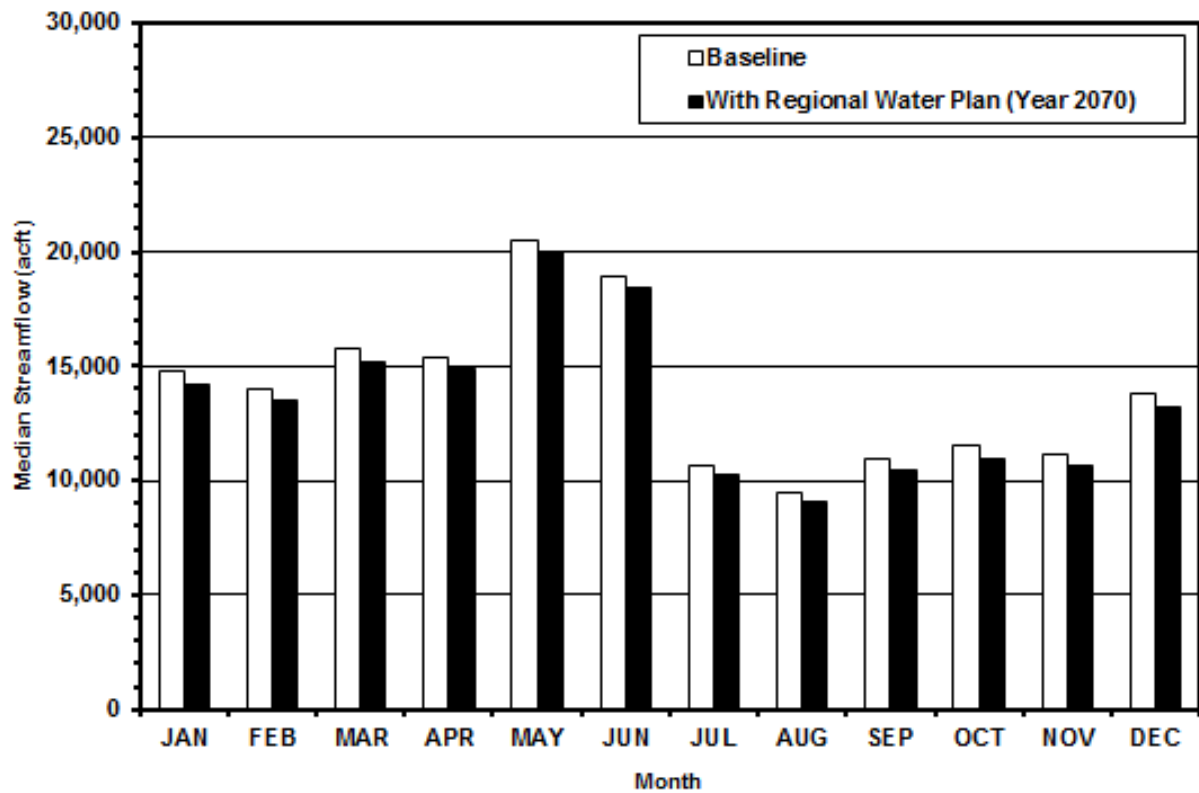
Figure 6-12 San Marcos River at Luling
