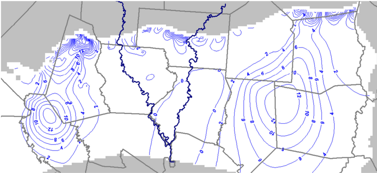
Figure 6-9 Gulf Coast Aquifer Drawdowns (2010-2060)
