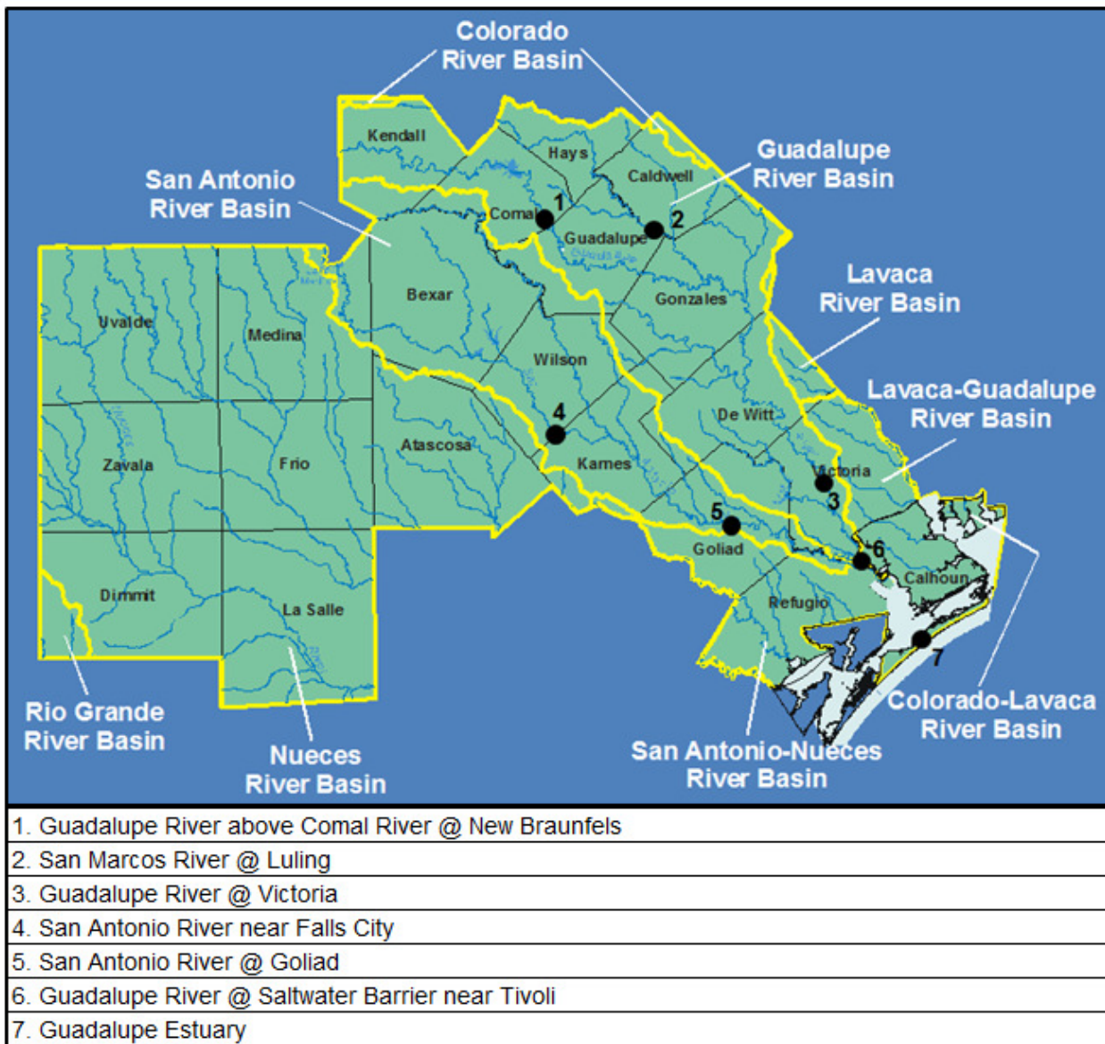
Figure 6-10 Flow Assessment Locations
