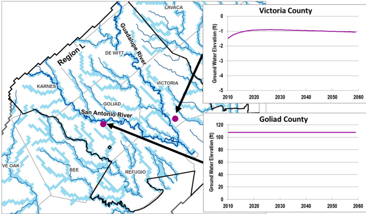
Figure 6-8 Gulf Coast Aquifer Well Hydrographs
