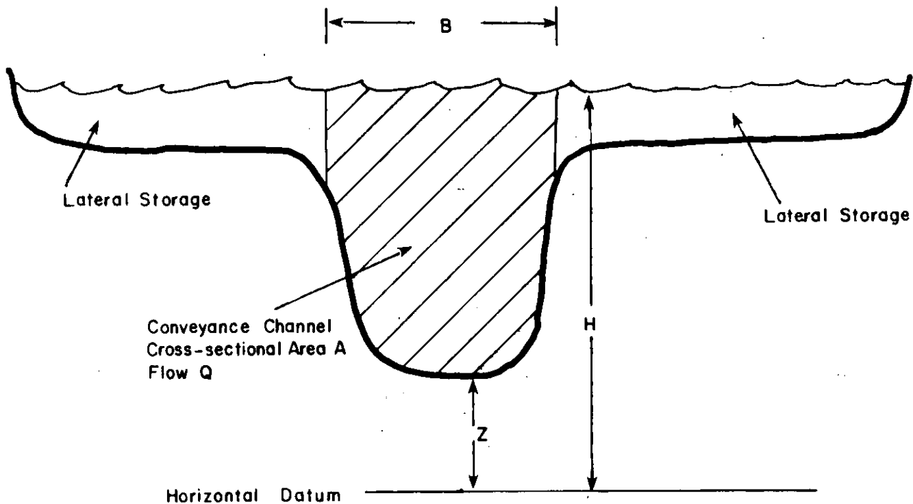
Figure 5-3. Definition of Variables in Cross Section (173)
