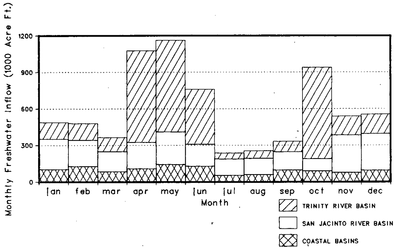
Figure 9-12. Estimated Freshwater Inflow Needs for the Trinity-San Jacinto Estuary Under Alternative II
