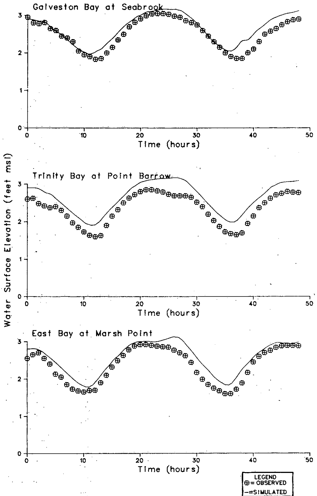
Figure 5-37. Comparison of Observed and Simulated Tidal Elevations, Trinity-San Jacinto Estuary, July 21-23, 1976
