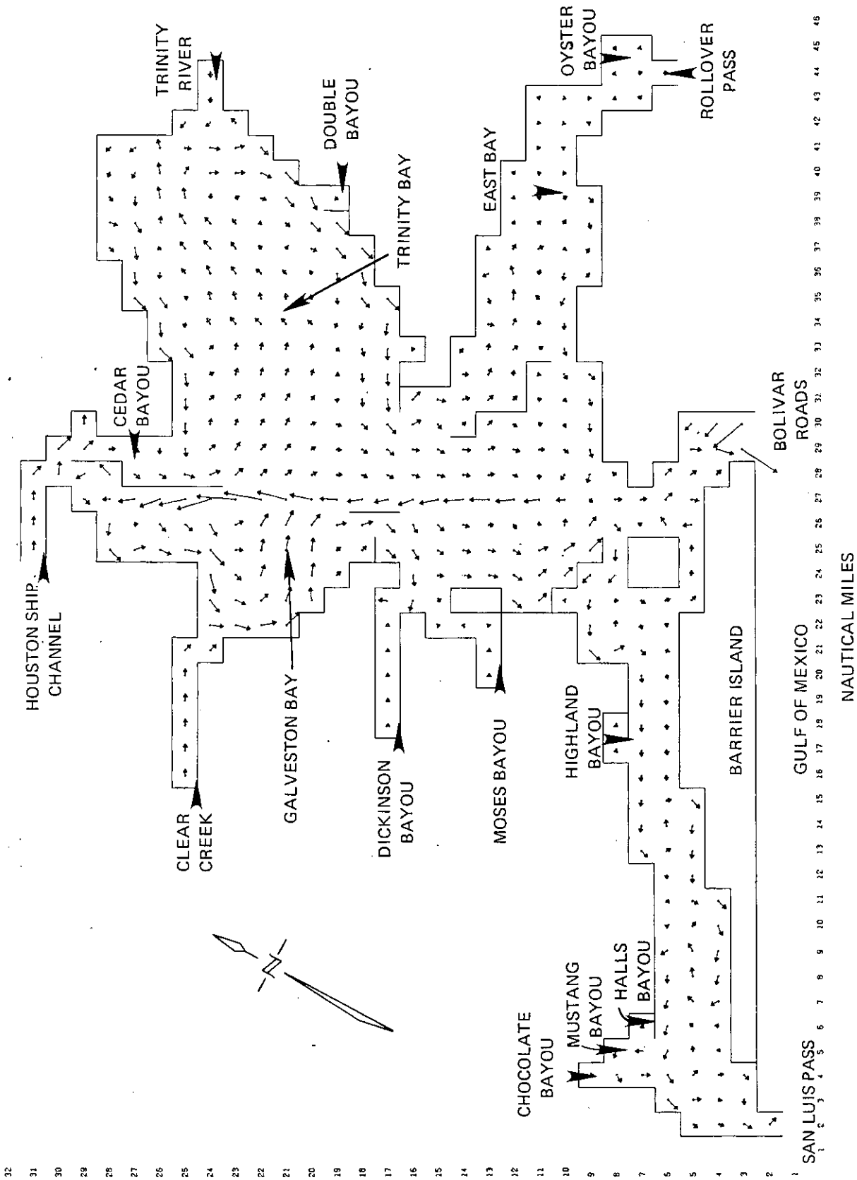
Figure 9-27. Simulated Net Steady-State Flows in the Trinity-San Jacinto Estuary Under August Freshwater Inflow Needs, Alternative I
