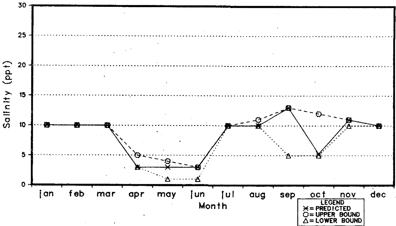
Figure 9-15. Average Monthly Salinities in Trinity Bay Under Alternative III
