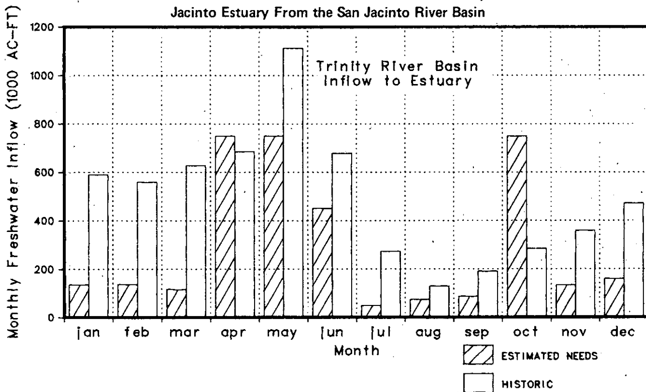
Figure 9-17. Comparison Between Mean Historical Freshwater Inflow and Inflow Needs Under Alternative III for the Trinity-San Jacinto Estuary From the Trinity River Basin
