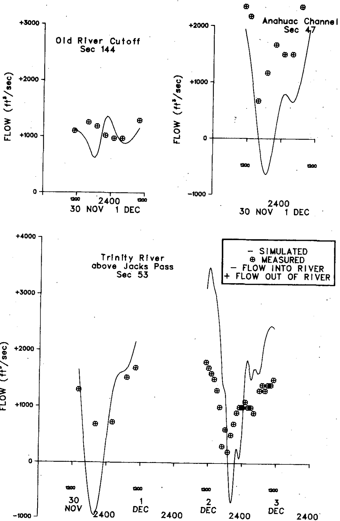
Figure 5-35. Comparison of Observed and Simulated Flows, Trinity-San Jacinto Estuary, November 30-December 3, 1976 (52)
