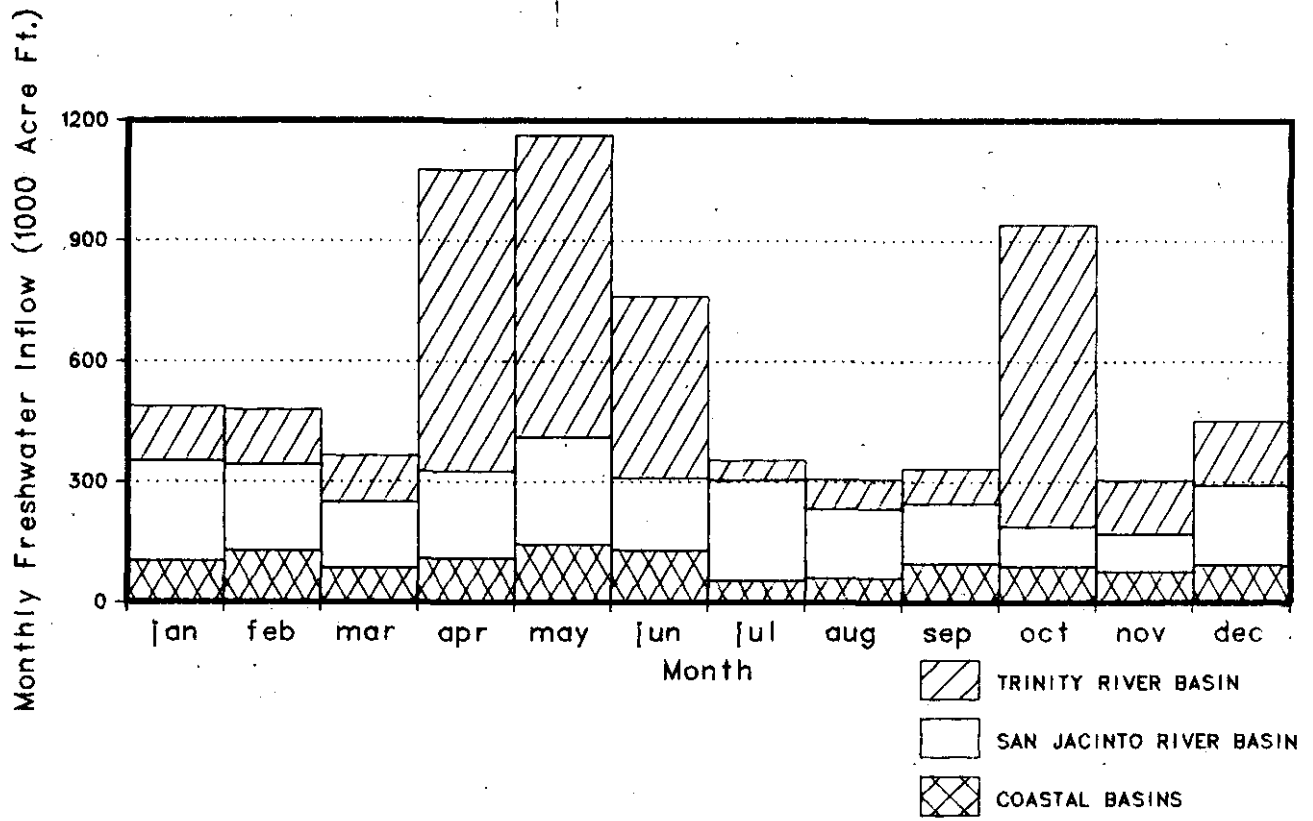
Figure 9-18. Estimated Freshwater Inflow Needs for the Trinity-San Jacinto Estuary Under Alternative III
