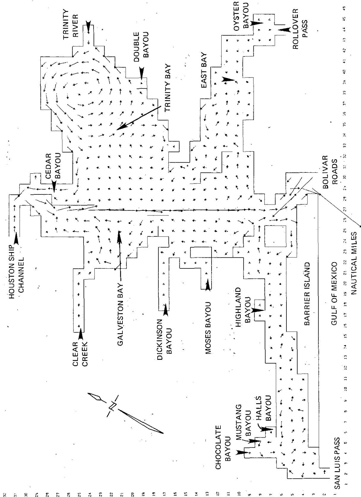
Figure 9-20. Simulated Net Steady-State Flows in the Trinity-San Jacinto Estuary Under January Freshwater Inflow Needs, Alternative I
