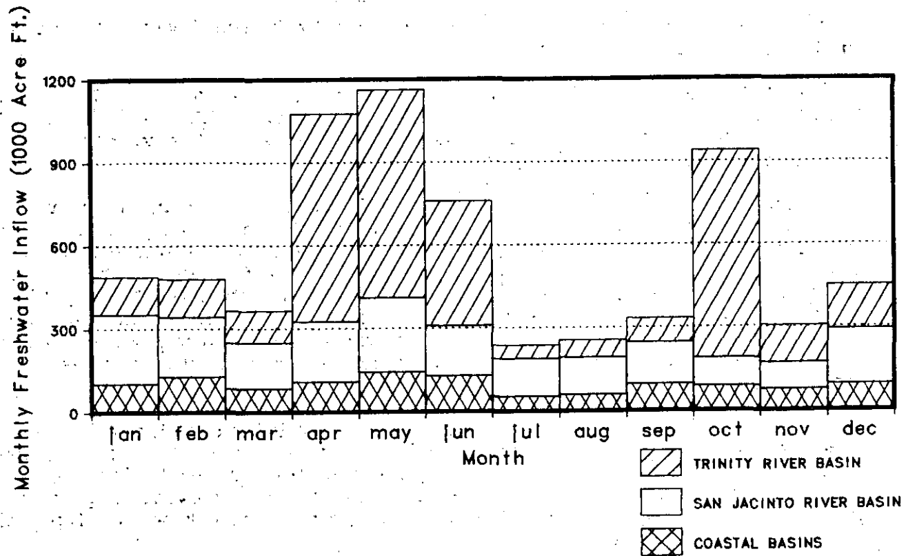
Figure 9-6. Estimated Freshwater Inflow Needs for the Trinity-San Jacinto Estuary Under Alternative I
