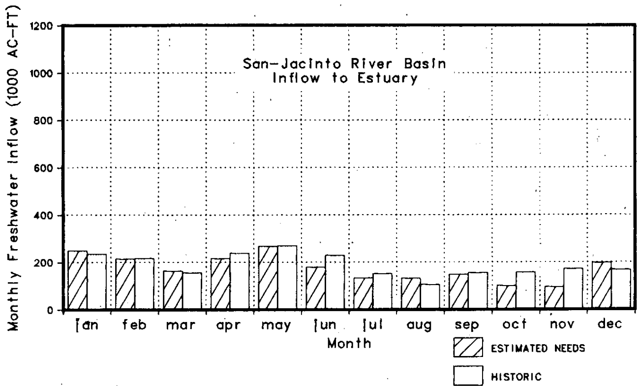
Figure 9-4. Comparison Between Mean Historical Freshwater Inflow and Inflow Needs Under Alternative I for the Trinity-San Jacinto Estuary From the San Jacinto River Basin
