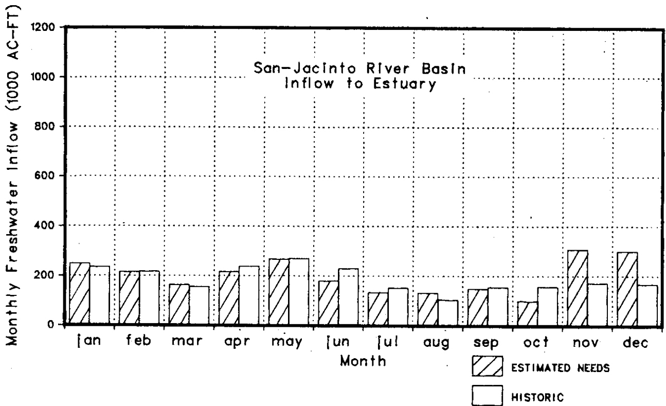
Figure 9-10. Comparison Between Mean Historical Freshwater Inflow and Inflow Needs Under Alternative II for the Trinity-San Jacinto Estuary From the San Jacinto River Basin
