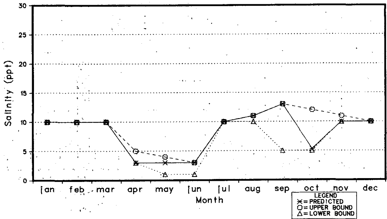
Figure 9-9. Average Monthly Salinities in Trinity Bay Under Alternative II
