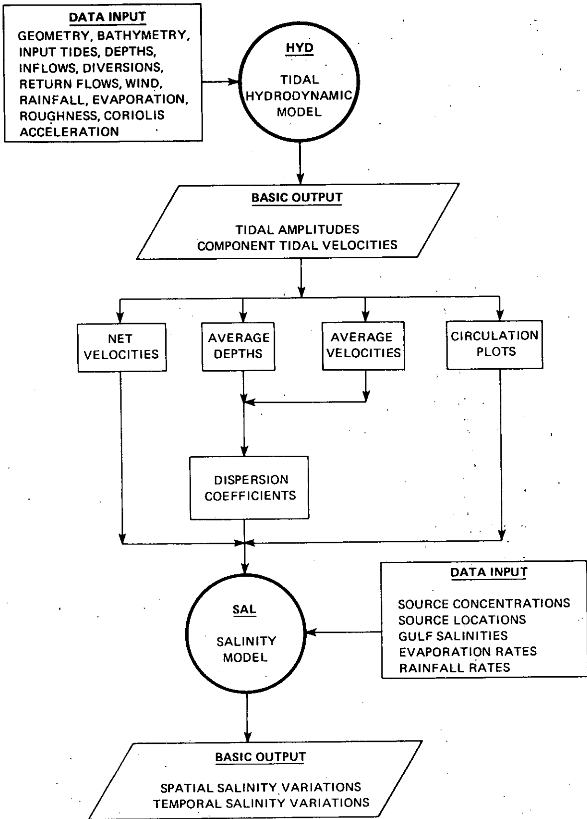
Figure 5-1. Relationship Between Tidal Hydrodynamic and Salinity Models (173)
