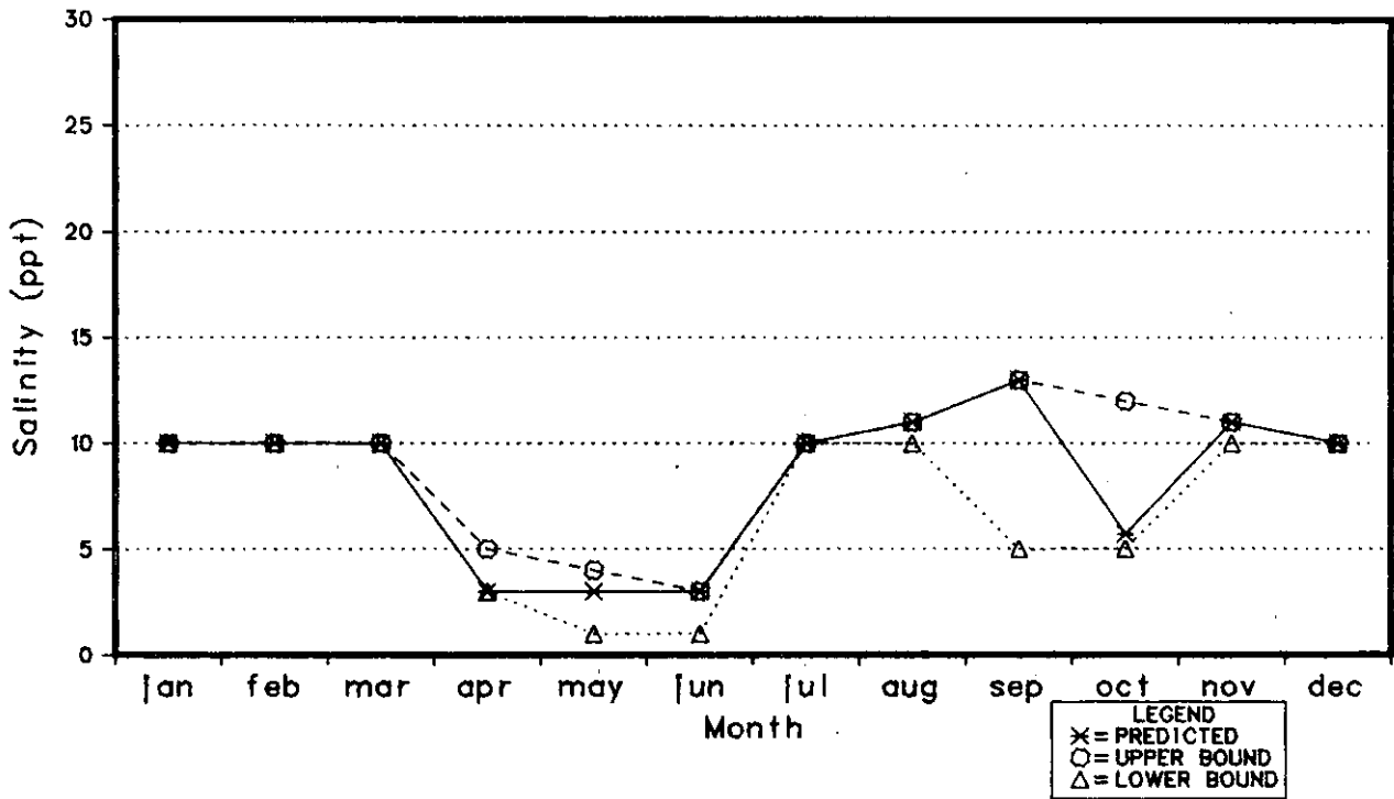
Figure 9-3. Average Monthly Salinities in Trinity Bay Under Alternative I
