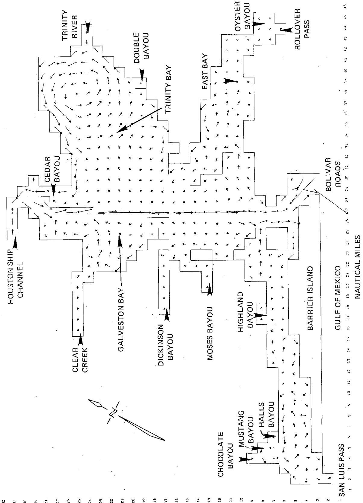
Figure 9-21. Simulated Net Steady-State Flows in the Trinity-San Jacinto Estuary Under February Freshwater Inflow Needs, Alternative I
