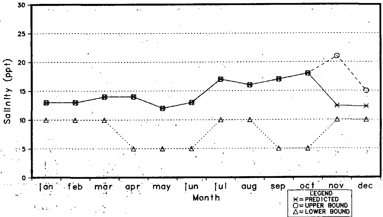
Figure 9-8. Average Monthly Salinities in Upper Galveston Bay Under Alternative II
