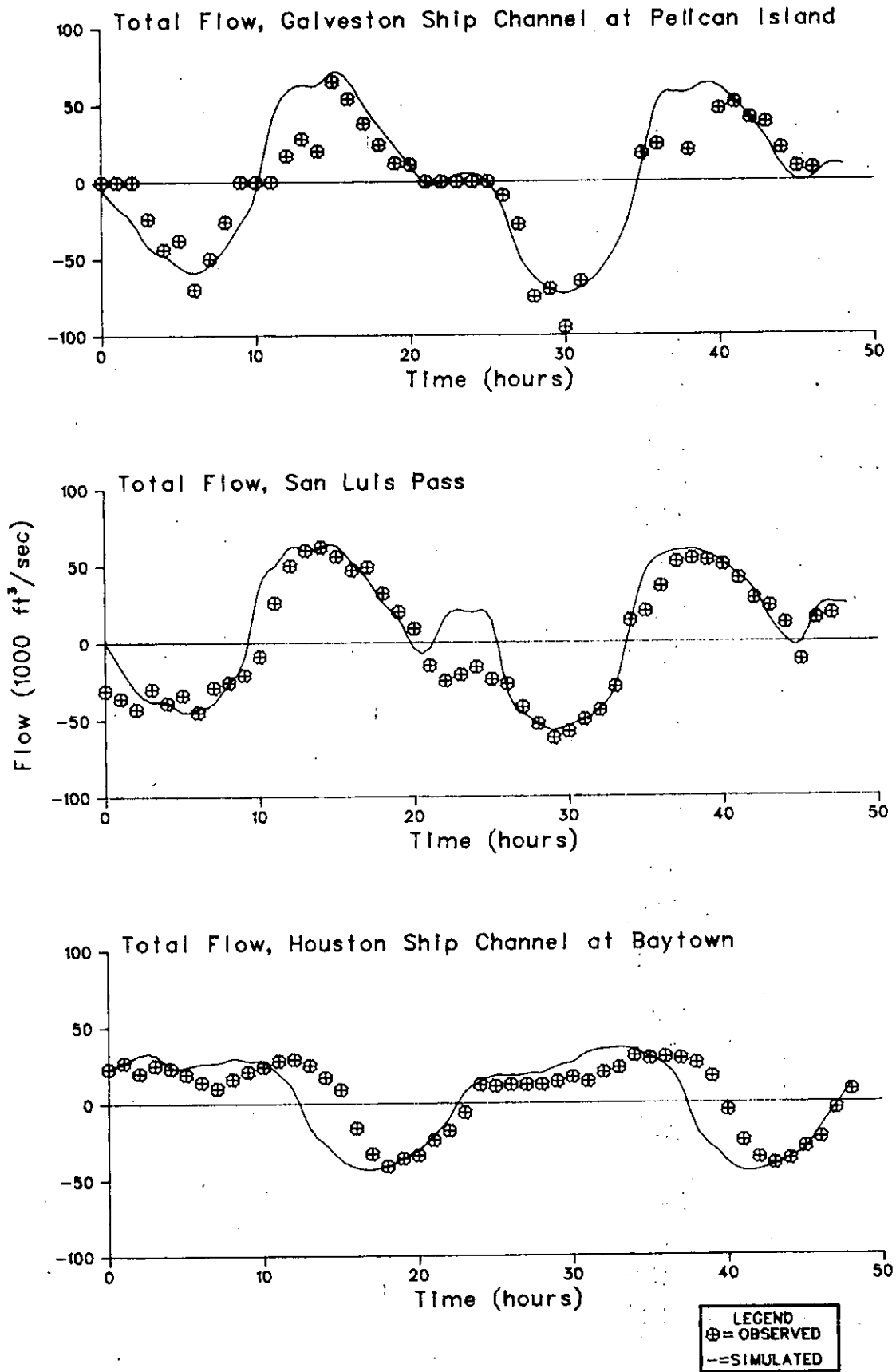
Figure 5-38. Comparison of Observed and Simulated Flows, Trinity-San Jacinto Estuary, July 21-23, 1976
