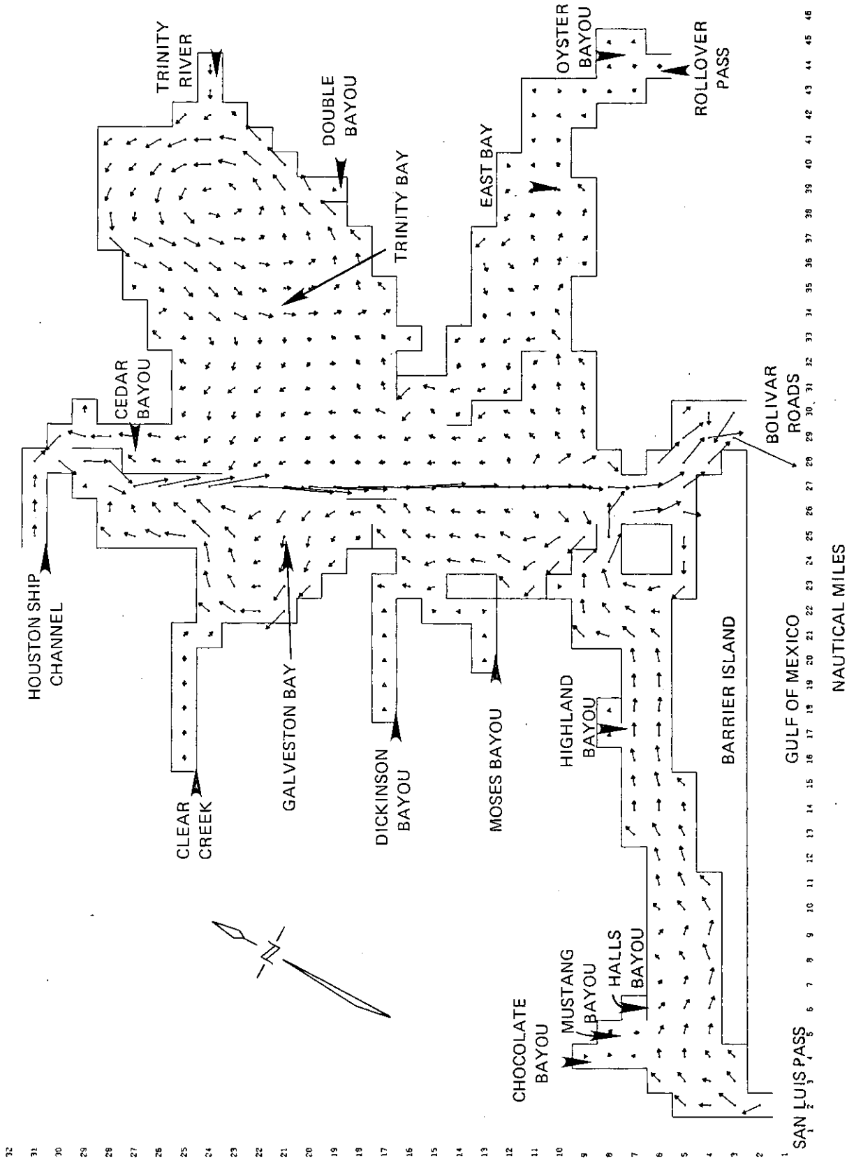
Figure 9-31. Simulated Net Steady-State Flows in the Trinity-San Jacinto Estuary Under December Freshwater Inflow Needs, Alternative I
