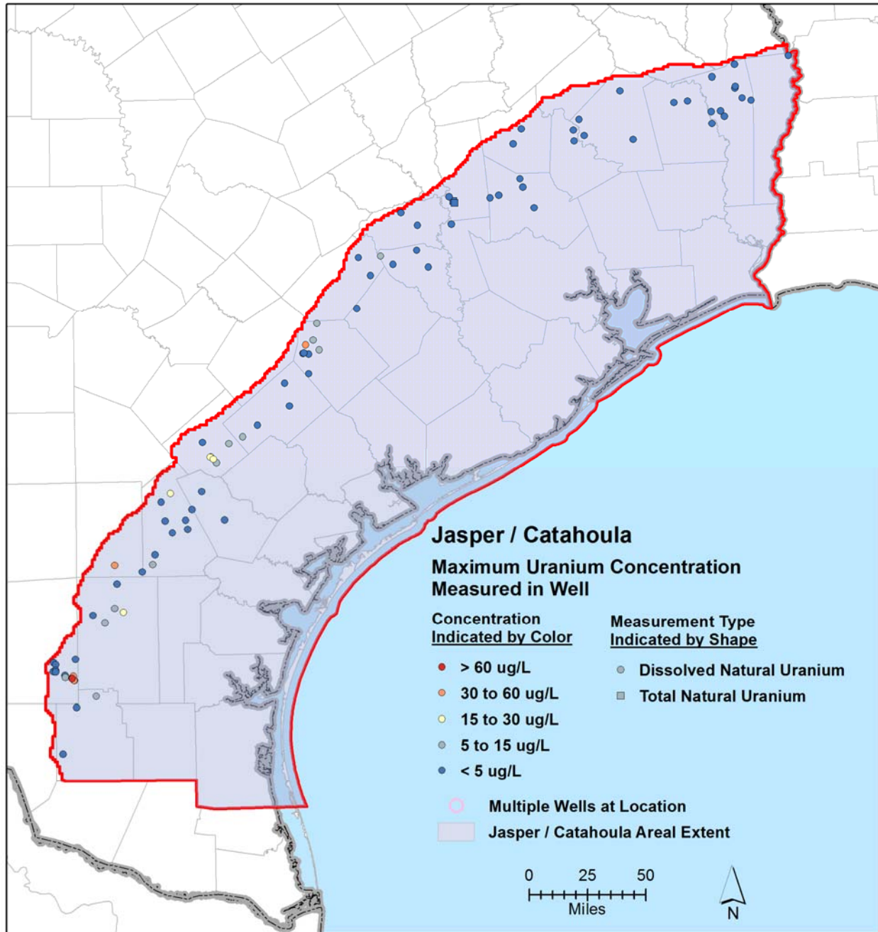
Figure 10-24. Maximum uranium concentration in the Jasper Aquifer and Catahoula Formation.
