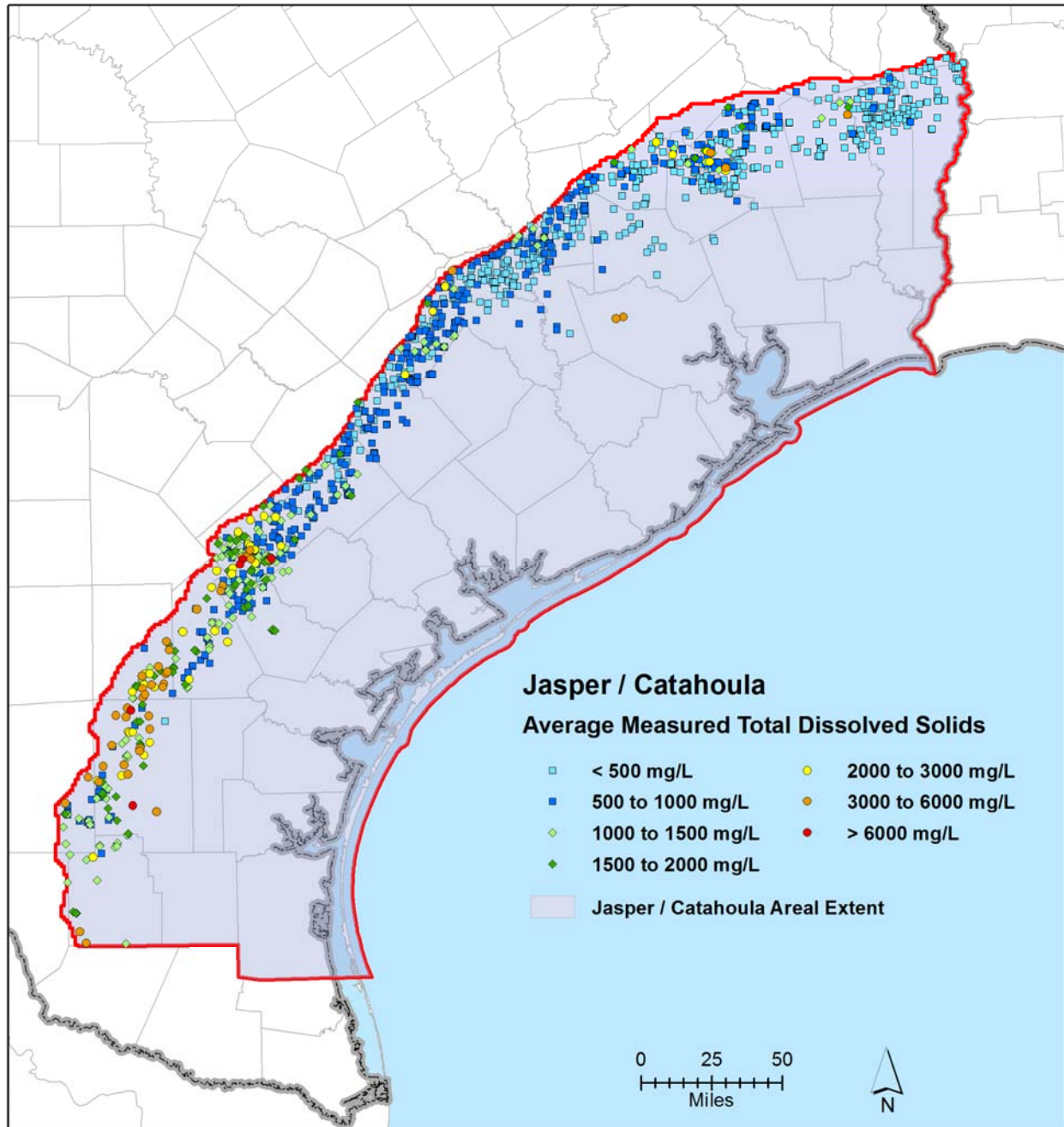
Figure 10-5. Average measured total dissolved solids concentration in the Jasper Aquifer and Catahoula Formation.
