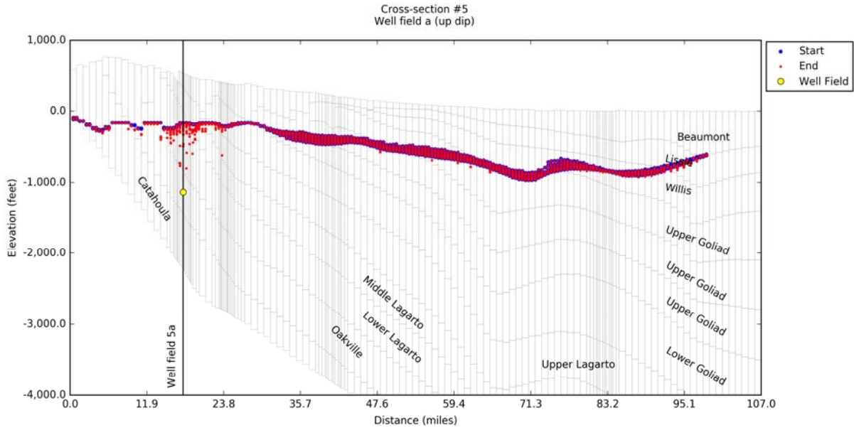
Figure 14-96. Simulated particle tracks 50 years after pumping the up dip Well Field #5a located along Cross-Section #5 on Figure 14-5 at 10,000 acre-feet per year.
