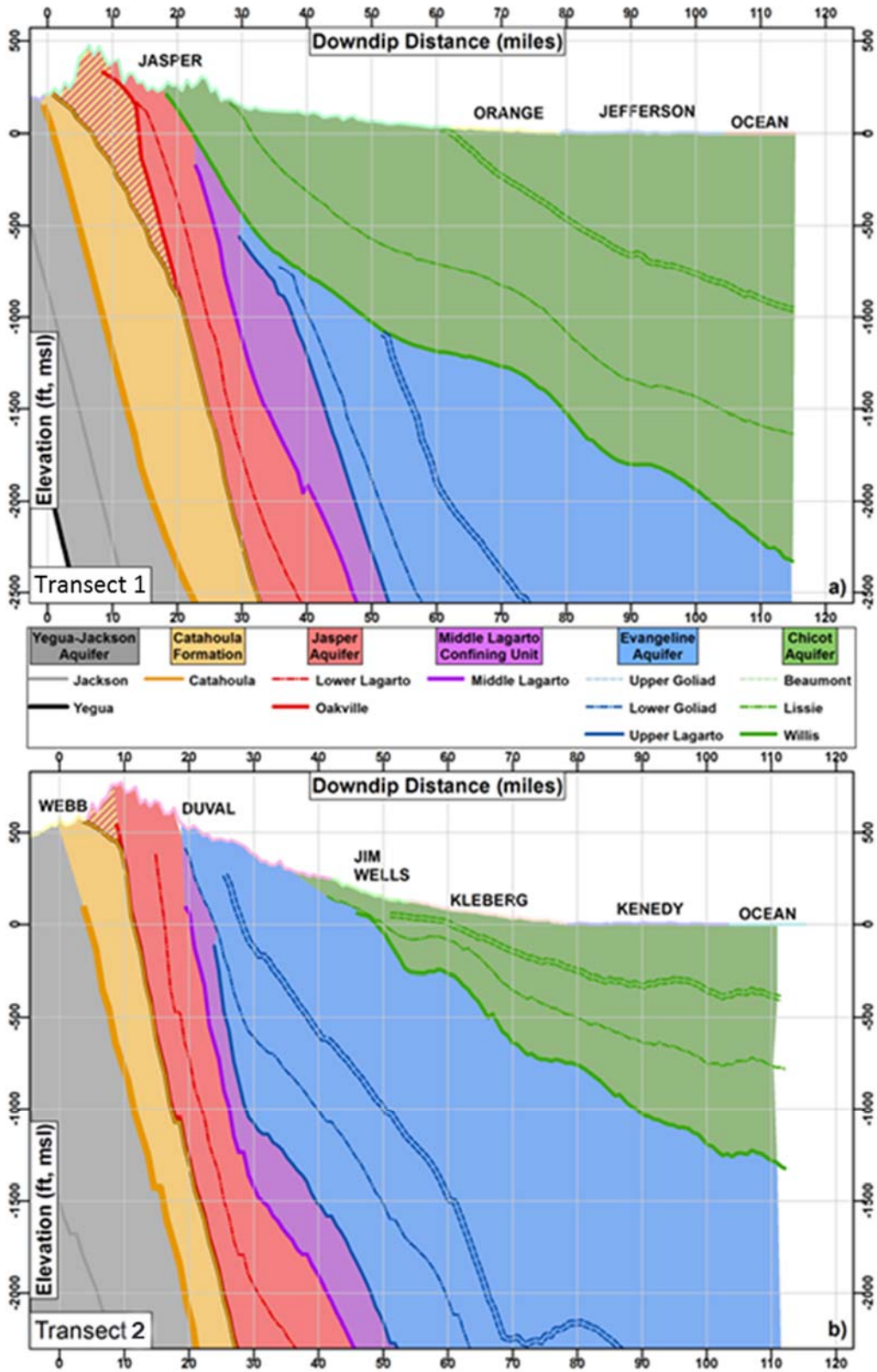
Figure 5-3. Geologic cross-sections through Transects 1 and 2 (note: surfaces represent the bottom of each geological formation).
