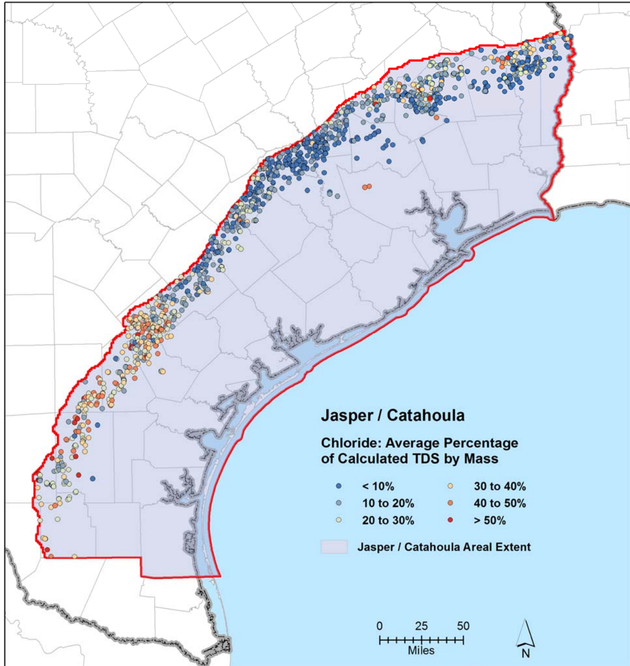
Figure 10-9. Chloride percentage of average calculated total dissolved solids concentration by mass for the Jasper Aquifer and Catahoula Formation.
