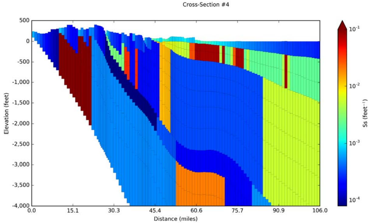
Figure 14-64. Specific storage (Ss) values for Cross-Section #4 on Figure 14-5 with aquifer properties from the Groundwater Management Area 16 Alternate Groundwater Availability Model (Hutchison and others, 2011) for model layers 1 to 12.
