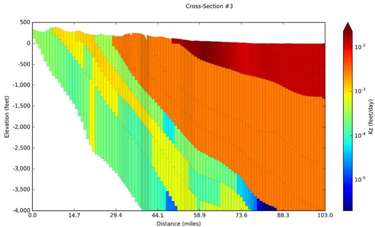
Figure 14-51. Vertical hydraulic (Kz) conductivity values in the groundwater model for Cross-Section #3 on Figure 14-5 for model layers 1 to 10.
