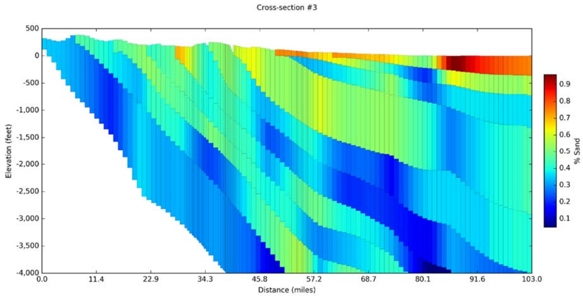
Figure 14-18. Sand fraction for model layers 1 to 10 for a vertical cross-section cut through the three-dimensional model for Cross-Section #3 on Figure 14-5.
