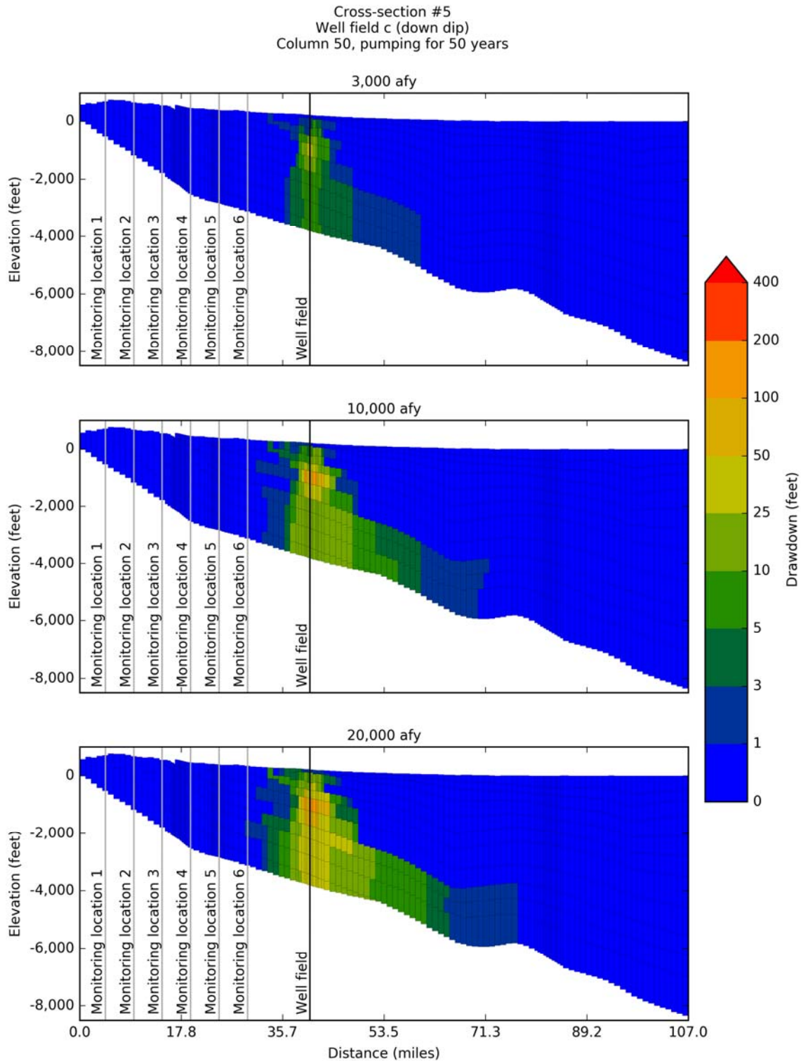
Figure 14-83. Simulated drawdown at 50 years after pumping the down dip Well Field #5c located along Cross-Section #5 on Figure 14-5 at 3,000 acre-feet per year, 10,000 acre-feet per year, and 20,000 acre-feet per year.
