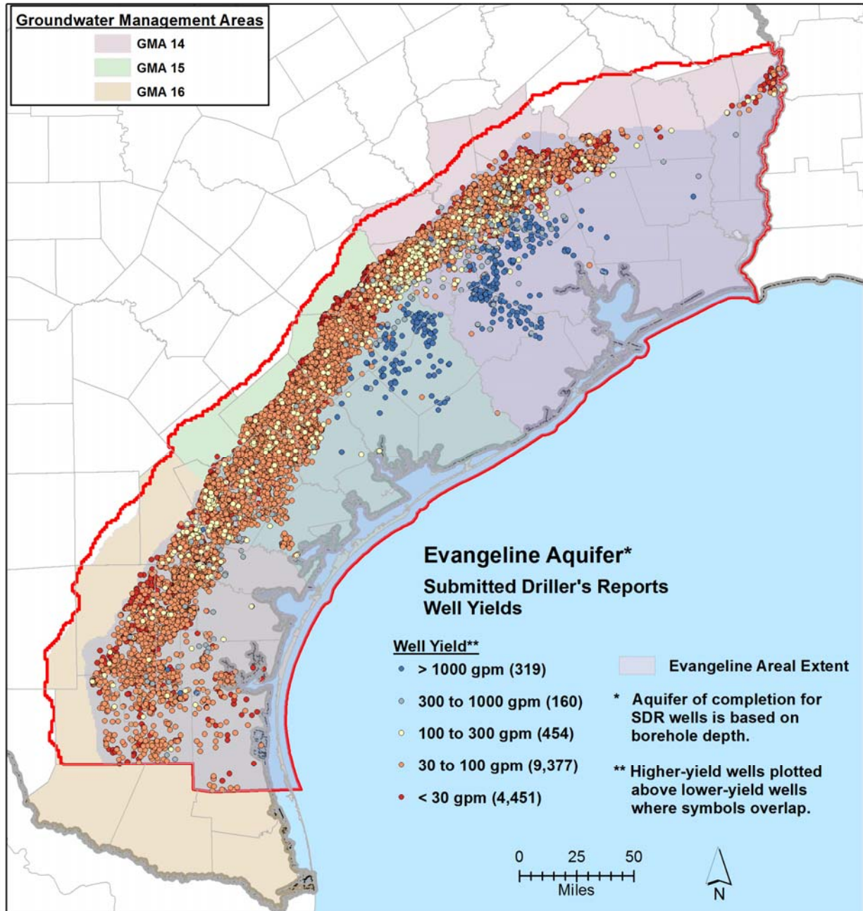
Figure 9-2. Reported well yields for the Evangeline Aquifer based on well information obtained from the TWDB Submitted Drillers Reports.
