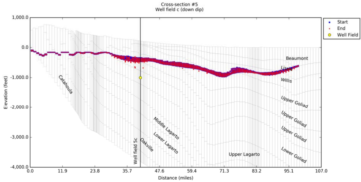
Figure 14-98. Simulated particle tracks 50 years after pumping the down dip Well Field #5c located along Cross-Section #5 on Figure 14-5 at 10,000 acre-feet per year.
