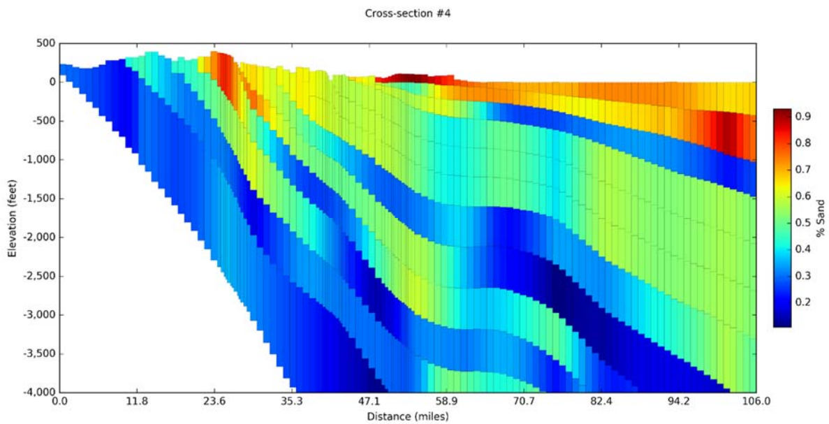
Figure 14-19. Sand fraction for model layers 1 to 12 for a vertical cross-section cut through the three-dimensional model for Cross-Section #4 on Figure 14-5.
