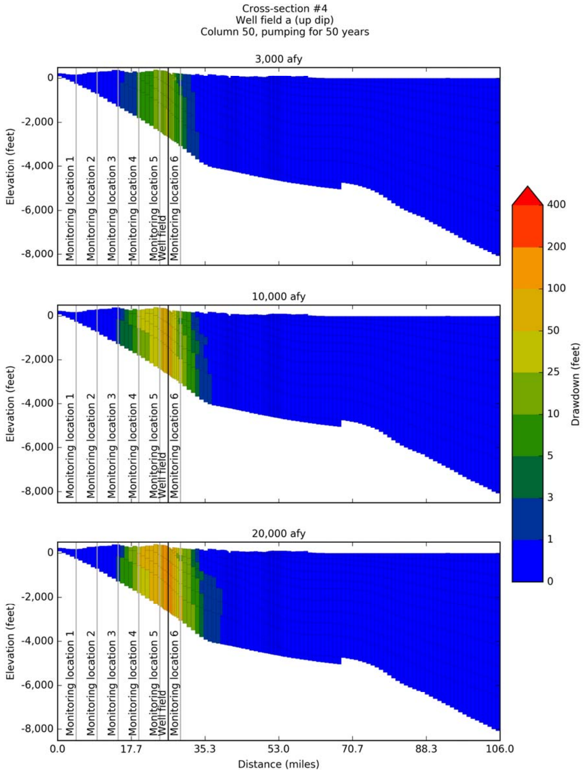
Figure 14-67. Simulated drawdown at 50 years after pumping the up dip Well Field #4a located along Cross-Section #4 on Figure 14-5 at 3,000 acre-feet per year, 10,000 acre-feet per year, and 20,000 acre-feet per year.
