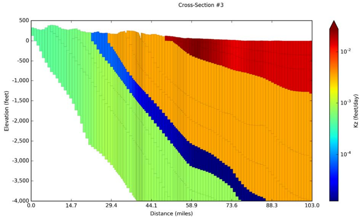
Figure 14-50. Vertical hydraulic conductivity (Kz) values for Cross-Section #3 on Figure 14-5 with aquifer properties from the Central Gulf Coast Groundwater Availability Model (Chowdhury and others, 2004) for model layers 1 to 10.
