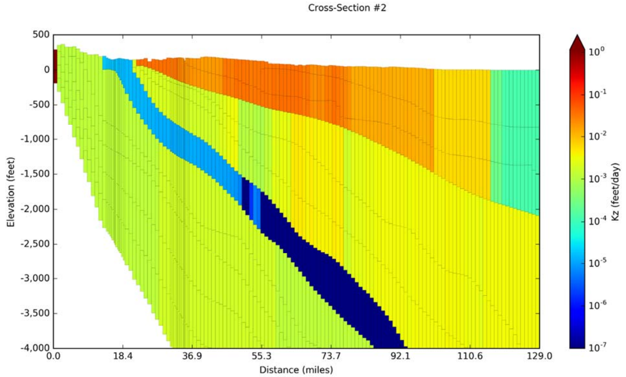
Figure 14-38. Vertical hydraulic conductivity ( K_z ) values for Cross-Section #2 on Figure 14-5 with aquifer properties from the Houston Area Groundwater Model (Kasmarek, 2012) for model layers 1 to 12.
