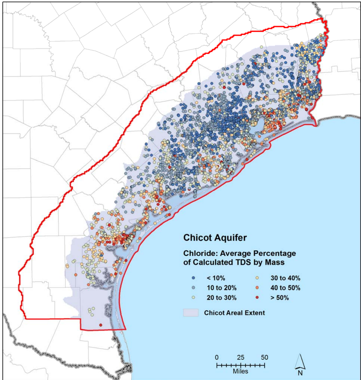
Figure 10-7. Chloride percentage of average calculated total dissolved solids concentration by mass for the Chicot Aquifer.
