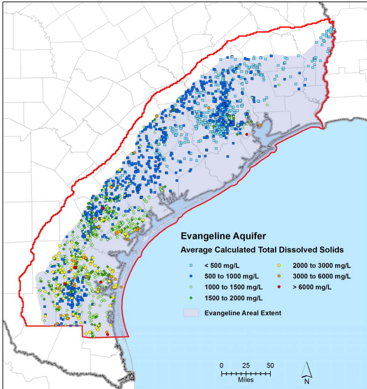
Figure 10-4. Average calculated total dissolved solids concentration in the Evangeline Aquifer.
