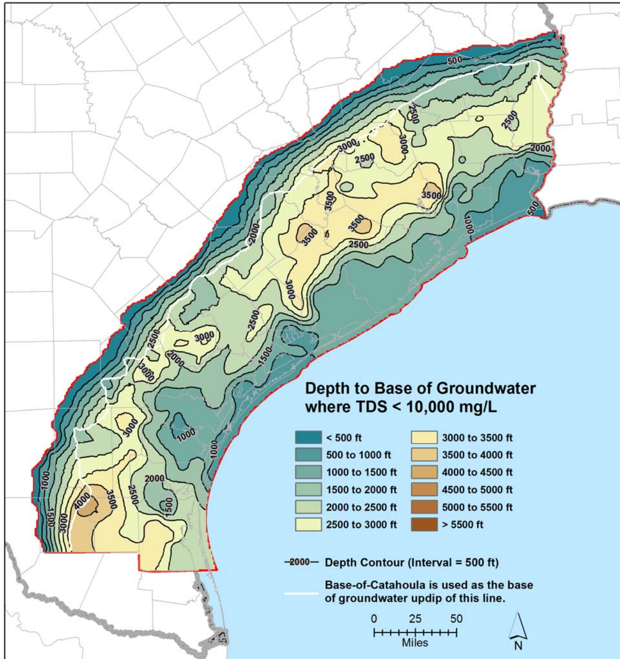
Figure 6-5. Base of the moderately saline zone.
