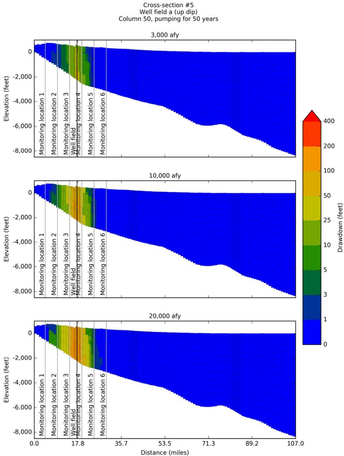
Figure 14-79. Simulated drawdown at 50 years after pumping the up dip Well Field #5a located along Cross-Section #5 on Figure 14-5 at 3,000 acre-feet per year, 10,000 acre-feet per year, and 20,000 acre-feet per year.
