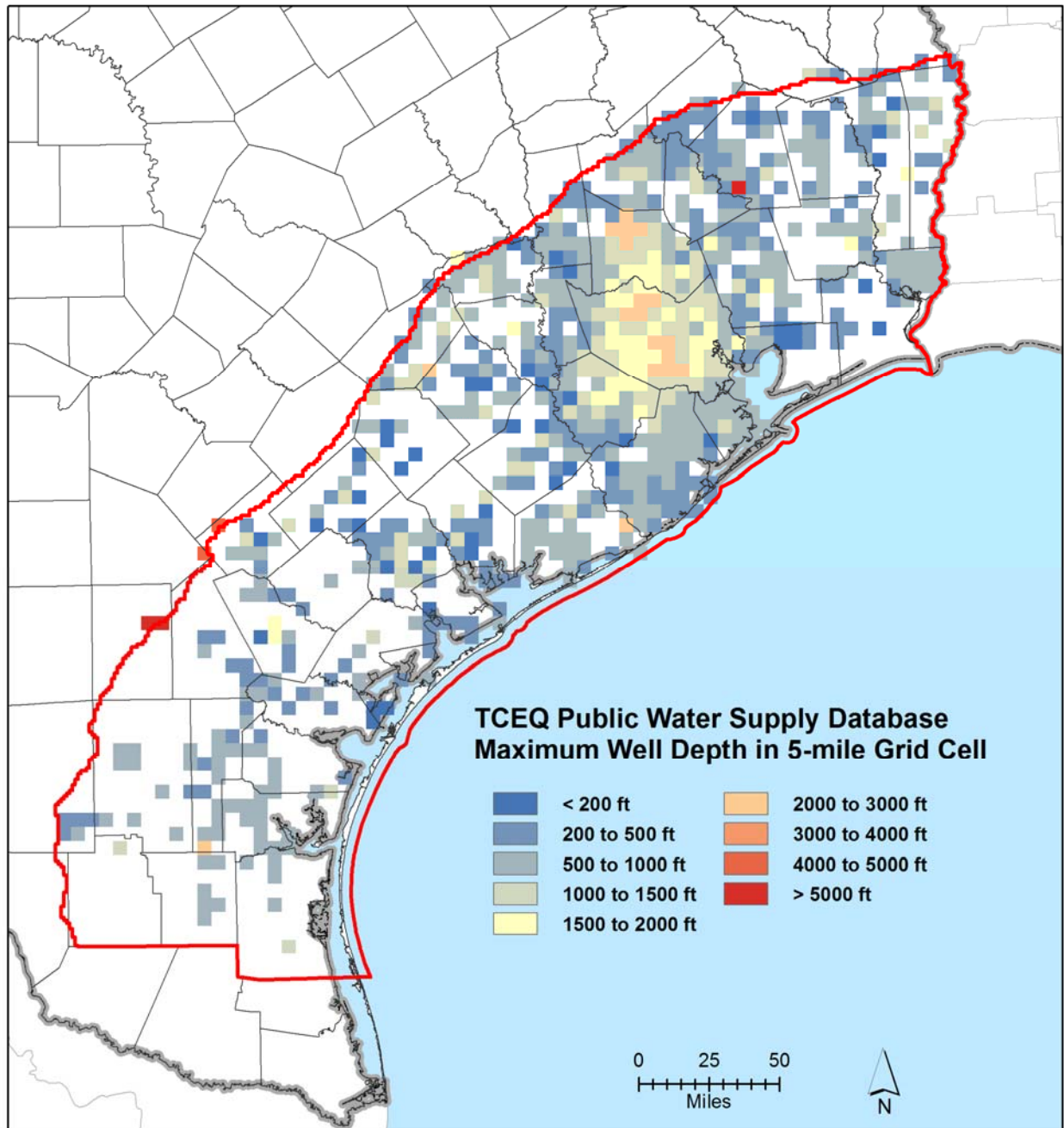
Figure 6-32. Maximum depth of public water supply wells that occur across 5 mile-by-5-mile grid cells based on well information obtained from the Texas Commission on Environmental Quality.
