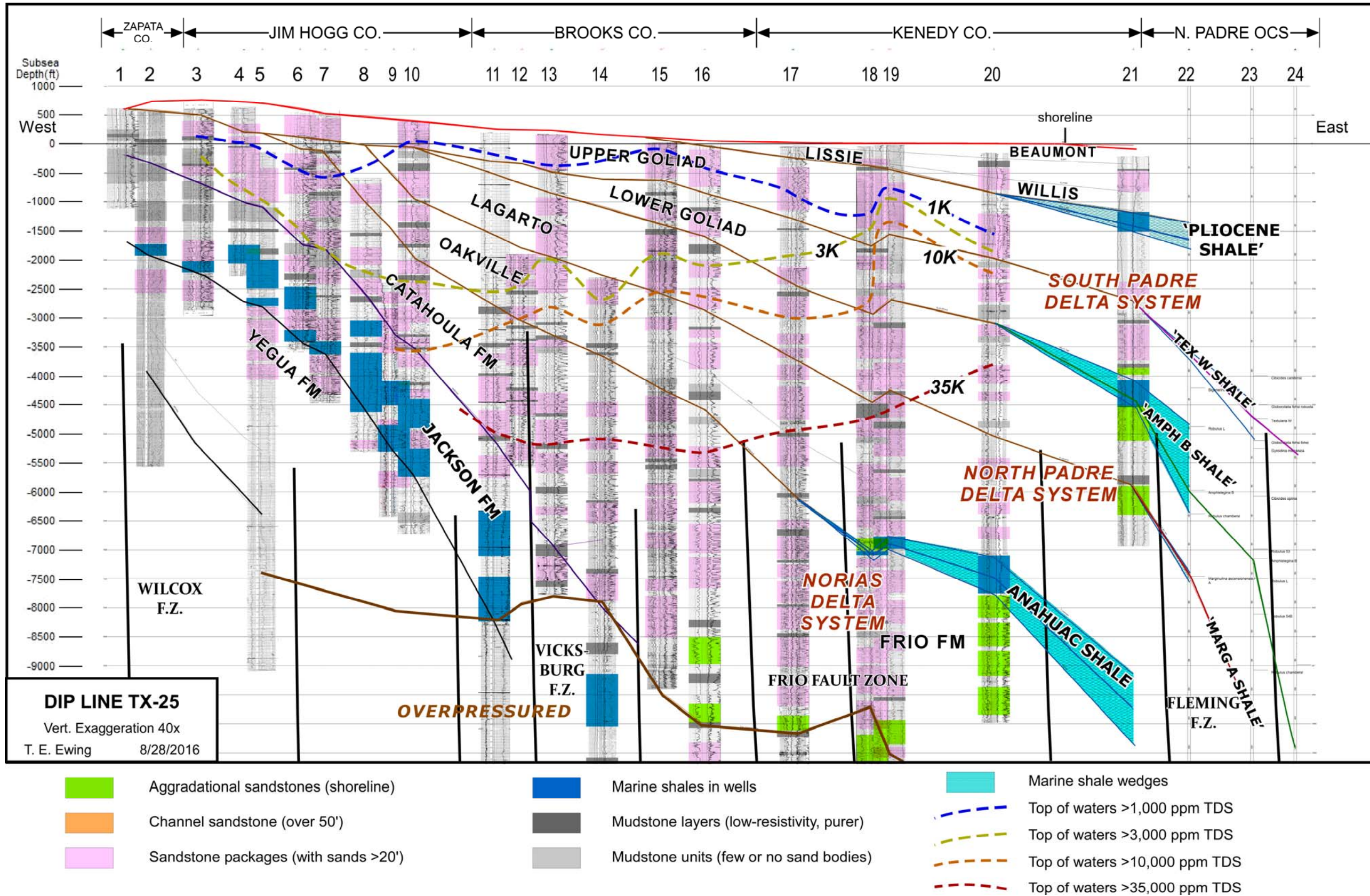
Figure 11-16. Analysis of sand and clay sequences, fault zones, along Cross-Section #25 in Figure 6-1.
