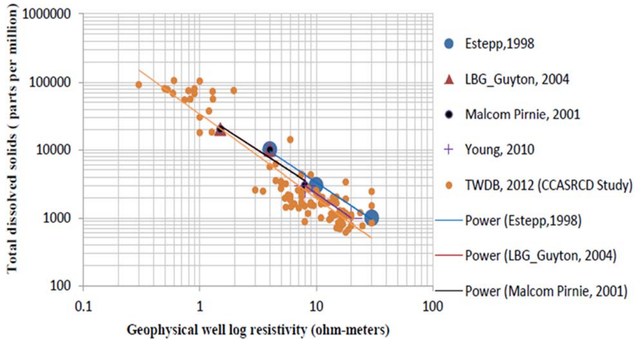
Figure 13-10 Comparison of total dissolved solids concentration of formation water and deep resistivity from geophysical well logs (from Meyer, 2012).
