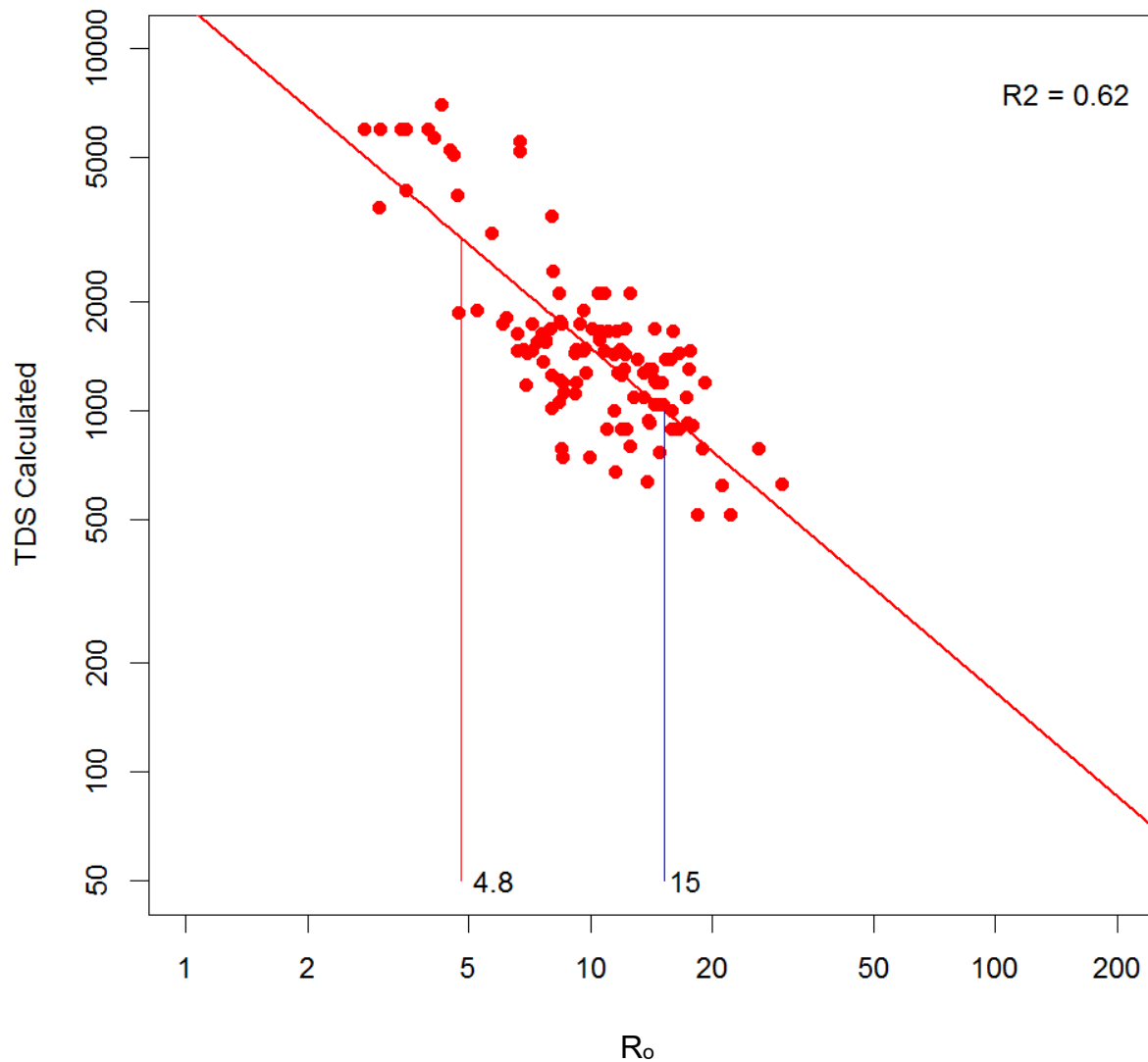
Figure 13-21. R 0 -TDS graph for the Jasper/Catahoula Aquifer Group (including the Lower Lagarto, Oakville, and Catahoula formations) based on 117 well-log pairs. The blue line is the formation resistivity value for a 1,000 milligram per liter total dissolved solids concentration and the red line is the formation resistivity value for 3,000 milligrams per liter total dissolved solids concentration.
