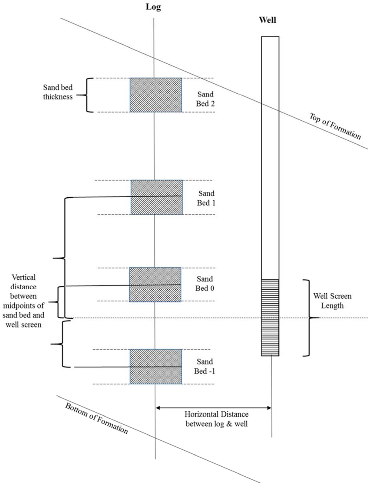
Figure 13-12. Schematic showing the sand beds identified on a geophysical log and a nearby well screen where total dissolved solids concentrations have been measured.
