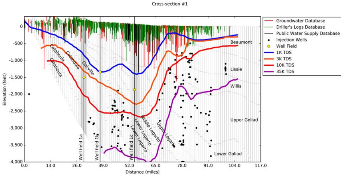
Figure 14-11. Boundaries for fresh water, slightly saline, moderately saline, and very saline groundwater along Cross-Section #1 on Figure 14-5.
