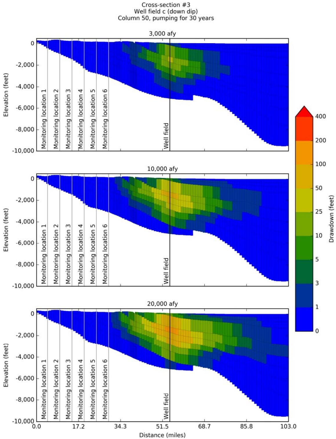
Figure 14-58. Simulated drawdown at 30 years after pumping the down dip Well Field #3c located along Cross-Section #3 on Figure 14-5 at 3,000 acre-feet per year, 10,000 acre-feet per year, and 20,000 acre-feet per year.
