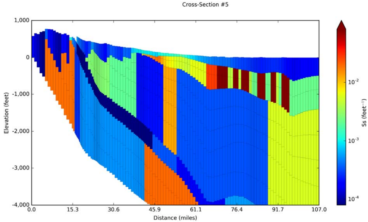
Figure 14-76. Specific storage (Ss) values for Cross-Section #5 on Figure 14-5 with aquifer properties from the Groundwater Management Area 16 Alternate Groundwater Availability Model (Hutchison and others, 2011) for model layers 1 to 12.
