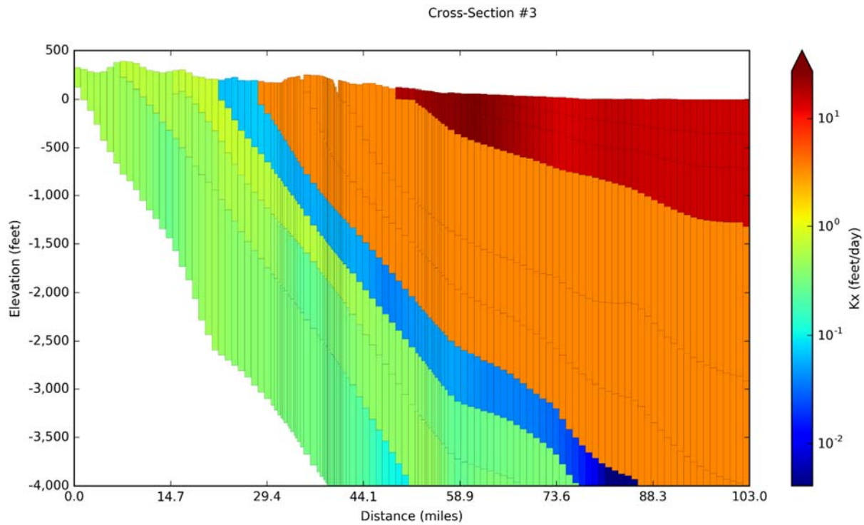
Figure 14-49. Horizontal hydraulic conductivity ( K_x ) values in the groundwater model for Cross-Section #3 on Figure 14-5 for model layers 1 to 10.
