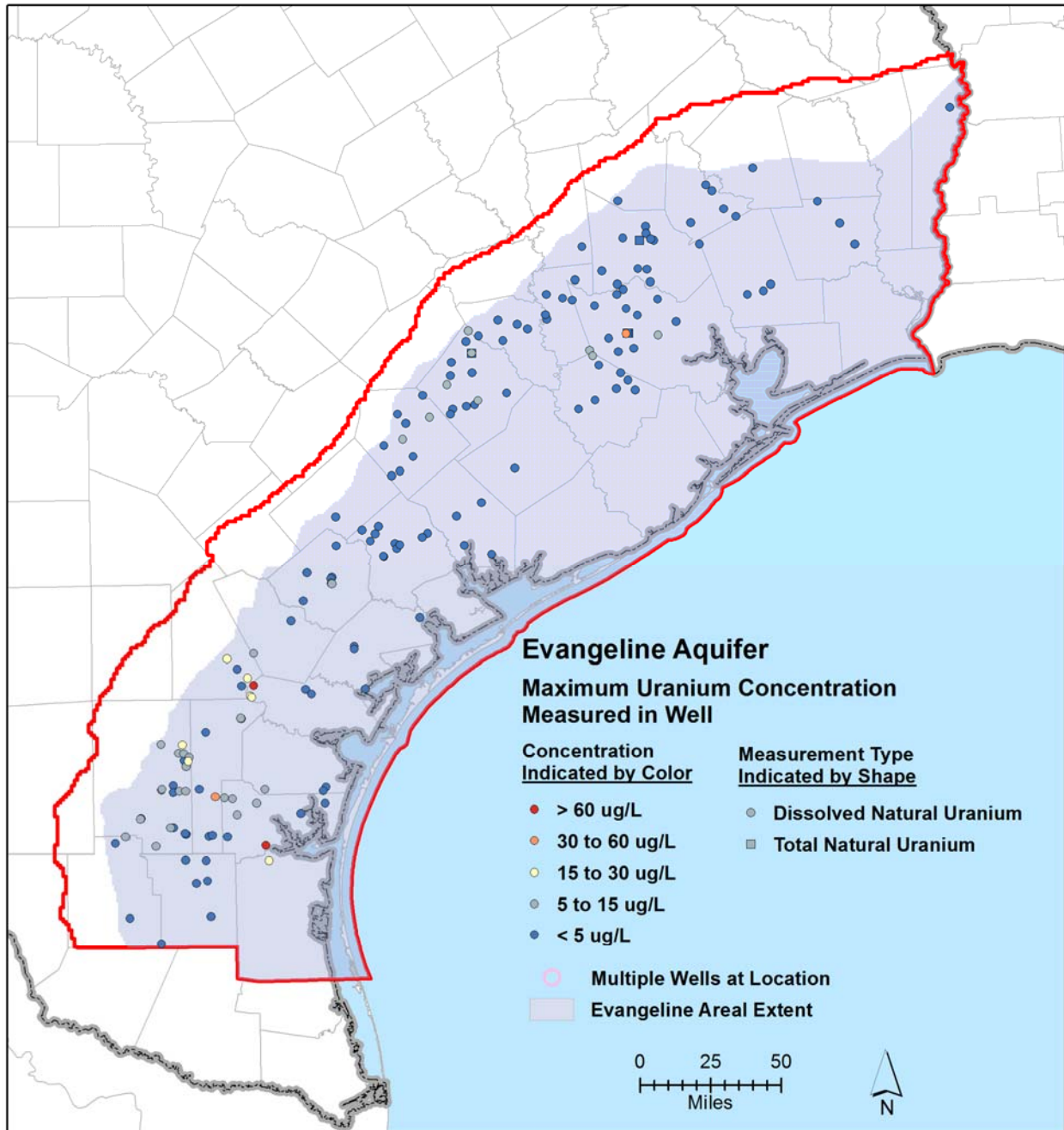
Figure 10-23. Maximum uranium concentration in the Evangeline Aquifer.
