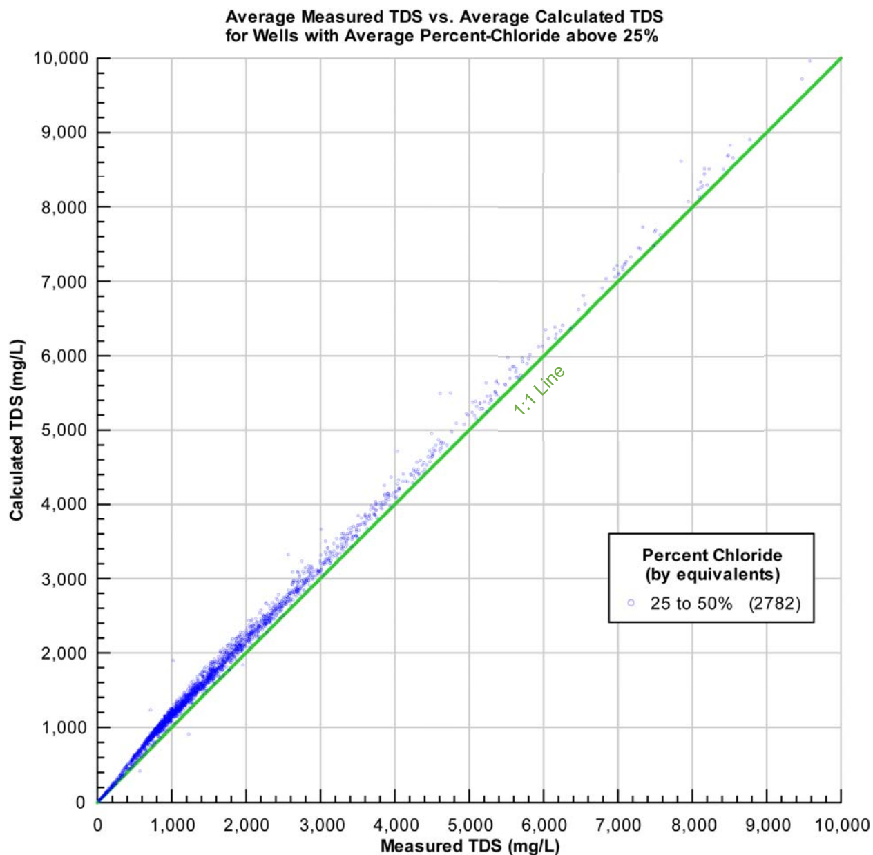
Figure 13-4. Calculated total dissolved solids concentration versus measured total dissolved solids concentration for groundwater samples from the Texas Gulf Coast Aquifer System that have more than 25 percent of their equivalents contributed by chloride.
