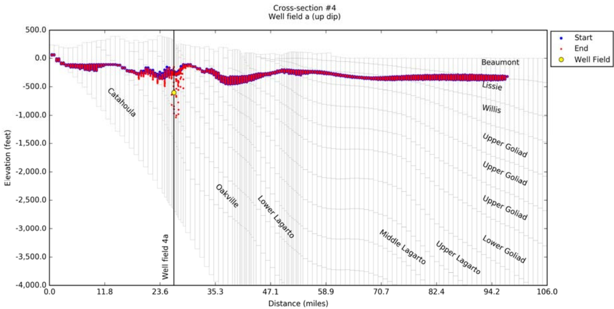
Figure 14-93. Simulated particle tracks 50 years after pumping the up dip Well Field #4a located along Cross-Section #4 on Figure 14-5 at 10,000 acre-feet per year.
