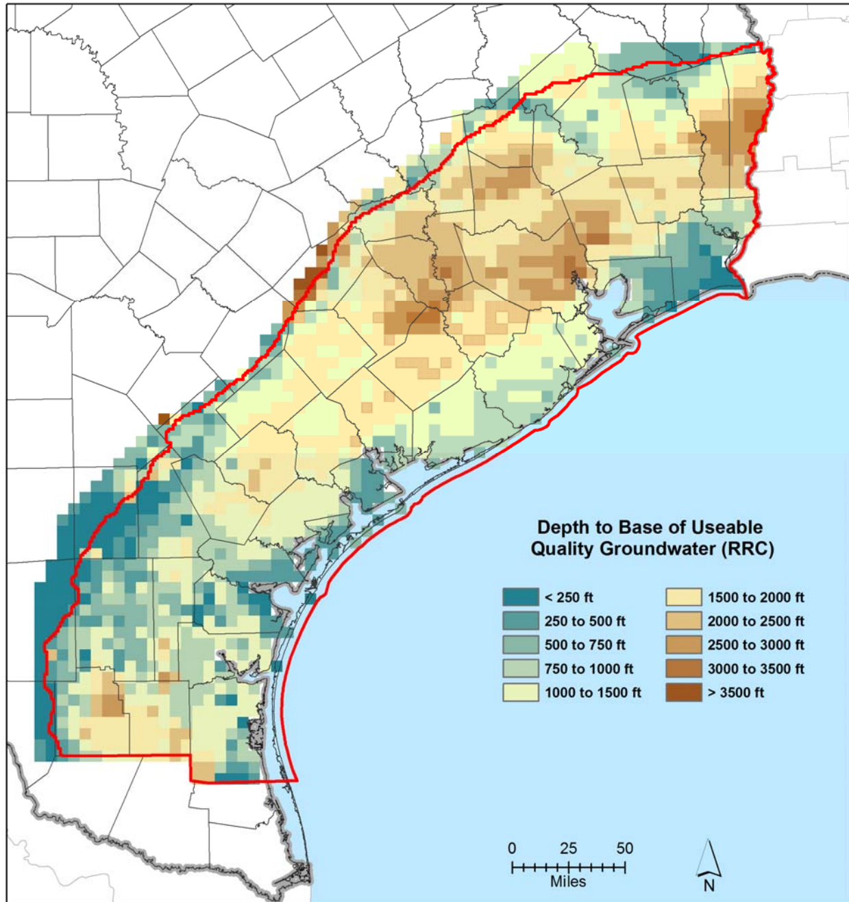
Figure 6-11. Estimated depth to useable quality water, which is defined as a total dissolved solid concentration of 3,000 milligrams per liter, based on 53,000 picks of depth to fresh water from a database maintained by the Groundwater Advisory Unit of the Railroad Commission of Texas
