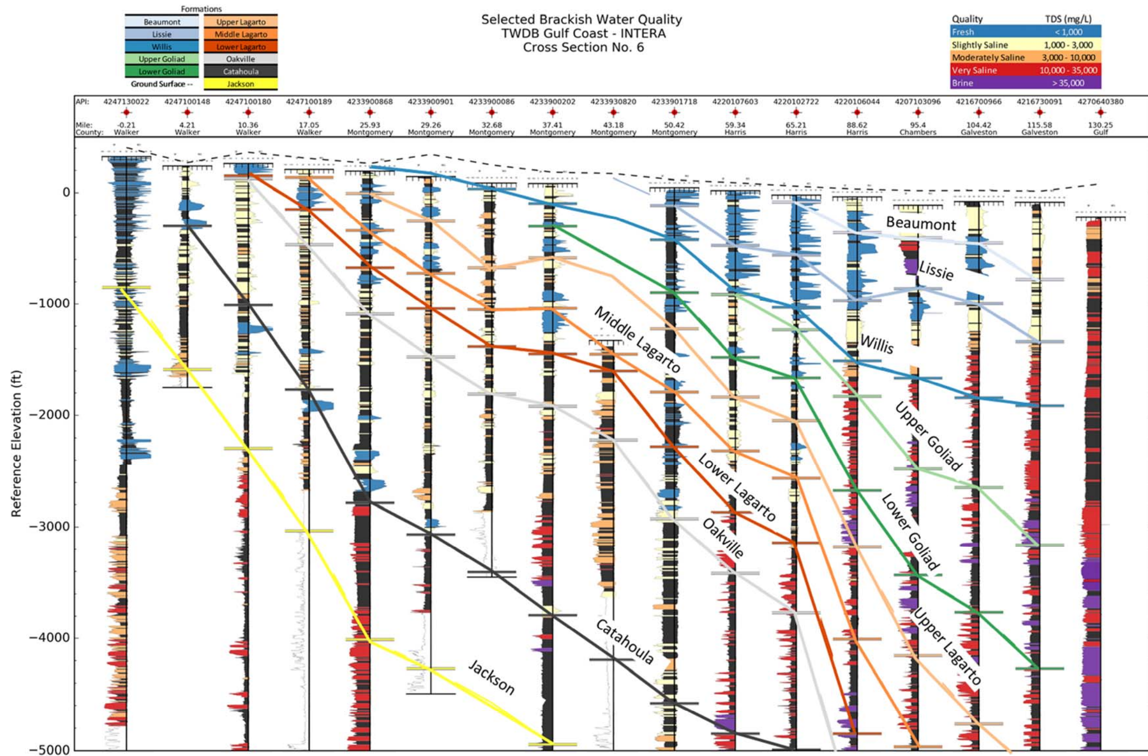
Figure 6-15. Profiles of calculated salinity zones for sand beds identified on geophysical logs aligned on Cross-Section #6 shown in Figure 6-1. Markers represent the base formations at each log location. The lines connecting the markers are for illustrative purposes only. Dashed line indicates crossing a log with no marker available in an active interval.
