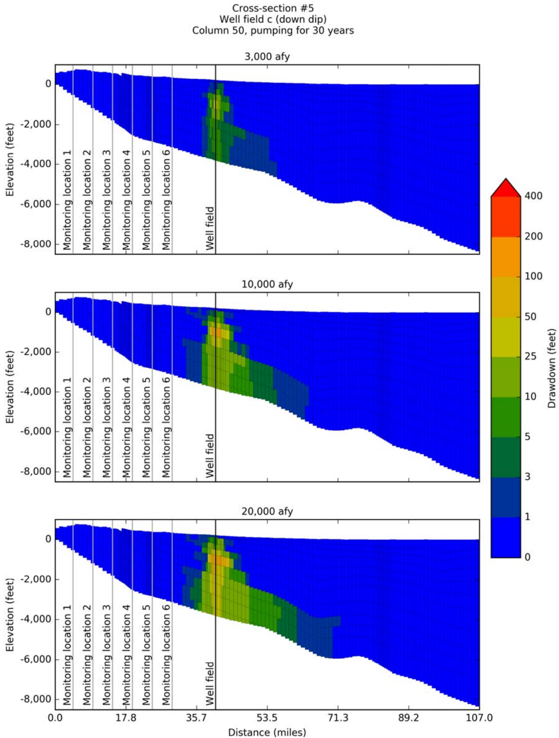
Figure 14-82. Simulated drawdown at 30 years after pumping the down dip Well Field #5c located along Cross-Section #5 on Figure 14-5 at 3,000 acre-feet per year, 10,000 acre-feet per year, and 20,000 acre-feet per year.
