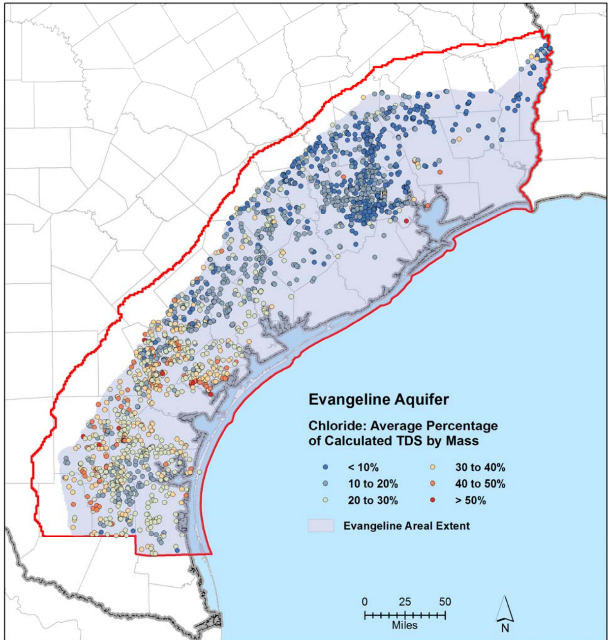
Figure 10-8. Chloride percentage of average calculated total dissolved solids concentration by mass for the Evangeline Aquifer.
