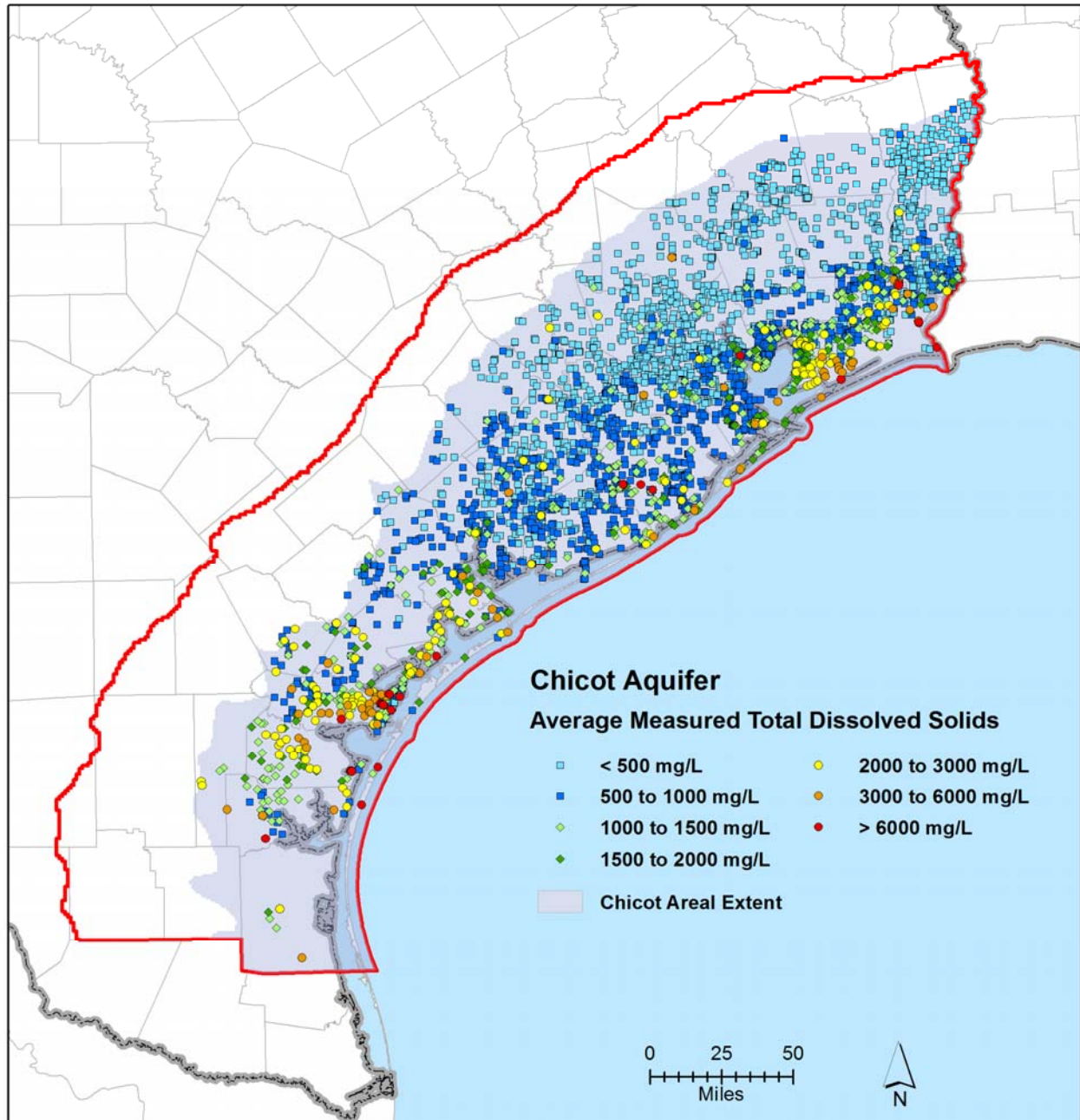
Figure 10-1. Average measured total dissolved solids concentration in the Chicot Aquifer.
