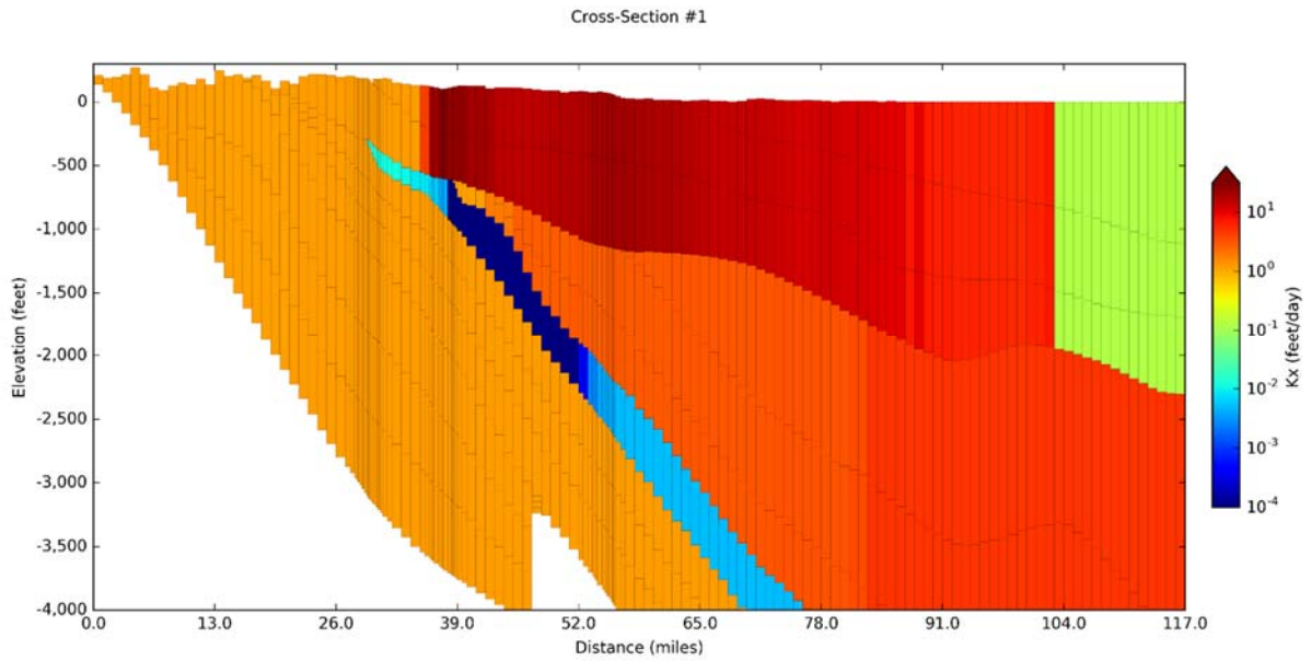
Figure 14-24. Horizontal hydraulic conductivity ( K_x ) values for Cross-Section #1 on Figure 14-5 with aquifer properties from the Houston Area Groundwater Model (Kasmarek, 2012) for model layers 1 to 13.
