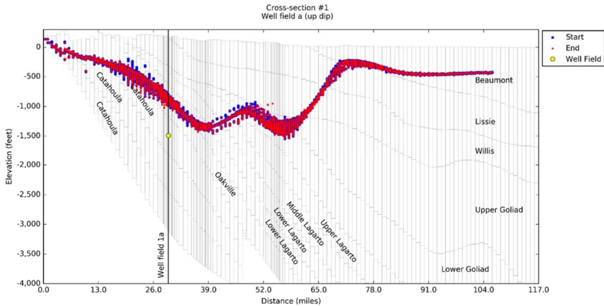
Figure 14-84 Simulated particle tracks 50 years after pumping the up dip Well Field #1a located along Cross-Section #1 on Figure 14-5 at 10,000 acre-feet per year.
