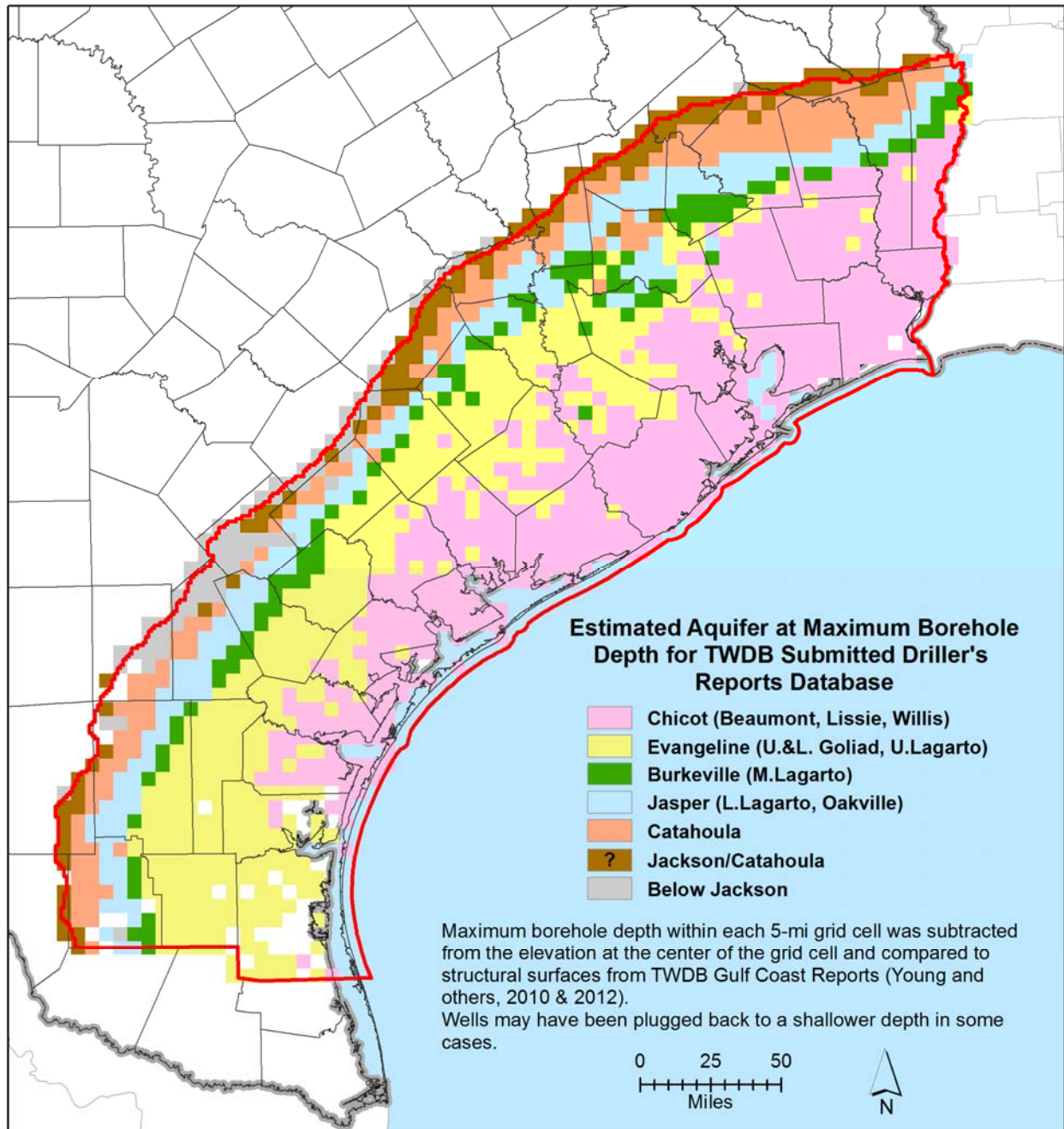
Figure 6-34. The estimated geologic formation in which the deepest well in 5 mile-by-5-mile grid cells terminates. Well information obtained from the TWDB Submitted Drillers Report.
