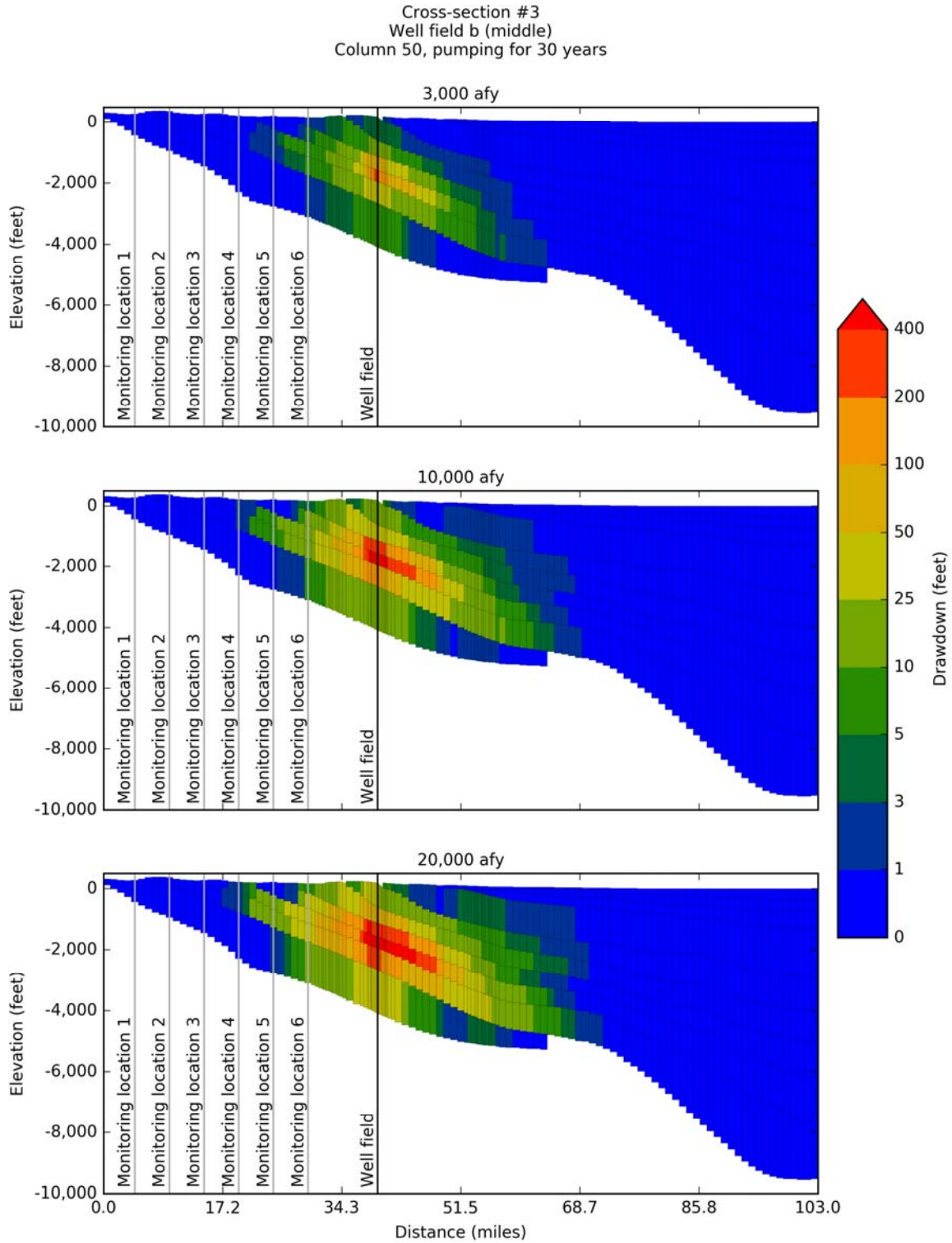
Figure 14-56. Simulated drawdown at 30 years after pumping the central Well Field #3b located along Cross-Section #3 on Figure 14-5 at 3,000 acre-feet per year, 10,000 acre-feet per year, and 20,000 acre-feet per year.
