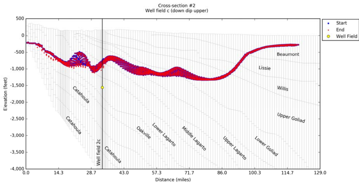
Figure 14-89. Simulated particle tracks 50 years after pumping the down dip Well Field #2c located along Cross-Section #2 on Figure 14-5 at 10,000 acre-feet per year.
