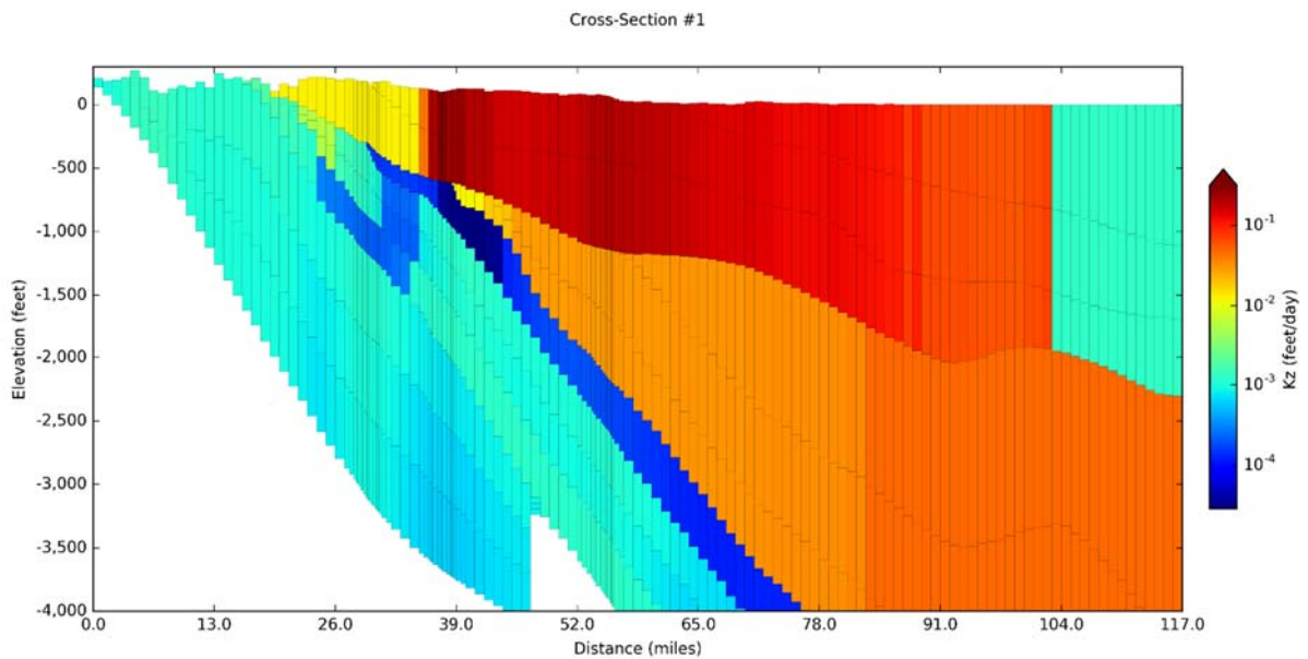
Figure 14-27. Vertical hydraulic conductivity ( K_z ) values in the groundwater model for Cross-Section #1 on Figure 14-5 for model layers 1 to 13.
