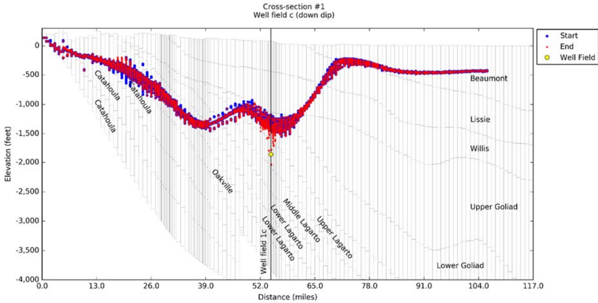
Figure 14-86. Simulated particle tracks 50 years after pumping the down dip Well Field #1c located along Cross-Section #1 on Figure 14-5 at 10,000 acre-feet per year.
