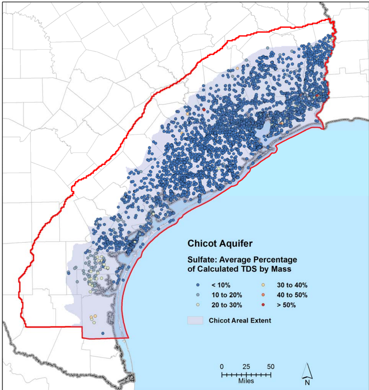
Figure 10-10. Sulfate percentage of average calculated total dissolved solids concentration by mass for the Chicot Aquifer.
