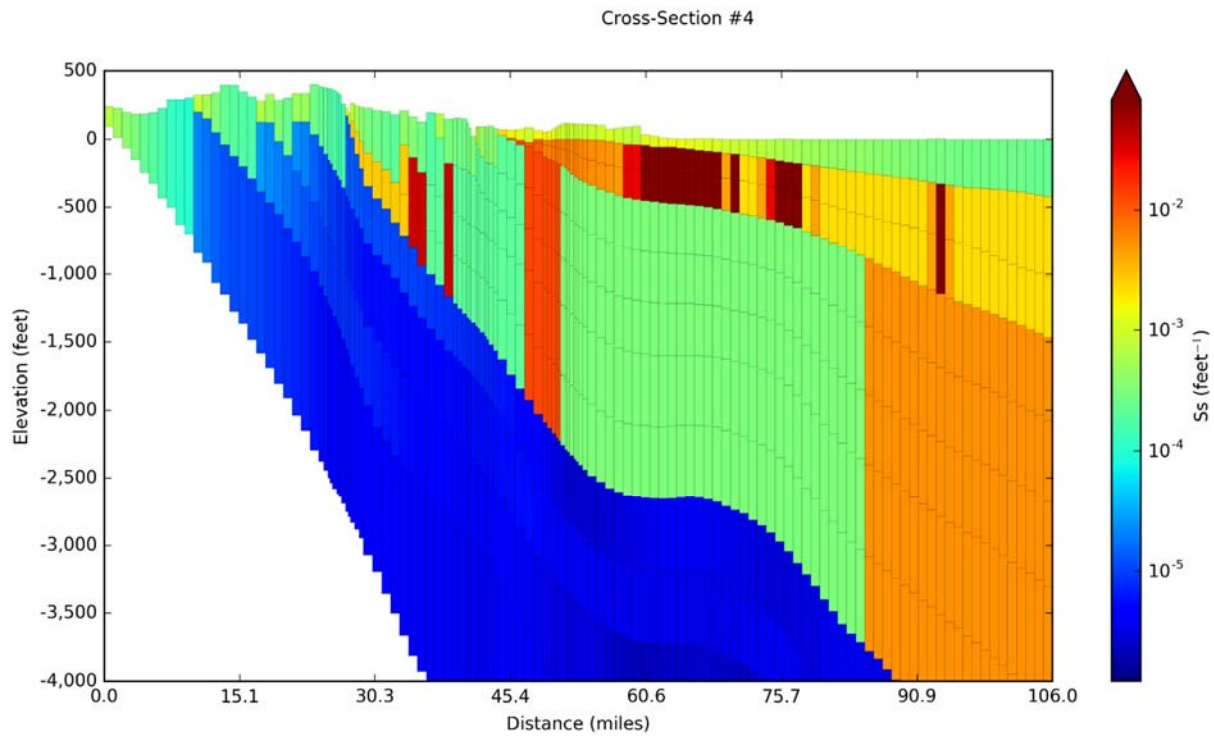
Figure 14-65. Specific storage (Ss) values in the groundwater model for Cross-Section #4 on Figure 14-5 for model layers 1 to 12.
