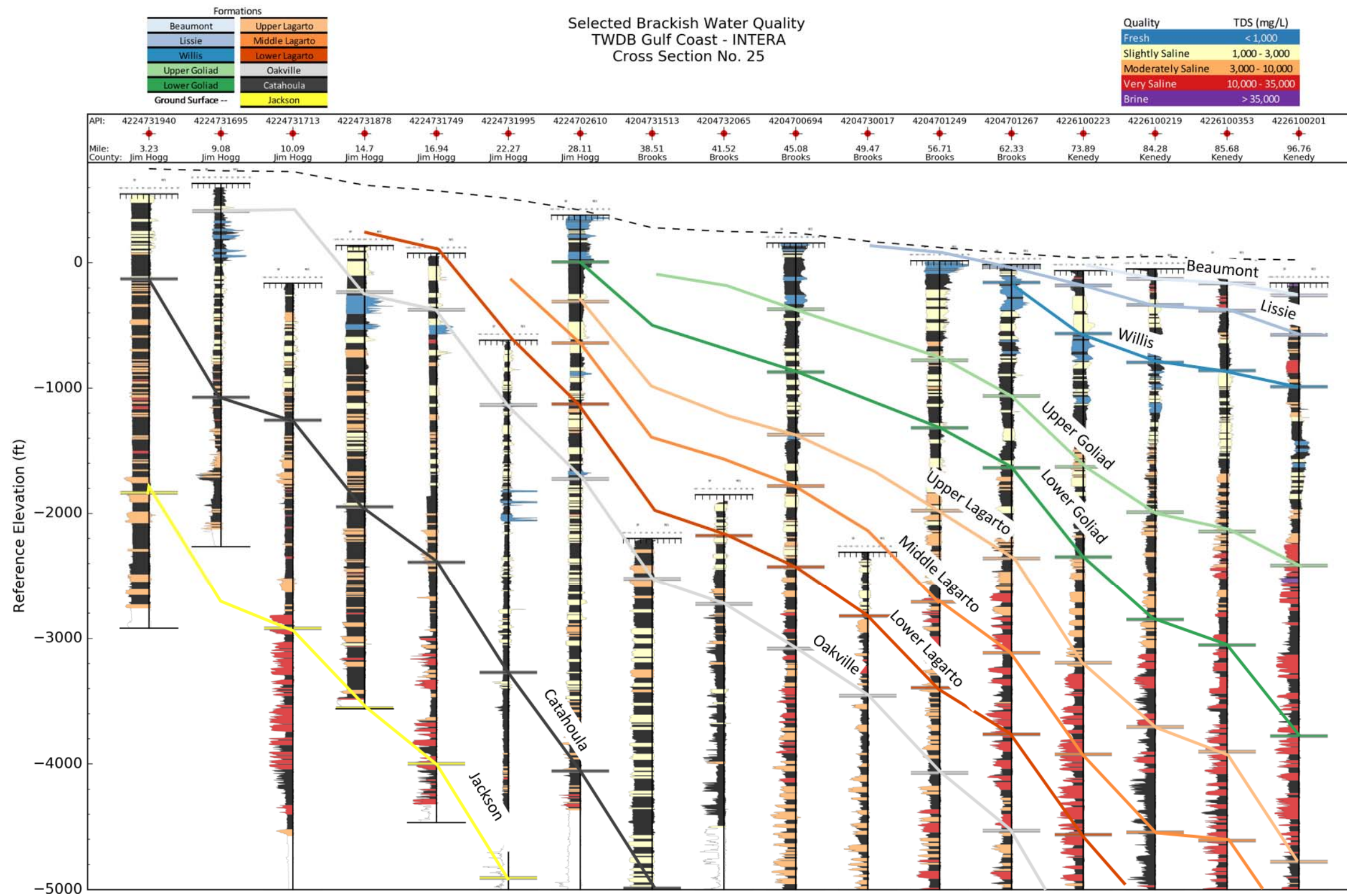
Figure 6-29. Profiles of calculated salinity zones for sand beds identified on geophysical logs aligned on Cross-Section #25 shown in Figure 6-1. Markers represent the base formations at each log location. The lines connecting the markers are for illustrative purposes only. Dashed line indicates crossing a log with no marker available in an active interval.
