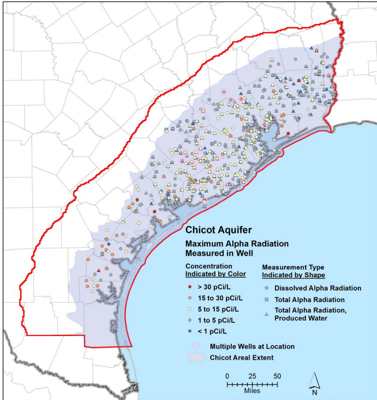
Figure 10-16. Maximum alpha radiation in the Chicot Aquifer.
