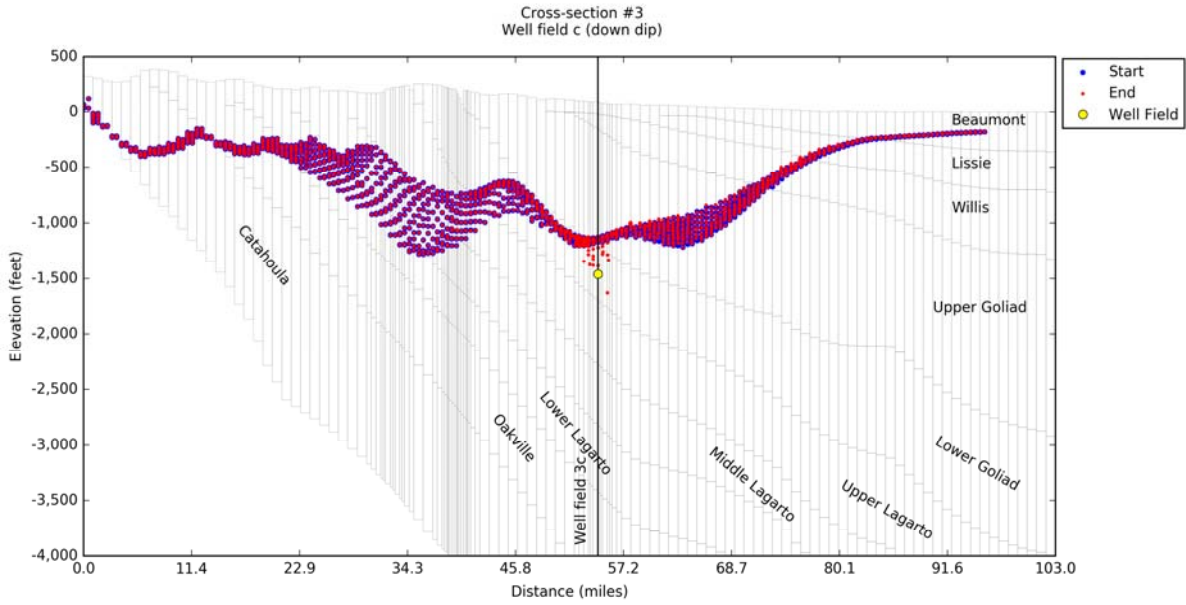
Figure 14-92. Simulated particle tracks 50 years after pumping the down dip Well Field #3c located along Cross-Section #3 on Figure 14-5 at 10,000 acre-feet per year.
