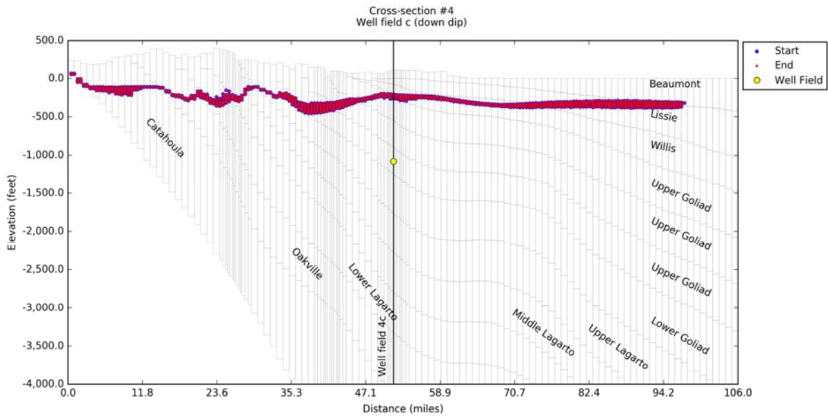
Figure 14-95. Simulated particle tracks 50 years after pumping the down dip Well Field #4c located along Cross-Section #4 on Figure 14-5 at 10,000 acre-feet per year.
