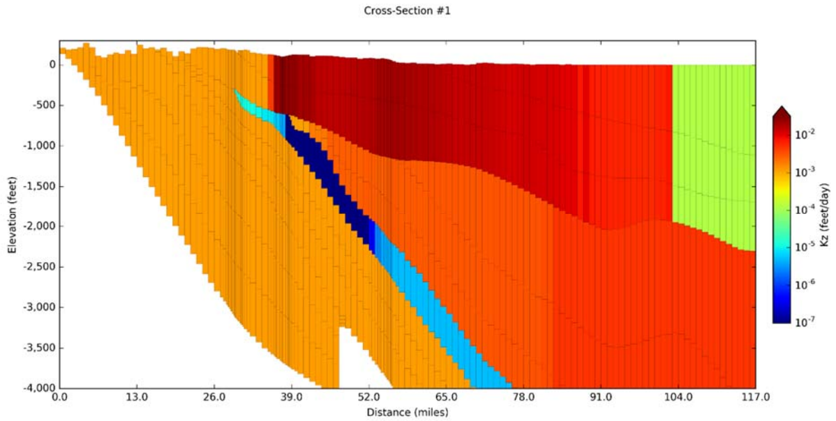
Figure 14-26. Vertical hydraulic conductivity ( K_z ) values for Cross-Section #1 on Figure 14-5 with aquifer properties from the Houston Area Groundwater Model (Kasmarek, 2012) for model layers 1 to 13.
