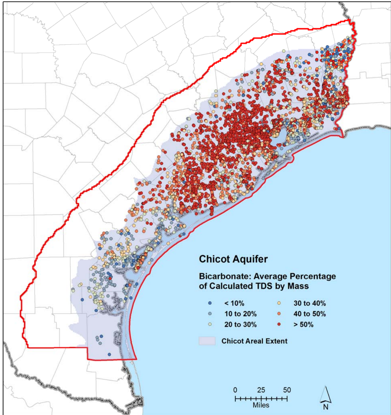
Figure 10-13. Bicarbonate percentage of average calculated total dissolved solids concentration by mass for the Chicot Aquifer.
