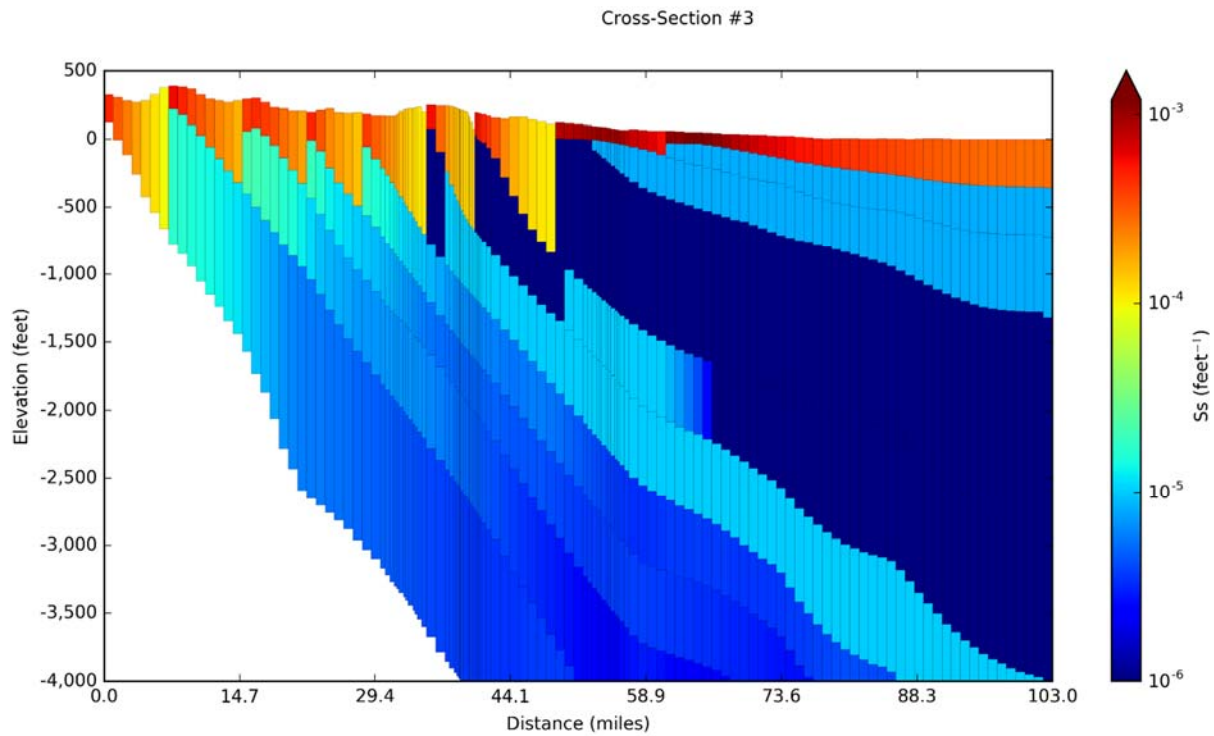
Figure 14-53. Specific storage (Ss) values in the groundwater model for Cross-Section #3 on Figure 14-5 for model layers 1 to 10.
