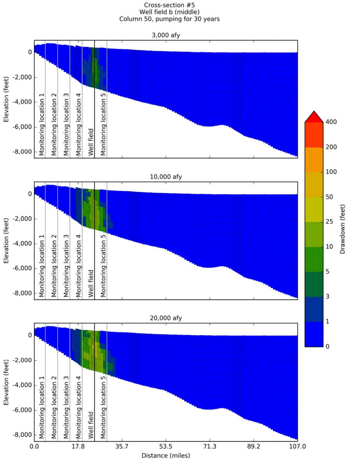
Figure 14-80. Simulated drawdown at 30 years after pumping the middle Well Field #5b located along Cross-Section #5 on Figure 14-5 at 3,000 acre-feet per year, 10,000 acre-feet per year, and 20,000 acre-feet per year.
