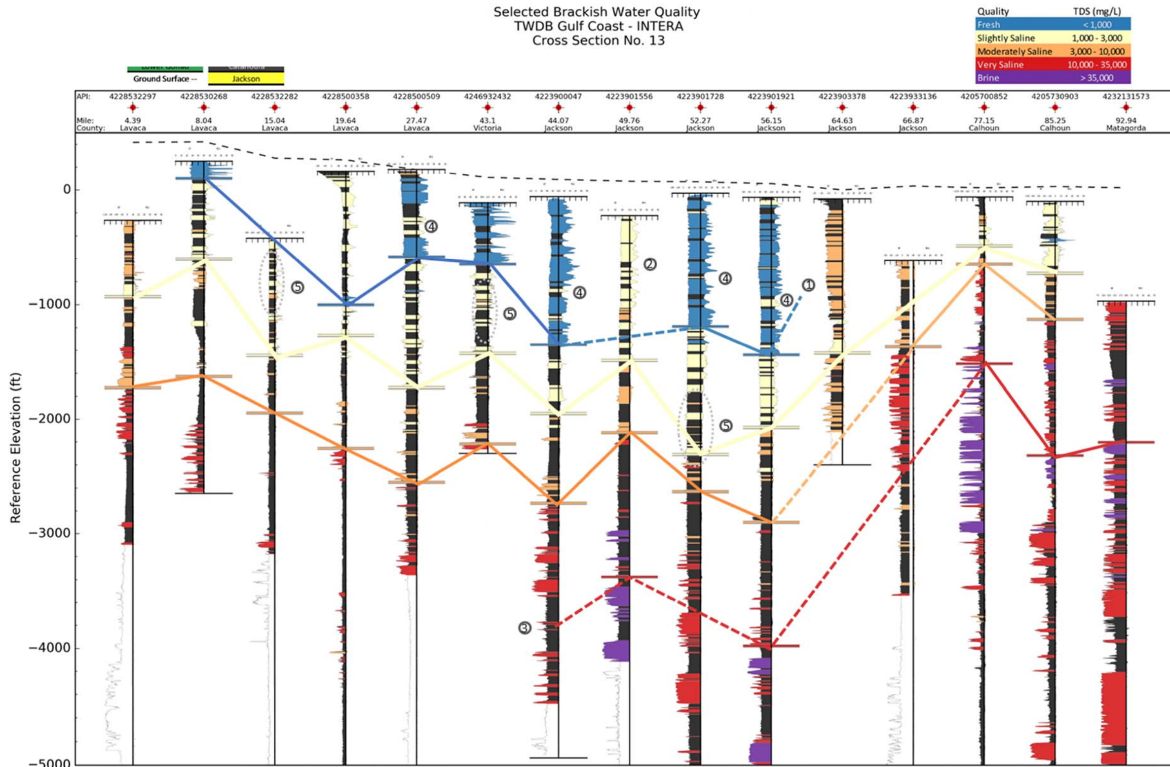
Figure 6-20. Profiles of calculated salinity zones for sand beds identified on geophysical logs aligned on Cross-Section #13 shown in Figure 6-1. Markers represent the base of the salinity zones at each log location. The lines connecting the markers are for illustrative purposes only. Dashed line indicates crossing a log with no marker available in an active interval.
