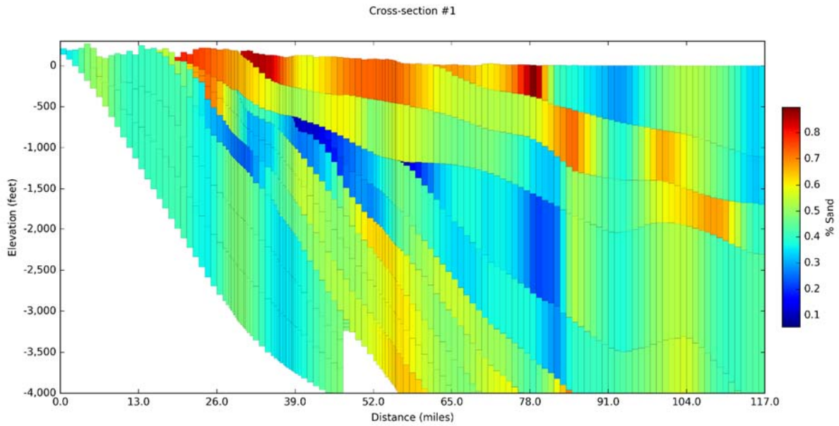
Figure 14-16. Sand fraction for model layers 1 to 13 for a vertical cross-section cut through the three-dimensional model for Cross-Section #1 on Figure 14-5.
