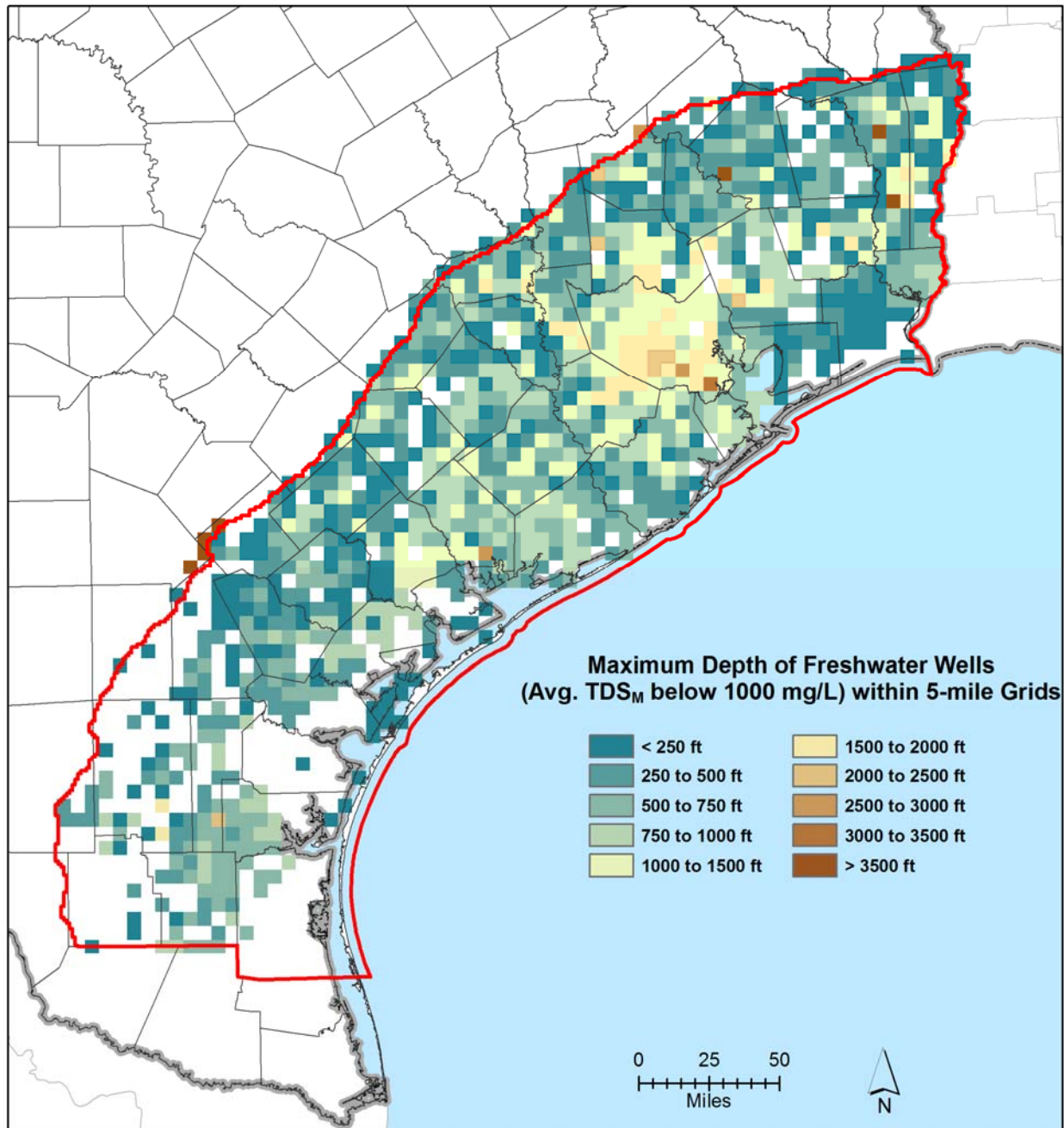
Figure 6-9. Maximum depth of fresh water sampled by wells located in a grid of 5-mile by 5-mile blocks based on information from the TWDB groundwater database.
