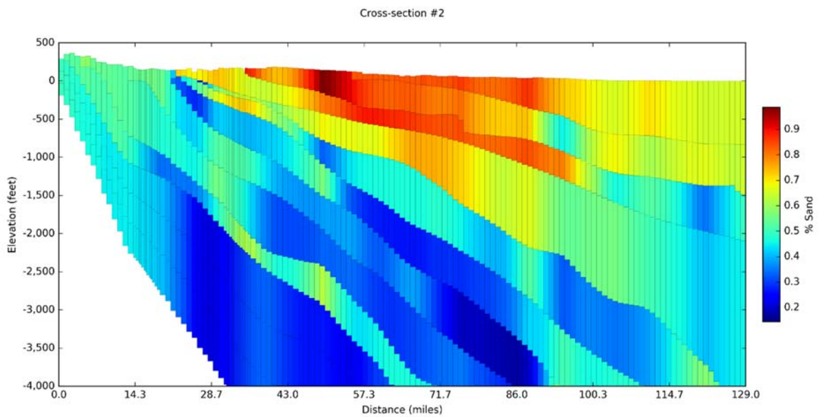
Figure 14-17. Sand fraction for model layers 1 to 12 for a vertical cross-section cut through the three-dimensional model for Cross-Section #2 on Figure 14-5.
