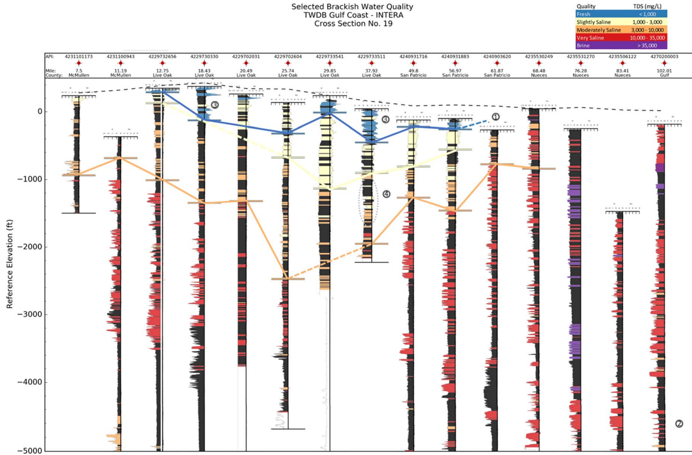
Figure 6-24. Profiles of calculated salinity zones for sand beds identified on geophysical logs aligned on Cross-Section #19 shown in Figure 6-1. Markers represent the base of the salinity zones at each log location. The lines connecting the markers are for illustrative purposes only. Dashed line indicates crossing a log with no marker available in an active interval.
