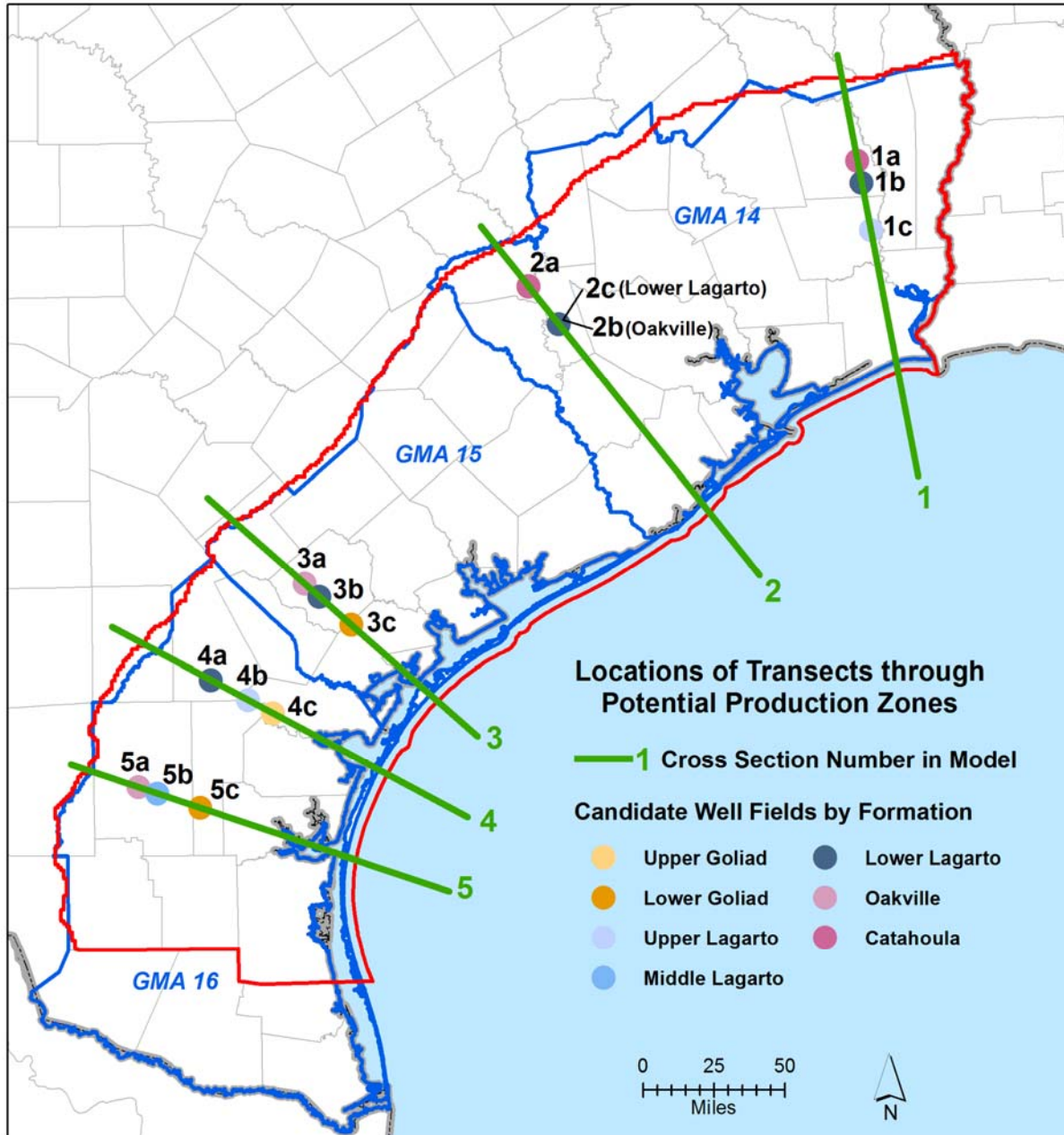
Figure 14-5. Location of five vertical cross-sections used to develop five groundwater models.
