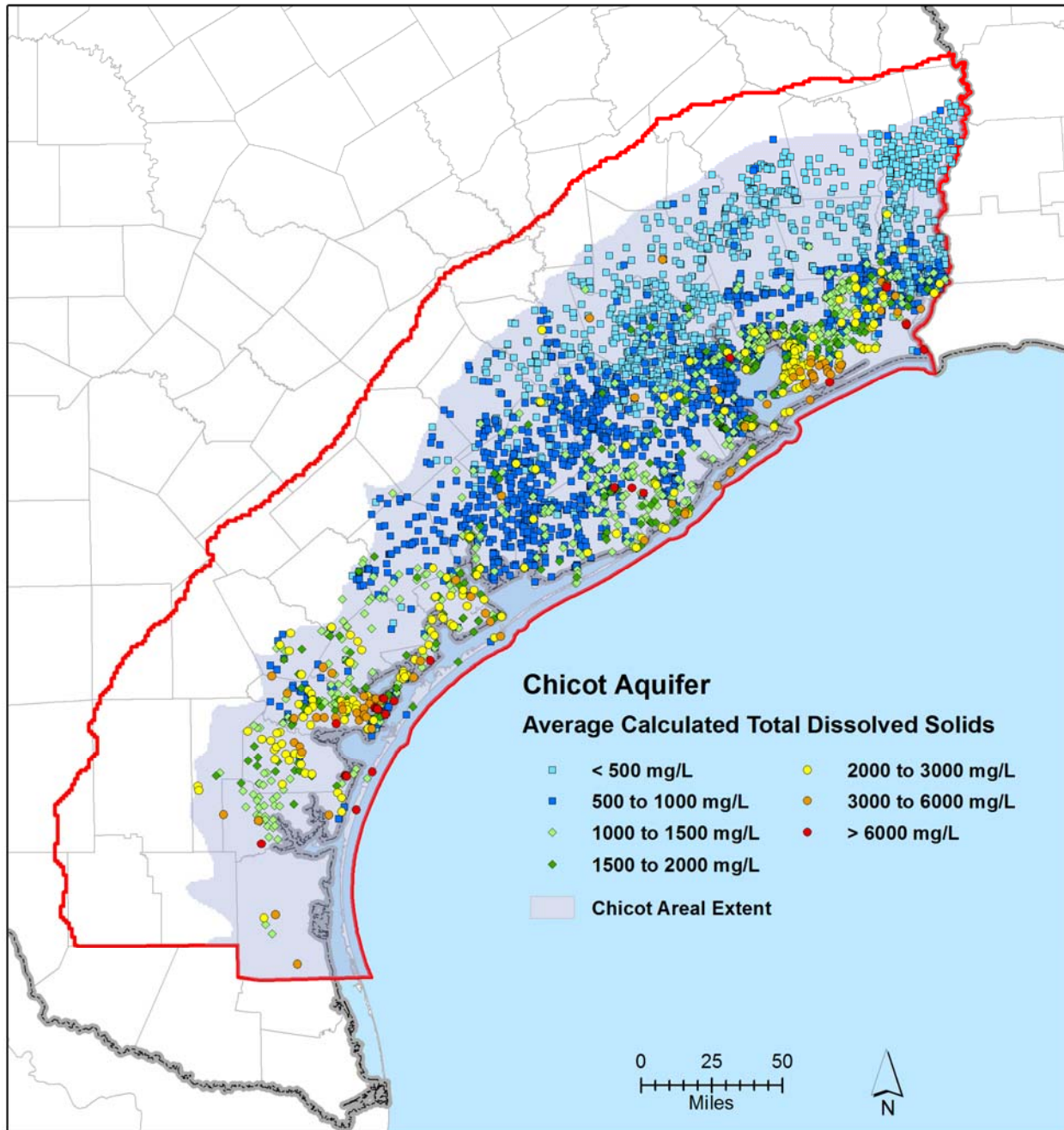
Figure 10-2. Average calculated total dissolved solids concentration in the Chicot Aquifer.
