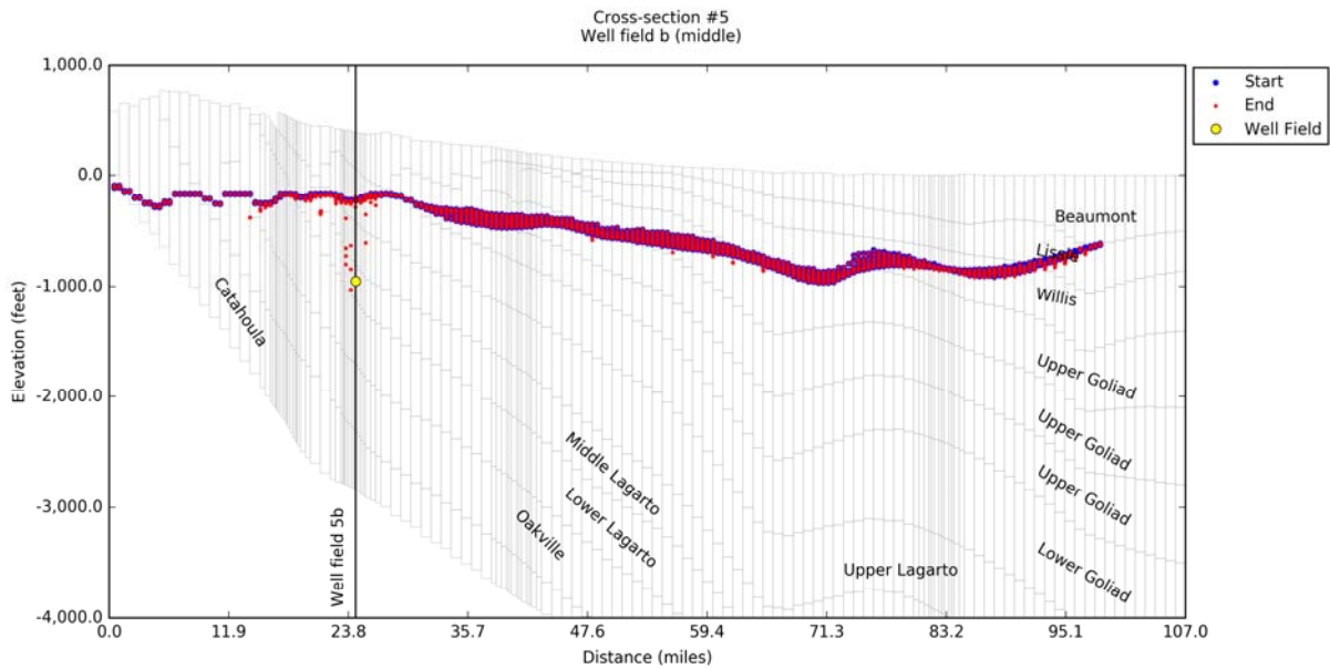
Figure 14-97. Simulated particle tracks 50 years after pumping the middle Well Field #5b located along Cross-Section #5 on Figure 14-5 at 10,000 acre-feet per year.
