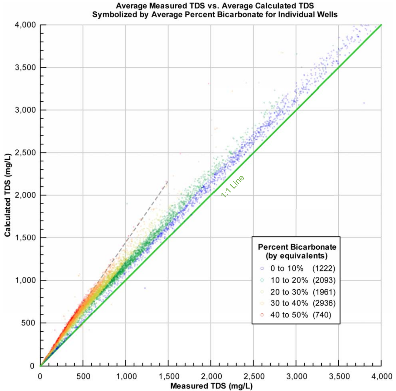
Figure 13-2. Calculated total dissolved solids concentration versus measured total dissolved solids concentration for groundwater samples from the Texas Gulf Coast Aquifer System grouped into class intervals based on their equivalents of bicarbonate.
