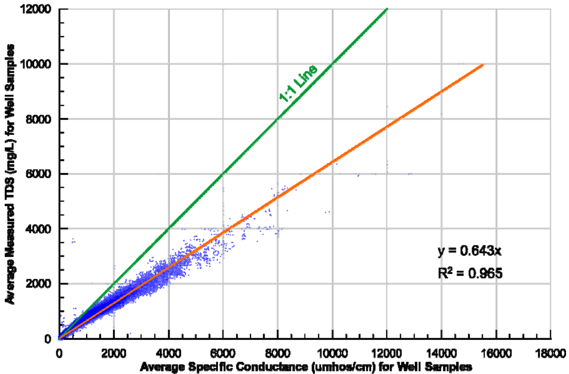
Figure 13-9. Linear regression between specific conductance and total dissolved solids concentration for 16,959 groundwater samples where (a) total dissolved solids concentration is measured and (b) total dissolved solids concentration is calculated.
