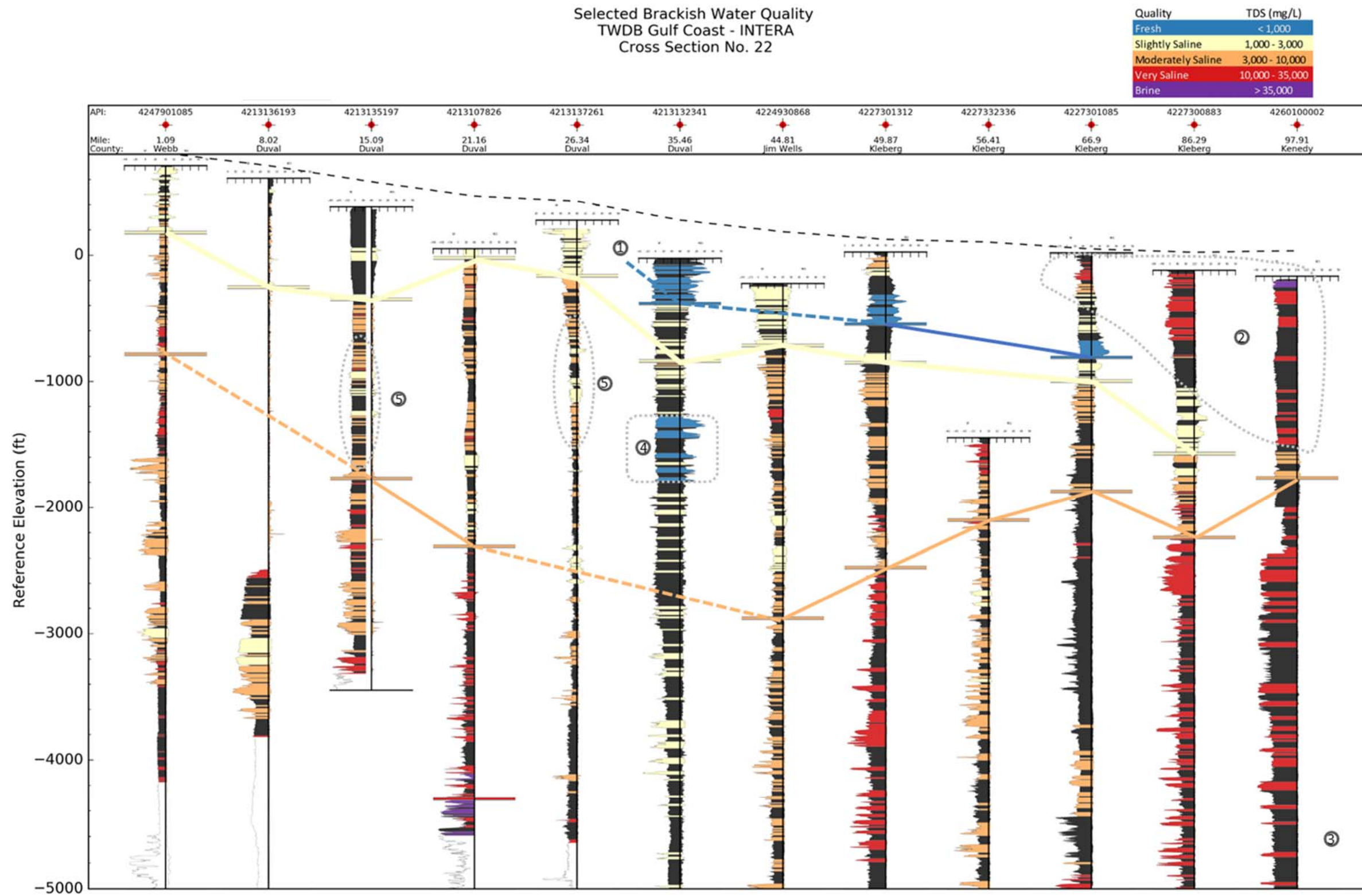
Figure 6-26. Profiles of calculated salinity zones for sand beds identified on geophysical logs aligned on Cross-Section #22 shown in Figure 6-1. Markers represent the base of the salinity zones at each log location. The lines connecting the markers are for illustrative purposes only. Dashed line indicates crossing a log with no marker available in an active interval.
