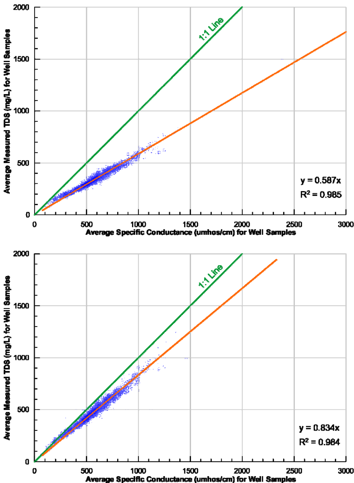
Figure 13-7. Linear regression between specific conductance and total dissolved solids concentration for 1,866 groundwater samples where bicarbonate comprises at least 35 percent of the equivalence in the charge balance where (a) total dissolved solids concentration is measured and (b) total dissolved solids concentration is calculated.
