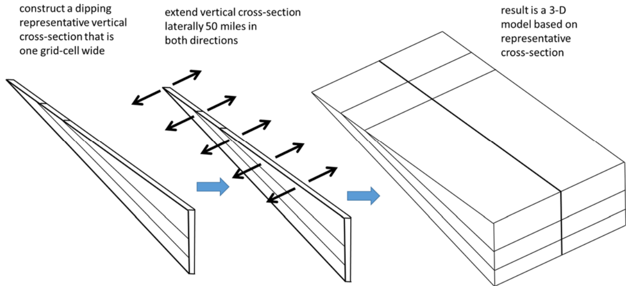
Figure 14-7. Schematic showing the lateral outward replication of a vertical cross-section, which is one grid-cell wide, to construct a three-dimensional model that covers a distance of 50 miles on both sides of the original cross-section.
