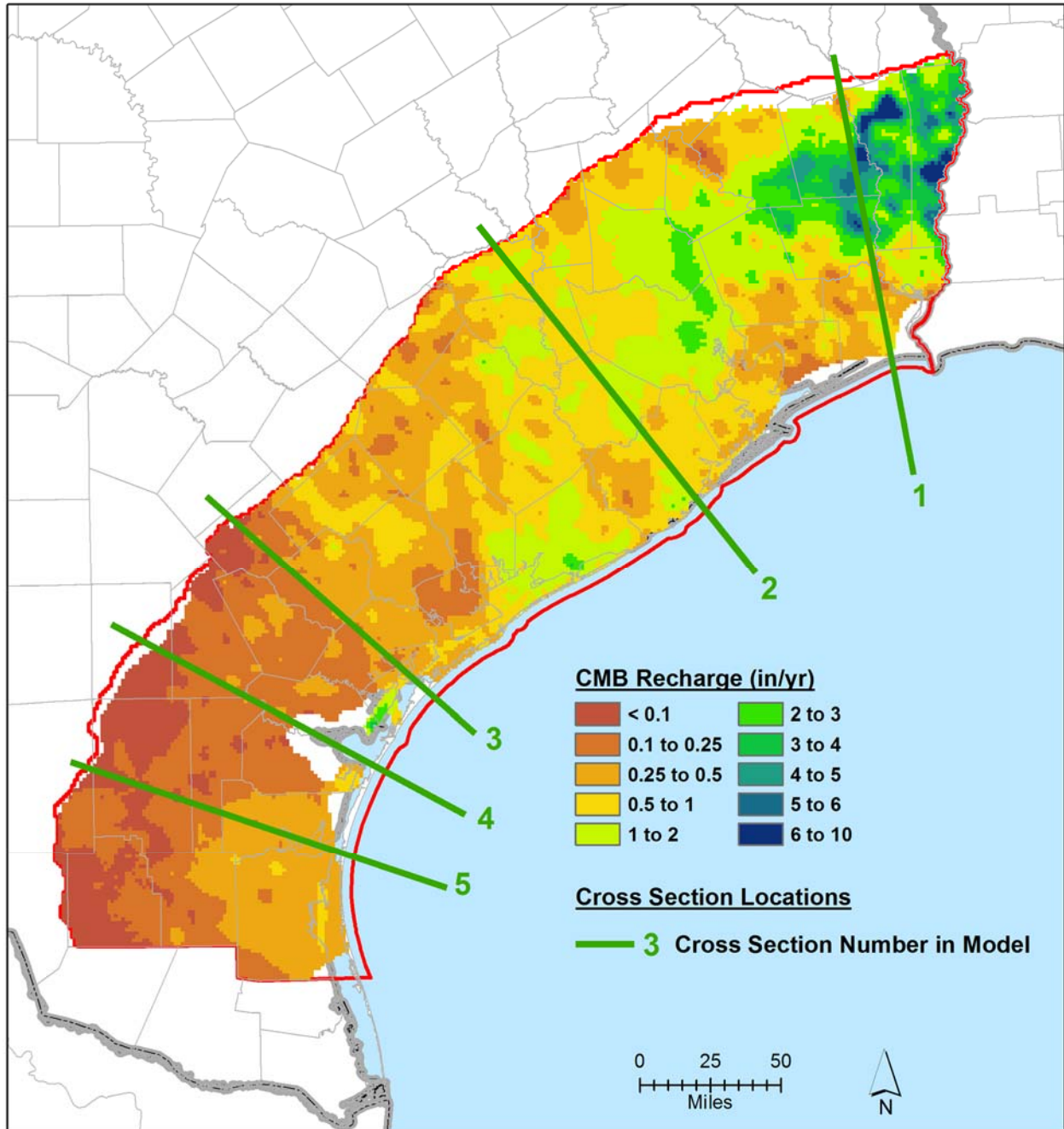
Figure 14-6. Recharge rates used in the groundwater models (from Scanlon and others, 2012).
