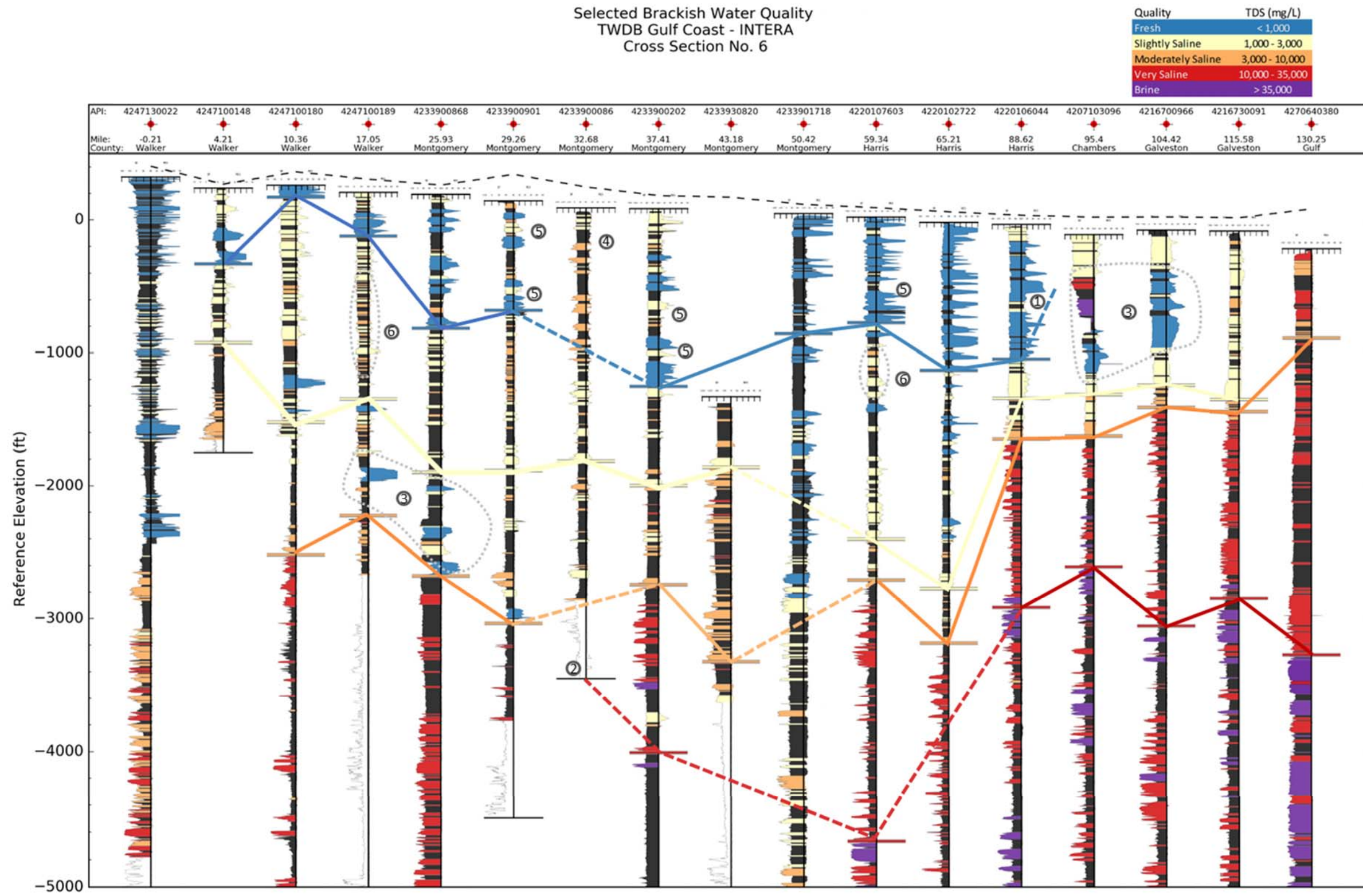
Figure 6-14. Profiles of calculated salinity zones for sand beds identified on geophysical logs aligned on Cross-Section #6 shown in Figure 6-1. Markers represent the base of the salinity zones at each log location. The lines connecting the markers are for illustrative purposes only. Dashed line indicates crossing a log with no marker available in an active interval.
