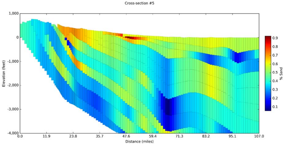
Figure 14-20. Sand fraction for model layers 1 to 12 for a vertical cross-section cut through the three-dimensional model for Cross-Section #5 on Figure 14-5.
