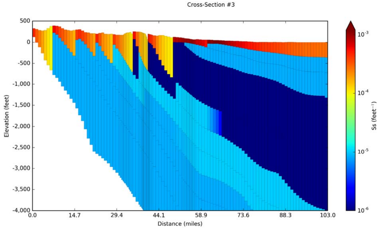
Figure 14-52. Specific storage (Ss) values for Cross-Section #3 on Figure 14-5 with aquifer properties from the Central Gulf Coast Groundwater Availability Model (Chowdhury and others, 2004) for model layers 1 to 10.
