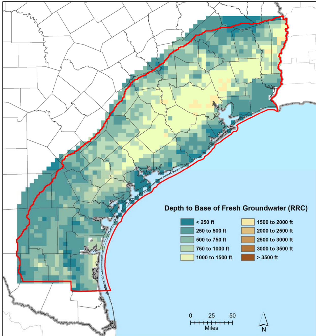
Figure 6-10. Estimated depth to base of fresh water, which is defined as a total dissolved solid concentration of 1,000 milligrams per liter, based on 23,000 picks of depth to freshwater from a database maintained by the Groundwater Advisory Unit of the Railroad Commission of Texas.
