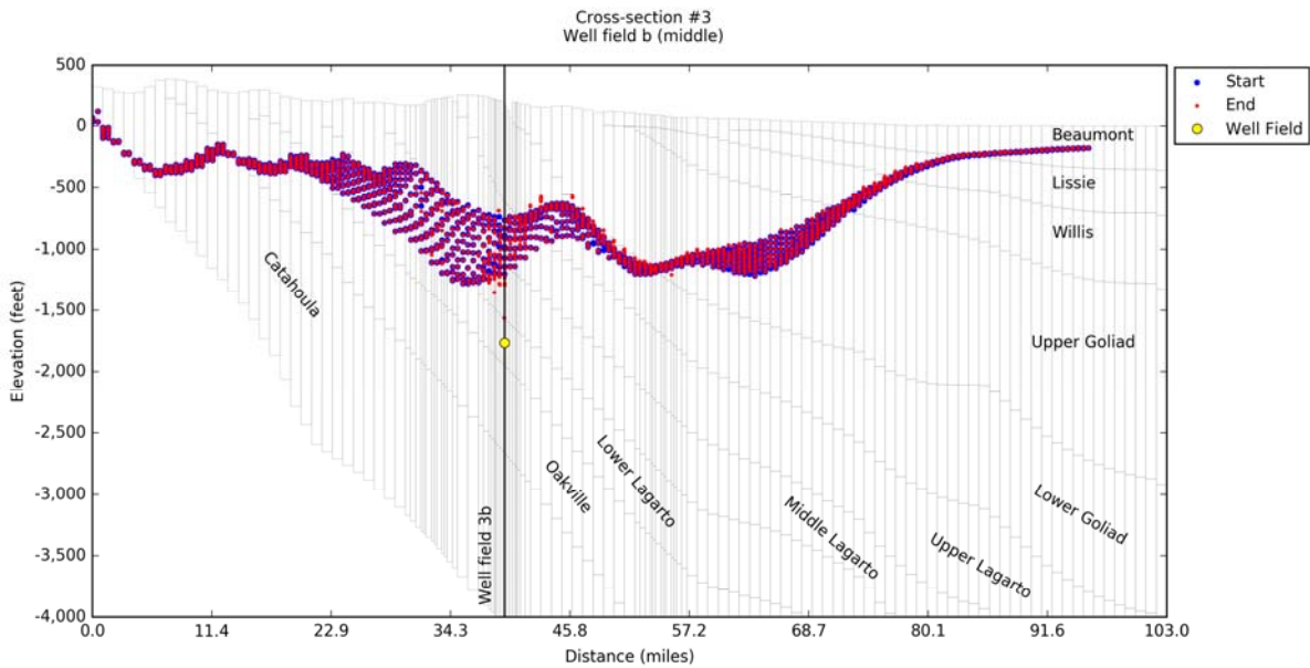
Figure 14-91. Simulated particle tracks 50 years after pumping the middle Well Field #3b located along Cross-Section #3 on Figure 14-5 at 10,000 acre-feet per year.
