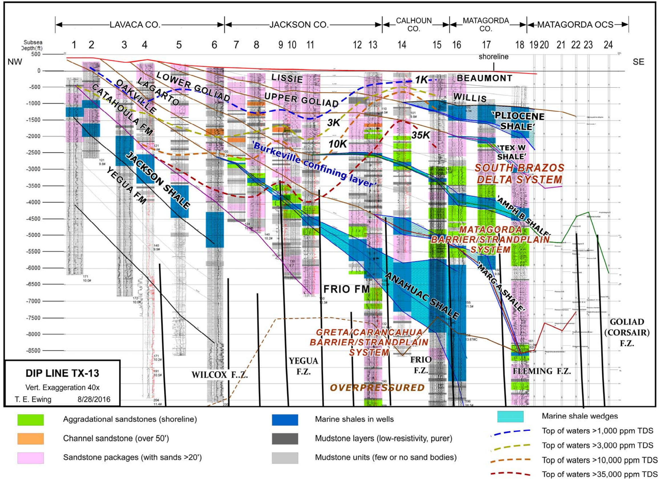
Figure 11-12. Analysis of sand and clay sequences, fault zones, along Cross-Section #13 in Figure 6-1.
