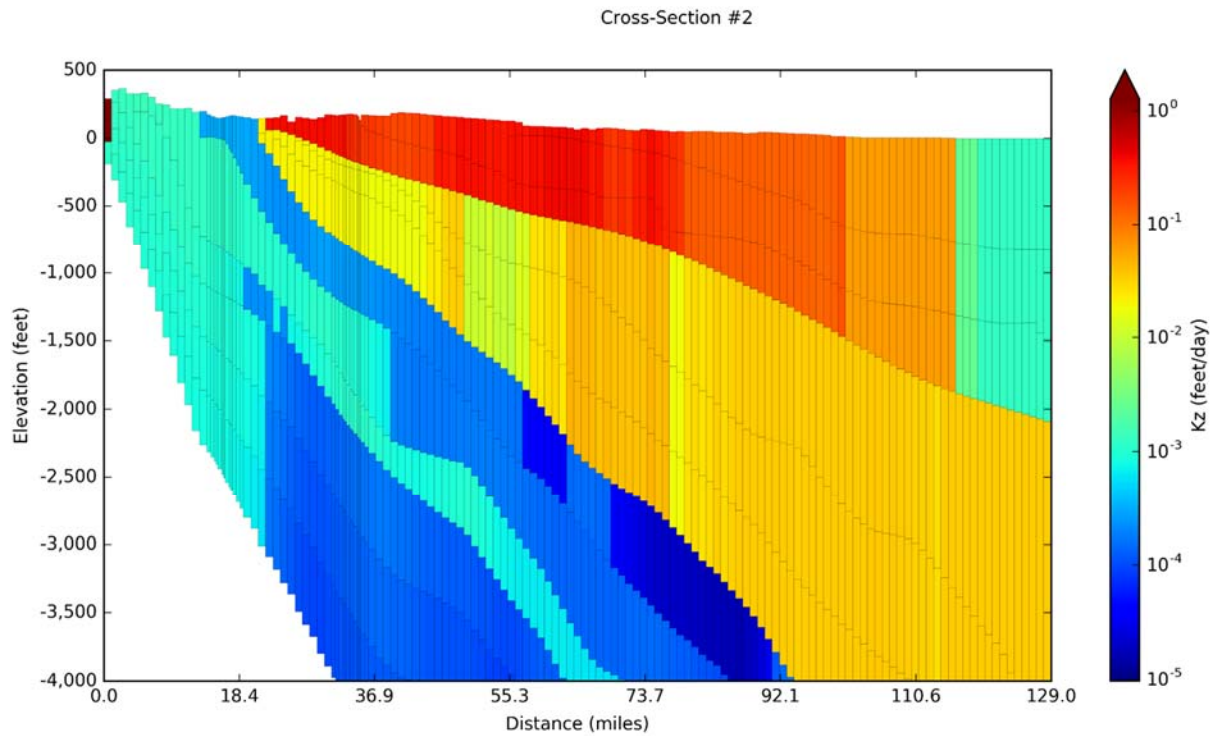
Figure 14-39. Vertical hydraulic conductivity ( K_z ) values in the groundwater model for Cross-Section #2 on Figure 14-5 for model layers 1 to 12.
