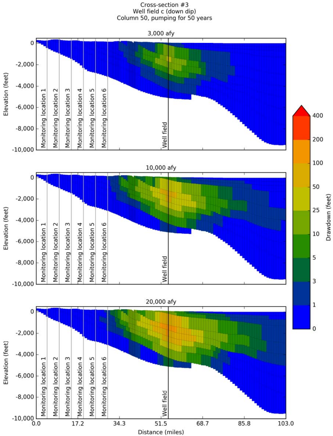
Figure 14-59. Simulated drawdown at 50 years after pumping the down dip Well Field #3c located along Cross-Section #3 on Figure 14-5 at 3,000 acre-feet per year, 10,000 acre-feet per year, and 20,000 acre-feet per year.
