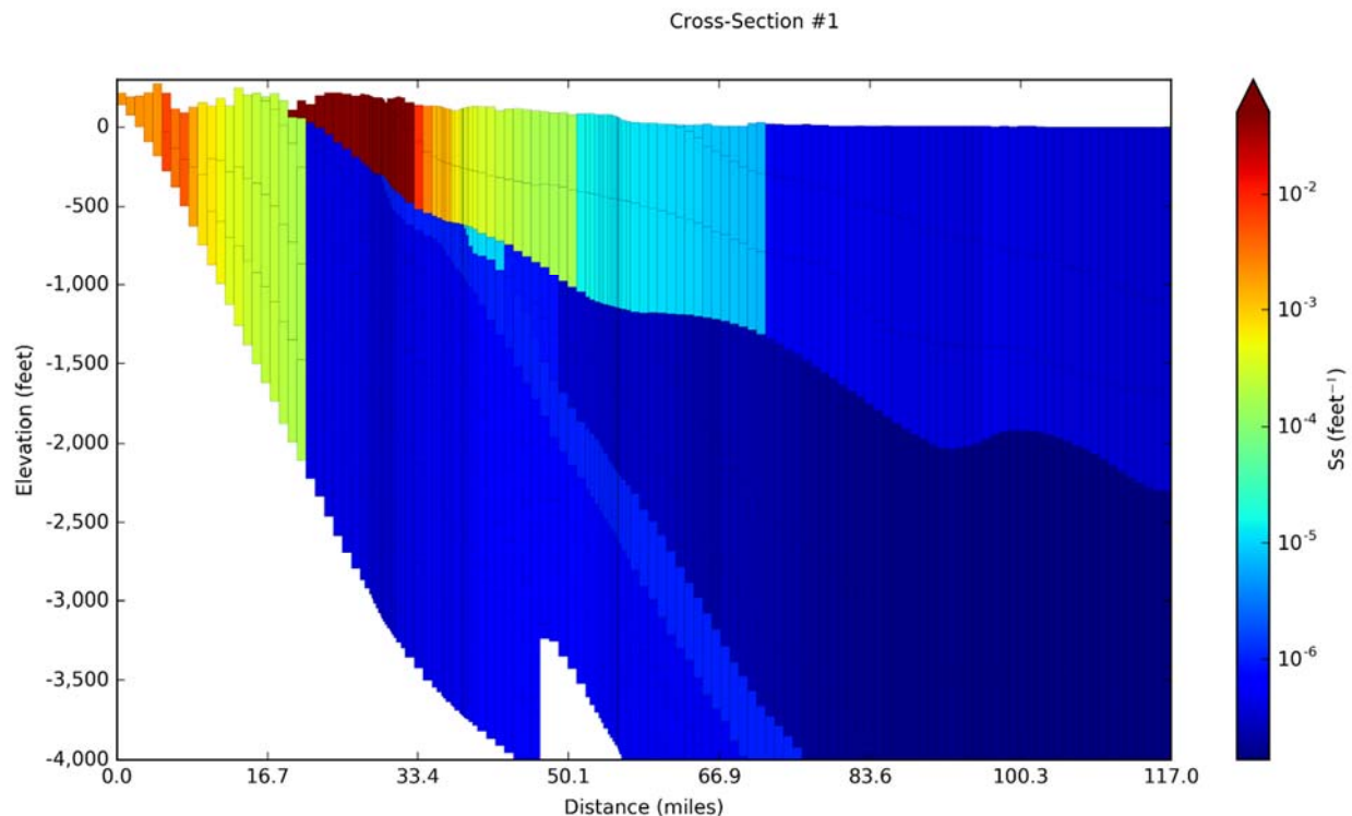
Figure 14-28. Specific storage (Ss) values for Cross-Section #1 on Figure 14-5 with aquifer properties from the Houston Area Groundwater Model (Kasmarek, 2012) for model layers 1 to 13.
