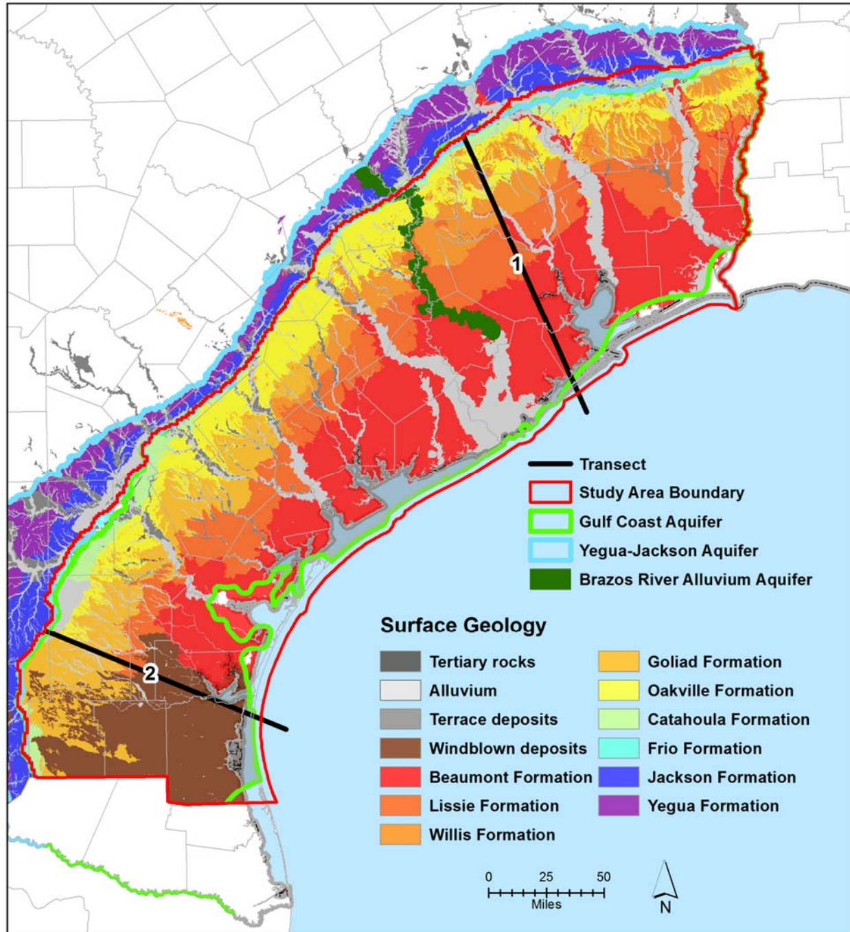
Figure 5-2. Map of the Texas Gulf Coast showing the surface geology and the outcrops of the Gulf Coast Aquifer System, Yegua-Jackson and Brazos River Alluvium aquifers.
