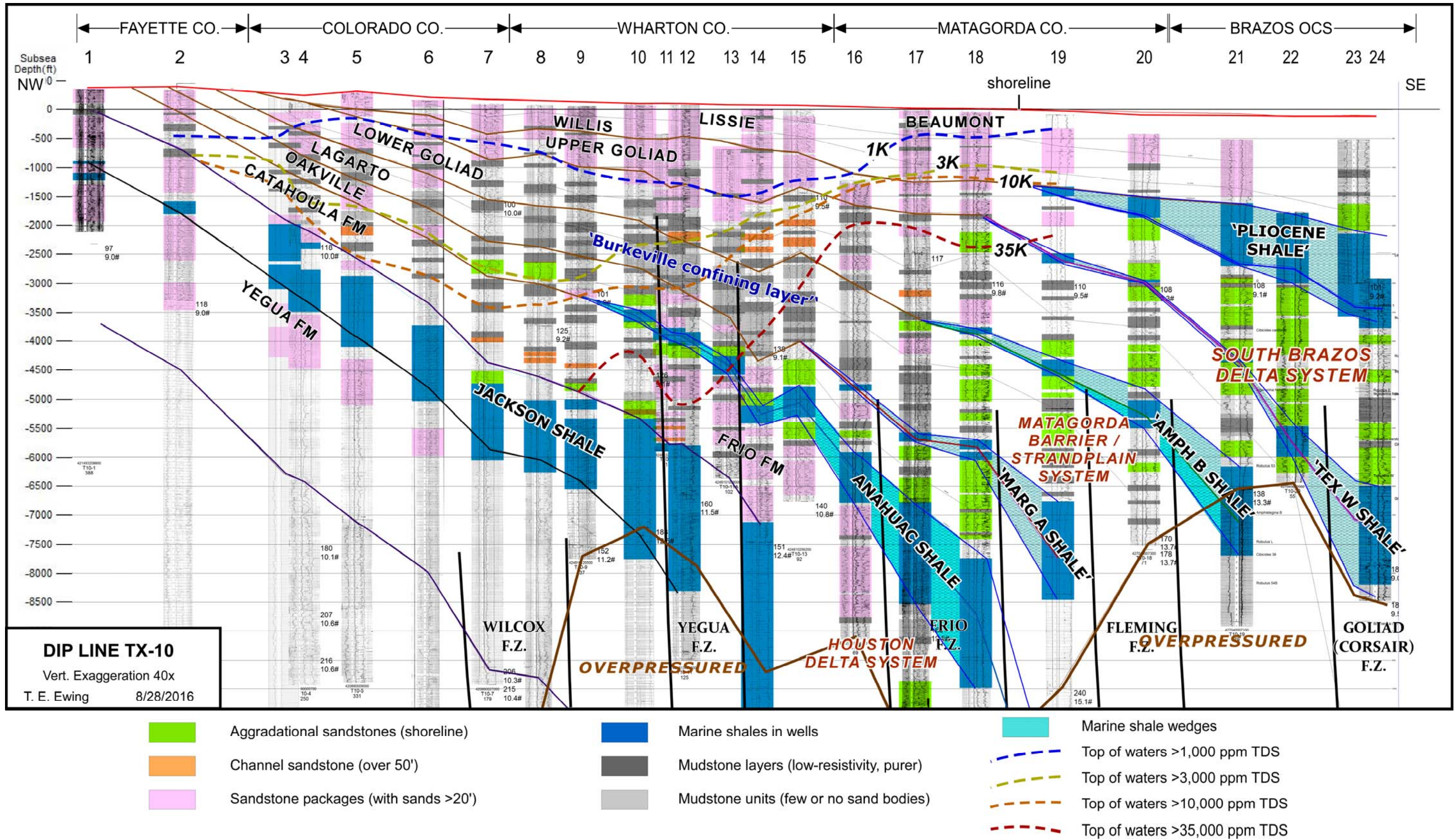
Figure 11-11. Analysis of sand and clay sequences, fault zones, along Cross-Section #10 in Figure 6-1.
