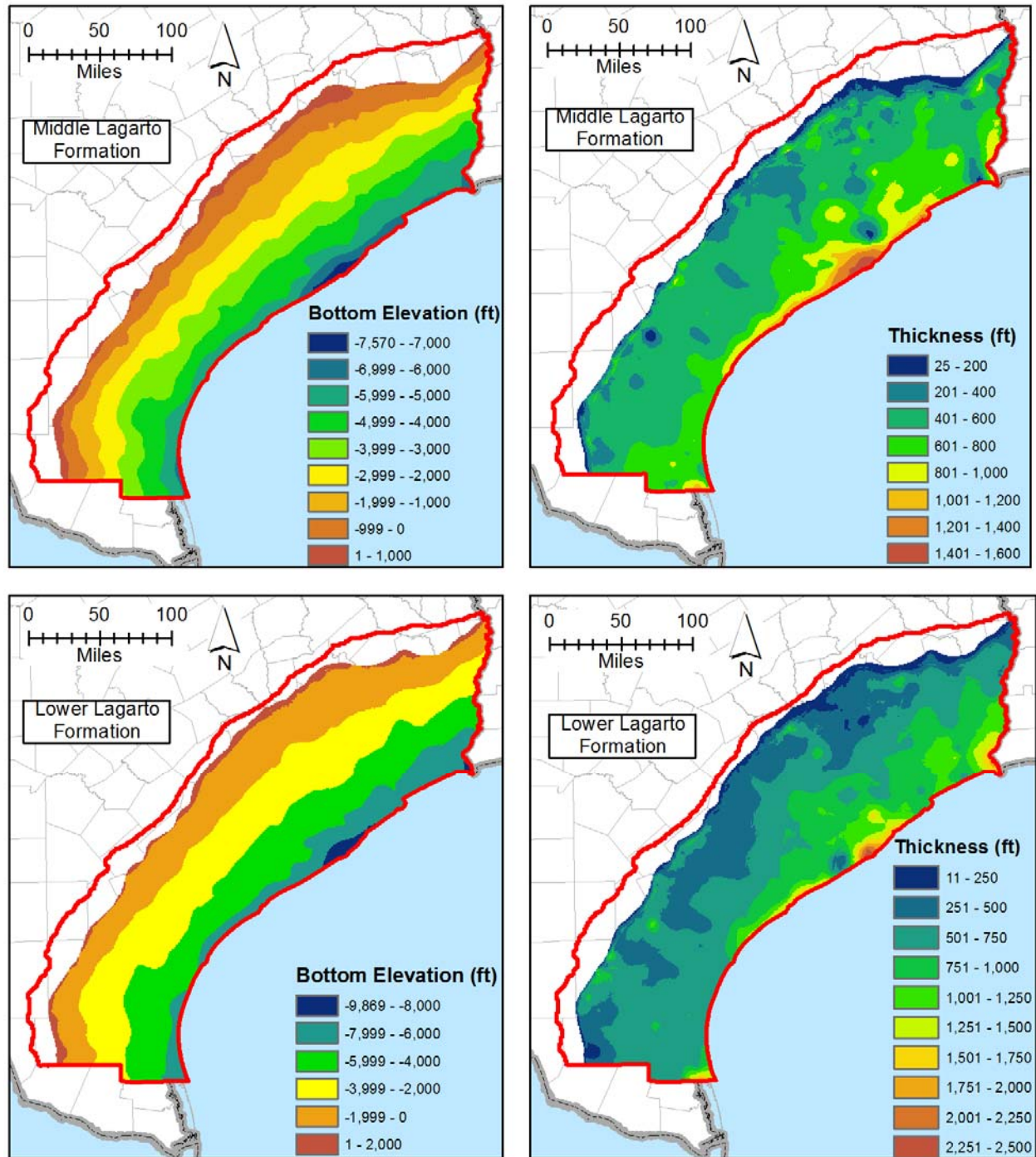
Figure 7-4. Bottom elevation and thickness for the Middle Lagarto and Lower Lagarto formations based on the data from Young and others (2010, 2012).
