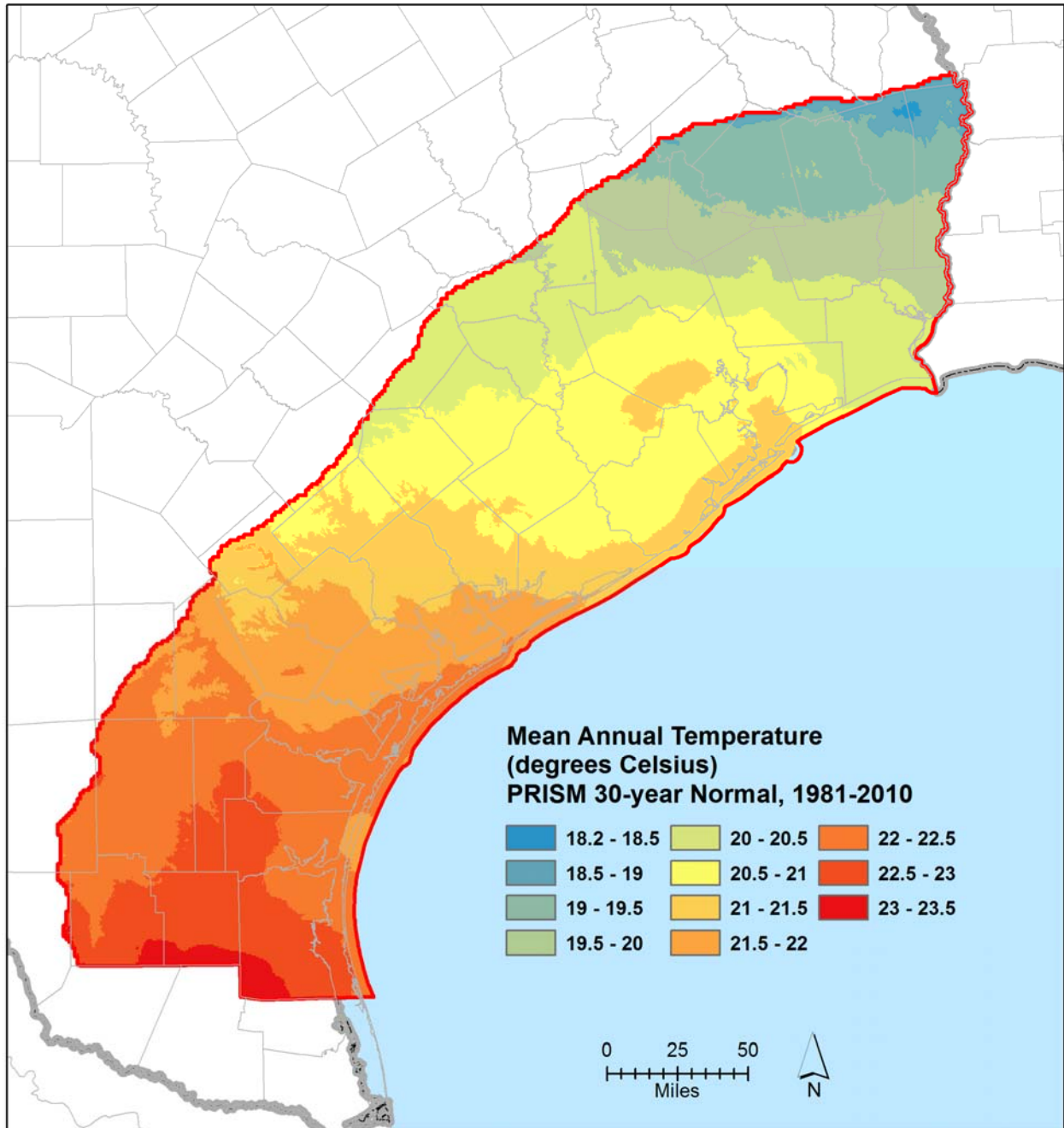
Figure 7-7. Average annual temperature based on a 30-year period from 1981 to 2010 (PRISM Climate Group, 2013).
