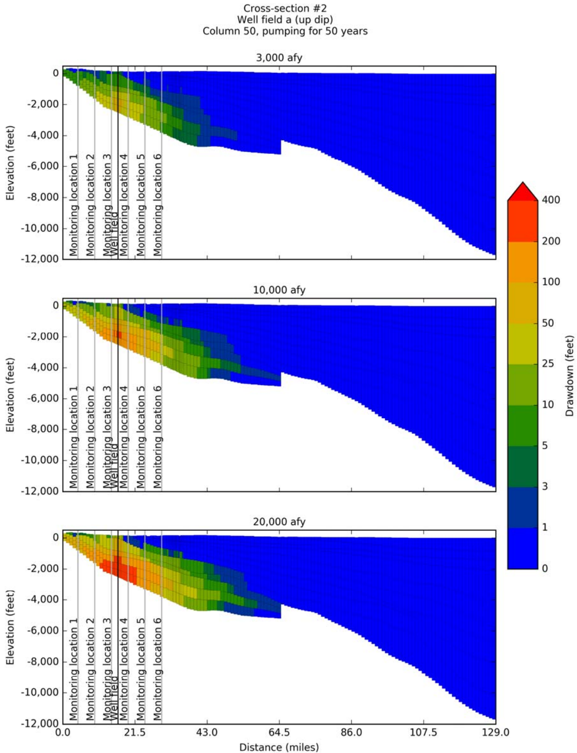
Figure 14-43. Simulated drawdown at 50 years after pumping the up dip Well Field #2a located along Cross-Section #2 on Figure 14-5 at 3,000 acre-feet per year, 10,000 acre-feet per year, and 20,000 acre-feet per year.
