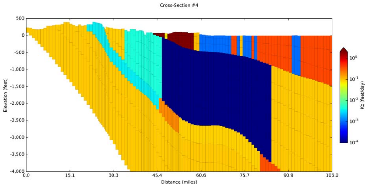
Figure 14-62. Vertical hydraulic conductivity ( K_z ) values for Cross-Section #4 on Figure 14-5 with aquifer properties from the Groundwater Management Area 16 Alternate Groundwater Availability Model (Hutchison and others, 2011) for model layers 1 to 12.
