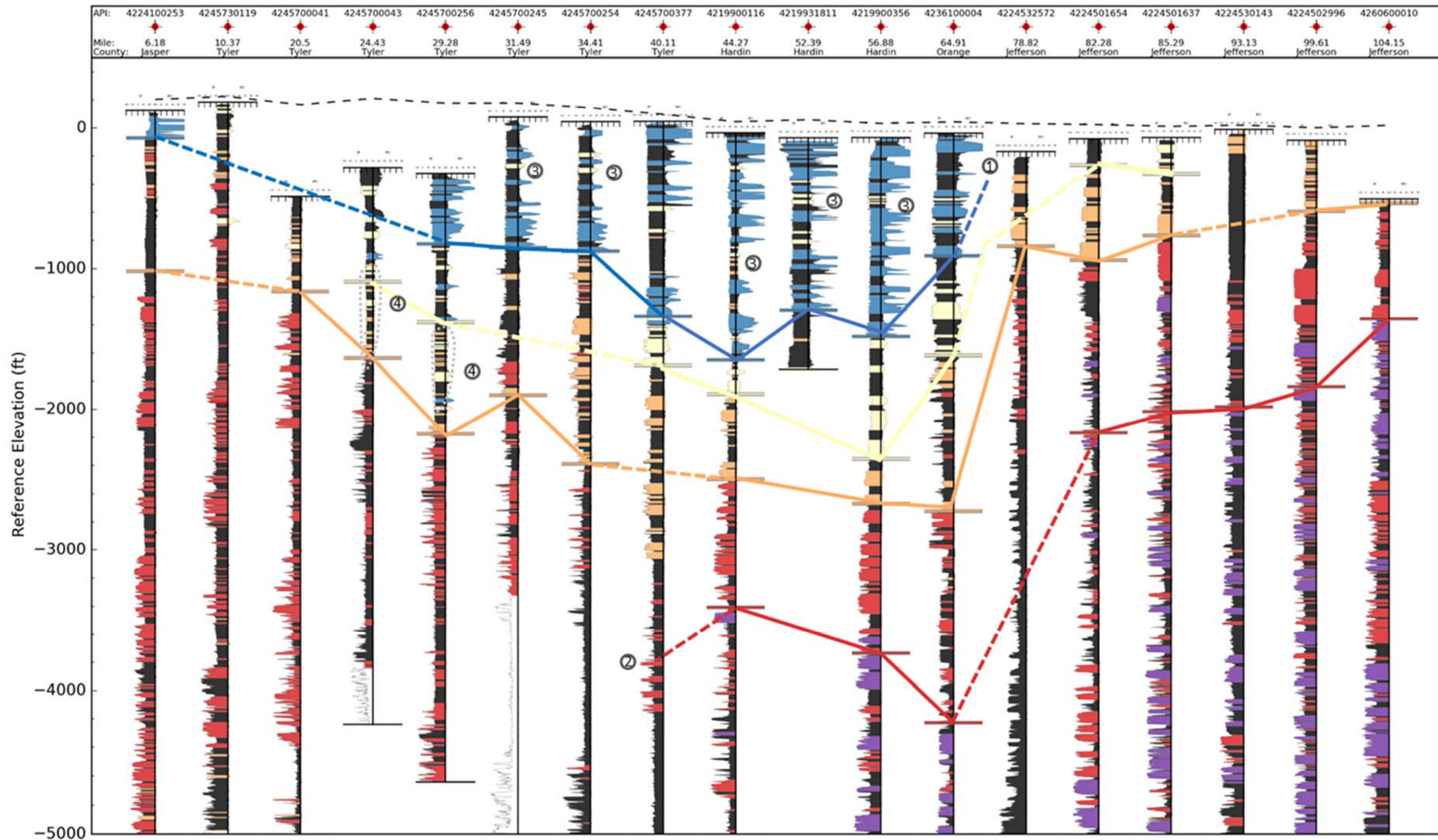
Figure 6-12. Profiles of calculated salinity zones for sand beds identified on geophysical logs aligned on Cross-Section #2 shown in Figure 6-1. Markers represent the base of the salinity zones at each log location. The lines connecting the markers are for illustrative purposes only. Dashed line indicates crossing a log with no marker available in an active interval.
