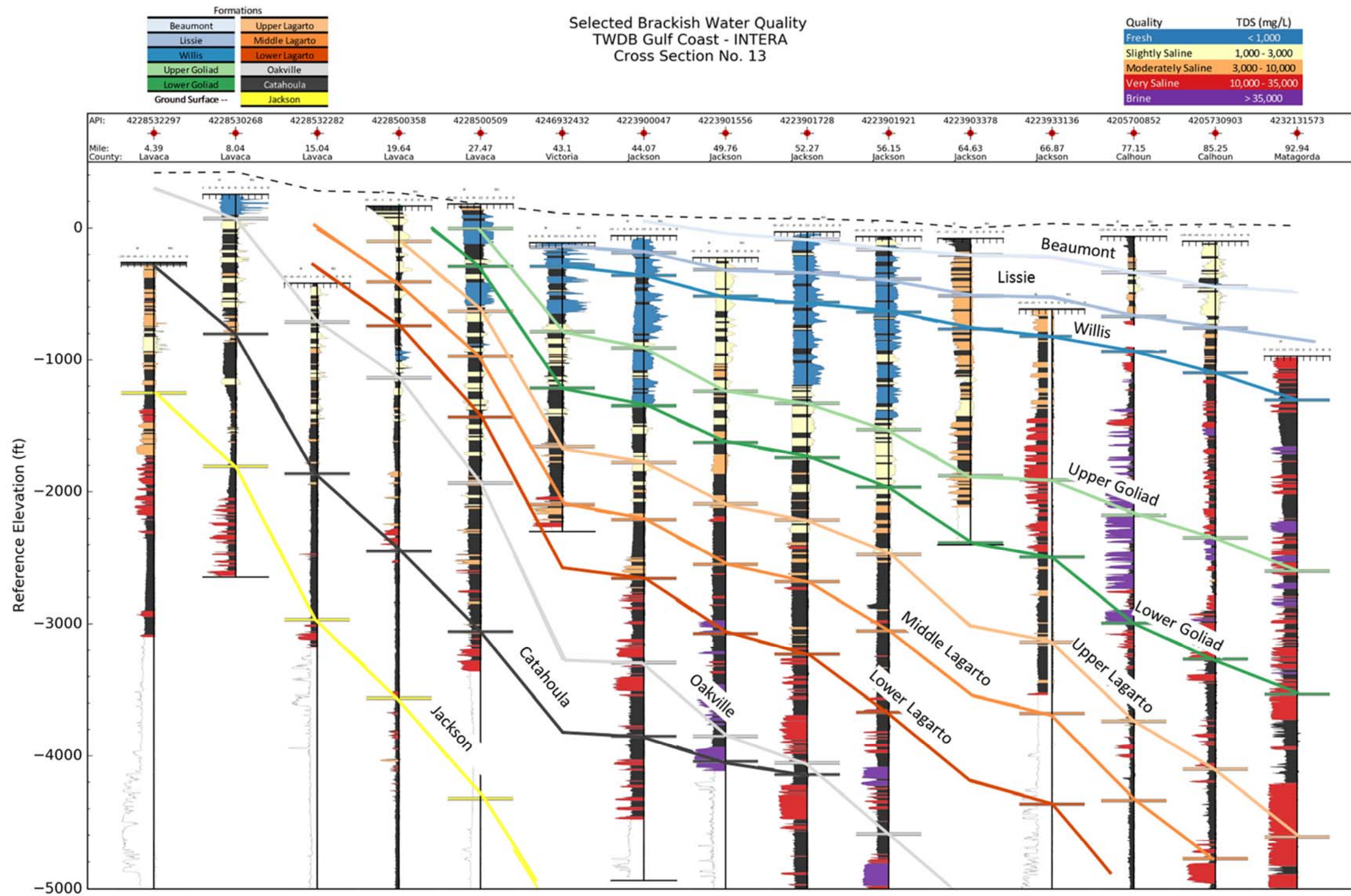
Figure 6-21. Profiles of calculated salinity zones for sand beds identified on geophysical logs aligned on Cross-Section #13 shown in Figure 6-1. Markers represent the base formations at each log location. The lines connecting the markers are for illustrative purposes only. Dashed line indicates crossing a log with no marker available in an active interval.
