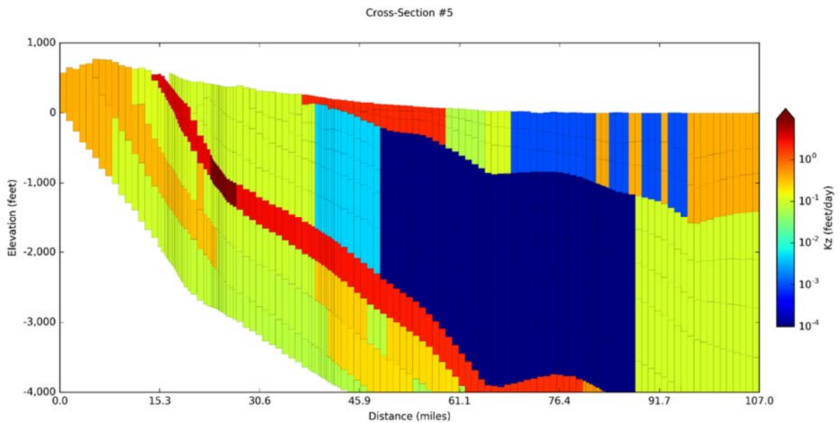
Figure 14-75. Vertical hydraulic conductivity ( K_z ) values in the groundwater model for Cross-Section #5 on Figure 14-5 for model layers 1 to 12.
