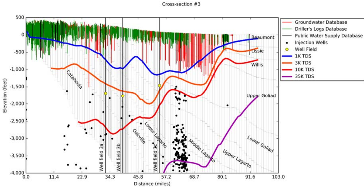
Figure 14-13. Boundaries for fresh water, slightly saline, moderately saline, and very saline groundwater along Cross-Section #3 on Figure 14-5.
