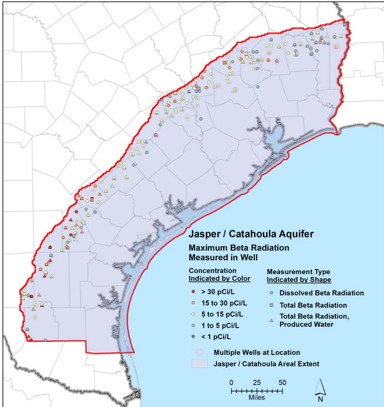
Figure 10-21. Maximum beta radiation in the Jasper Aquifer and Catahoula Formation.
