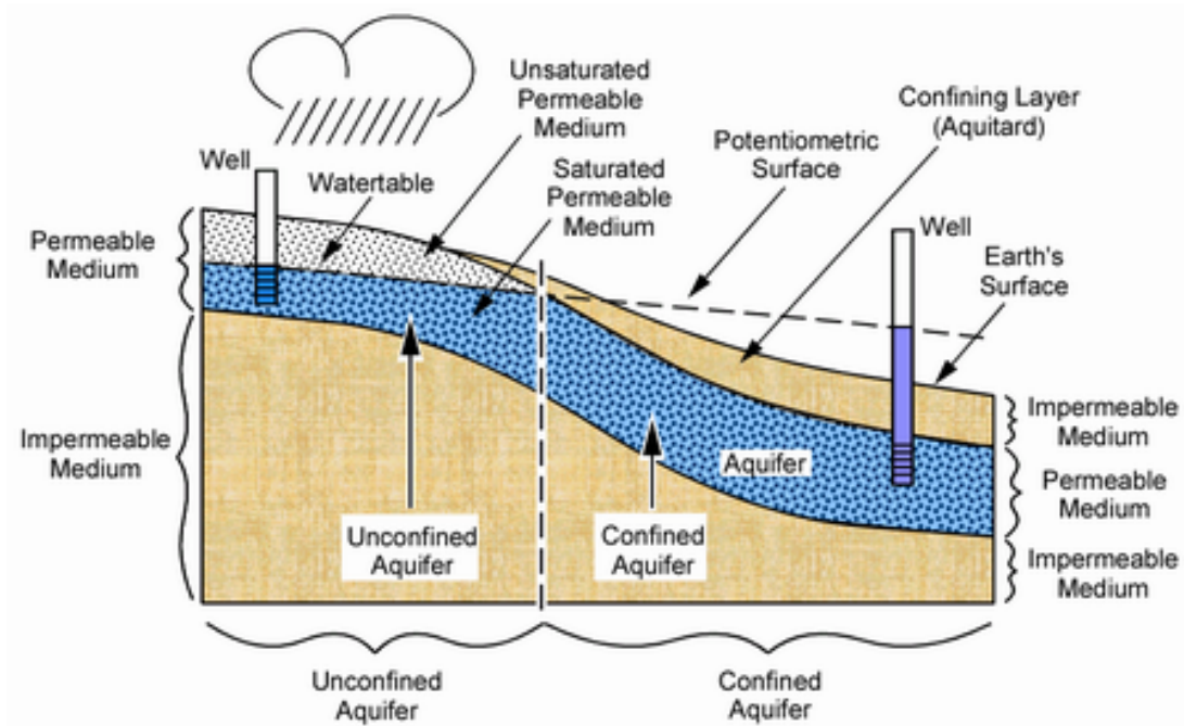
Figure 12-2. Schematic of aquifer transitioning from unconfined in outcrop region, where recharge from precipitation occurs, to confined conditions in the down dip regions of the aquifer (from http://www.geo.brown.edu/research/Hydrology/ge58_IntrodHydrology/ge58_index.htm ).
