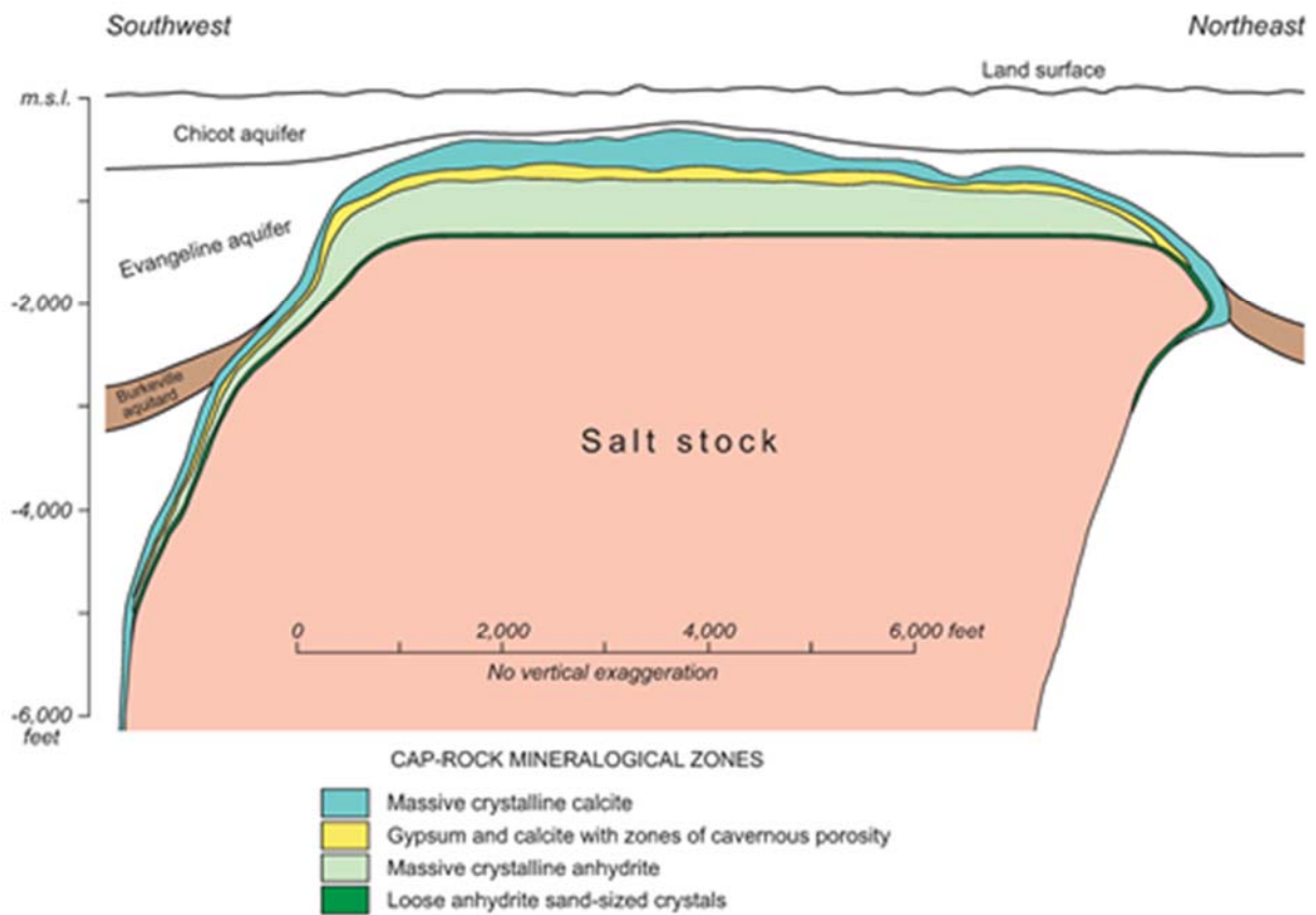
Figure 5-5. Cross-section of Barbers Hill salt dome in Chambers County showing the salt stock, cap rock mineralogical zones, and enclosing hydrostratigraphic intervals (modified from Hamlin and others, 1988).
