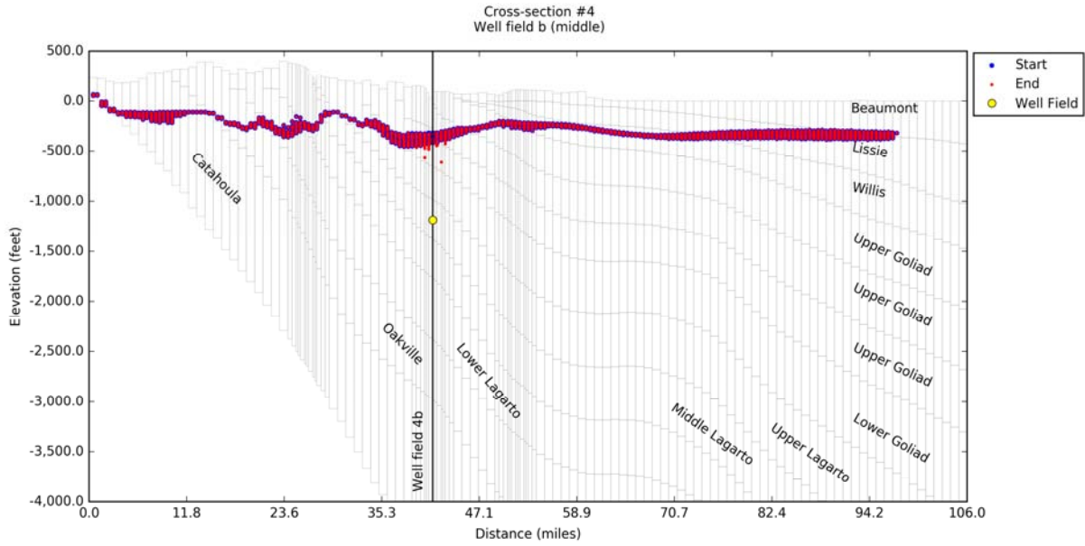
Figure 14-94. Simulated particle tracks 50 years after pumping the middle Well Field #4b located along Cross-Section #4 on Figure 14-5 at 10,000 acre-feet per year.
