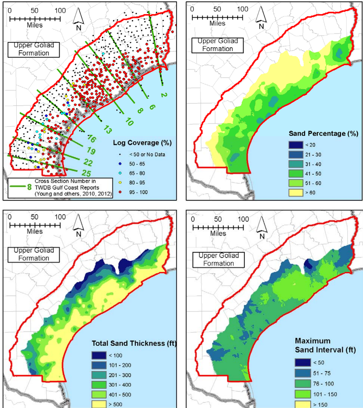
Figure 11-1. Maps of log coverage, sand percentage, total sand thickness and maximum sand interval for the Upper Goliad Formation. Log coverage is the percentage of the formation intersected by the portion of the geophysical log analyzed for the presence of sand beds.
