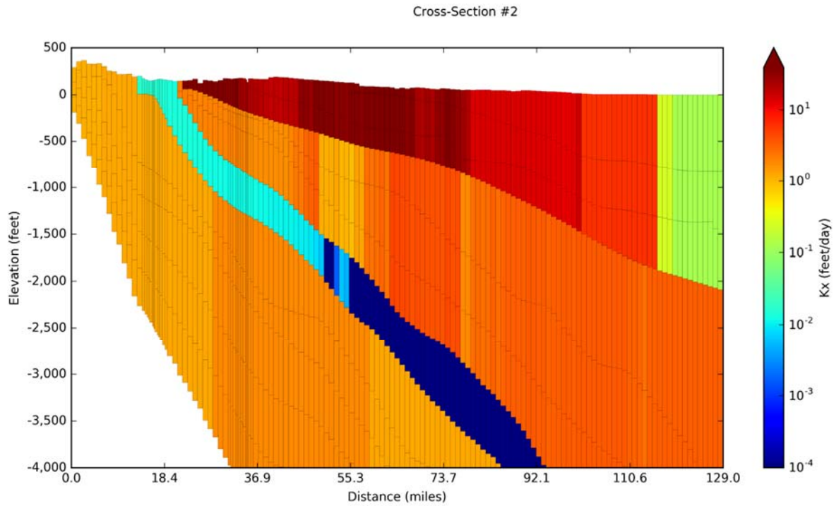
Figure 14-36. Horizontal hydraulic conductivity (Kx) values for Cross-Section #2 on Figure 14-5 with aquifer properties from the Houston Area Groundwater Model (Kasmarek, 2012) for model layers 1 to 12.
