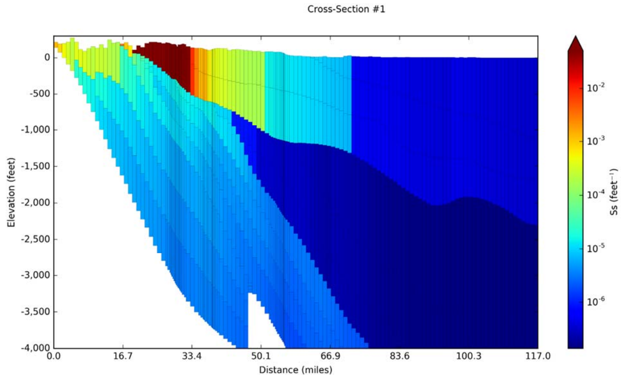
Figure 14-29. Specific storage (Ss) values in the groundwater model for Cross-Section #1 on Figure 14-5 for model layers 1 to 13.
