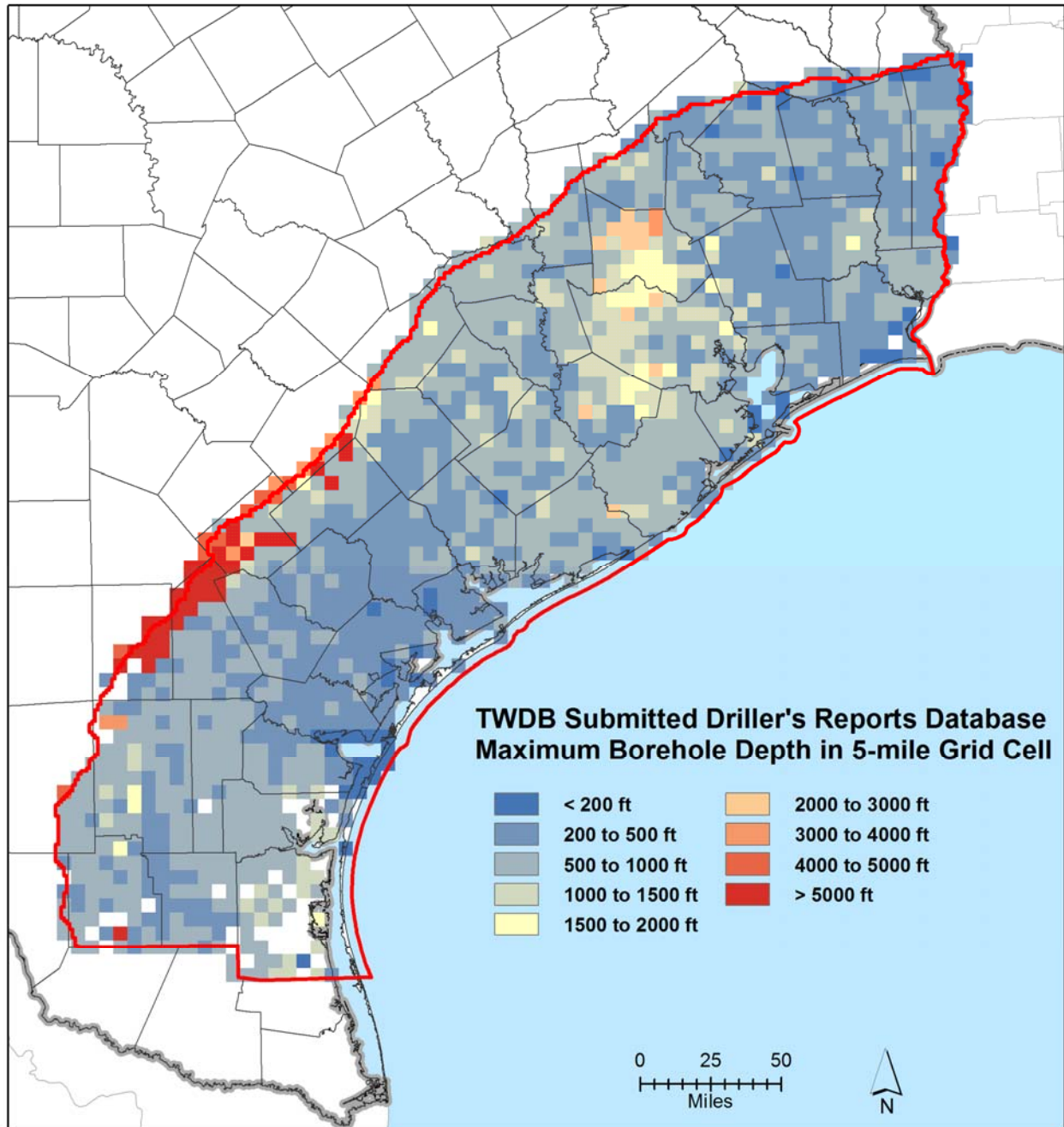
Figure 6-33. Maximum well depth that occurs across 5 mile-by-5-mile grid cells based on well information obtained from the TWDB Submitted Drillers Report.
