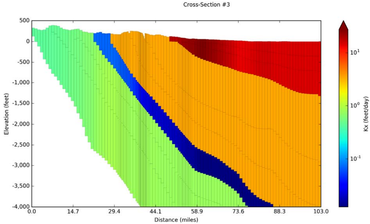
Figure 14-48. Horizontal hydraulic conductivity ( K_x ) values for Cross-Section #3 on Figure 14-5 with aquifer properties from the Central Gulf Coast Groundwater Availability Model (Chowdhury and others, 2004) for model layers 1 to 10.
