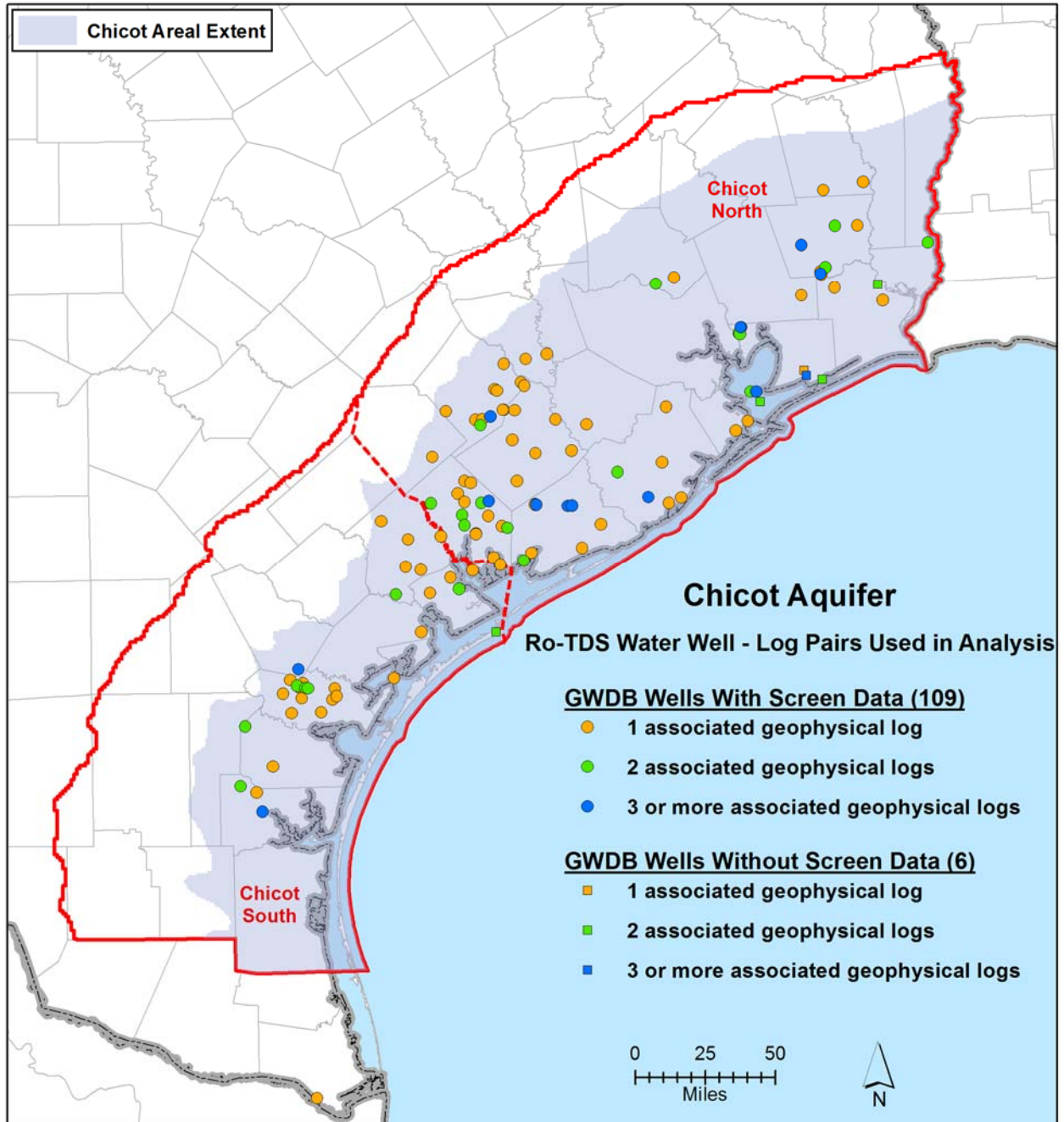
Figure 13-22. Location of the 164 well pairs used to construct the Ro-TDS graph for the Chicot Aquifer Group, which includes the Beaumont, Lissie, and Willis formations.
