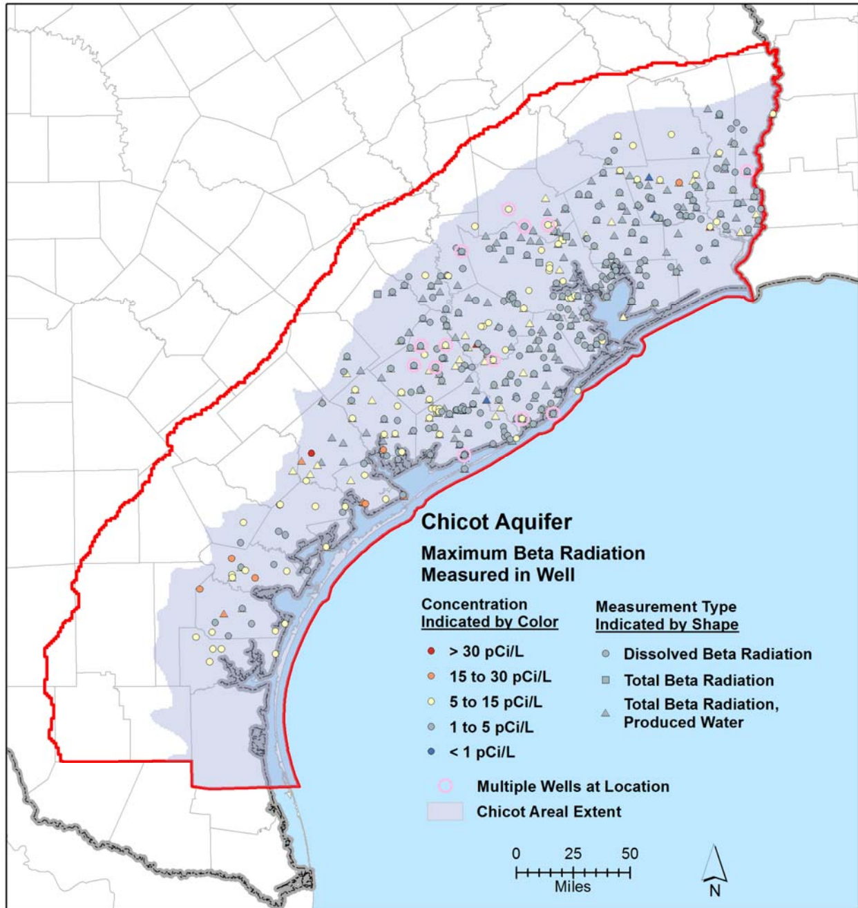
Figure 10-19. Maximum beta radiation in the Chicot Aquifer.
