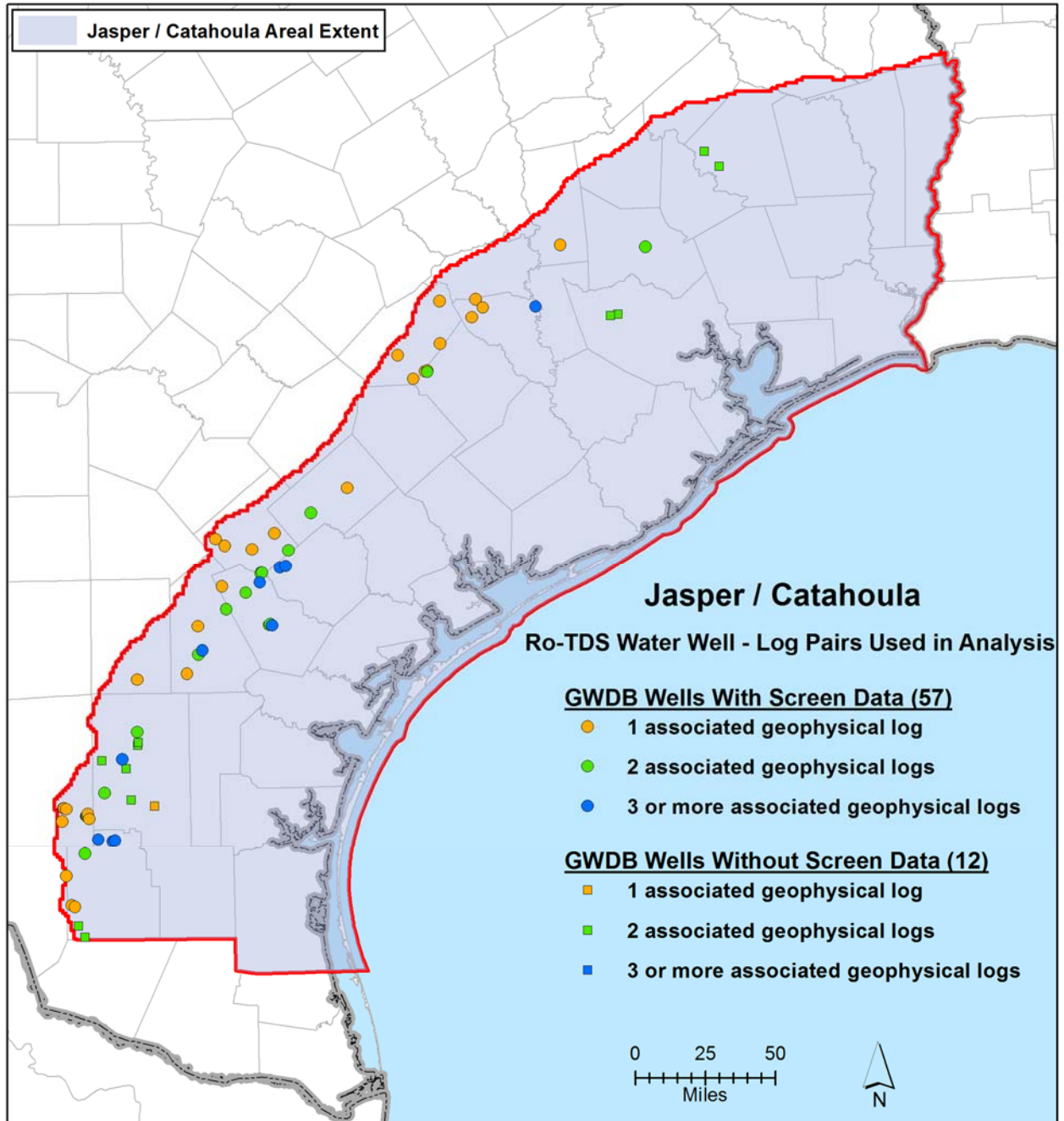
Figure 13-24. Location of the 117 well pairs used to construct the R 0 -TDS graph for Jasper/Catahoula Aquifer Group, which includes the Lower Lagarto, Oakville, Catahoula formations.
