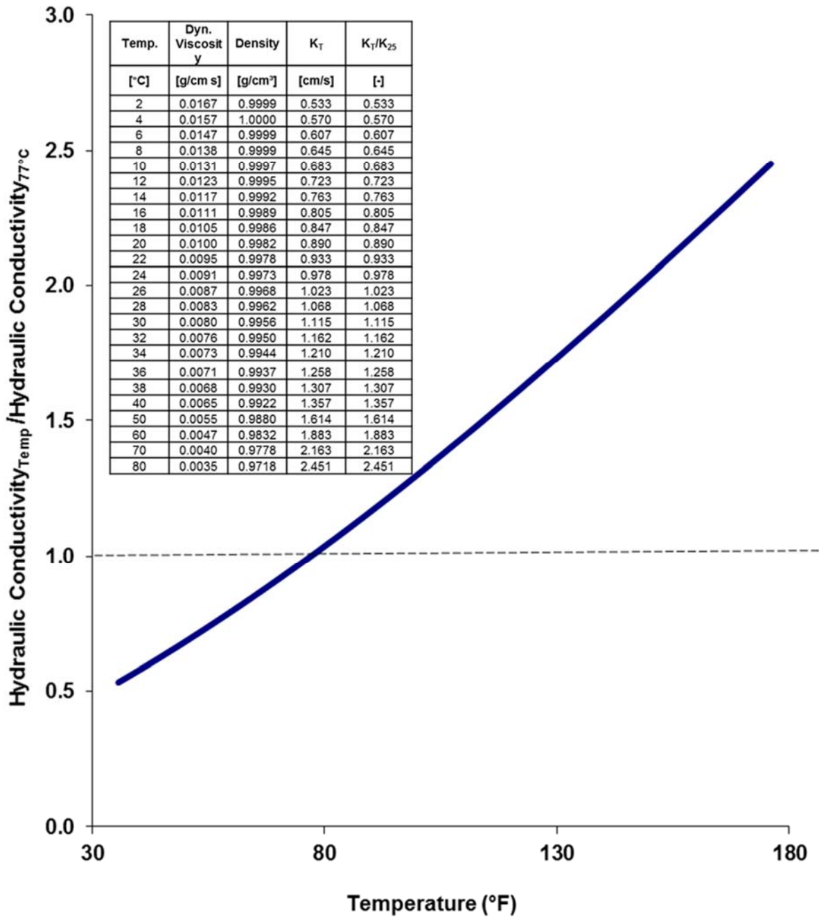
Figure 14-22. Relative change in hydraulic conductivity values caused by the temperature dependence of the density and viscosity of water (data from . http://www.viscopedia.com/viscosity-tables/substances/water/ )
