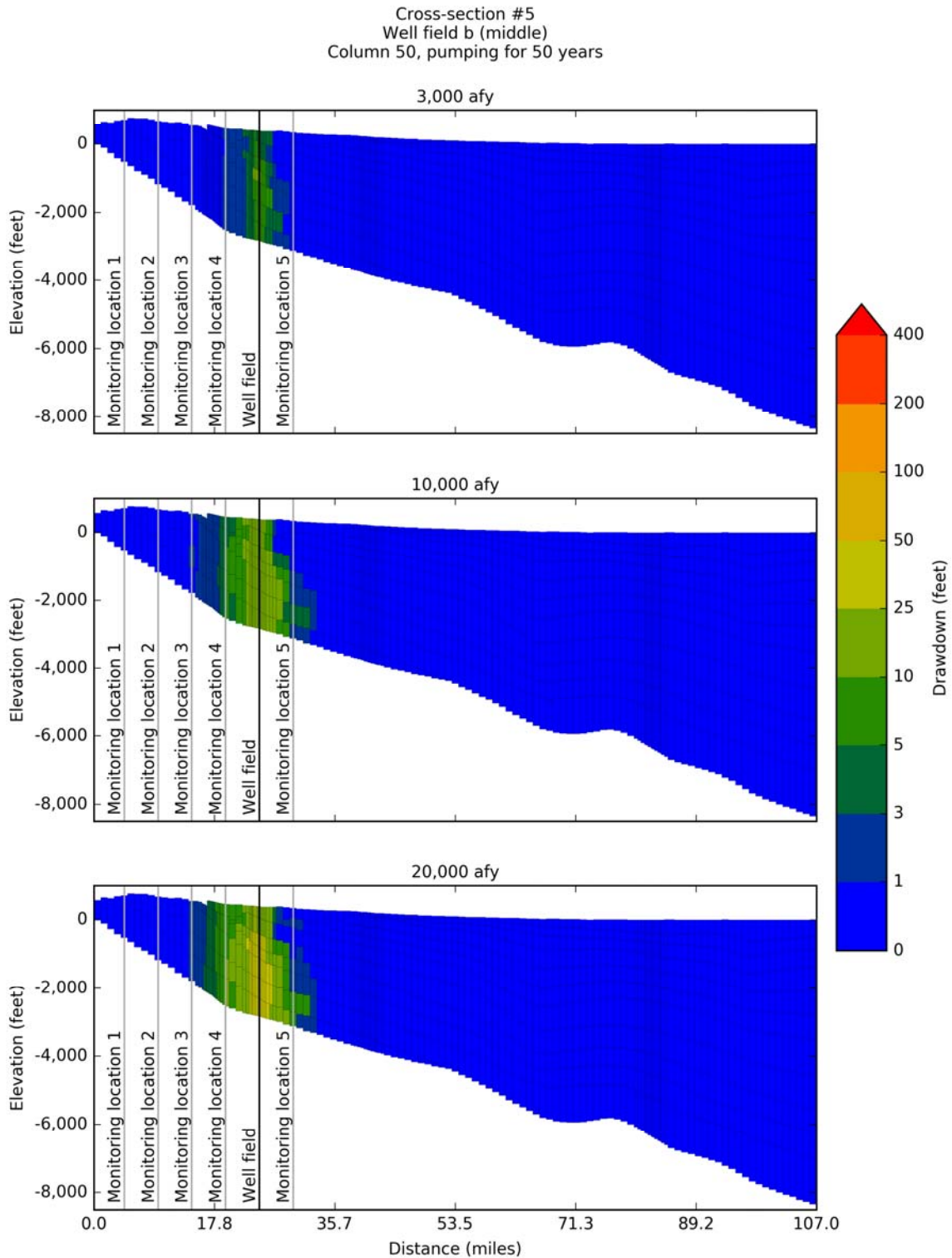
Figure 14-81. Simulated drawdown at 50 years after pumping the middle Well Field #5b located along Cross-Section #5 on Figure 14-5 at 3,000 acre-feet per year, 10,000 acre-feet per year, and 20,000 acre-feet per year.
