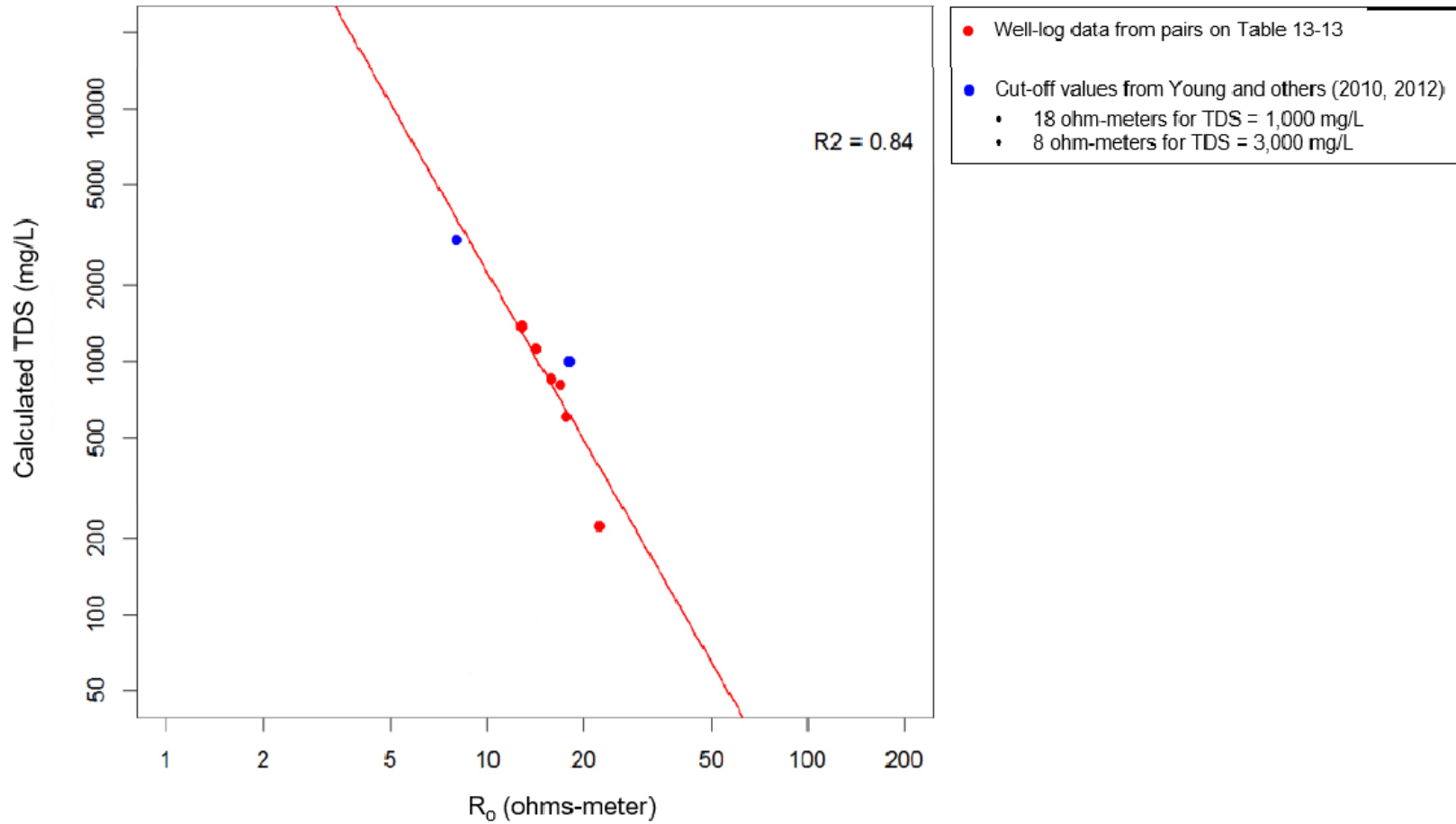
Figure 13-16. R 0 -TDS graph for the formations associated with the Chicot Aquifer Group (including the Beaumont, Lissie, and Willis formations) developed using the R 0 -TDS data in Table 13-13 (red dots) and resistivity “cut-off” values used by Young and others (2010, 2012) (blue dots).
