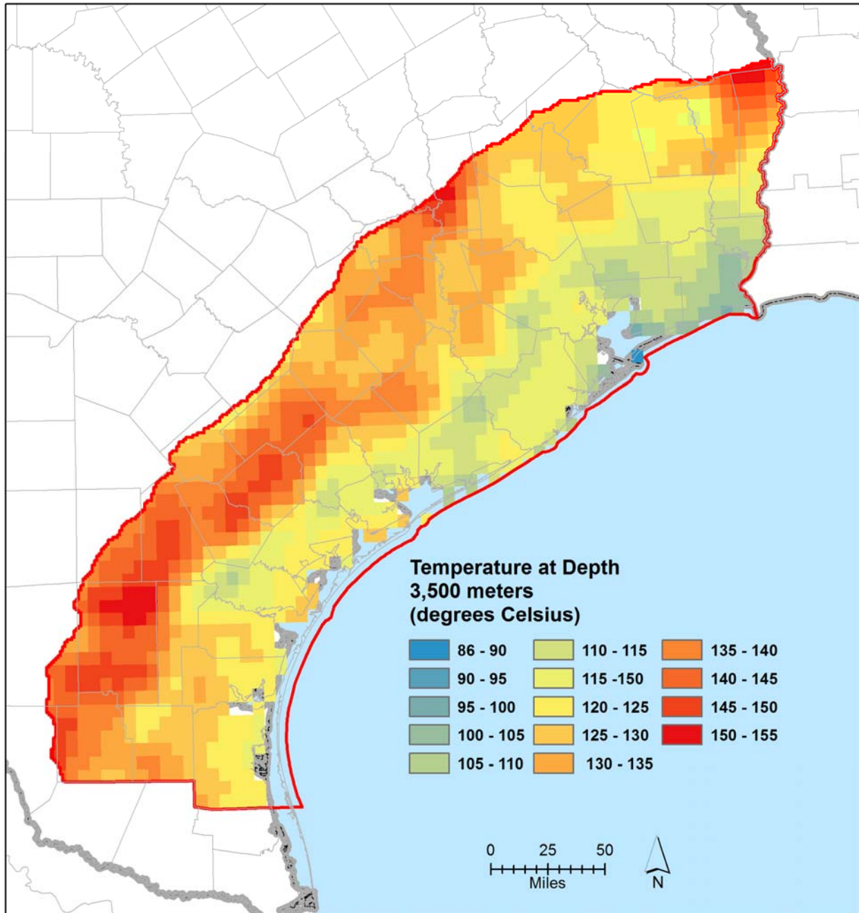
Figure 7-8. Temperature at depth of 3,500 meters based on analysis of bottom hole temperatures (Blackwell and others, 2011).
