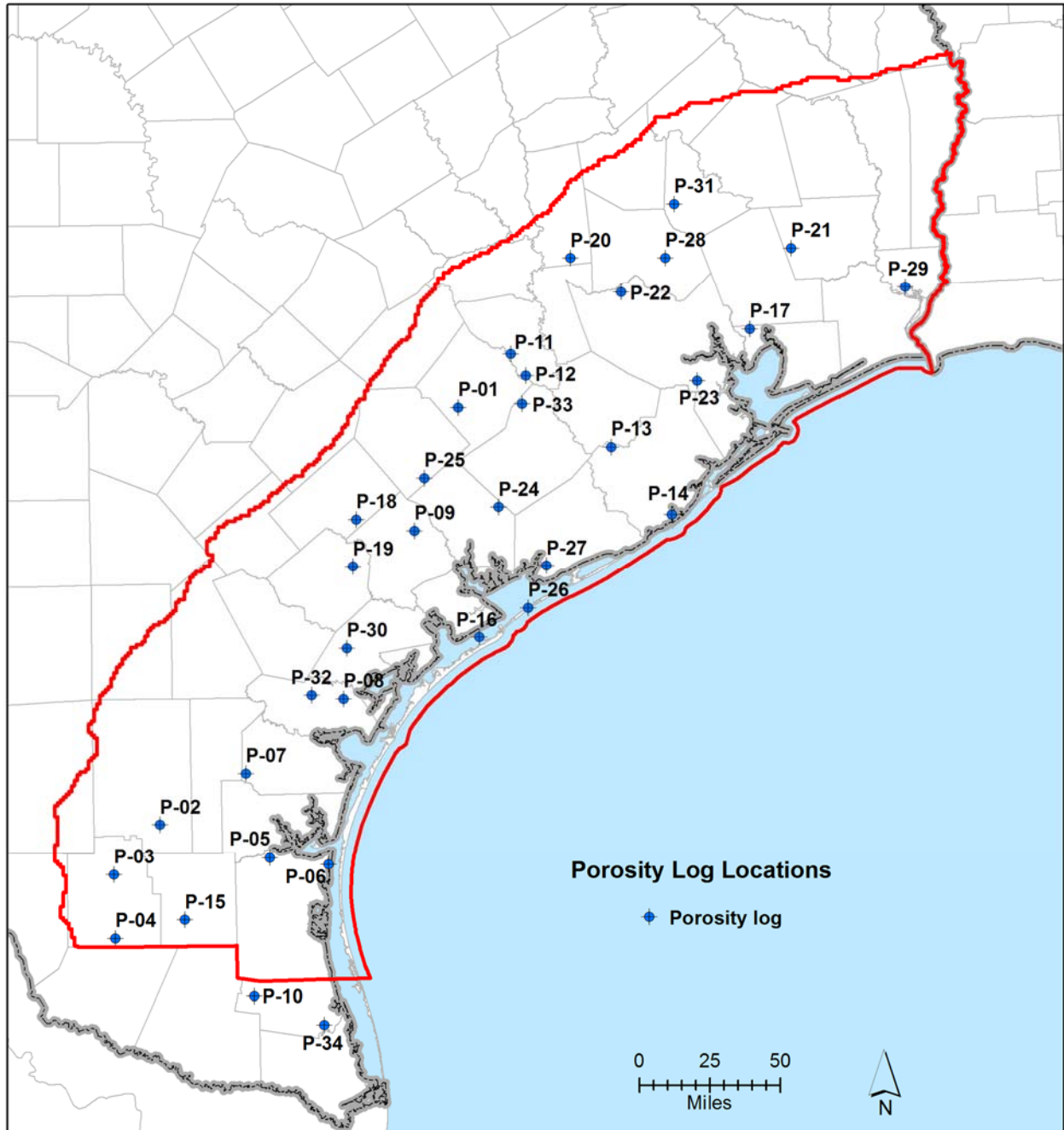
Figure 11-17. Locations of thirty-four logs that were analyzed to determine porosity values.
