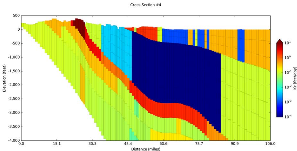
Figure 14-63. Vertical hydraulic conductivity ( K_z ) values in the groundwater model for Cross-Section #4 on Figure 14-5 for model layers 1 to 12.
