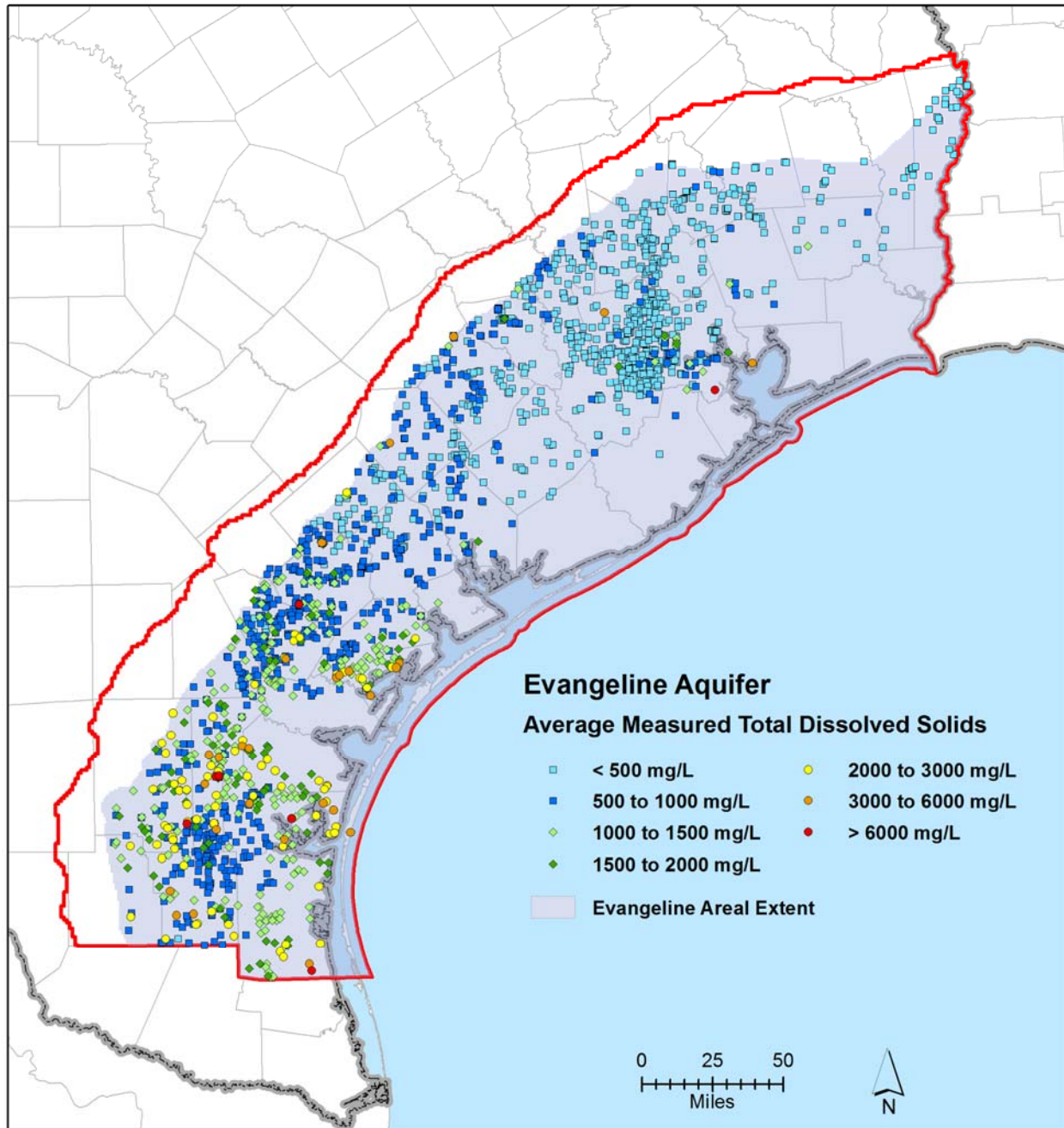
Figure 10-3. Average measured total dissolved solids concentration in the Evangeline Aquifer.
