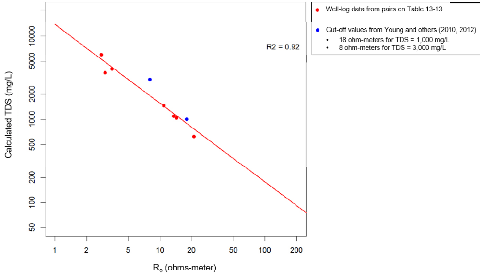
Figure 13-18. R 0 -TDS graph for the formations associated with the Jasper/Catahoula Aquifer Group (including the Lower Lagarto, Oakville, and Catahoula formations) developed using the R 0 -TDS data in Table 13-13 (red dots) and resistivity “cut-off” values used by Young and others (2010, 2012) (blue dots).
