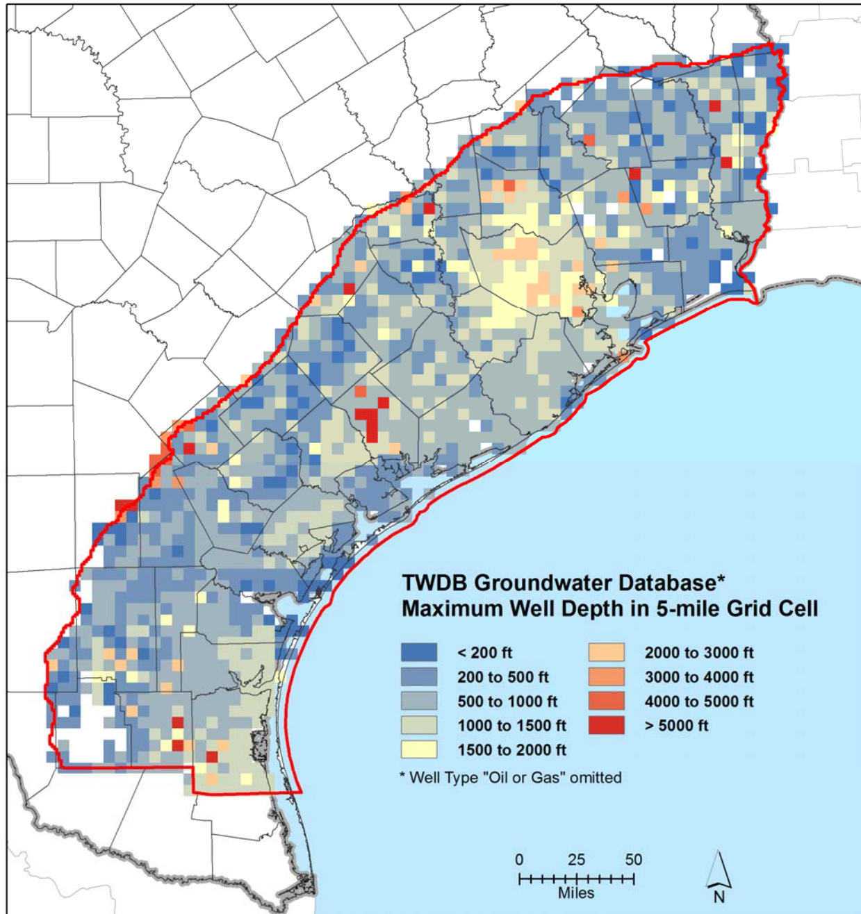
Figure 6-31. Maximum well depth that occurs across 5 mile-by-5-mile grid cells based on well information obtained from the TWDB groundwater database.
