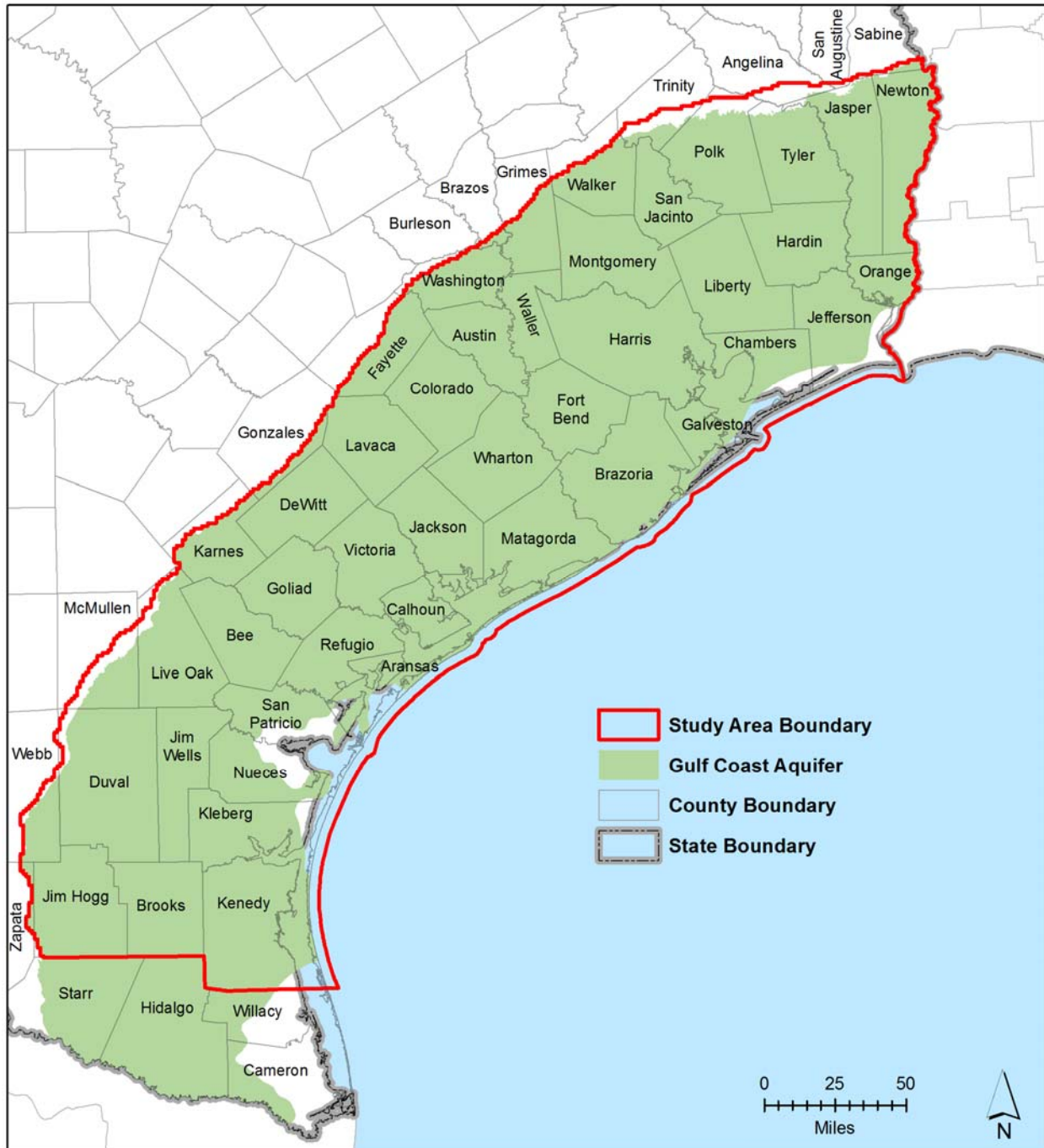
Figure 2-1. Study area.
