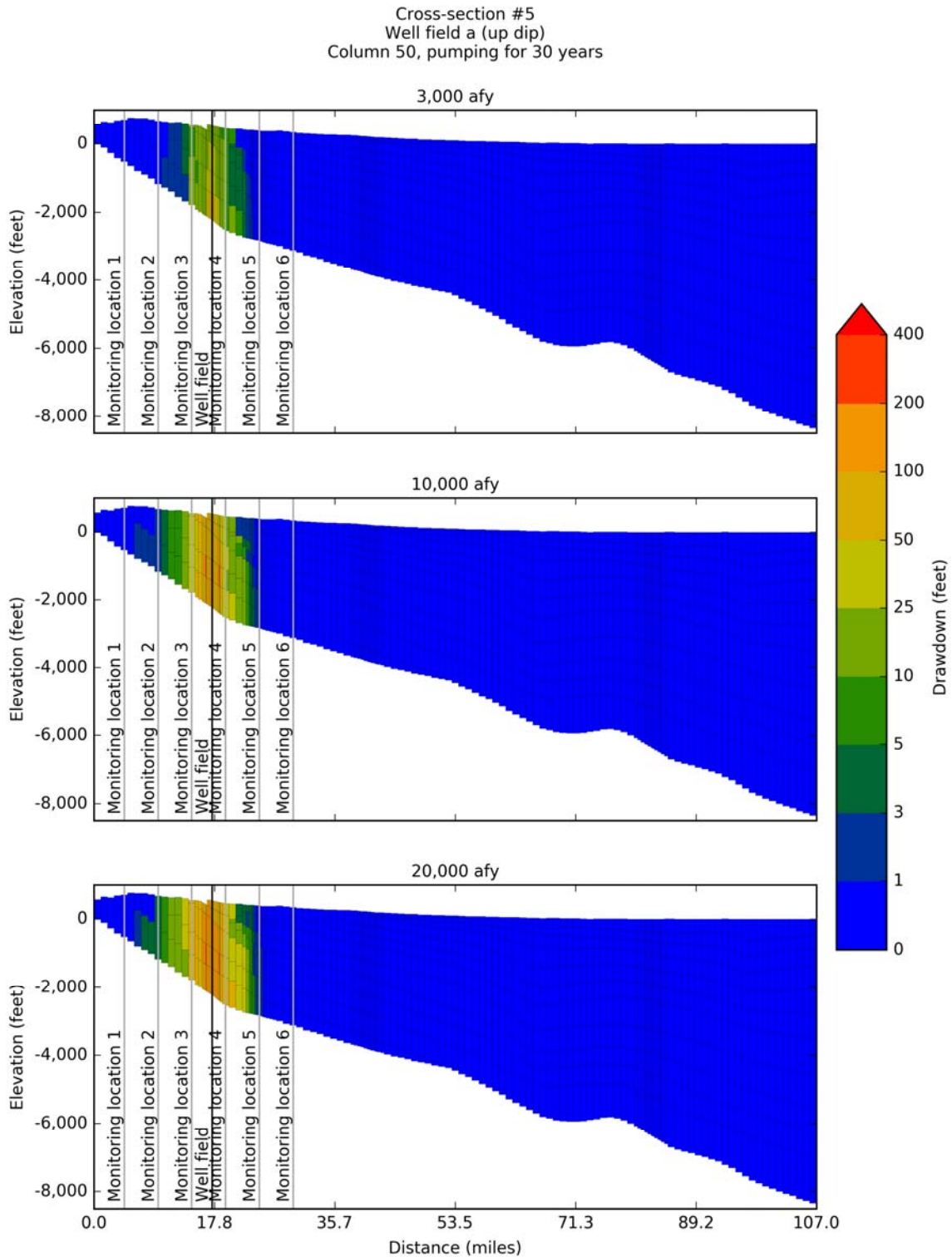
Figure 14-78. Simulated drawdown at 30 years after pumping the up dip Well Field #5a located along Cross-Section #5 on Figure 14-5 at 3,000 acre-feet per year, 10,000 acre-feet per year, and 20,000 acre-feet per year.
