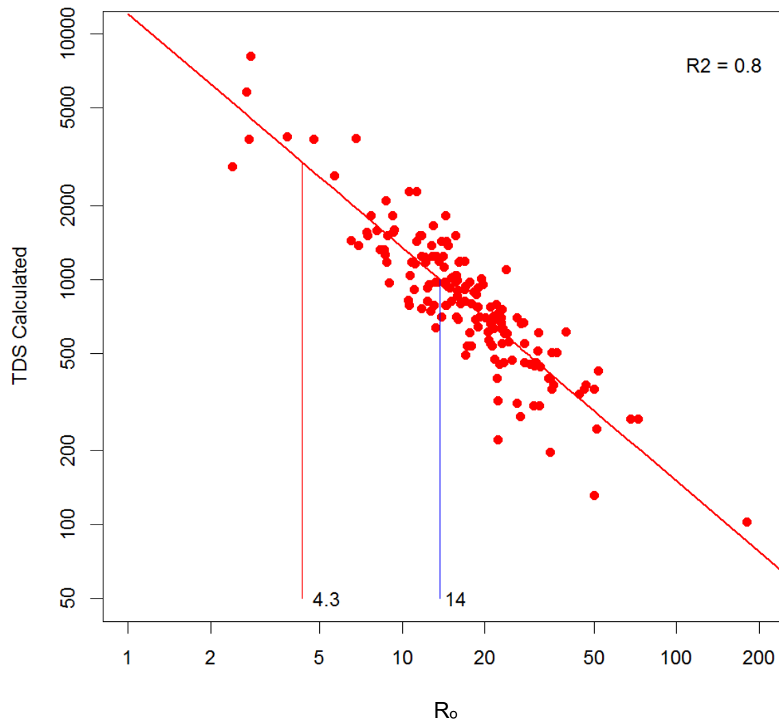
Figure 13-19. R o -TDS graph for the Chicot Aquifer Group (including the Beaumont, Lissie, and Willis formations) based on 164 well-log pairs. The blue line is the formation resistivity value for a 1,000 milligram per liter total dissolved solids concentration and the red line is the formation resistivity value for 3,000 milligrams per liter total dissolved solids concentration.
