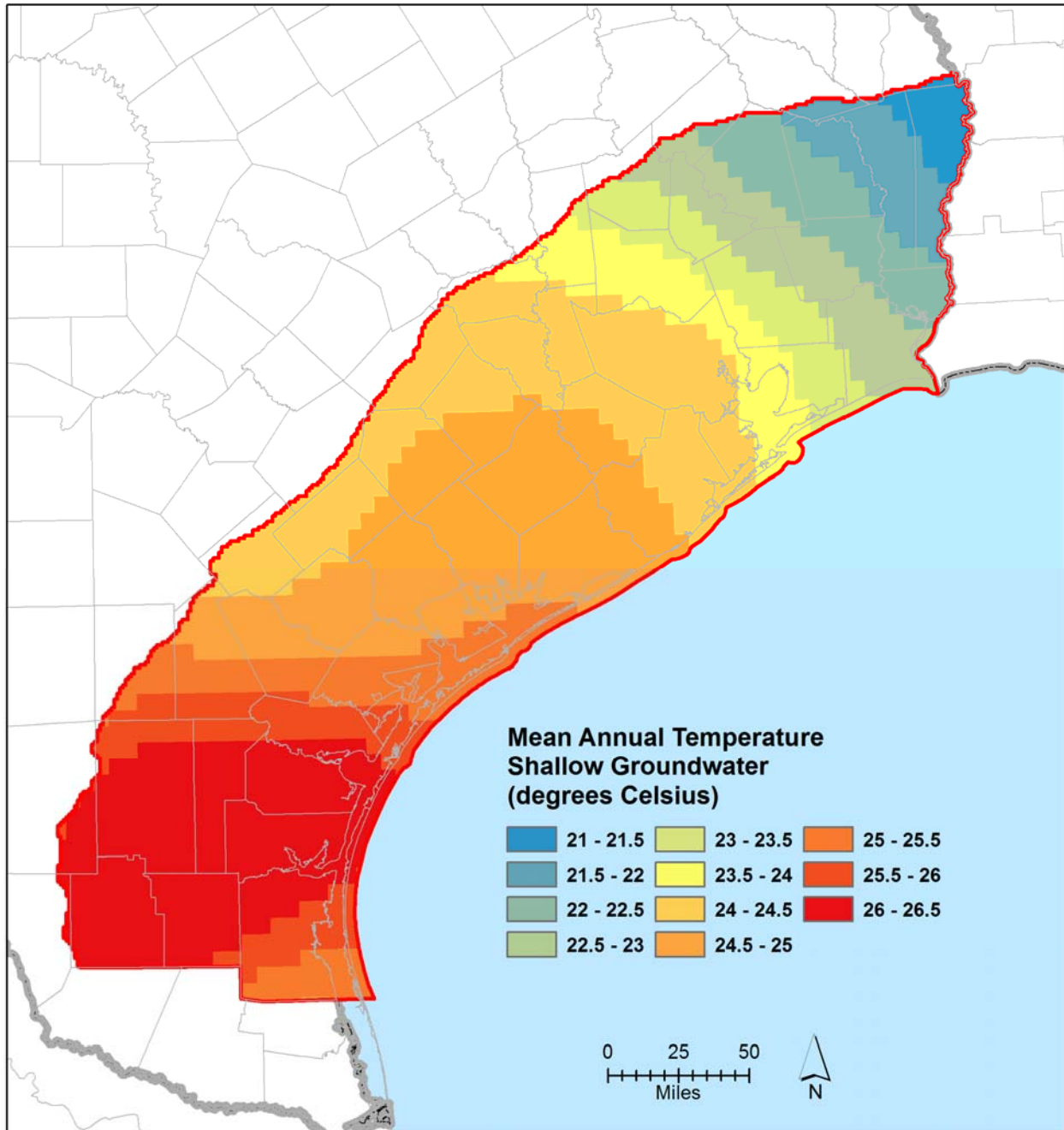
Figure 7-6. Temperature of shallow groundwater based on measurements from wells with depths ranging from 50 to 150 feet (based on Gass, 1982).
