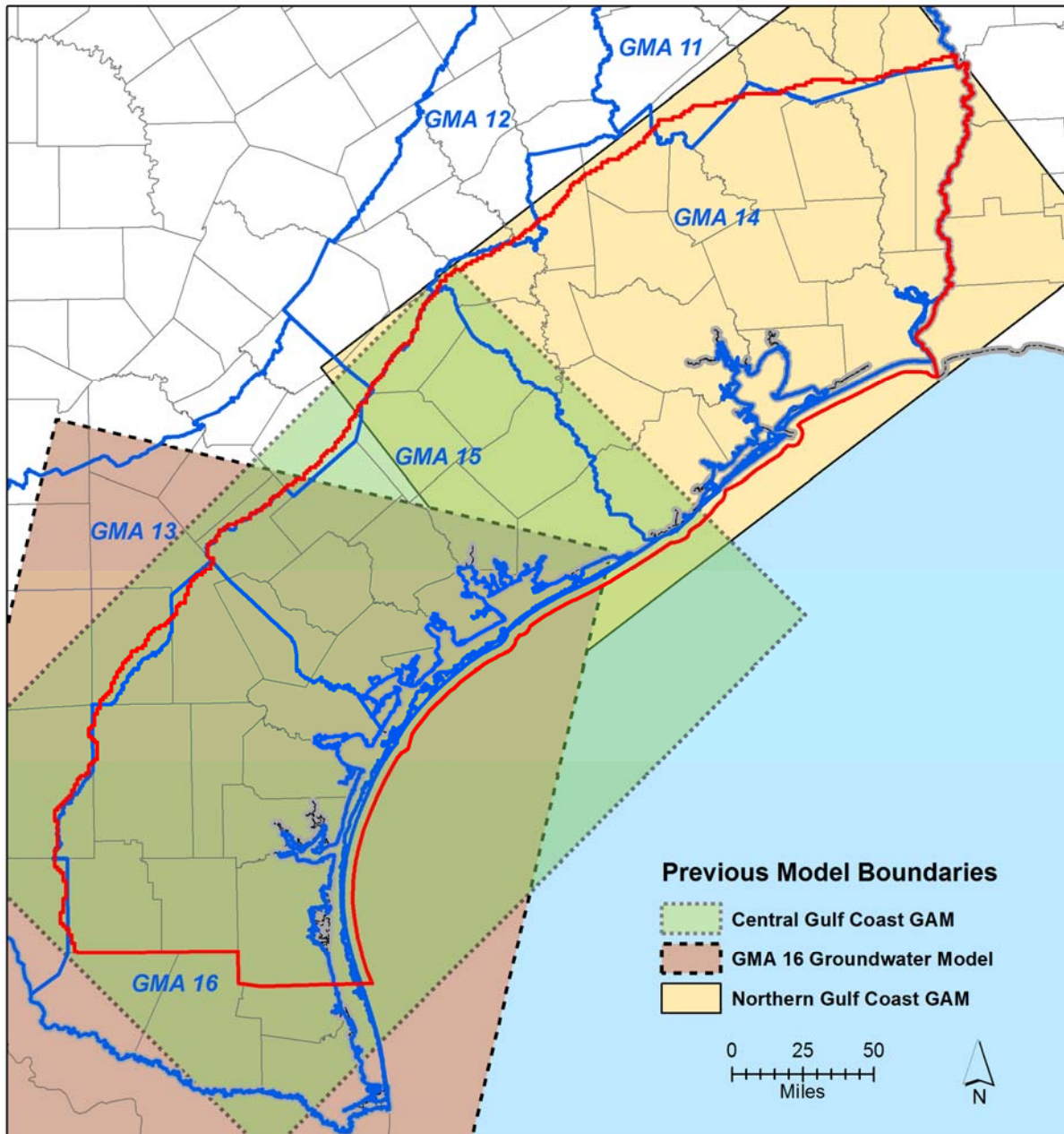
Figure 14-2. Model domains of the groundwater models used for joint planning in Groundwater Management Areas 14, 15, and 16.
