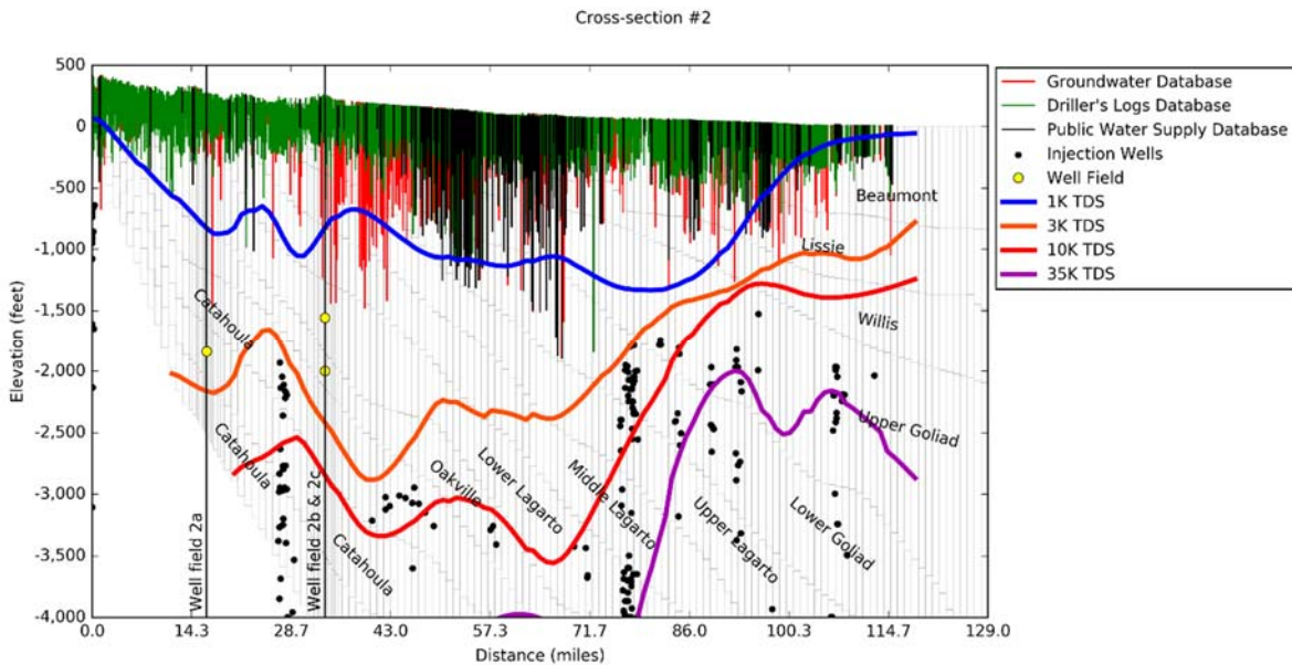
Figure 14-12. Boundaries for fresh water, slightly saline, moderately saline, and very saline groundwater along Cross-Section #2 on Figure 14-5.
