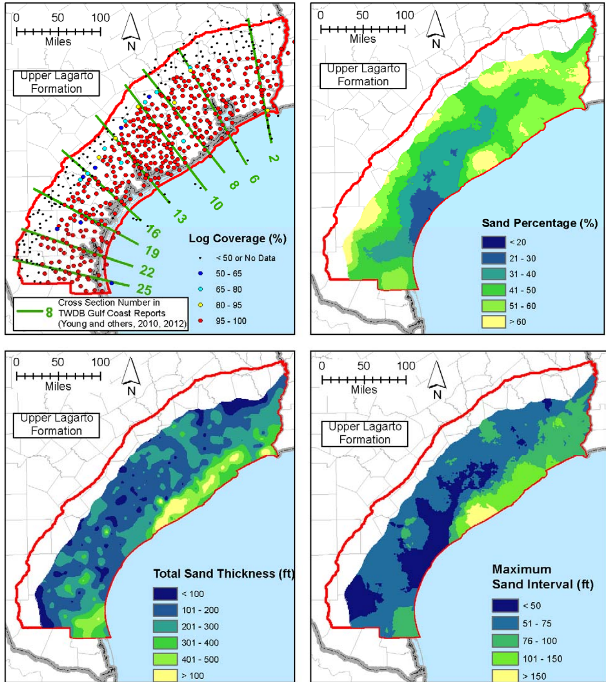
Figure 11-3. Maps of log coverage, sand percentage, total sand thickness and maximum sand interval for the Upper Lagarto Formation. Log coverage is the percentage of the formation intersected by the portion of the geophysical log analyzed for the presence of sand beds.
