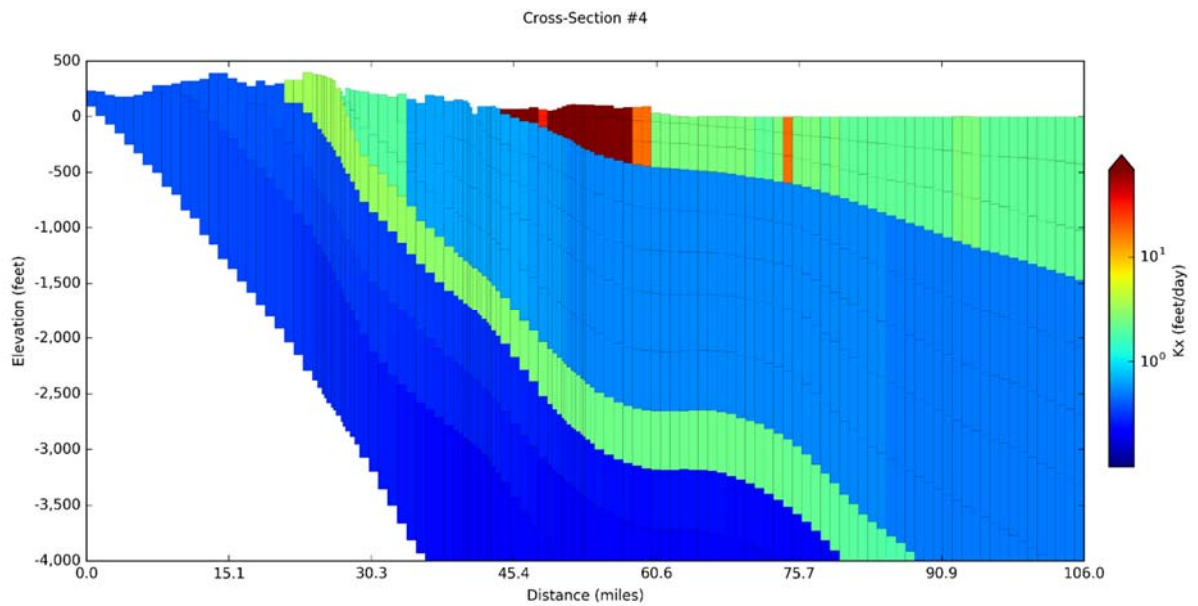
Figure 14-61. Horizontal hydraulic conductivity ( K_x ) values in the groundwater model for Cross-Section #4 on Figure 14-5 for model layers 1 to 12.
