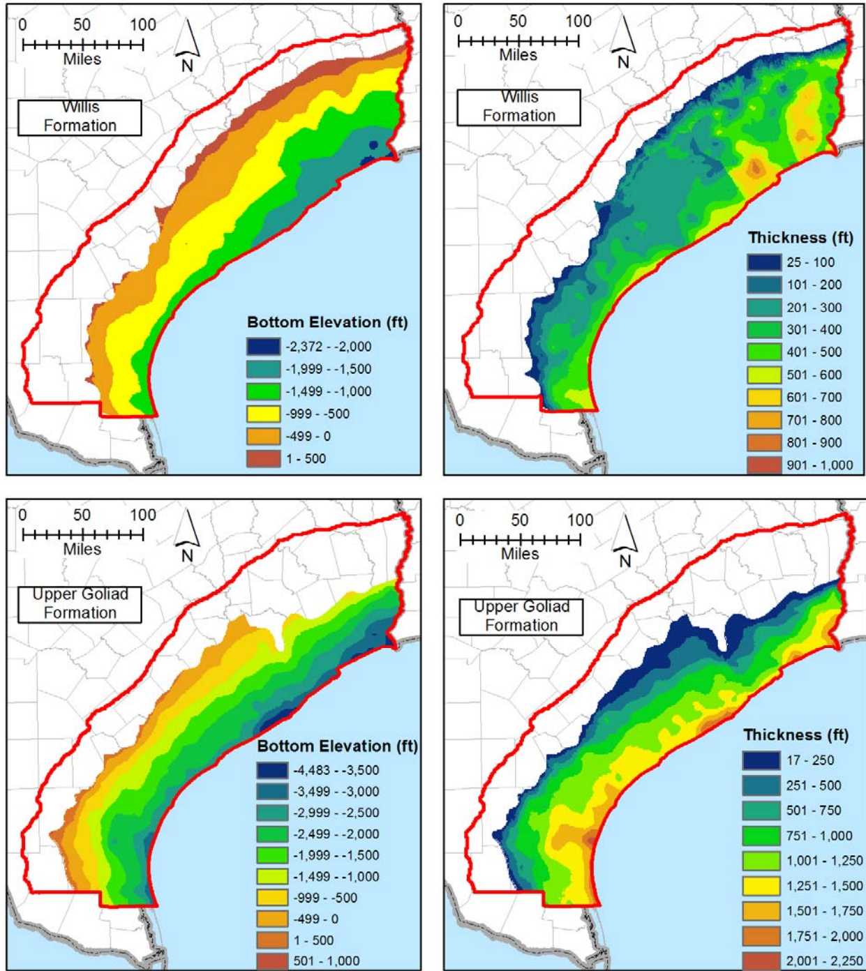
Figure 7-2. Bottom elevation and thickness for the Willis and Upper Goliad formations based on the data from Young and others (2010, 2012).
