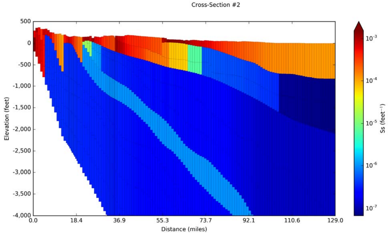
Figure 14-40. Specific storage (Ss) values for Cross-Section #2 on Figure 14-5 with aquifer properties from the Houston Area Groundwater Model (Kasmarek, 2012) for model layers 1 to 12.
