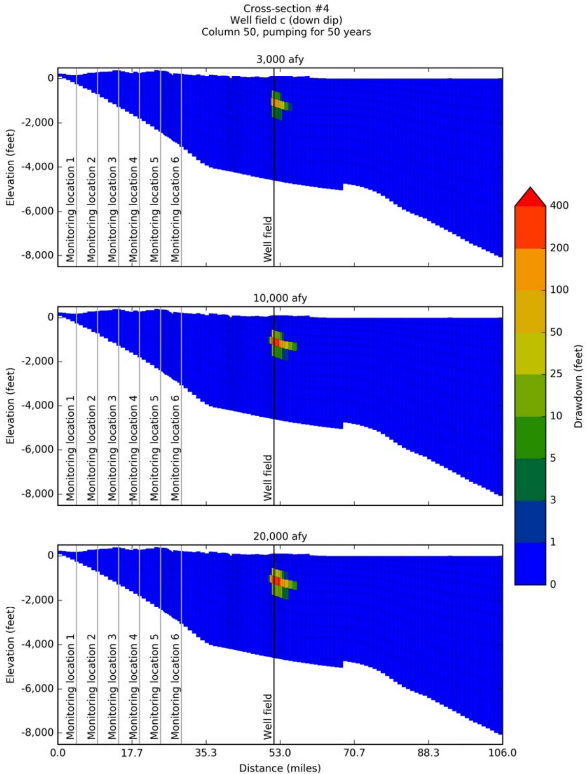
Figure 14-71. Simulated drawdown at 50 years after pumping the down dip Well Field #4c located along Cross-Section #4 on Figure 14-5 at 3,000 acre-feet per year, 10,000 acre-feet per year, and 20,000 acre-feet per year.
