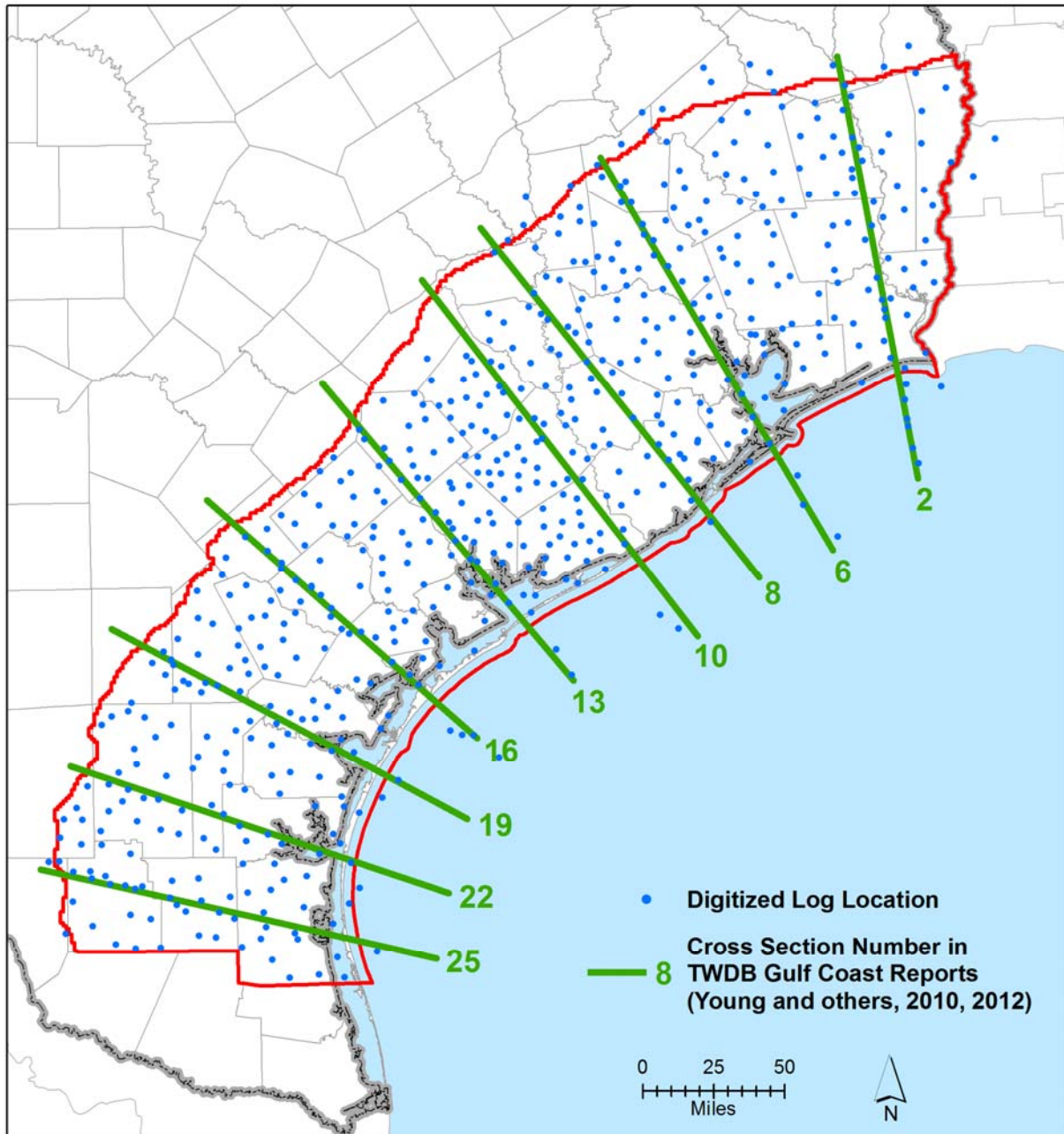
Figure 6-1. Location of the geophysical logs that were interpreted to develop salinity zones and location of nine cross-sections where vertical cross-sections of salinity zones are discussed.
