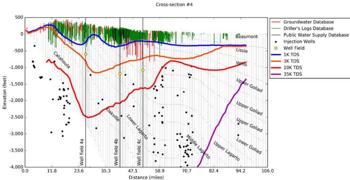
Figure 14-14. Boundaries for fresh water, slightly saline, moderately saline, and very saline groundwater along Cross-Section #4 on Figure 14-5.
