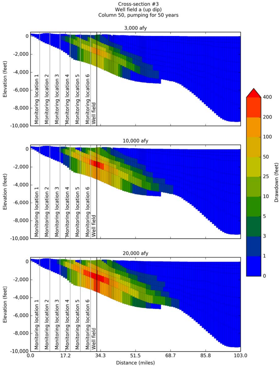
Figure 14-55. Simulated drawdown at 50 years after pumping the up dip Well Field #3a located along Cross-Section #3 on Figure 14-5 at 3,000 acre-feet per year, 10,000 acre-feet per year, and 20,000 acre-feet per year.
