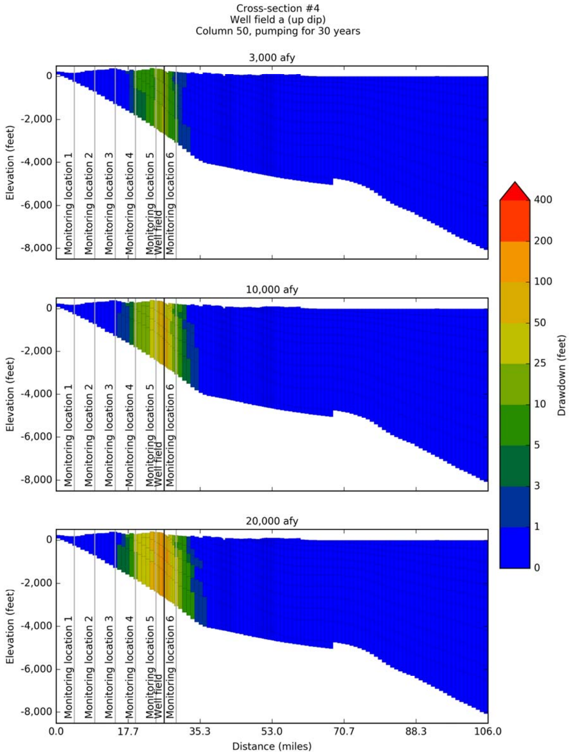
Figure 14-66. Simulated drawdown at 30 years after pumping the up dip Well Field #4a located along Cross-Section #4 on Figure 14-5 at 3,000 acre-feet per year, 10,000 acre-feet per year, and 20,000 acre-feet per year.
