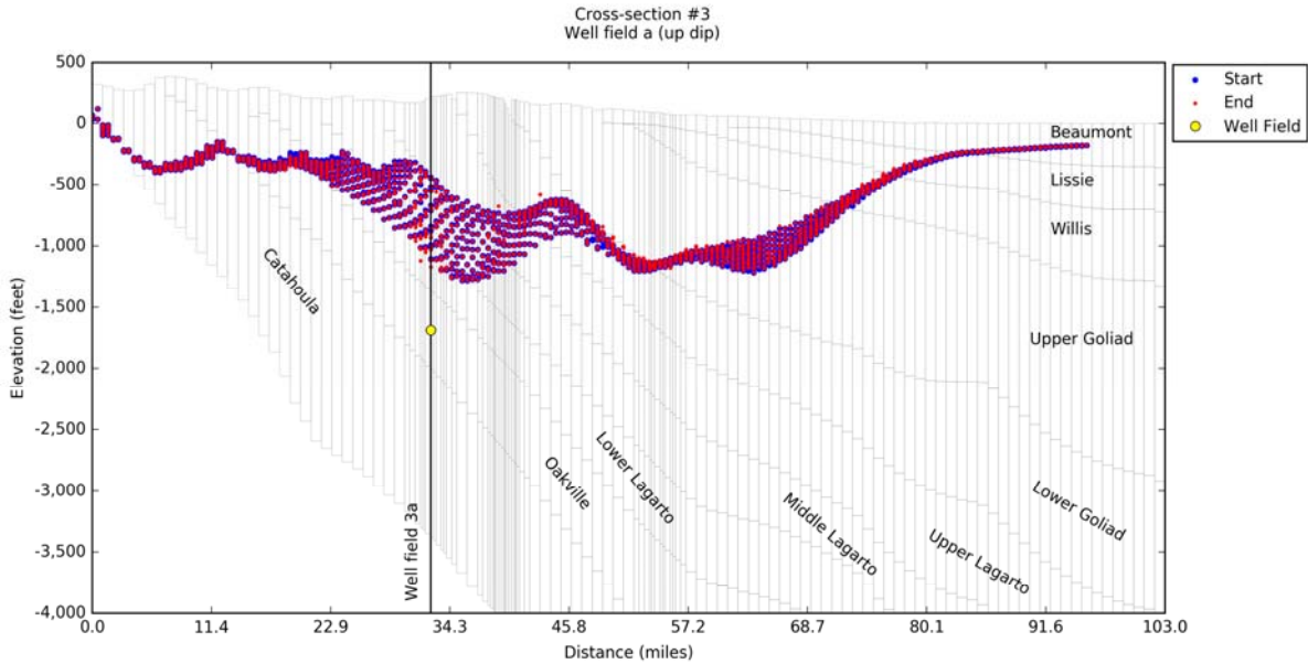
Figure 14-90. Simulated particle tracks 50 years after pumping the up dip Well Field #3a located along Cross-Section #3 on Figure 14-5 at 10,000 acre-feet per year.
