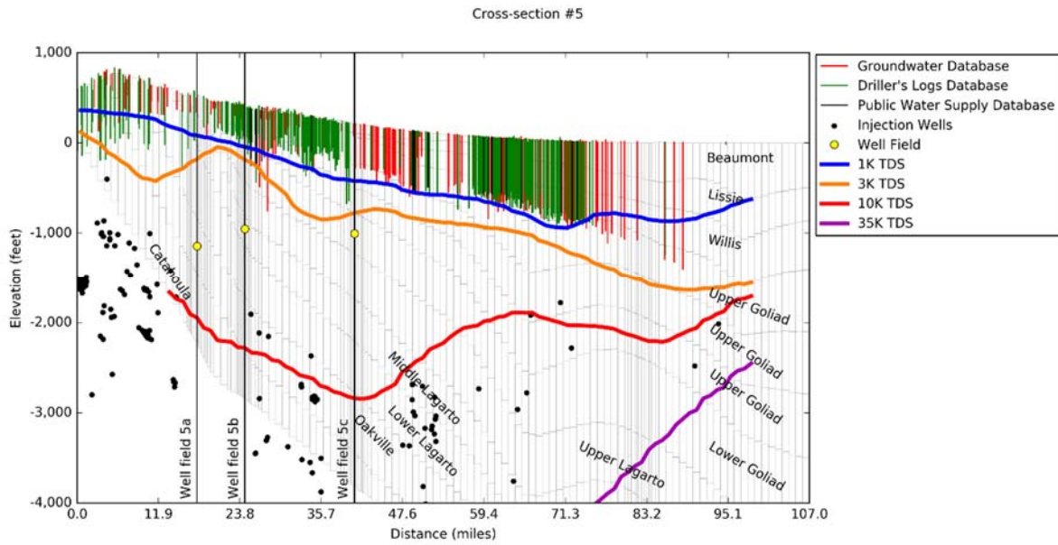
Figure 14-15. Boundaries for fresh water, slightly saline, moderately saline, and very saline groundwater along Cross-Section #5 on Figure 14-5.
