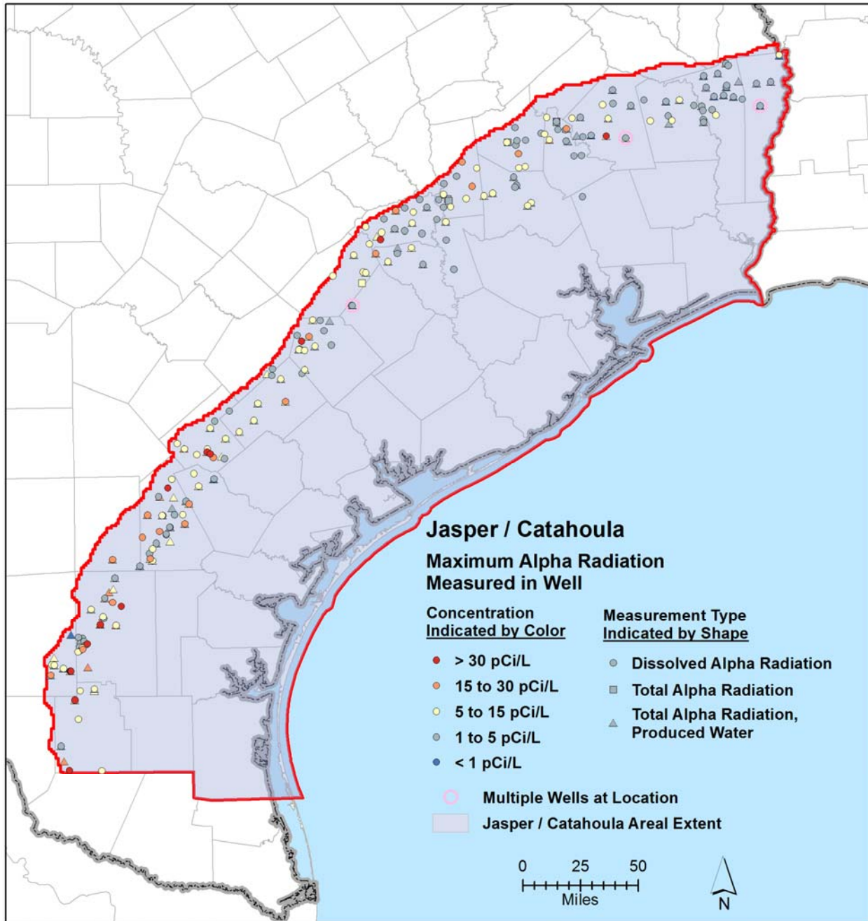
Figure 10-18. Maximum alpha radiation in the Jasper Aquifer and Catahoula Formation.
