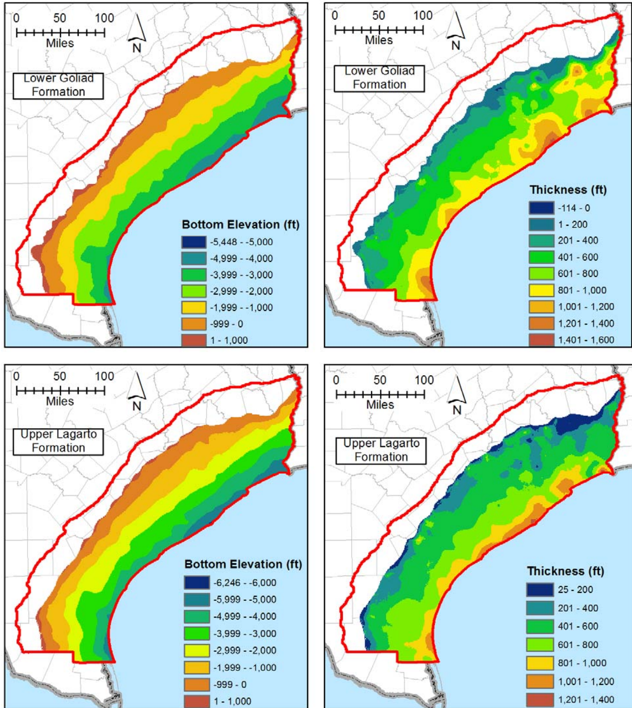
Figure 7-3. Bottom elevation and thickness for the Lower Goliad and Upper Lagarto formations based on the data from Young and others (2010, 2012).
