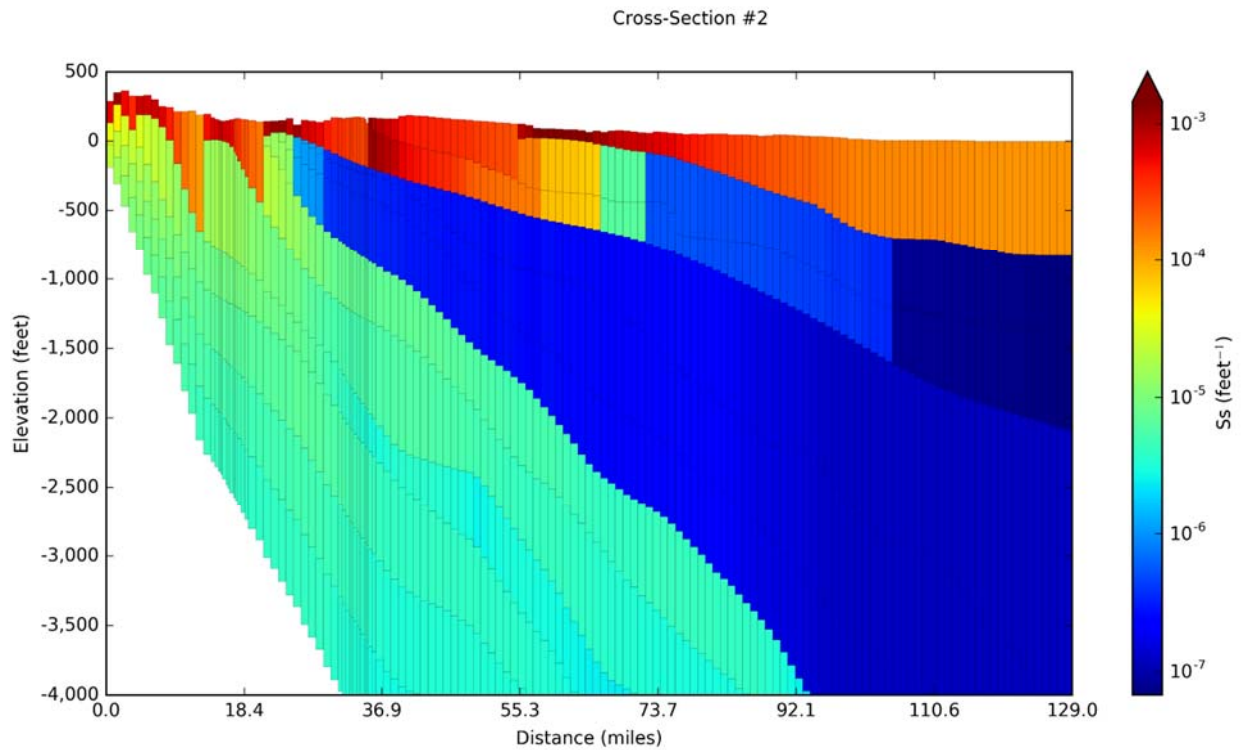
Figure 14-41. Specific storage (Ss) values in the groundwater model for Cross-Section #2 on Figure 14-5 for model layers 1 to 12.
