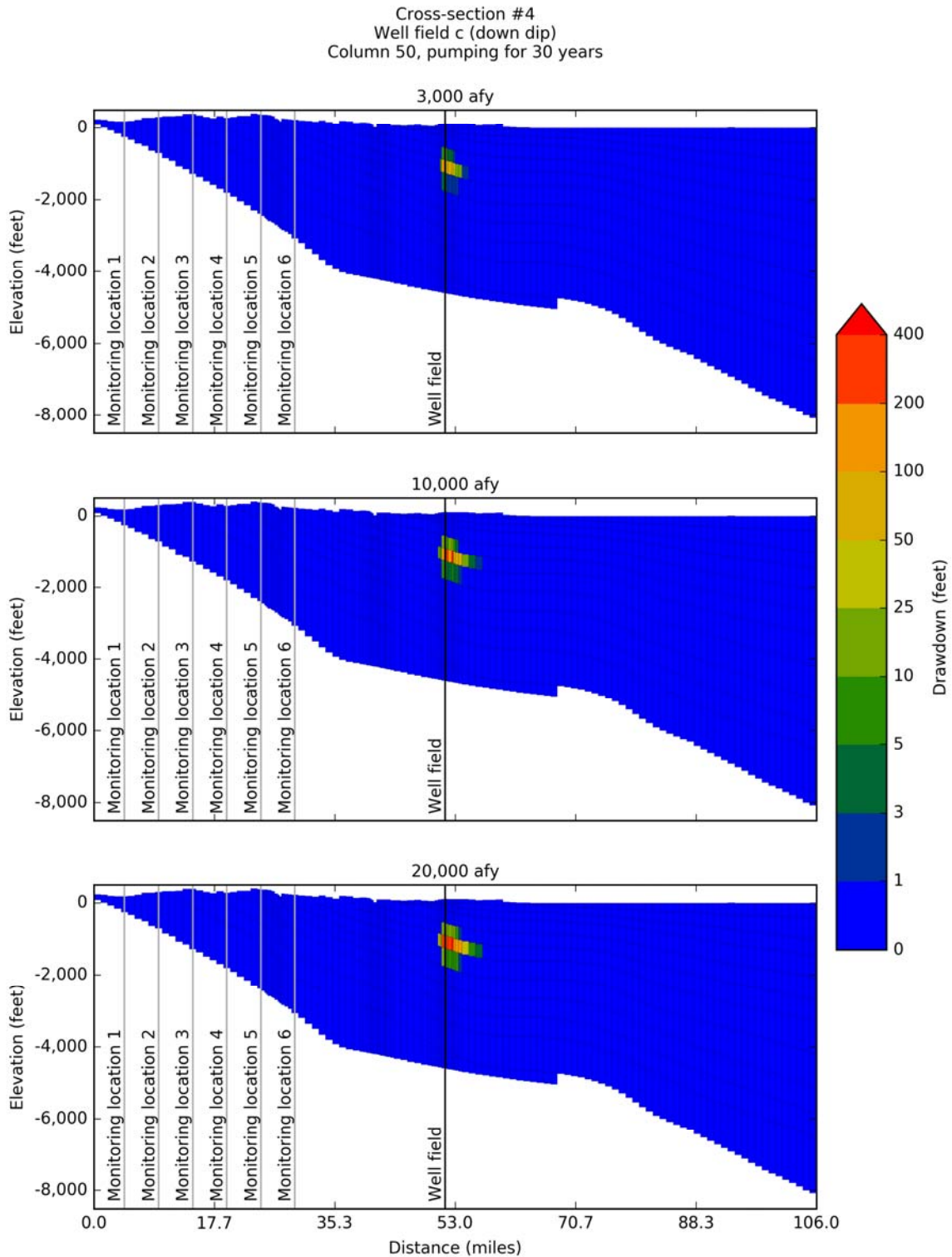
Figure 14-70. Simulated drawdown at 30 years after pumping the down dip Well Field #4c located along Cross-Section #4 on Figure 14-5 at 3,000 acre-feet per year, 10,000 acre-feet per year, and 20,000 acre-feet per year.
