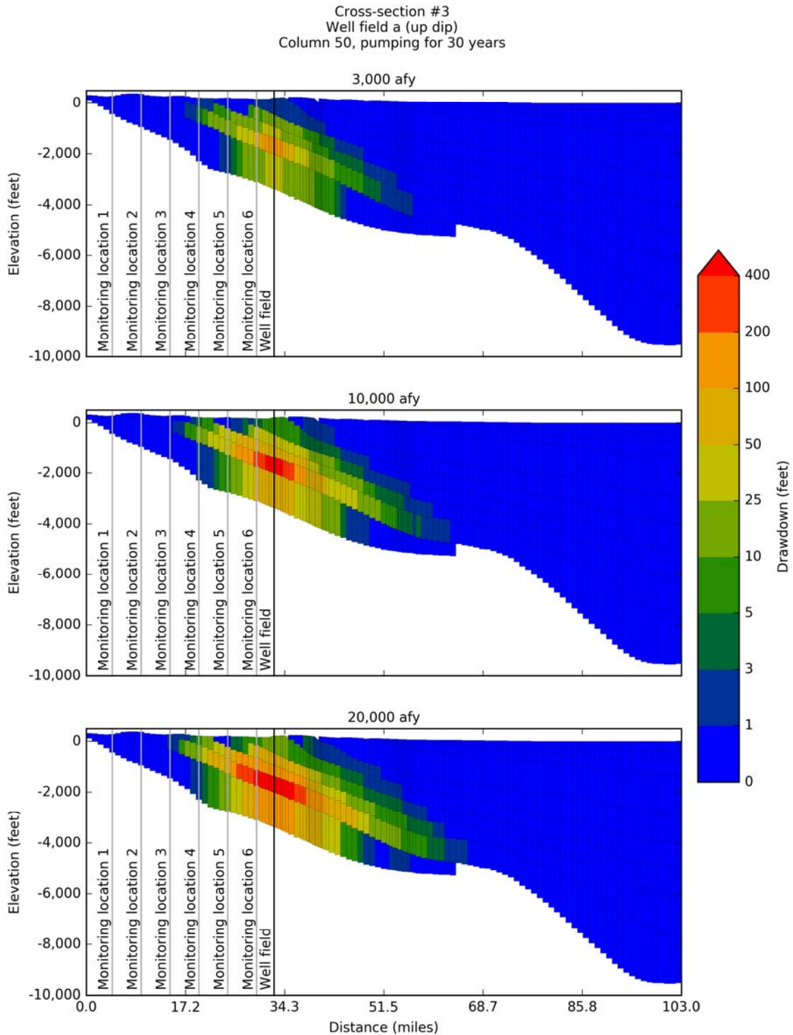
Figure 14-54. Simulated drawdown at 30 years after pumping the up dip Well Field #3a located along Cross-Section #3 on Figure 14-5 at 3,000 acre-feet per year, 10,000 acre-feet per year, and 20,000 acre-feet per year.
