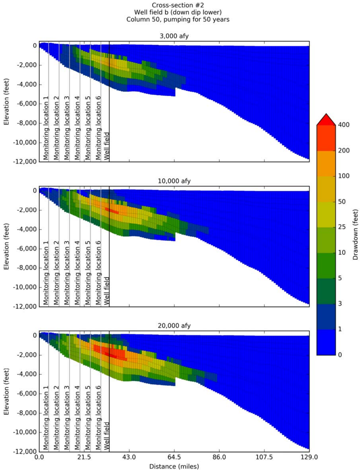
Figure 14-45. Simulated drawdown at 50 years after pumping the Well Field #2b located along Cross-Section #2 on Figure 14-5 at 3,000 acre-feet per year, 10,000 acre-feet per year, and 20,000 acre-feet per year.
