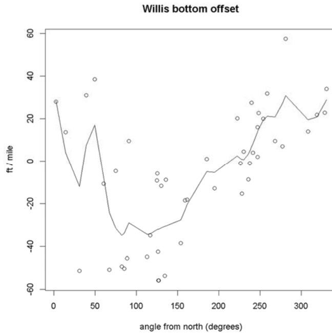
Figure 13-14. Offset of the Willis Formation bottom between paired water well and geophysical log(s) assigned to the Willis Formation calculated as a function of orientation angle.
