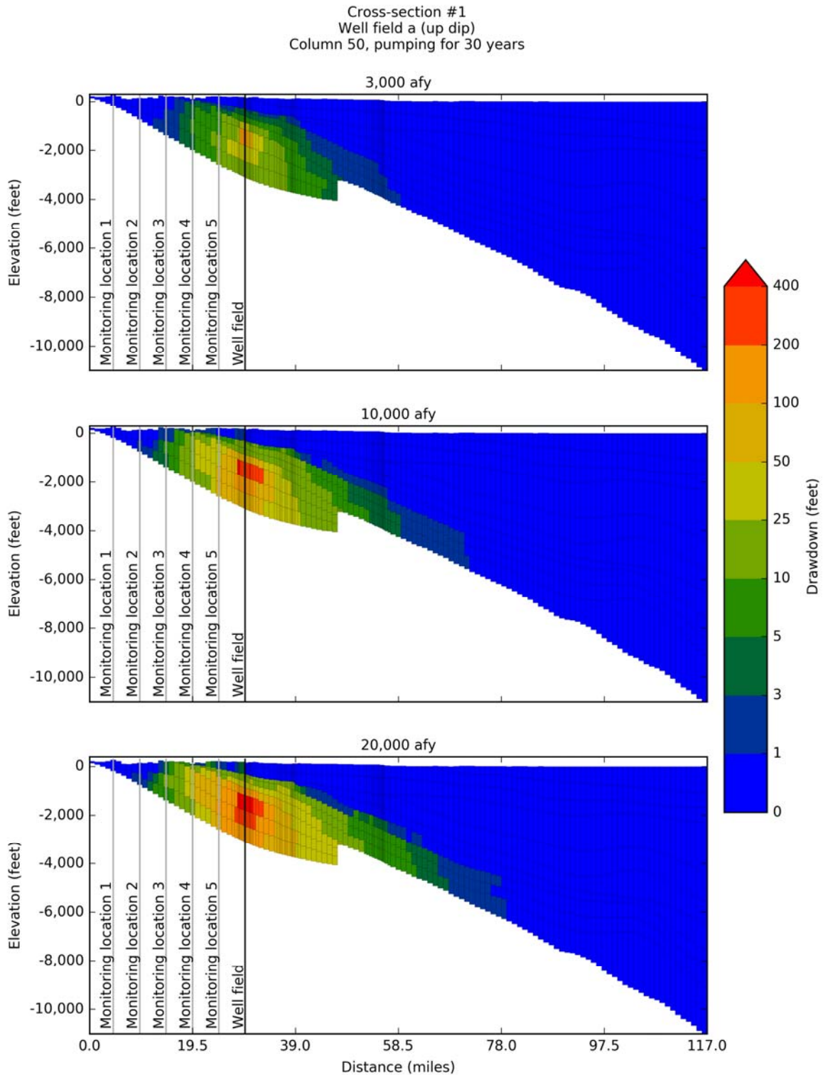
Figure 14-30. Simulated drawdown at 30 years after pumping the up dip Well Field #1a located along Cross-Section #1 on Figure 14-5 at 3,000 acre-feet per year, 10,000 acre-feet per year, and 20,000 acre-feet per year.
