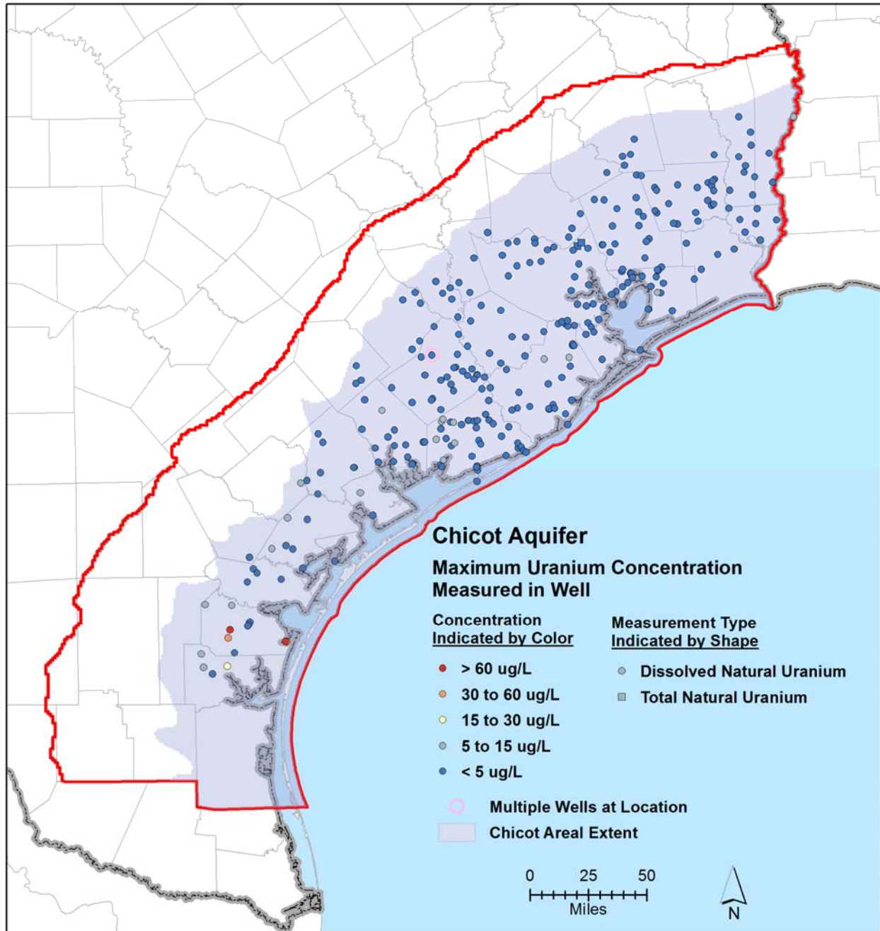
Figure 10-22. Maximum uranium concentration in the Chicot Aquifer.
