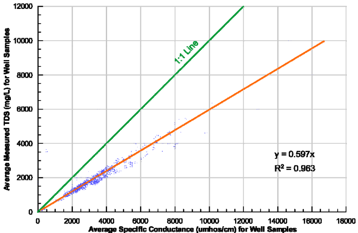
Figure 13-8. Linear regression between specific conductance and total dissolved solids concentration for 587 groundwater samples where chloride comprises at least 35 percent of the equivalence in the charge balance where (a) total dissolved solids concentration is measured and (b) total dissolved solids concentration is calculated.
