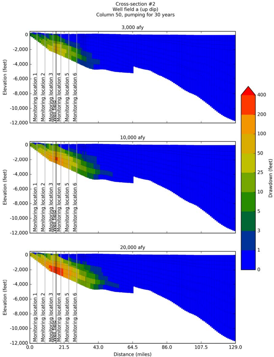
Figure 14-42. Simulated drawdown at 30 years after pumping the up dip Well Field #2a located along Cross-Section #2 on Figure 14-5 at 3,000 acre-feet per year, 10,000 acre-feet per year, and 20,000 acre-feet per year.
