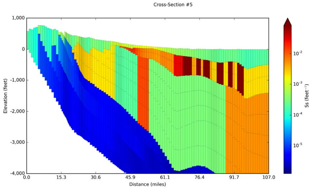
Figure 14-77. Specific storage (Ss) values in the groundwater model for Cross-Section #5 on Figure 14-5 with for model layers 1 to 12.
