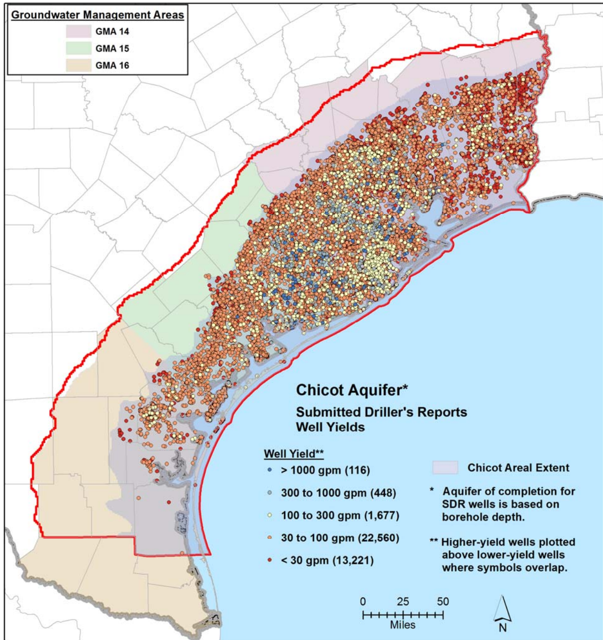
Figure 9-1. Reported well yields for the Chicot Aquifer based on well information obtained from the TWDB Submitted Drillers Reports.
