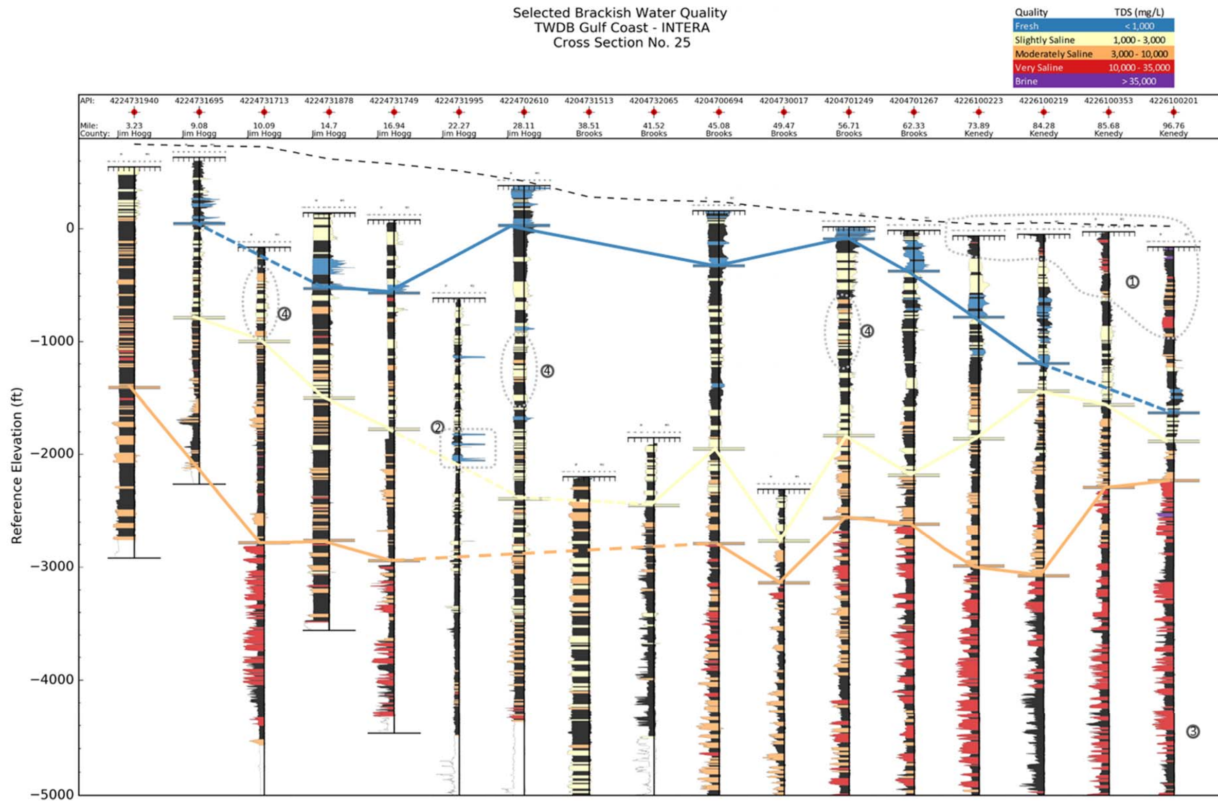
Figure 6-28. Profiles of calculated salinity zones for sand beds identified on geophysical logs aligned on Cross-Section #25 shown in Figure 6-1. Markers represent the base of the salinity zones at each log location. The lines connecting the markers are for illustrative purposes only. Dashed line indicates crossing a log with no marker available in an active interval.
