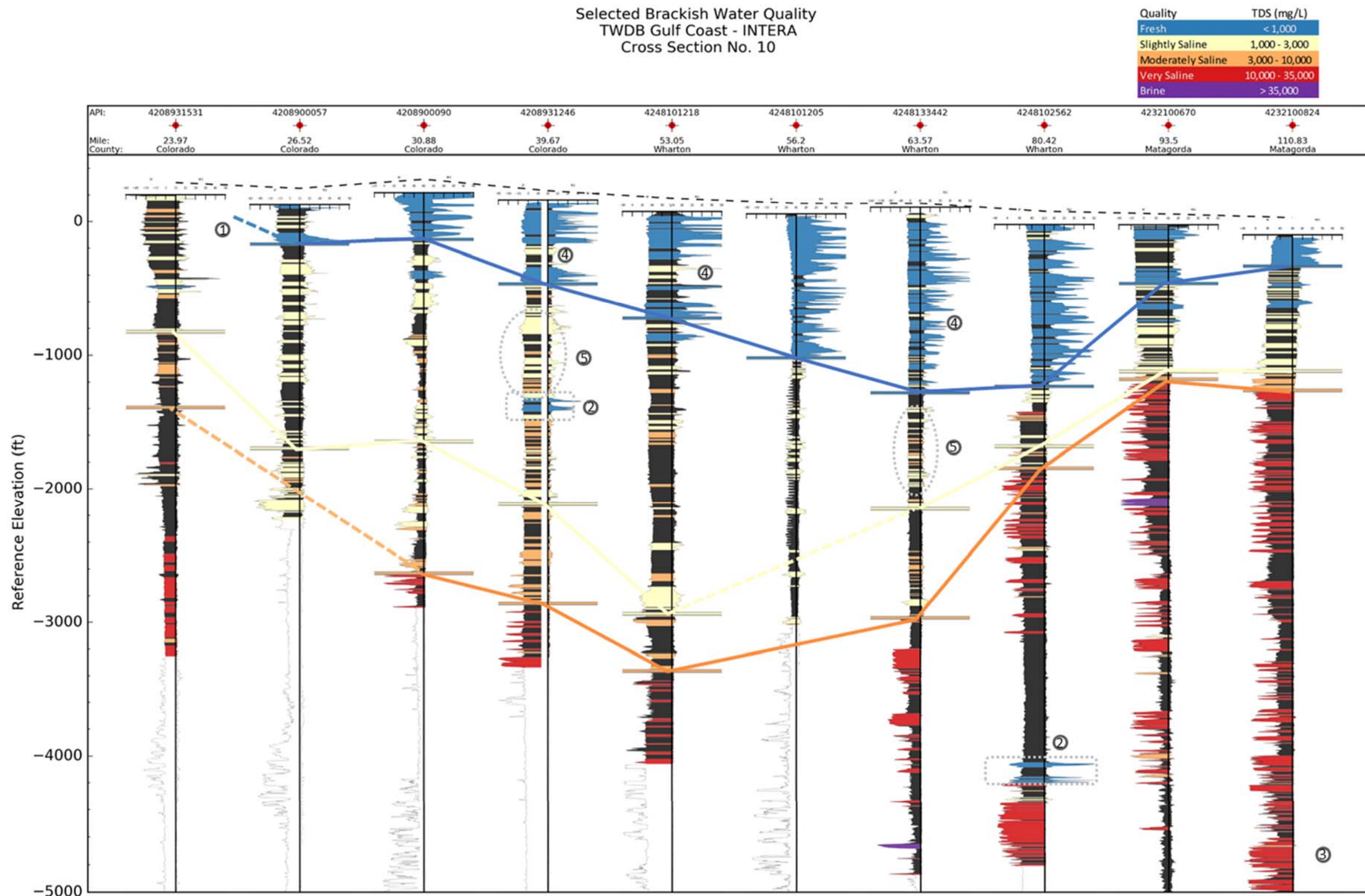
Figure 6-18. Profiles of calculated salinity zones for sand beds identified on geophysical logs aligned on Cross-Section #10 shown in Figure 6-1. Markers represent the base of the salinity zones at each log location. The lines connecting the markers are for illustrative purposes only. Dashed line indicates crossing a log with no marker available in an active interval.
