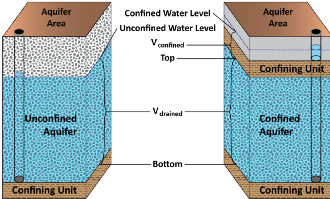
Figure 12-1. Schematic graph showing the difference between unconfined and confined aquifers (from Jigmond and Wade, 2013).
