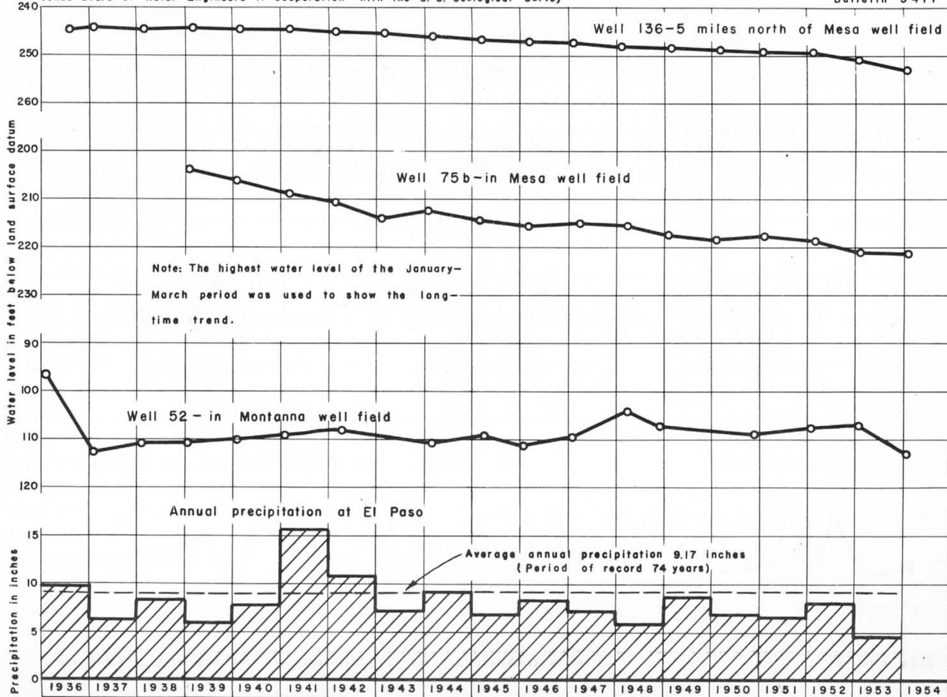
Hydrographs showing fluctuation of water levels in El Paso County wells and the annual precipitation at El Paso, Tex.
