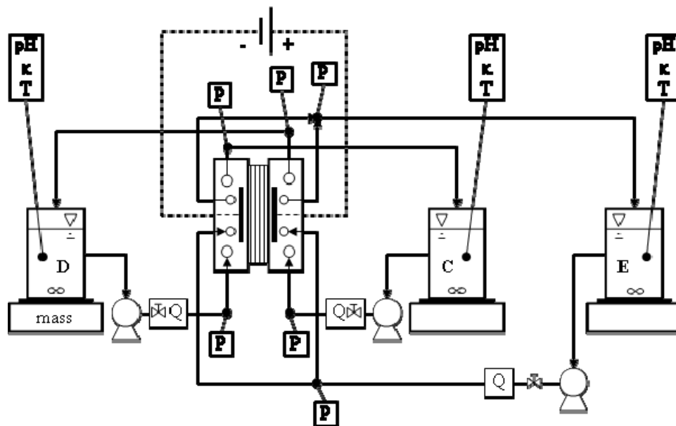
Figure 4-6. Schematic of batch-recycle experimental ED apparatus.
