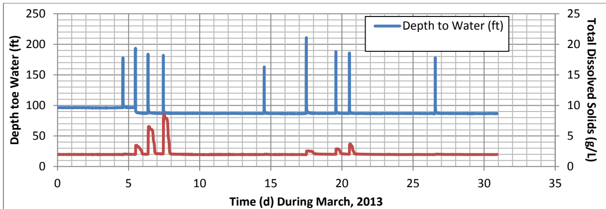
Figure 1. Depth to water and total dissolved solids variations from February 8 to 28, 2013
